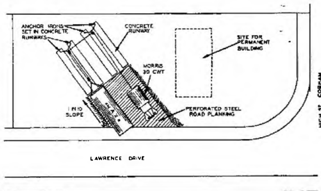
SITE PLAN SHOWING METHOD OF DRAWING-IN M.A.X.
