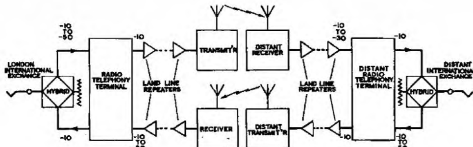
NOTE:—LEVELS ARE IN dB RELATIVE TO REFERENCE TELEPHONE POWER. FIG. 2.—BLOCK SCHEMATIC DIAGRAM OF LONG-DISTANCE RADIO TELEPHONE CIRCUIT.
