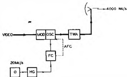
FIG. 2.—BLOCK SCHEMATIC DIAGRAM OF TERMINAL TRANSMITTER.
