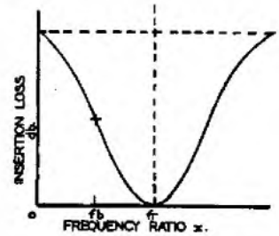
FIG. 3.—INSERTION-LOSS/FREQUENCY CHARACTERISTIC FOR EQUALISER SHOWN IN FIG. 2.
