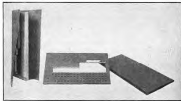
FIG. 3.—COMPLETED KEYSHELF.
