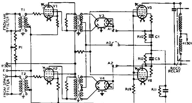
FIG. 8.—TWO-TONE DETECTOR.
