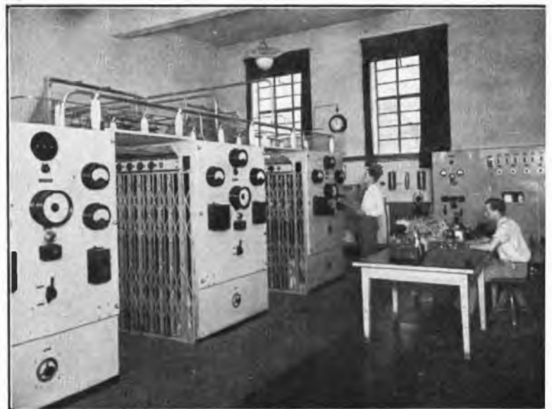
FIG. 5.—HIGH-POWER AMPLIFIER STAGE OF V.L.F. TRANSMITTER.
