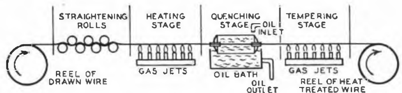
FIG. 1.—HEAT TREATMENT OF CONTINUOUS ROD.
