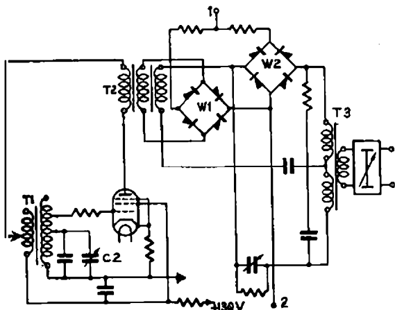
FIG. 7.—OSCILLATOR MODULATOR.
