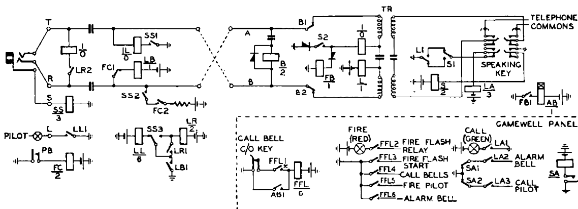
FIG. 4.—SIMPLIFIED CIRCUIT SHOWING HEADQUARTERS AND STATION TERMINATIONS.
