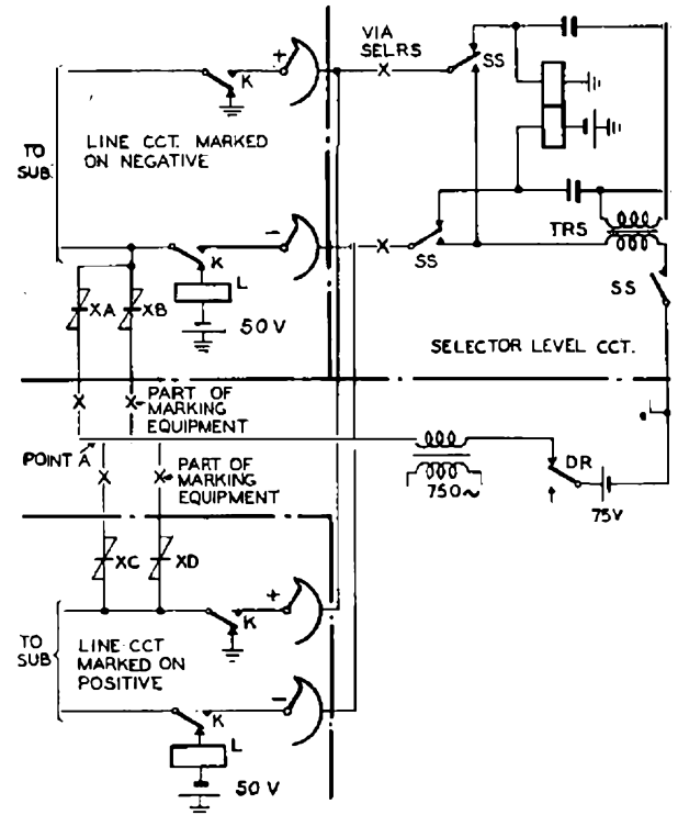
FIG. 3.—SWITCHING OF MARKING SIGNALS TO LINE CIRCUIT:
