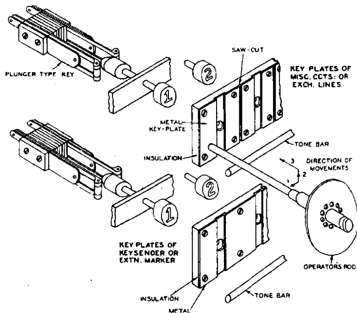
FIG. 1.—MECHANICAL ARRANGEMENT OF KEYBOARD.
