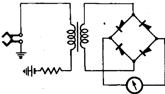
FIG. 1.—SPEED MEASURING ELEMENT.
