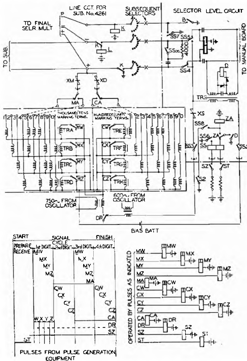
FIG. 4.—TRANSMISSION OF IDENTIFICATION SIGNAL.
