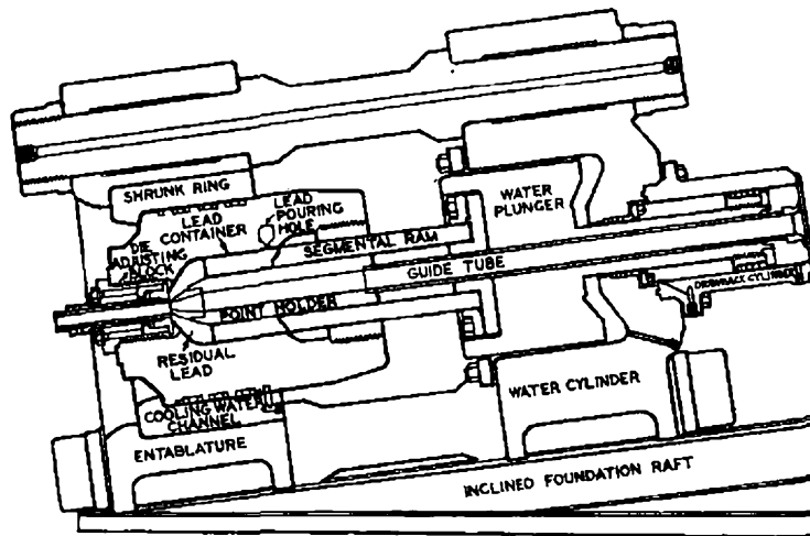
FIG. 3.—HENLEY STRAIGHT-THROUGH LEAD PRESS.
