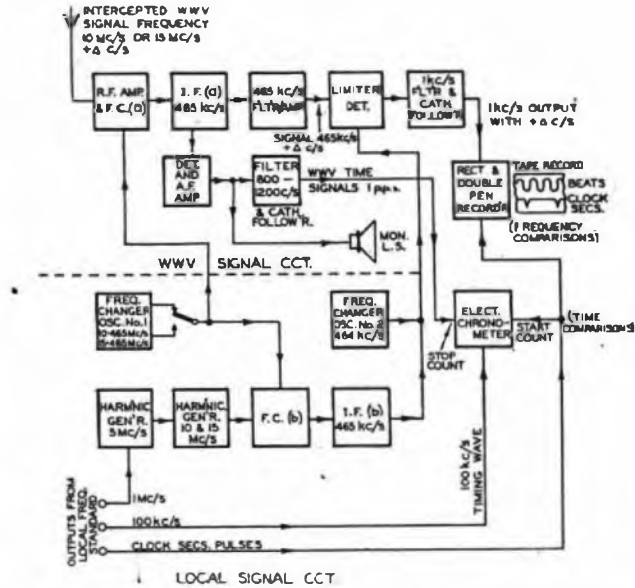
FIG. 4.—ARRANGEMENT OF EQUIPMENT FOR THE RECEPTION AND MEASUREMENT OF WWV SIGNALS.
