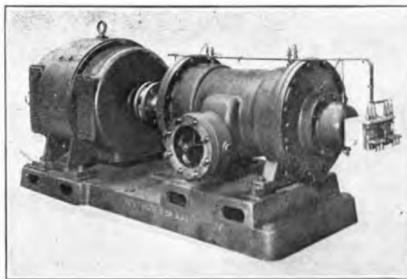
FIG. 6.—COMPRESSOR SET.
