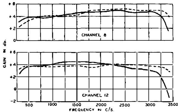
FIG. 13.—OVERALL GAIN/FREQUENCY RESPONSE OF CHANNELS.
