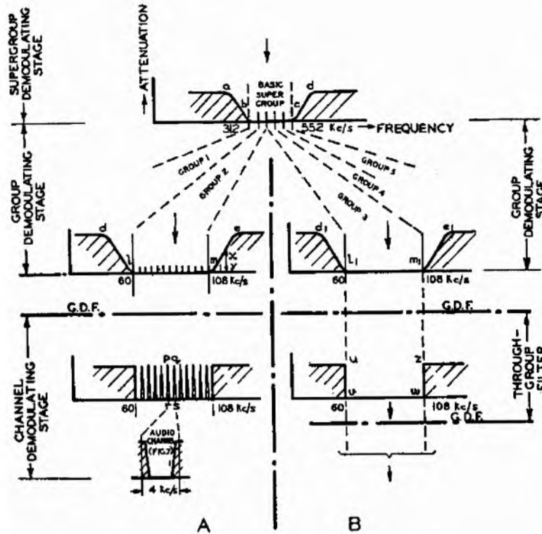
FIG. 4.—SIGNAL FREQUENCY BANDS IN DEMODULATING STAGES OF A COAXIAL TERMINAL.
