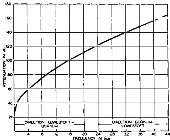
FIG. 3.—CABLE ATTENUATION.
