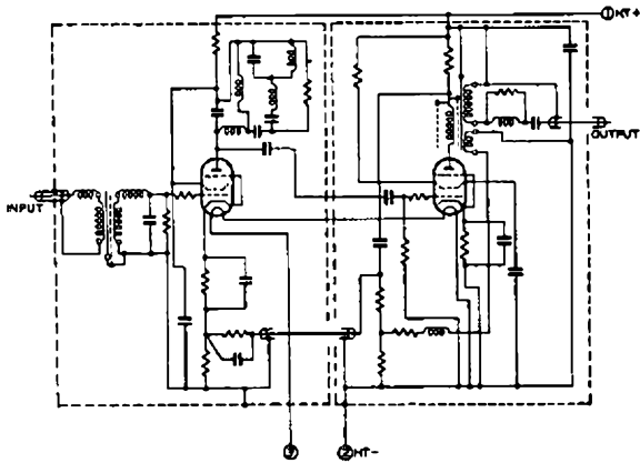
FIG. 10.—CIRCUIT SCHEMATIC OF SUBMERGED REPEATER.
