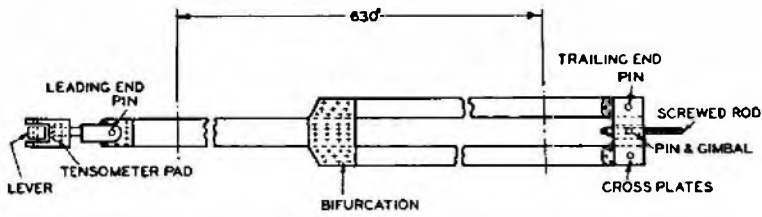
FIG. 1.—DEVELOPMENT OF BRAKE BAND SHOWING END FIXINGS.
