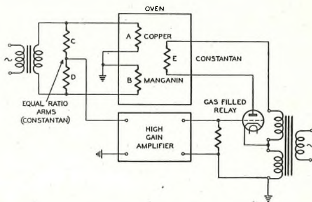
FIG. 4.—50 c/s BRIDGE CONTROL CIRCUIT.
