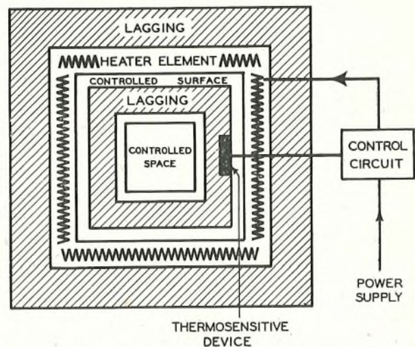
FIG. 1.—SCHEMATIC DIAGRAM OF AN ELECTRIC THERMOSTAT.
