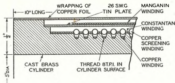
FIG. 8.—CROSS SECTION OF WINDINGS OF BRIDGE THERMOSTAT.
