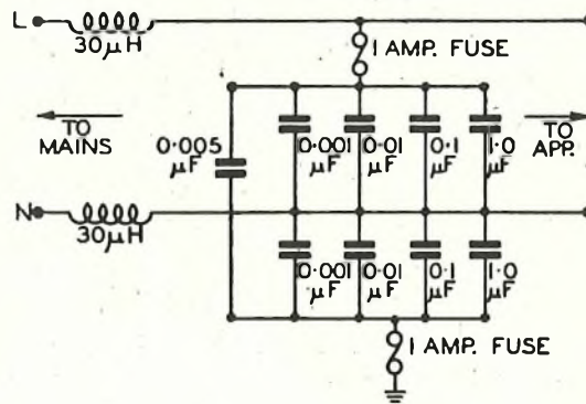
FIG. 3.—FILTER CIRCUIT FOR USE WITH HIGH FREQUENCY APPARATUS.
