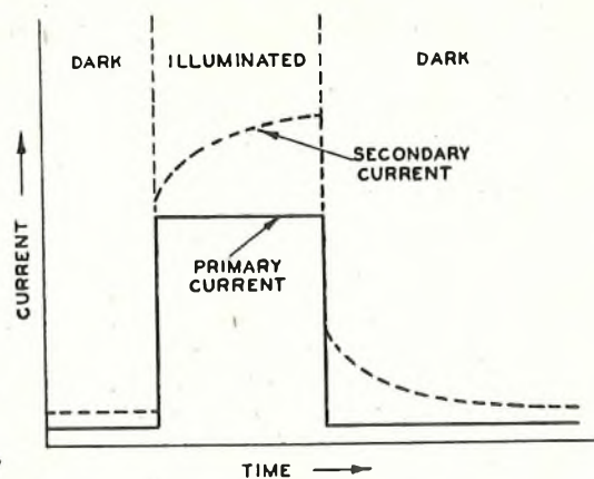
FIG. 5.—PHOTOELECTRIC EFFECT IN COLOURED ALKALI HALIDES.
