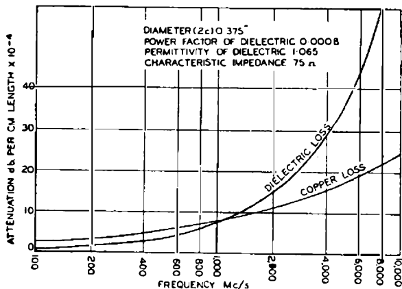
FIG. 6.—THEORETICAL ATTENUATION OF AIR SPACE SINGLE COAXIAL CABLE.
