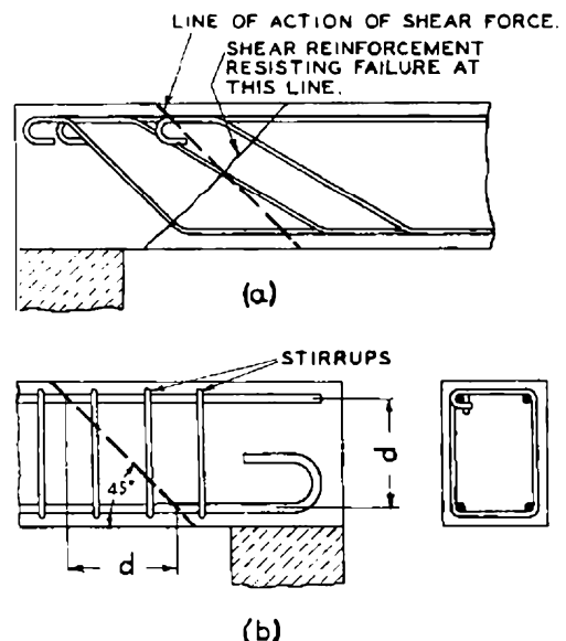
FIG. 4.—SHEAR REINFORCEMENT.
