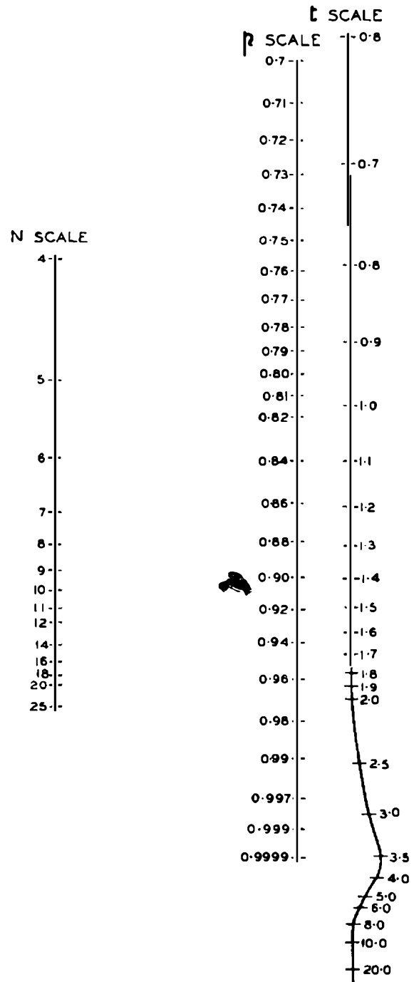
FIG. 2.—PROBABILITY CHART FOR "t" TEST.
