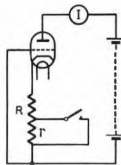
FIG. 7.—PRINCIPLE OF VALVE TEST.
