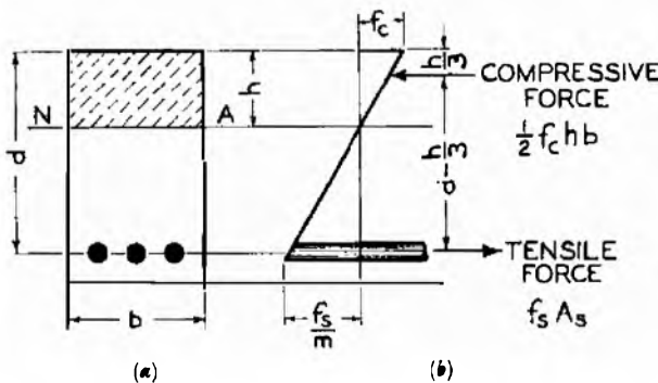
FIG. 1.—STRESS DIAGRAM.
