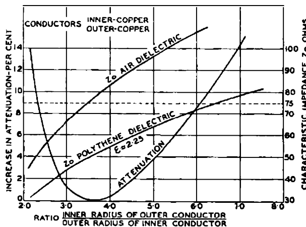
FIG. 3.—CHARACTERISTICS OF COAXIAL CABLES WITH COPPER CONDUCTORS.
