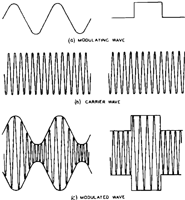
FIG. 1.—AMPLITUDE MODULATION BY SINGLE SINE WAVE AND BY RECTANGULAR PULSE. LATTER CASE MAY BE COMPARED WITH FIGS. 2 AND 3.
