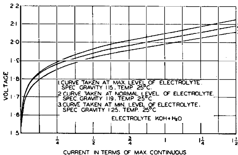
FIG. 2.—VOLTAGE CHARACTERISTICS OF CELL.
