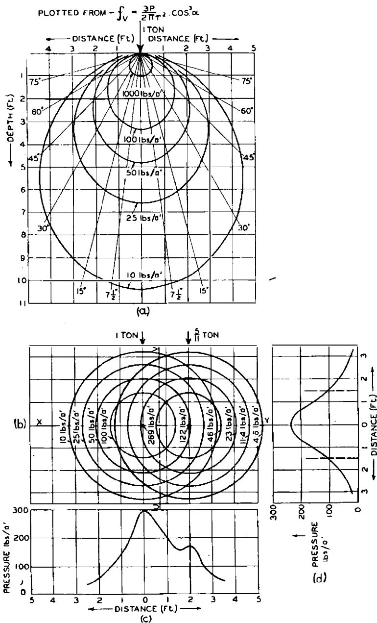
FIG. 11.—EQUIVALENT UNIFORM PRESSURE AT VARIOUS DEPTHS.
