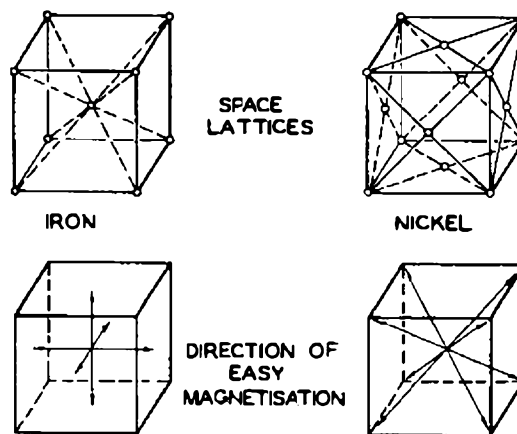
FIG. 2.—SPACE LATTICES AND DIRECTIONS OF EASY MAGNETISATION IN CRYSTALS OF IRON AND NICKEL.
