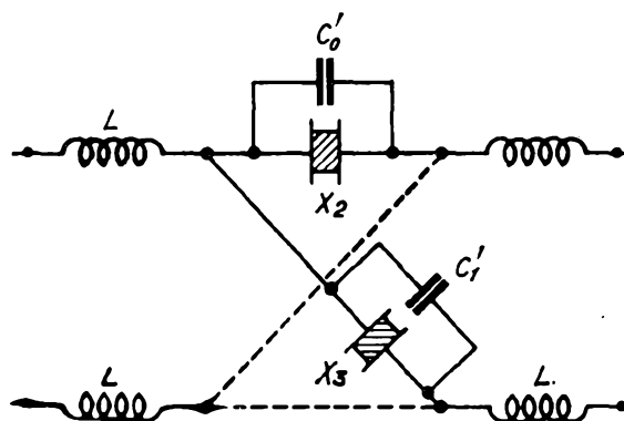
FIG. 5.—CHANNEL FILTER SECTION.
