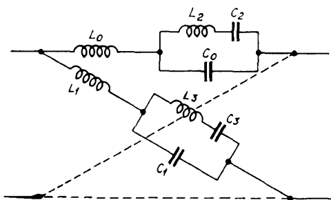
FIG. 3.—FILTER SECTION.
