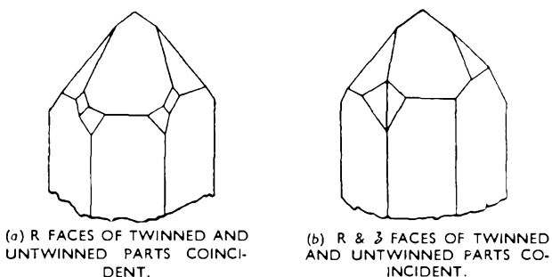
FIG. 9.—TWO TYPES OF PERFECT INTERPENETRANT CHIRAL TWIN.
