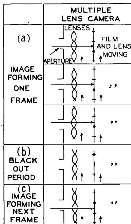
FIG. 2.—OPTICAL PRINCIPLE OF MULTIPLE LENS CINEMATOGRAPH CAMERA.
