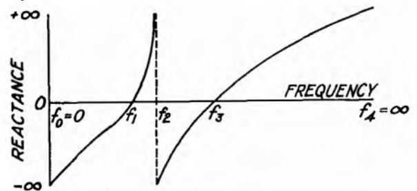
FIG. 10.—REACTANCE-FREQUENCY CHARACTERISTIC.
