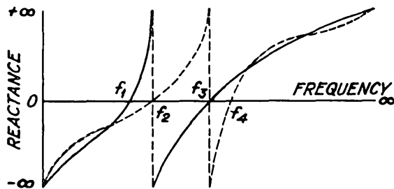
FIG. 6.—REACTANCE-FREQUENCY CHARACTERISTIC OF FILTER ARMS.
