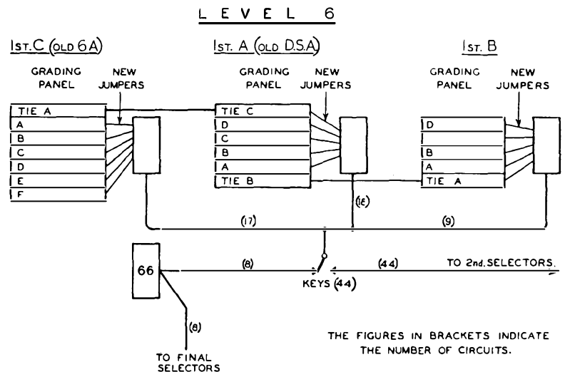
FIG. 4.—CHANGE-OVER ARRANGEMENTS FOR LEVEL 6.
