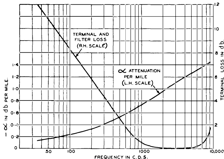
FIG. 6.—CABLE AND TERMINAL LOSSES PER CABLE SECTION.
