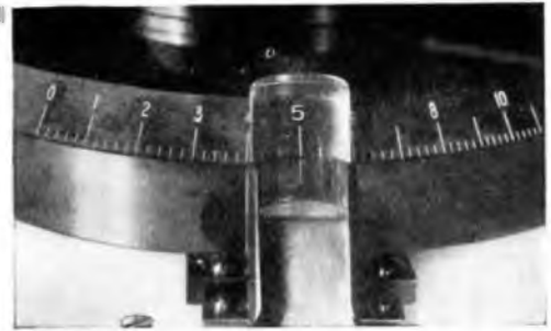
Illustrating the great openness of scale and the simple magnifier employed on this bridge to facilitate rapid reading with accuracy.
