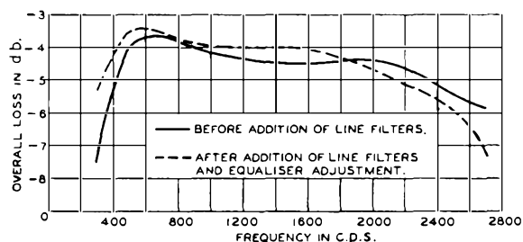
FIG. 5.—EFFECT ON CARRIER CHANNEL NO. 1
