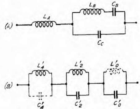
FIG. 9.—ILLUSTRATION OF NETWORK TRANSFORMATION.
