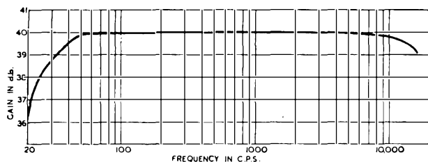
FIG. 3.—GAIN-FREQUENCY CHARACTERISTIC.
