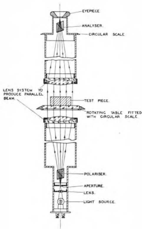
FIG. 10.—POLARISCOPE.
