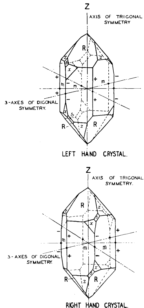
FIG. 1.—RIGHT AND LEFT HAND CRYSTALS.
