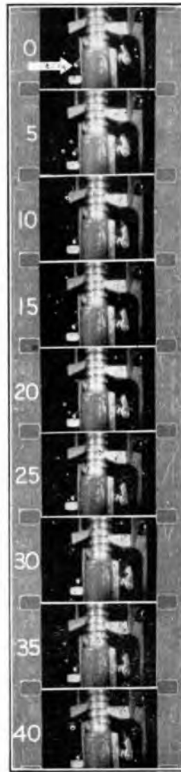
FIG. 7—EXTRACT FROM FILM SHOWING REBOUND OF AUTOMATIC SELECTOR PAWL.
