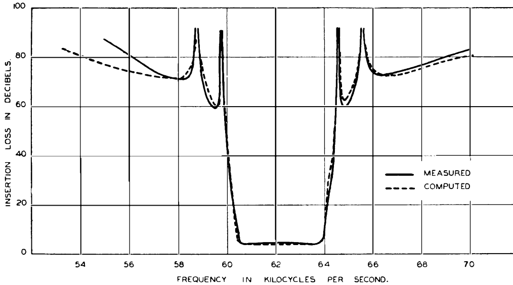
FIG. 11.—COMPARISON OF MEASURED AND COMPUTED INSERTION LOSS.
