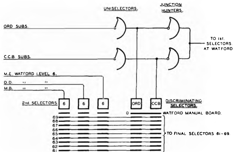
NOTE. THE DISCRIMINATING SELECTORS ABSORB "6" AS A FIRST DIGIT. FIG. 1.—TRUNKING DIAGRAM OF RADLETT SATELLITE EXCHANGE
