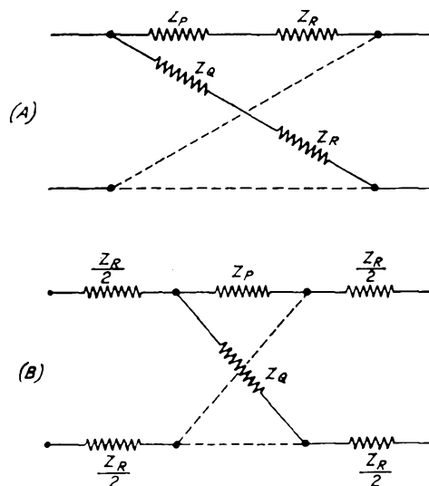
FIG. 4.—EQUIVALENT NETWORKS.
