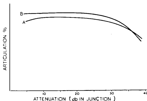
FIG. 5.—COMPARISON OF TWO MICROPHONES.
