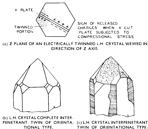
FIG. 6.—EXAMPLES OF PURE ELECTRICAL TWINNING.
