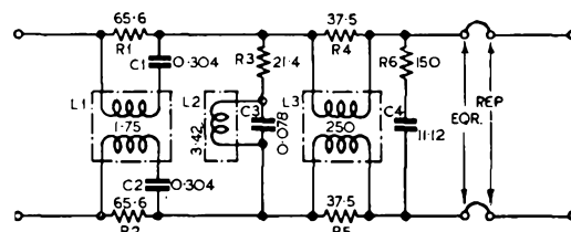
FIG. 7.—TYPICAL EQUALISER CIRCUIT.
