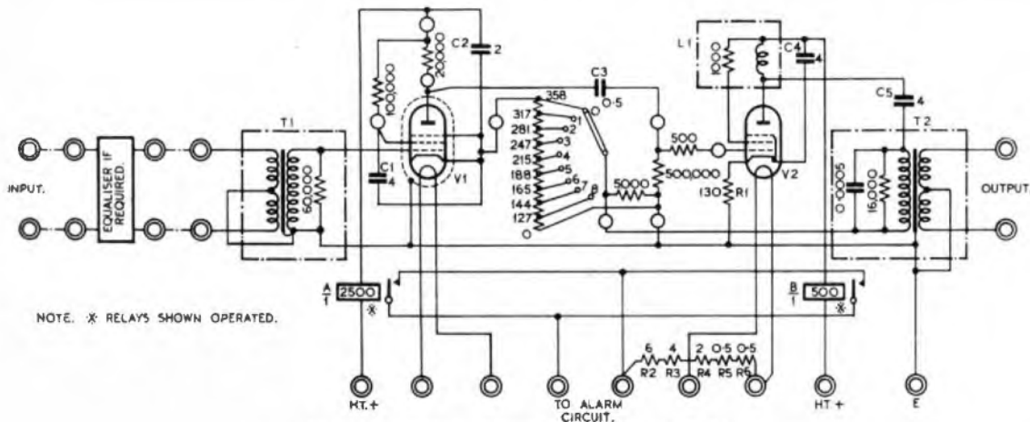
FIG. 2.—CIRCUIT OF UNIT AMPLIFYING No. 24.
