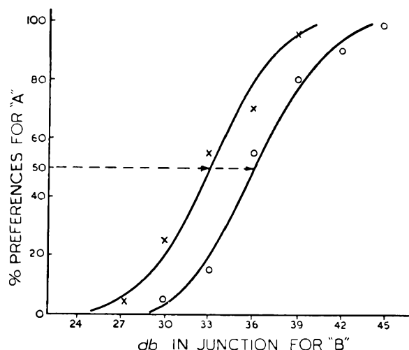
FIG. 4.—PERCENTAGE PREFERENCES FOR ONE OF TWO MICROPHONES.
