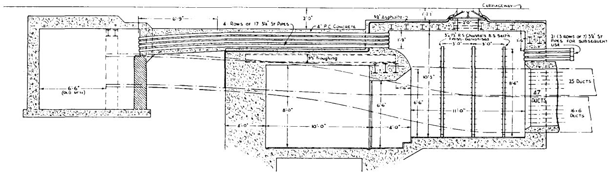
ENLARGED SECTION ON A-A. SHOWING ARRANGEMENT OF 68 3/4" TUBES.
