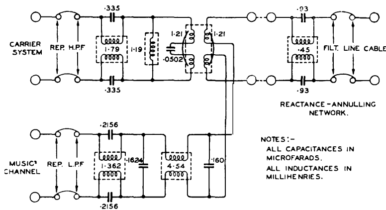
FIG. 2.—LINE FILTERS—CIRCUIT DIAGRAM.
