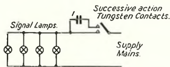
FIG. 14.—SPARK QUENCHING CIRCUIT.
