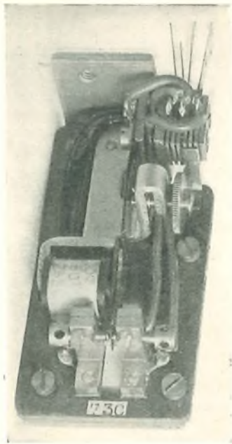
FIG. 13.—" RIGHT-OF-WAY " RELAY.
