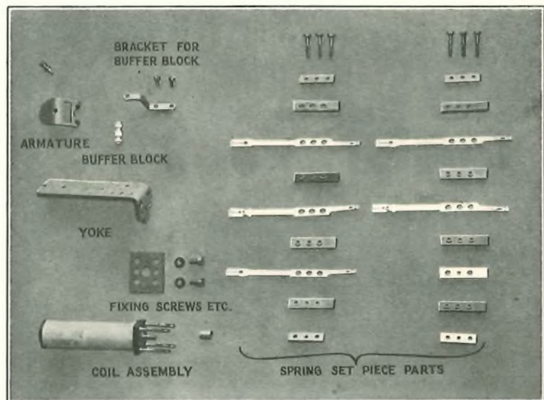
FIG. 2.—COMPONENT PARTS.
