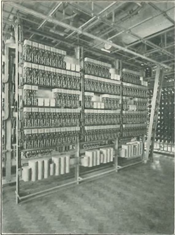
FIG. 7.—LINE FINDER RACKS, CENTRAL EXCHANGE.
