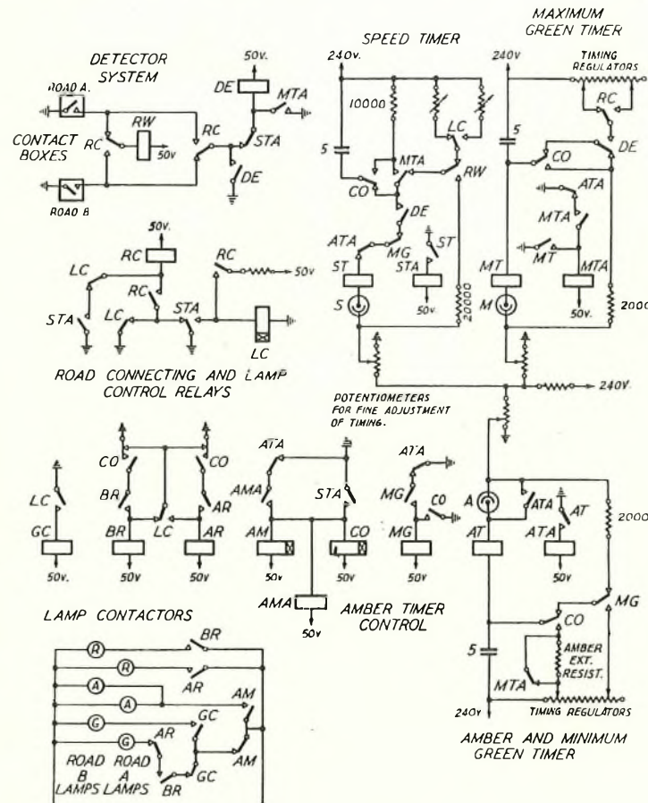
FIG. 17.—BASIC CIRCUIT OF AUTOFLEX TWO-PART CYCLE CONTROLLER.
