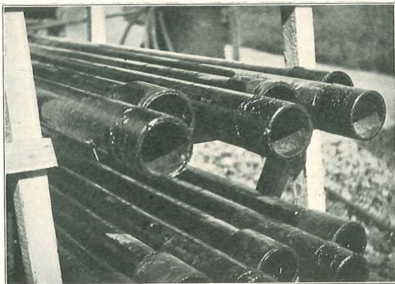
FIG. 5.—DUCTS WITH JOINTING COMPOUND APPLIED.
