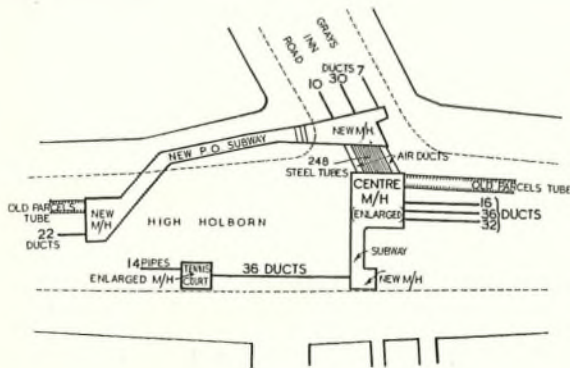
FIG. 4.—PLAN OF HOLBORN AFTER THE DIVERSIONS.
