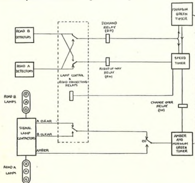
FIG. 15.—PRINCIPLE OF AUTOFLEX CONTROLLER CIRCUIT.
