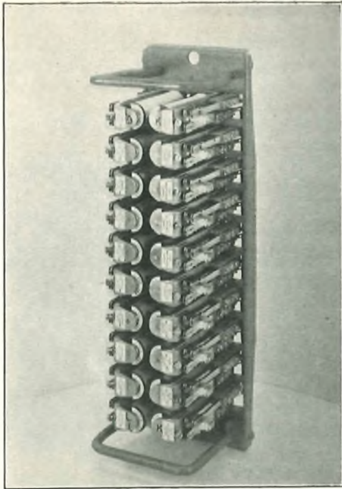
FIG. 3.—VERTICAL MOUNTING.
