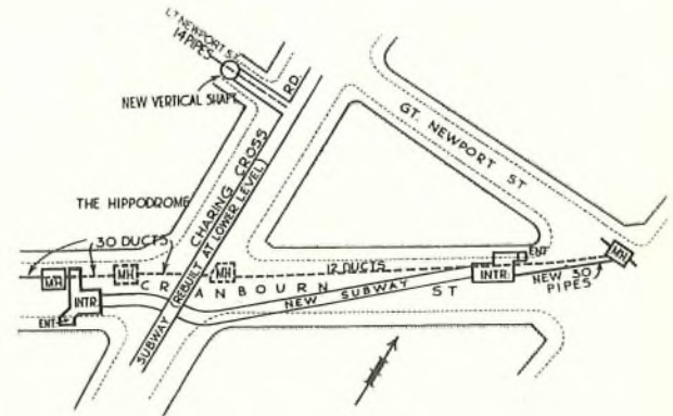
FIG. 13.—PLAN SHOWING DEPARTMENT'S PLANT, LEICESTER SQUARE STATION.
