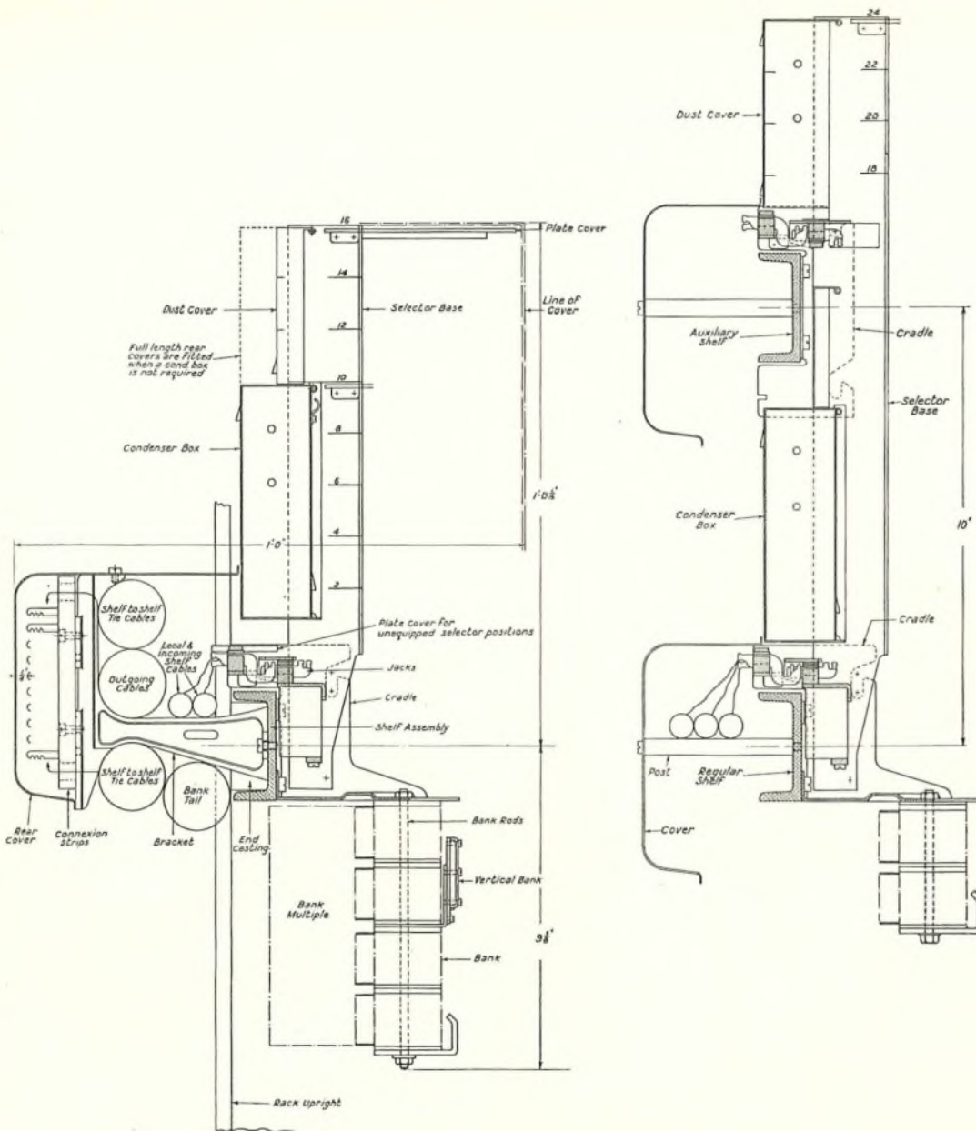
FIG. 1.—TYPICAL VIEWS OF SELECTOR MOUNTING ARRANGEMENTS.
