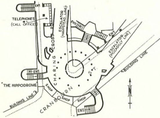
FIG. 11.—LEICESTER SQUARE TUBE STATION, NEW BOOKING HALL.
