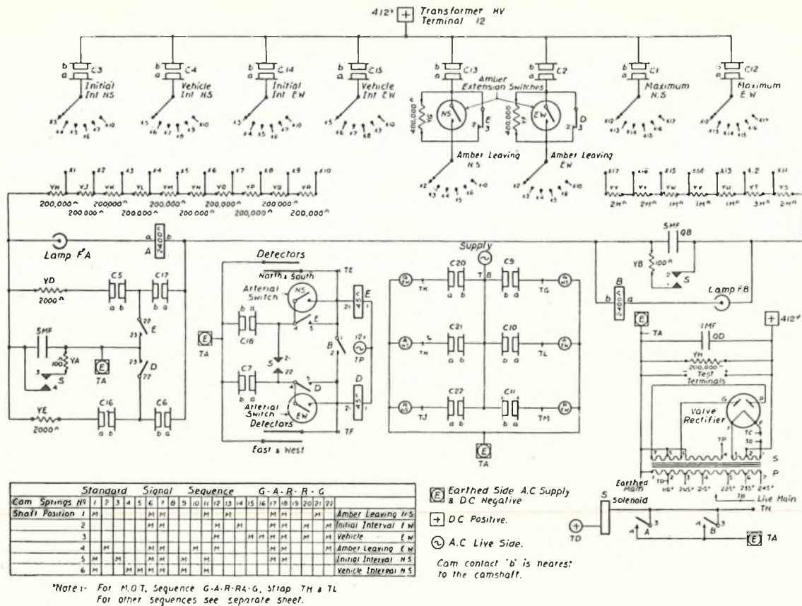
FIG. 8.—ELECTROMATIC CONTROLLER CIRCUIT.
