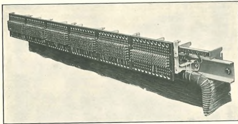
FIG. 5(b).—REAR OF SHELF WITH COVER REMOVED.
