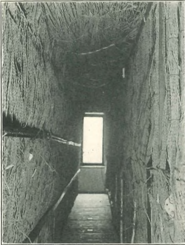
FIG. 3.—M.D.F., OLD BELFAST CENTRAL EXCHANGE.
