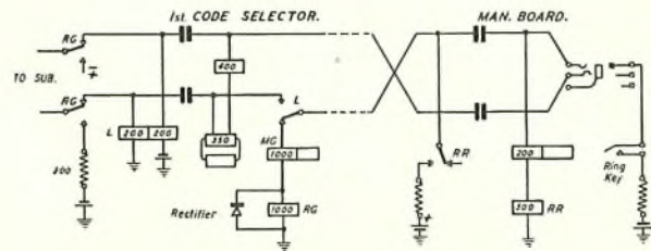
FIG. 4.—RE-RINGING FACILITY.
