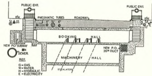
FIG. 6.—CROSS SECTION OF HOLBORN AFTER THE DIVERSIONS.
