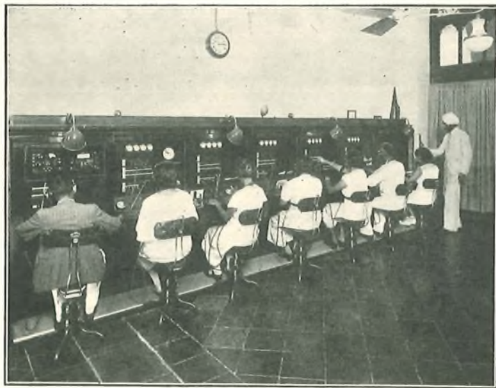
FIG. 2.—TRUNK SWITCHBOARD.
