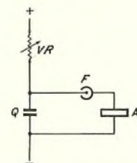
FIG. 4.—PRINCIPLE ELECTROMATIC TIMING CIRCUIT.
