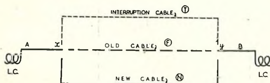
FIG. 10.—SUBSTITUTION METHOD OF REBALANCING.
