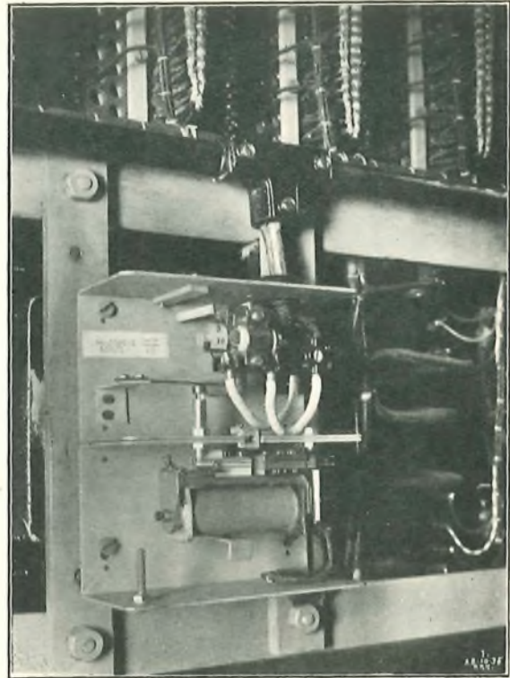
FIG. 9.—MERCURY RELAY SWITCH.
