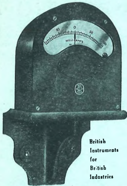
T. 1088 WALL MOUNTING TYPE.
