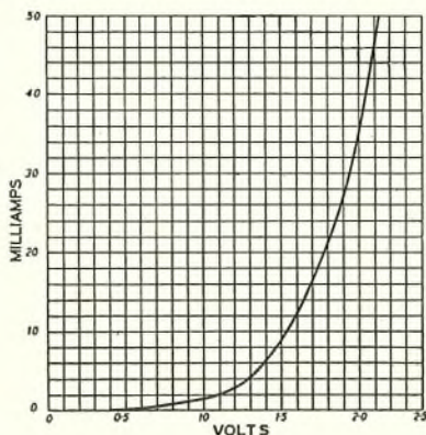
FIG. 2.—VOLTAGE-CURRENT CURVE, FORWARD DIRECTION.
