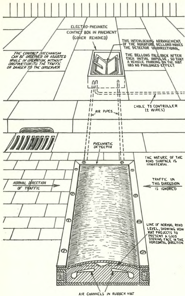
FIG. 2.—PNEUMATIC DETECTOR.
