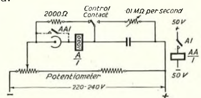
FIG. 12.—AUTOFLEX BASIC TIMING CIRCUIT.
