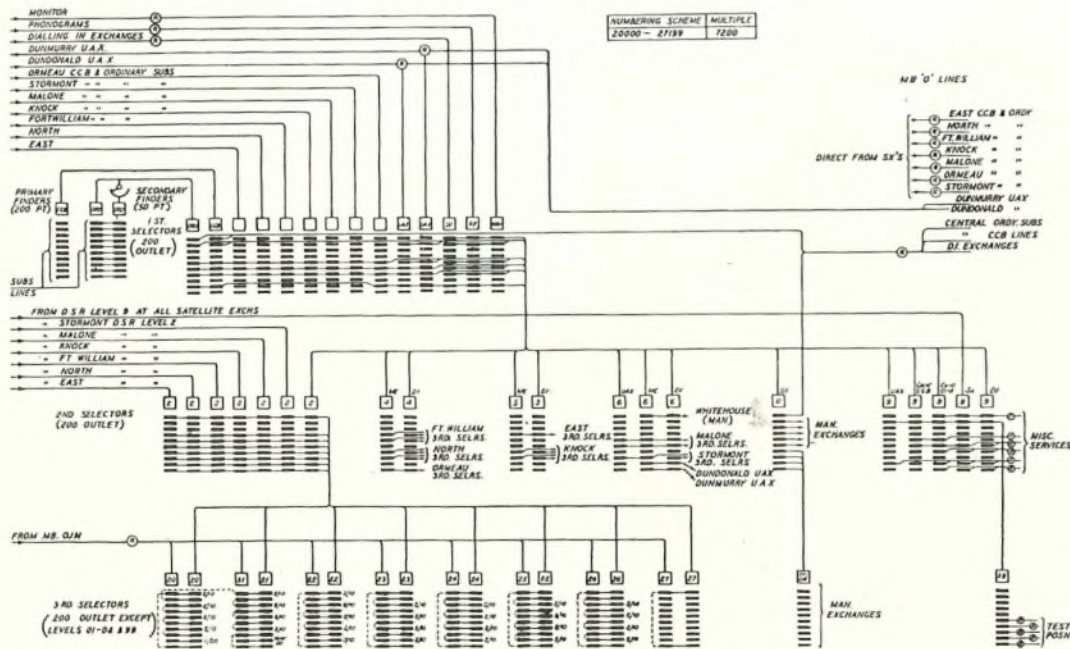
FIG. 13.—TRUNKING DIAGRAM, CENTRAL EXCHANGE.
