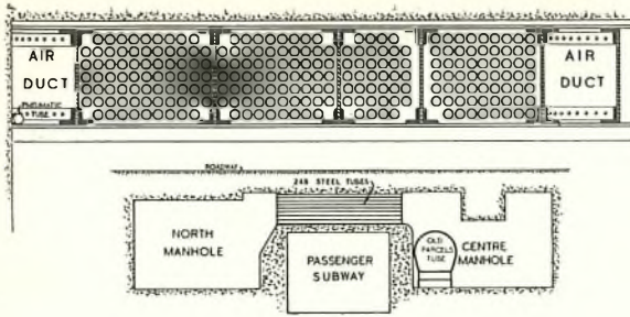
FIG. 7.—ACCOMMODATION OF STEEL PIPES OVER PASSENGER SUBWAY.
