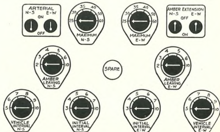
FIG. 7.—ELECTROMATIC CONTROLLER.
