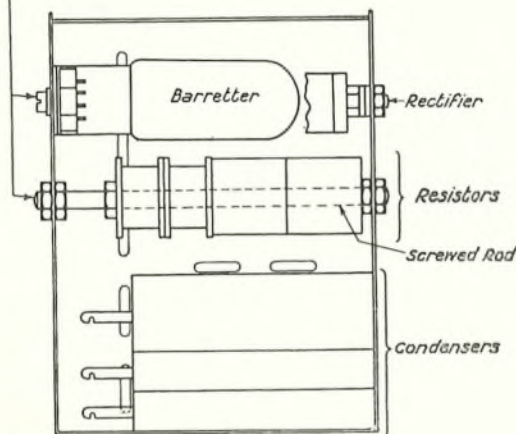
FIG. 2.—CONDENSER BOX—MIXED EQUIPMENT.
