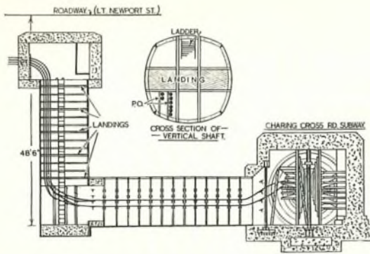
FIG. 19.—NOVELTY HEADING AND VERTICAL SHAFT AT LITTLE NEWPORT STREET.
