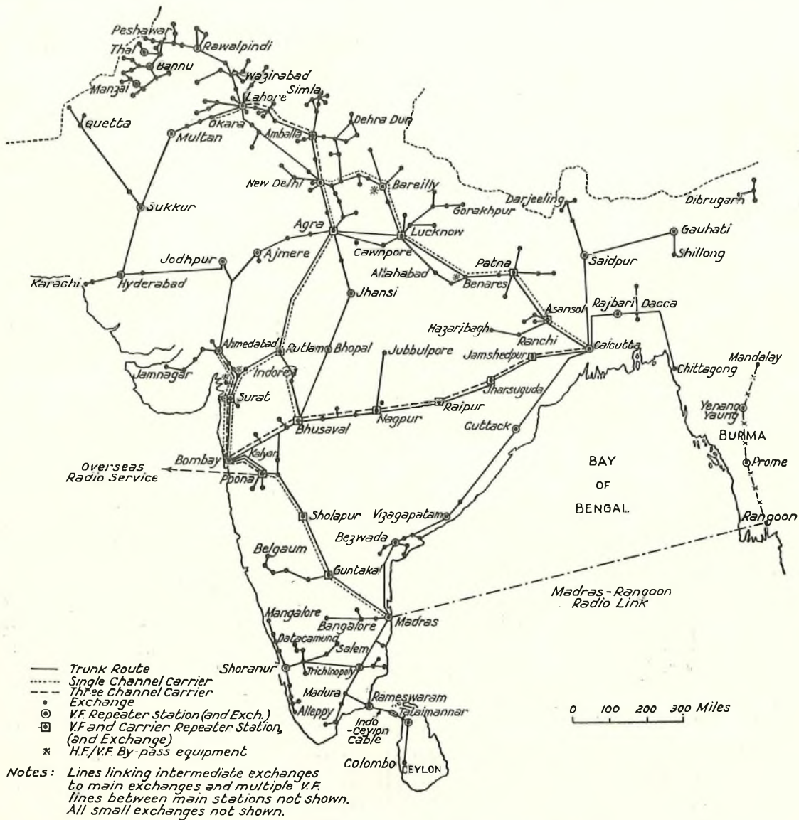
FIG. 1.—LONG DISTANCE TELEPHONE SYSTEM OF INDIA.
