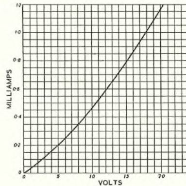
FIG. 3.—VOLTAGE-CURRENT CURVE, BACKWARD DIRECTION.
