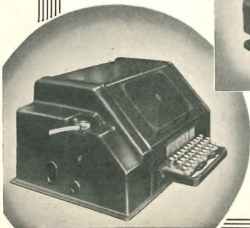
Model No. 3a Tape Teleprinter
