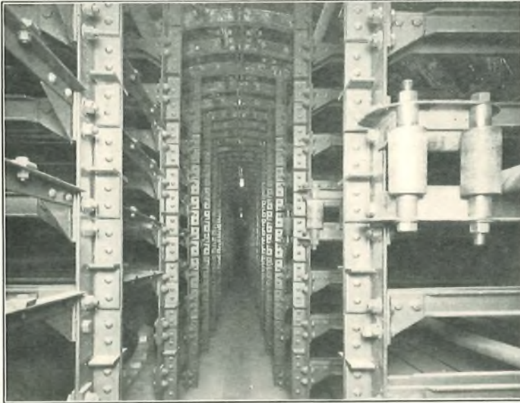
FIG. 17.—NEW L.C.C. SUBWAY.
