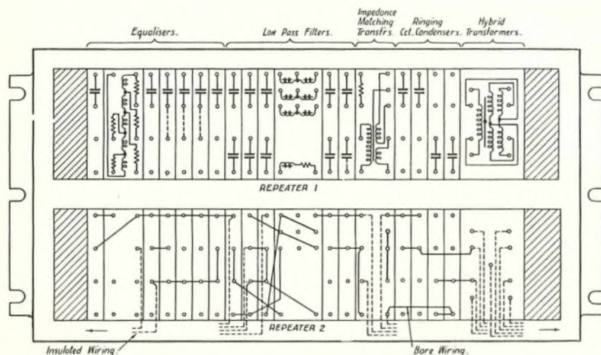
FIG. 4.—REPEATER PANEL, REAR VIEW.
