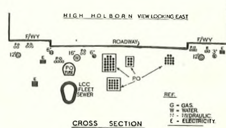
FIG. 2.—LAY-OUT OF PLANT BEFORE DIVERSION.
