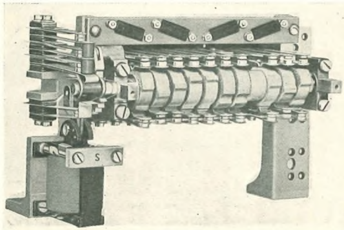
FIG. 9.—SOLENOID OPERATED CAM SHAFT.
