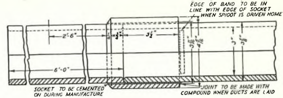
FIG. 2.—JOINT BETWEEN TWO PIPES.
