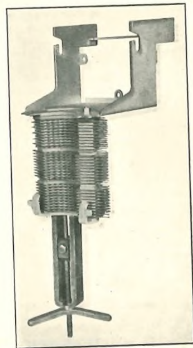
FIG. 8.—BANK ROD EXTRACTOR.
