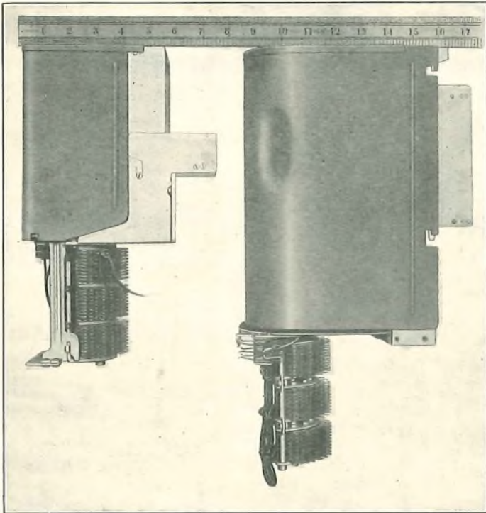
FIG. 1.—COMPARATIVE SIZES OF 2000 AND STROWGER SELECTORS.
