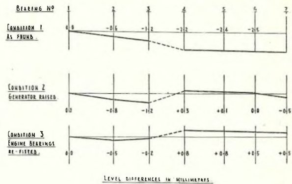
FIG. 3.—BEARING LEVELS.
