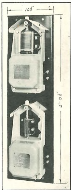
FIG. 3.—CARBON PILE VOLTAGE REGULATOR.
