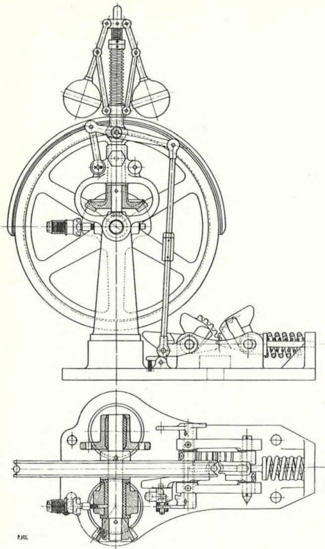
FIG. 6.—CENTRIFUGAL GOVERNOR.
