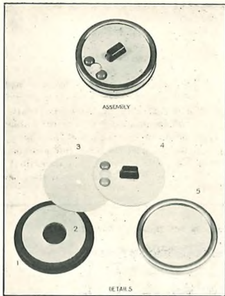
FIG. 7.—PALLADIUM CHLORIDE GAS INDICATOR.
