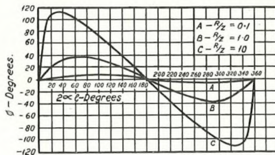
FIG. 2.—VARIATION OF ERROR WITH PHASE CHANGE AND WITH MAGNITUDE OF FAULT.
