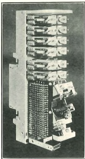
FIG. 5.—MULTI-METERING RELAY SET.
