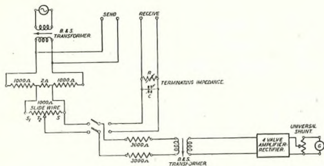
FIG. 1.—CONNEXIONS OF VISUAL CROSS-TALK SET.
