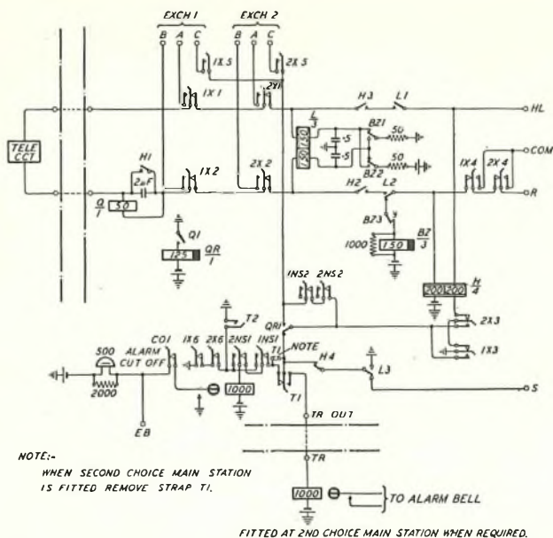
FIG. 10.—Circuit of External Extension Unit, Used on Installations with Two Exchange Lines.
