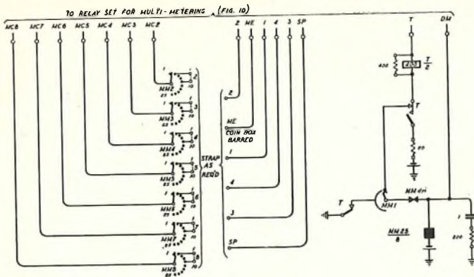
FIG. 11.—COMMON MULTI-METERING SET.
