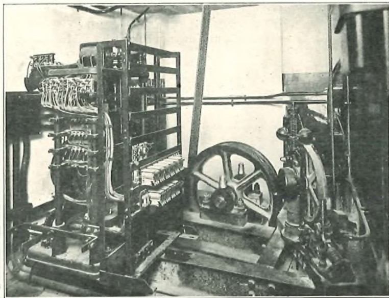
FIG. 10.—FLOOR SELECTOR.
