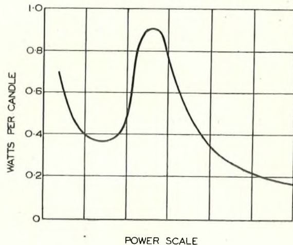
FIG. 1.—VARIATION IN WATTS PER CANDLE OF A QUARTZ MERCURY ARC LAMP.
