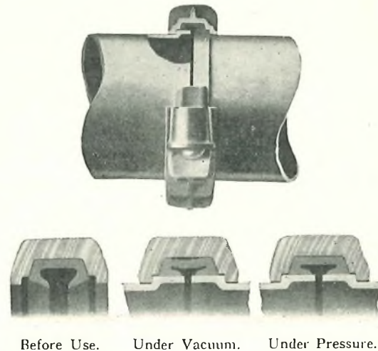
FIG. 2.—MECHANICAL JOINT SHOWING SECTIONS THROUGH HOUSINGS AND RINGS.
