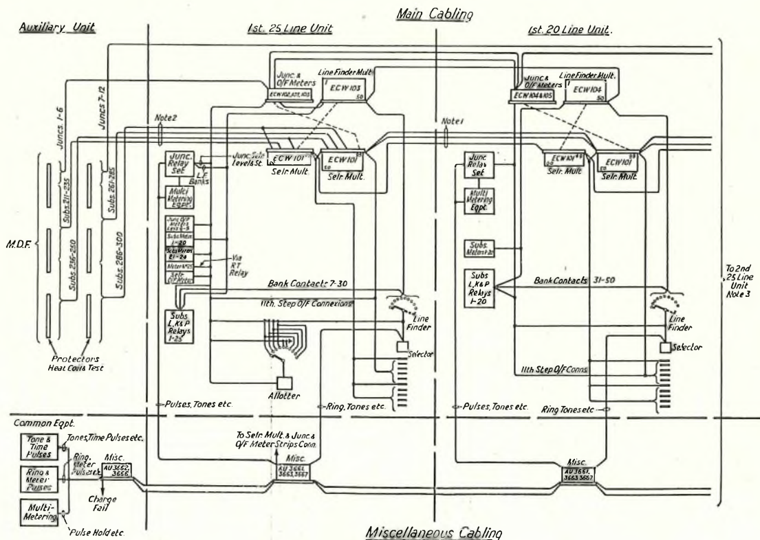
FIG. 4.—CABLING SCHEMATIC.
