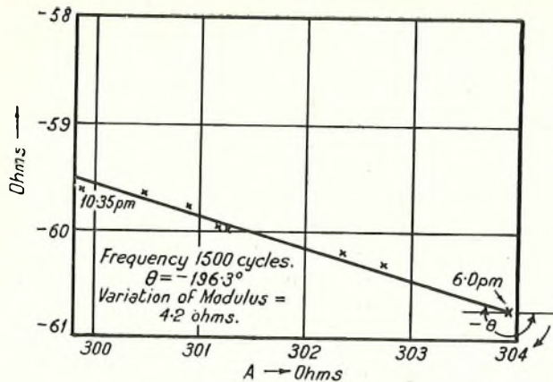
FIG. 10.—TEST ON SUBMARINE CABLE. VARIATION OF IMPEDANCE AT 1500 CYCLES.
