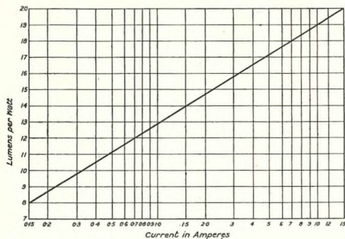
FIG. 6.—EFFICIENCY-CURRENT CHARACTERISTIC OF GENERAL SERVICE LAMPS.
