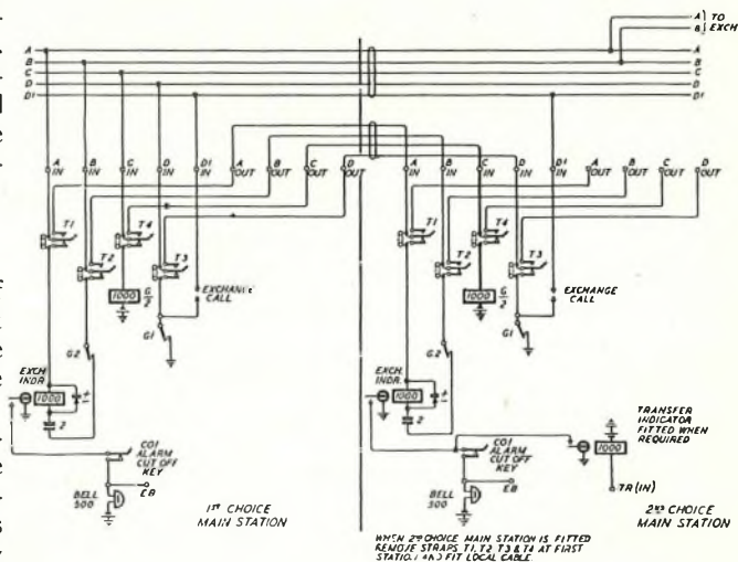
FIG. 11.—Circuit of Main Station on Installation Having One Exchange Line.
