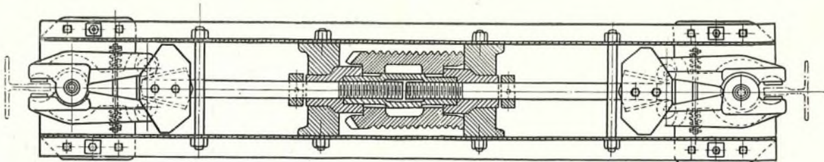
FIG. 7.—SAFETY GEAR.
