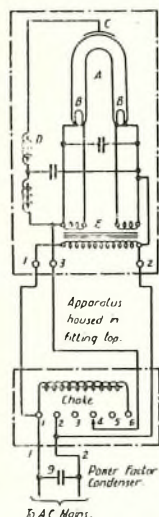
FIG. 2.—CIRCUIT OF THE PHILORA SODIUM LAMP.
