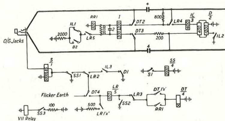
FIG. 13.—OUTGOING JUNCTION TO AUTO EXCHANGES.
