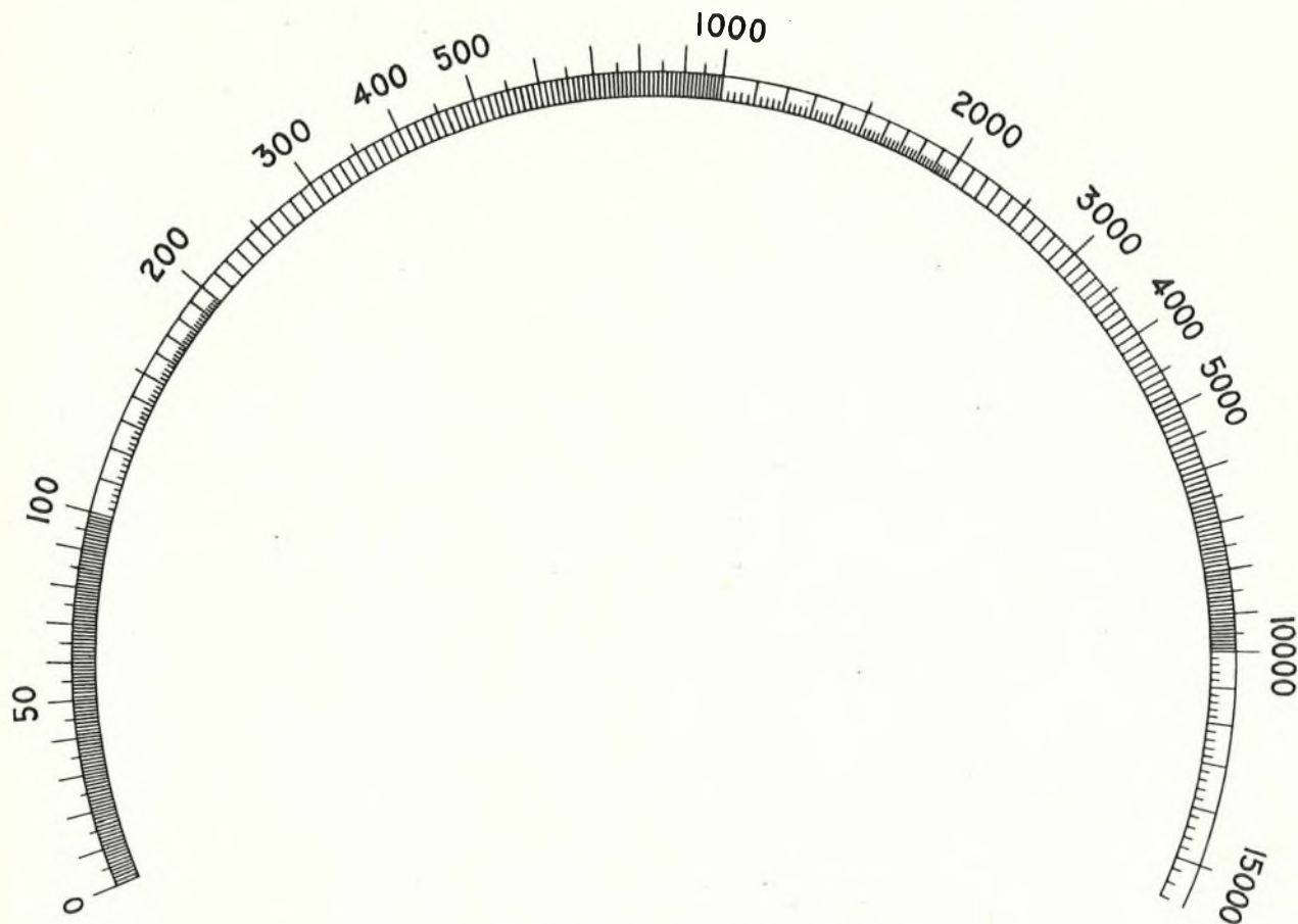
FIG. 6.—FREQUENCY SCALE OF RYALL-SULLIVAN HETERODYNE OSCILLATOR.
