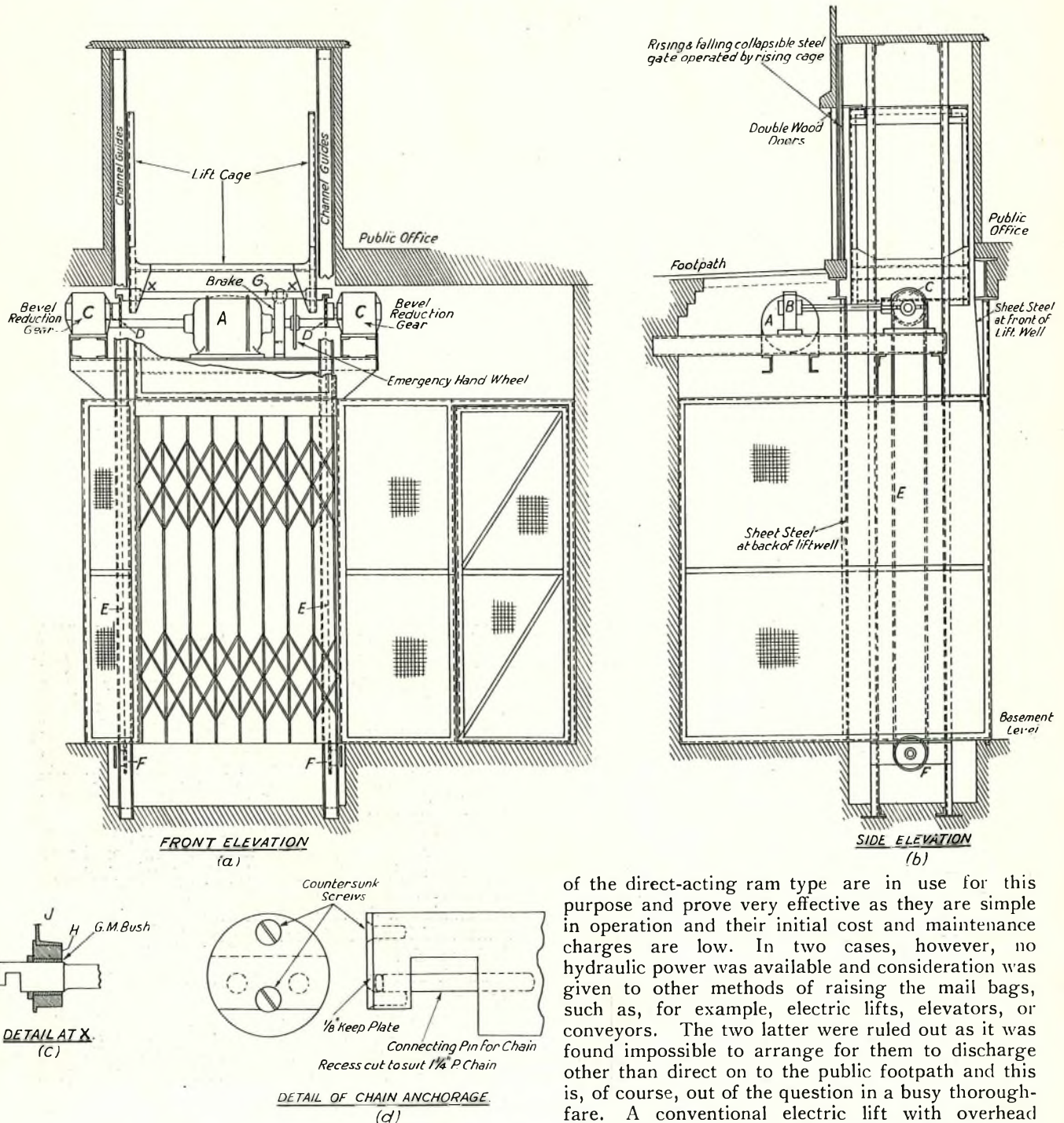
FIG. 1.—DETAIL OF ELECTRIC MAILS LIFT.
