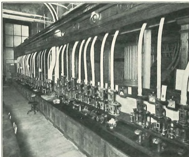
FIG. 1.—OLD TUBE TABLE, CENTRAL HALL.
