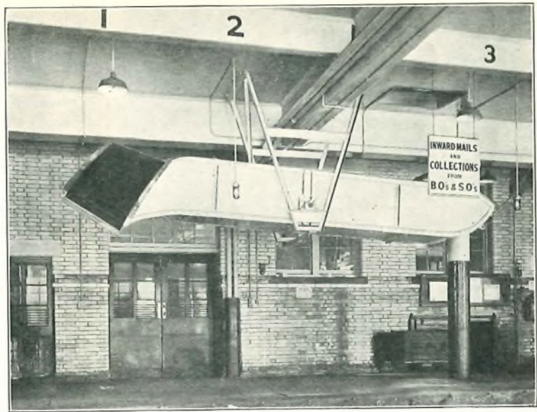
FIG. 12.—BALANCED CHUTE.
