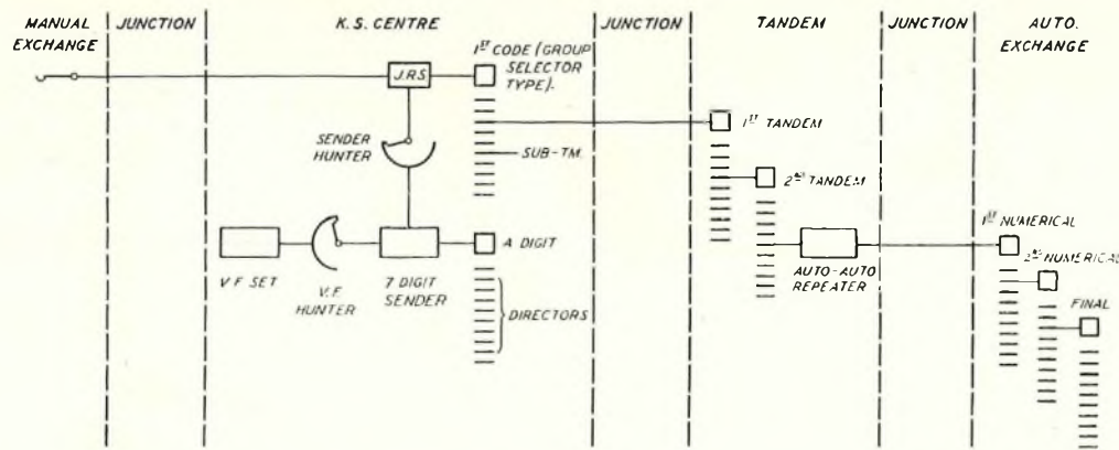
(a) Manual-Auto Call via K.S. Centre and Tandem.
