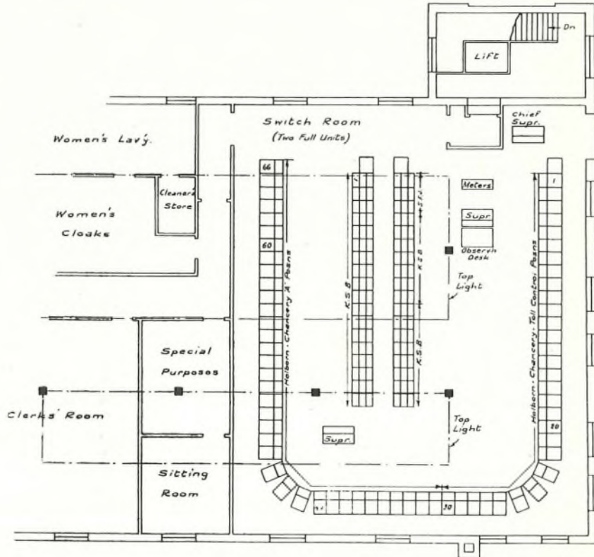
FIG. 5.—TANDEM-HOLBORN-CHANCERY SWITCHROOM, 1936.
