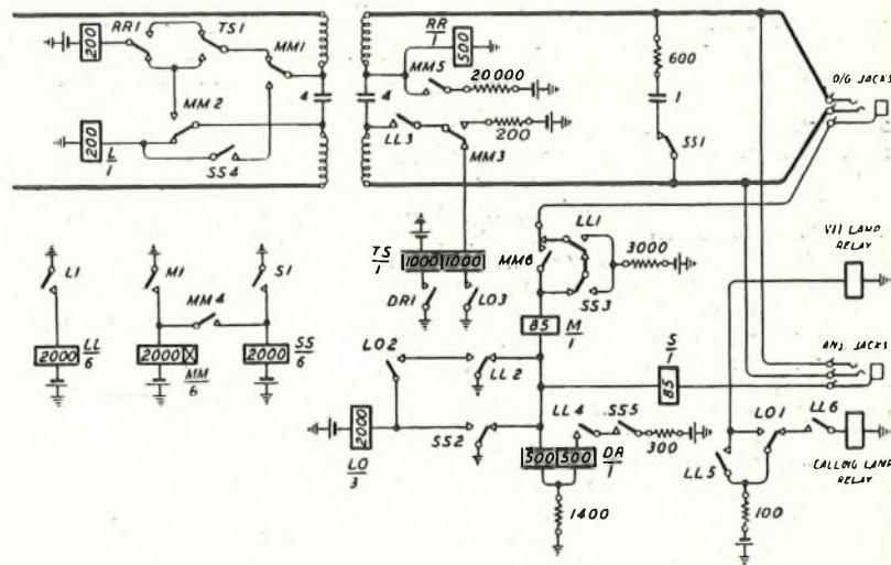
FIG. 14.—BOTHWAY AUTOMATIC SIGNALLING TRUNK.
