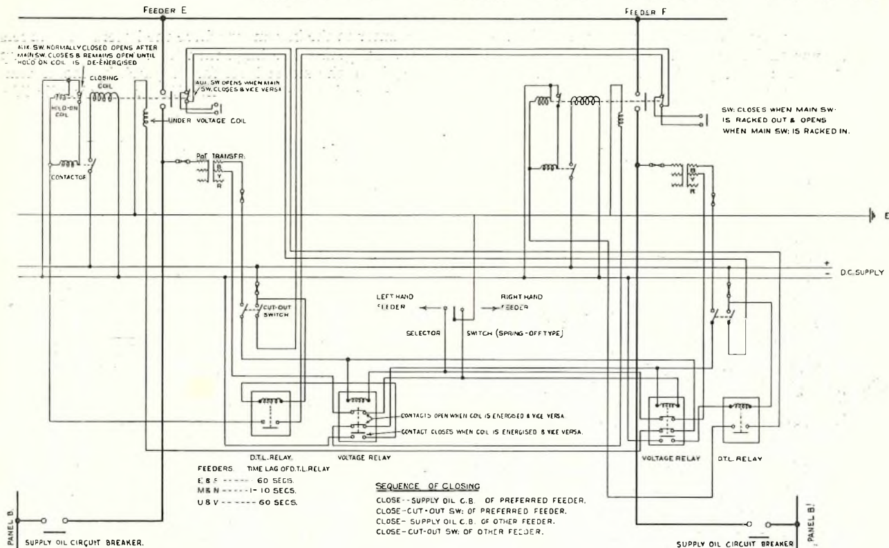
FIG. 5.—AUTOMATIC CHANGE-OVER SCHEME.
