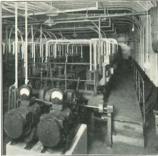
FIG. 2.—AUTOMATIC SWITCH ROOM.
