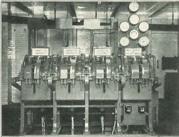
FIG. 1.—CONTROL PANEL.
