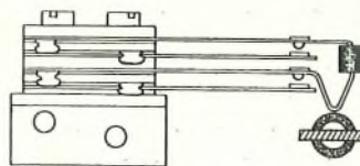
FIG. 12.—OFF-NORMAL SPRING ASSEMBLY.
