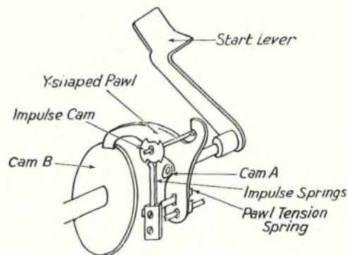
FIG. 5.—CONTROL MECHANISM.
