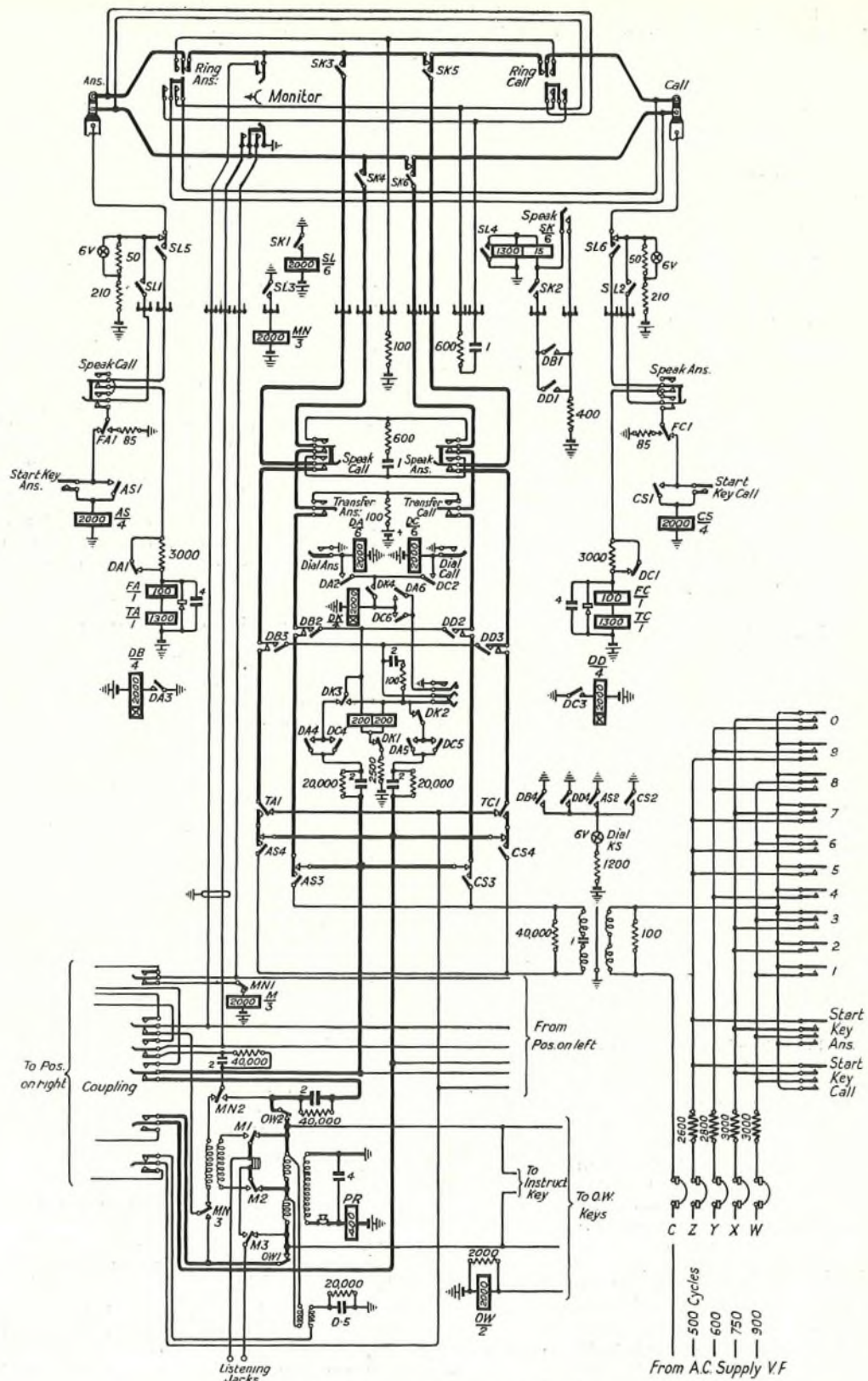
FIG. 11.—CORD AND POSITION CIRCUIT.
