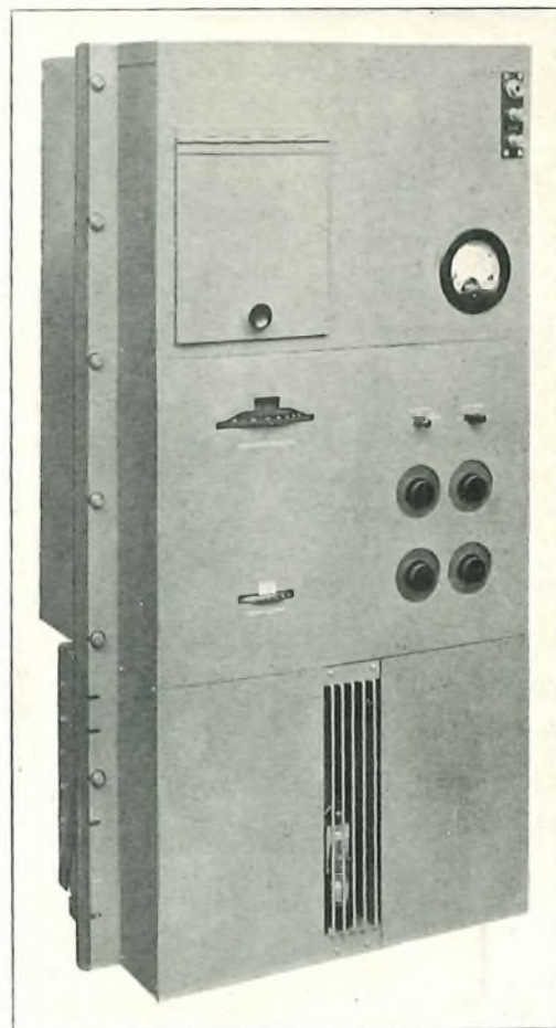
FIG. 2.—THE RYALL-SULLIVAN HETERODYNE OSCILLATOR—FRONT VIEW.
