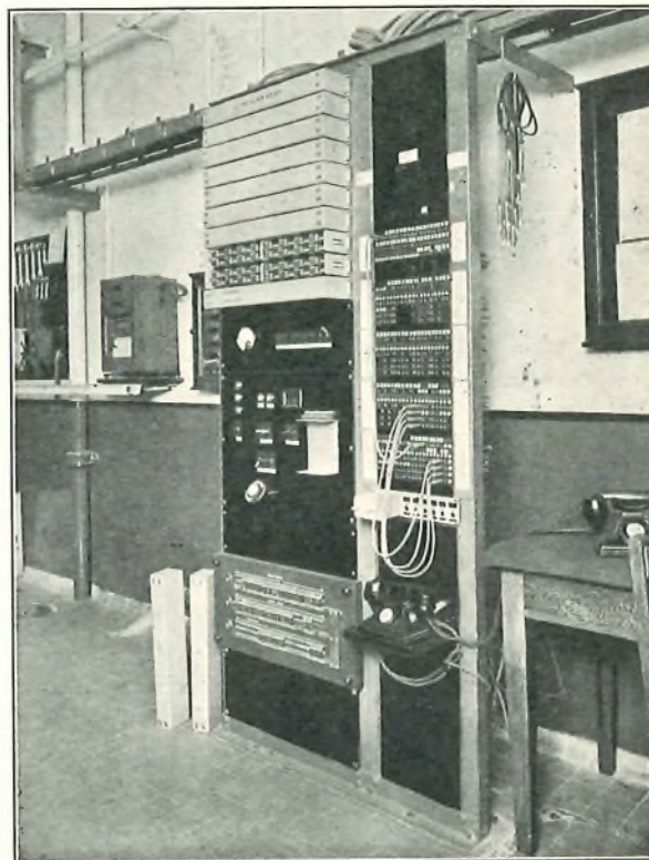
FIG. 11.—MISCELLANEOUS APPARATUS RACK.
