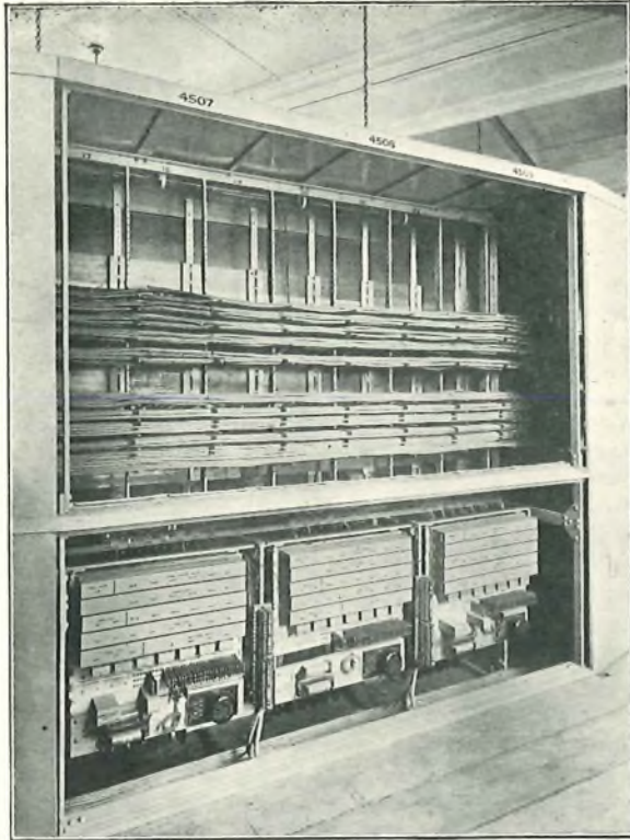
FIG. 8.—TRUNK DEMAND SECTION, REAR VIEW.
