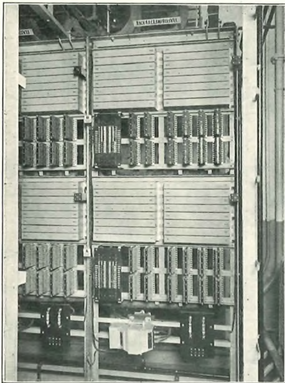
FIG. 10.—A.C. LAMP SUPPLY RACKS.
