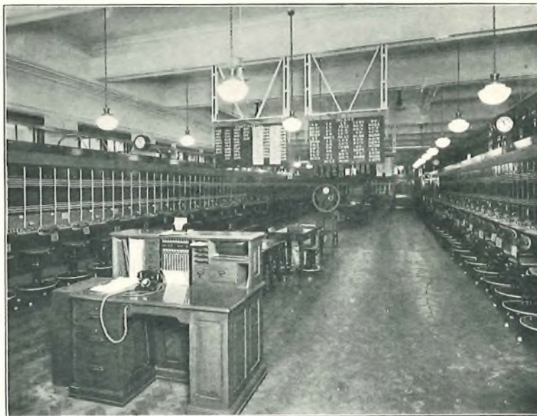
FIG. 9.—PROVINCIAL EXCHANGE SWITCHROOM.
