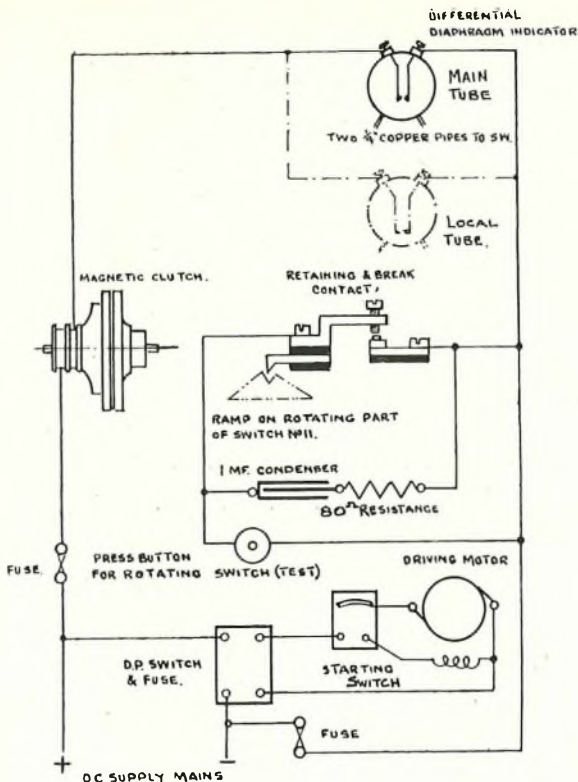
FIG. 6.—ELECTRICAL CONNEXIONS OF ROTARY SWITCH.
