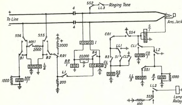
FIG. 12.—INCOMING JUNCTION FROM AUTO EXCHANGES.
