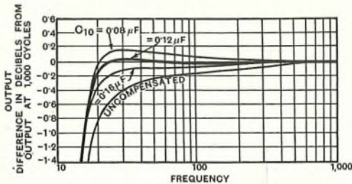
FIG. 10.—L.F. CORRECTOR CHARACTERISTICS.
