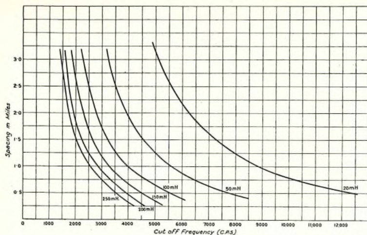
FIG. 6.—VARIATION OF CUT OFF FREQUENCY WITH LOADING SPACING; C = 0.065 \mu\text{F} PER MILB.
