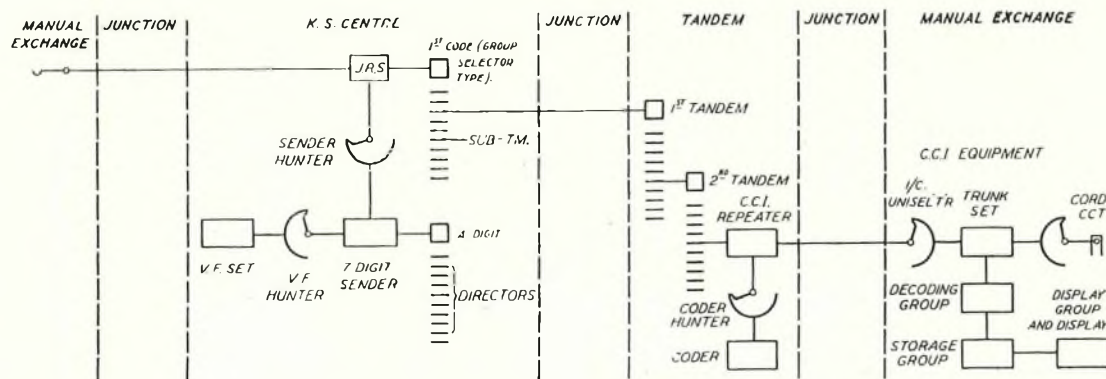
(b) Manual-Manual Call via K.S. Centre and Tandem.
