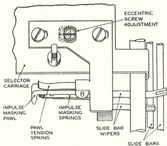
FIG. 10.—NUMBER SELECTOR.
