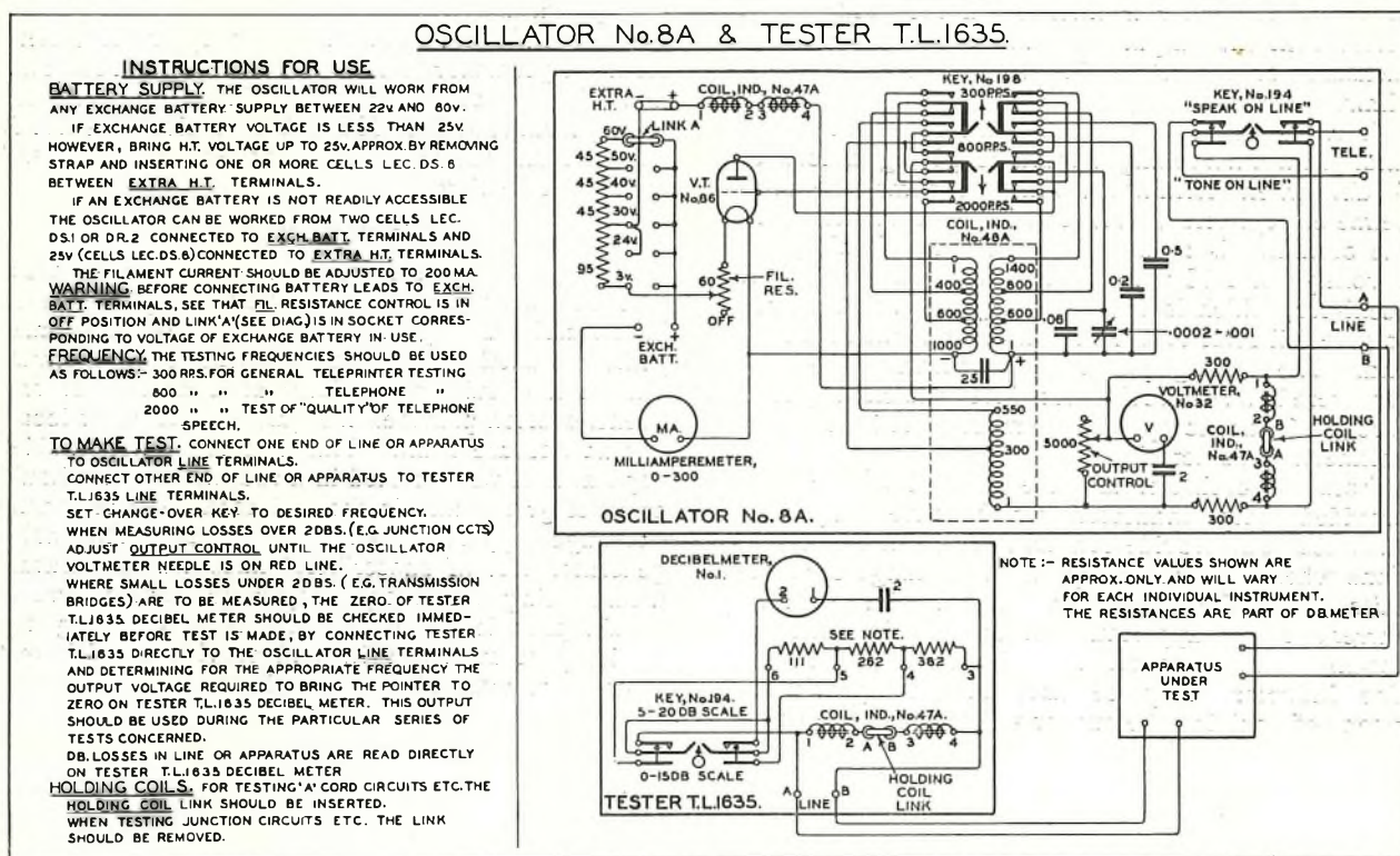
FIG. 4.—OSCILLATOR No. 8A AND TESTER T.L.1635.
