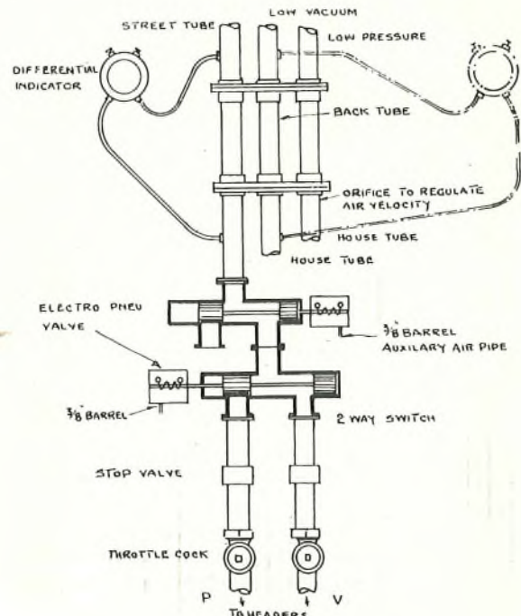
FIG. 5.—PIPEWORK CONNEXIONS OF ROTARY SWITCH.
