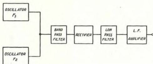
FIG. 1.—PRINCIPLE OF THE HETERODYNE OSCILLATOR (SCHEMATIC).
