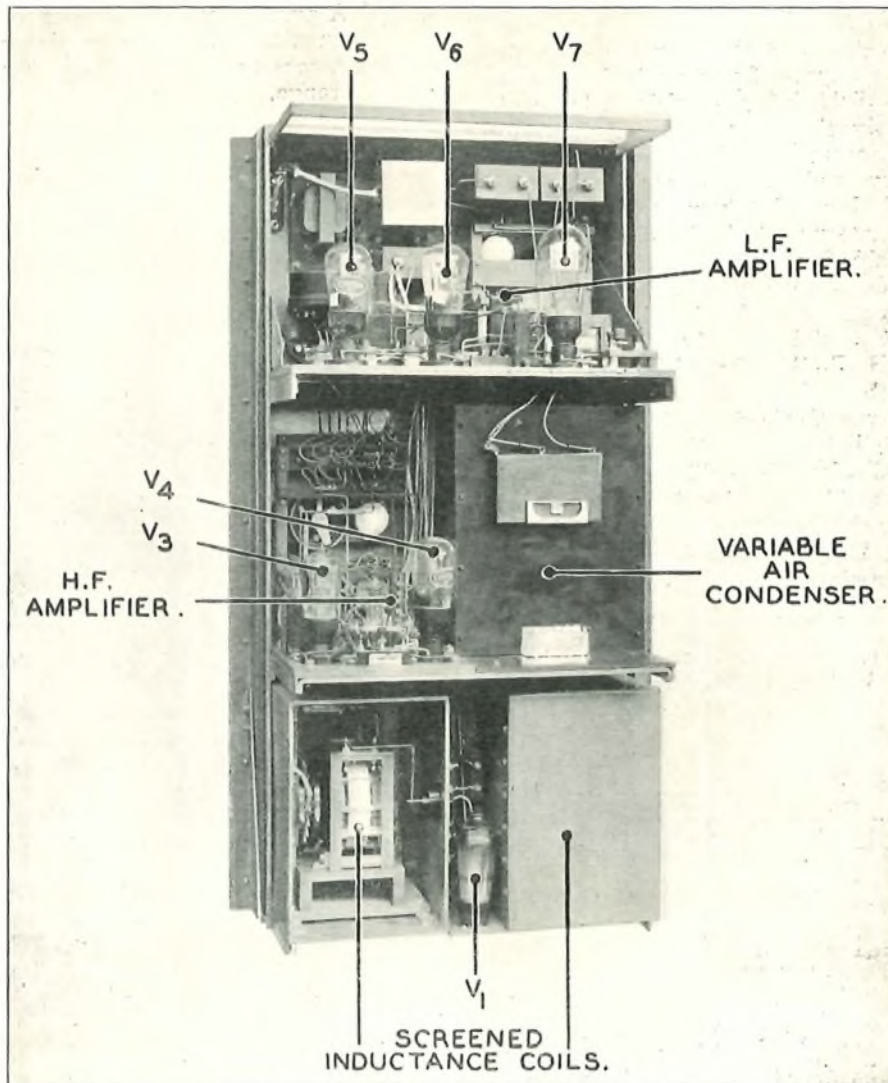
FIG. 3.—THE RYALL-SULLIVAN HETERODYNE OSCILLATOR—REAR VIEW WITH COVERS REMOVED.
