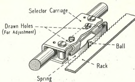
FIG. 11.—SLIDING CARRIAGE LOCATING DEVICE.
