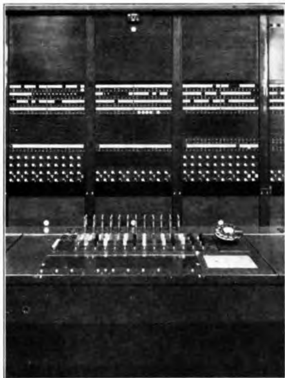
FIG. 3.—" INTERMEDIATE " TYPE.
