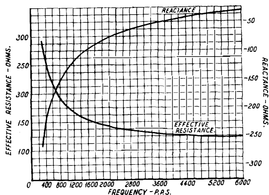
FIG. 8.—IMPEDANCE CHARACTERISTICS.
