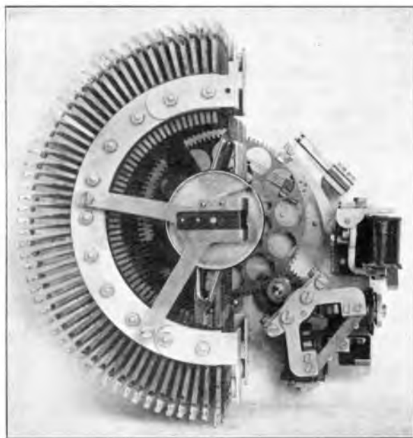
FIG. 1(a).—MOTOR UNISELECTOR: LEFT SIDE VIEW.
