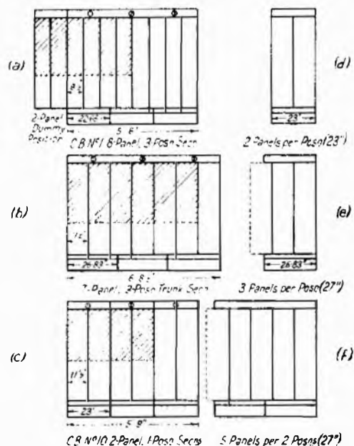
FIG. 4.—TYPICAL LAY-OUTS OF ONE-POSITION AND THREE-POSITION SECTIONS, SHOWING RELATION BETWEEN MULTIPLE PANELS AND POSITIONS.
