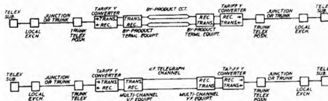
FIG. 1.—SCHEMATIC TARIFF "Y" CONNEXION.
