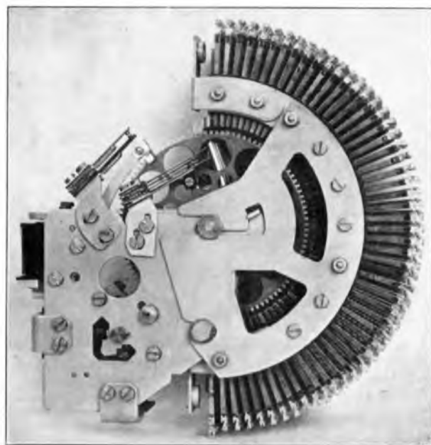
FIG. 1(b).—MOTOR UNISELECTOR: RIGHT SIDE VIEW.
