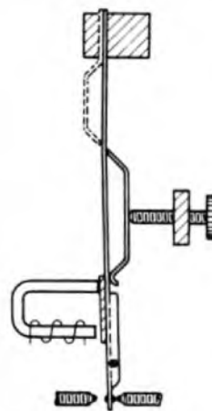
FIG. 3(b).—ELEMENTS OF HIGH-SPEED RELAY.
