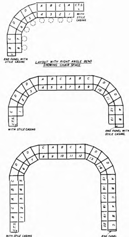
FIG. 9.—TYPICAL SWITCHROOM LAY-OUTS WITH ONE-POSITION SECTIONS
