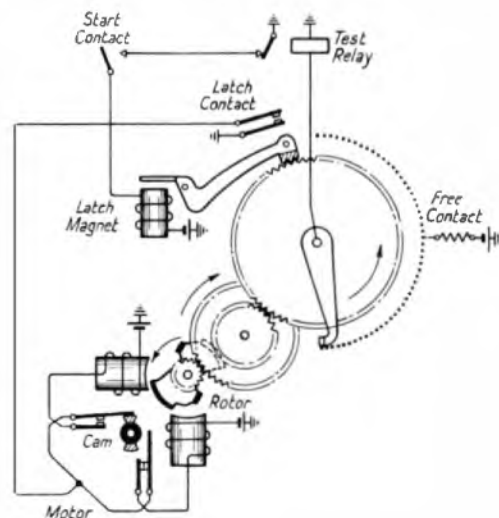
FIG. 2.—MOTOR UNISELECTOR; ELECTRICAL CONNEXIONS.
