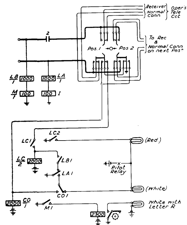
FIG. 3.—INCOMING JUNCTION AND MONITORIAL POSITION CIRCUIT.
