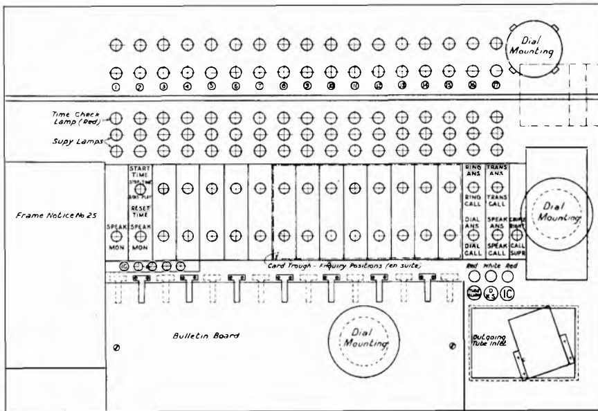
FIG. 8.—KEYSHELF, 27 INS. BY 18 INS.
