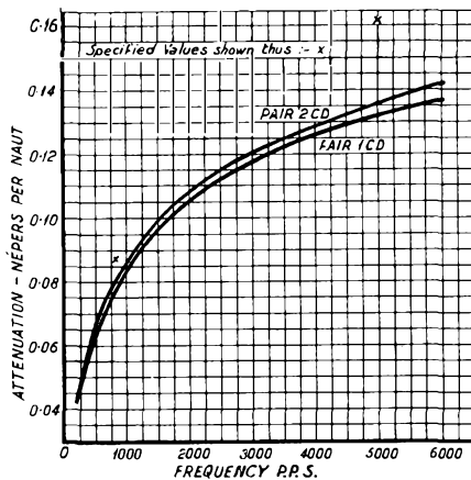
FIG. 13.—SIDE CIRCUIT ATTENUATION.
