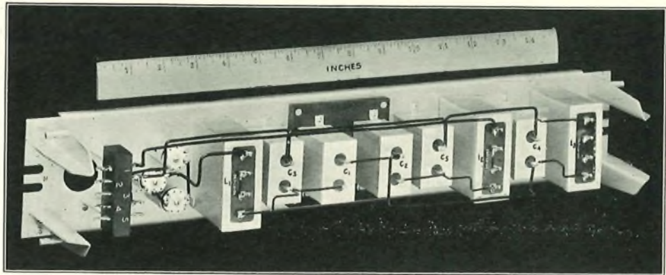
FIG. 3.—SENDING-END FILTER.
