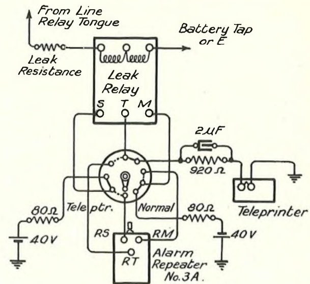
FIG. 2.—LEAK TELEPRINTER CIRCUIT.
