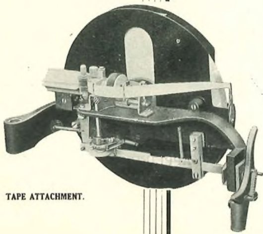
No. 7a MODEL (Back View)
