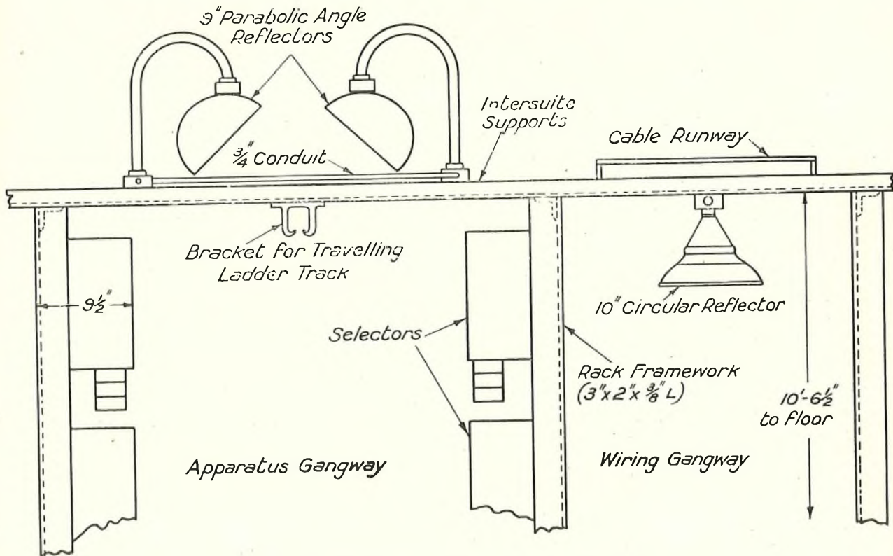
FIG. 11.—END VIEW OF UPPER PORTION OF GANGWAYS.
