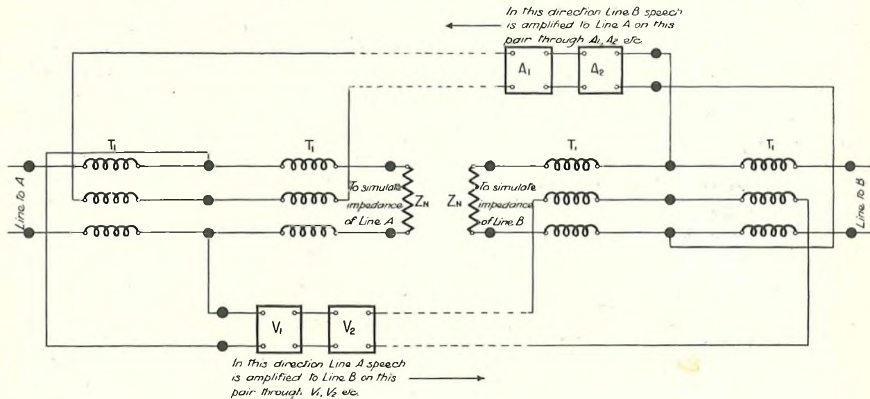
FIG. 50.—"FOUR WIRE" REPEATER CIRCUIT.
