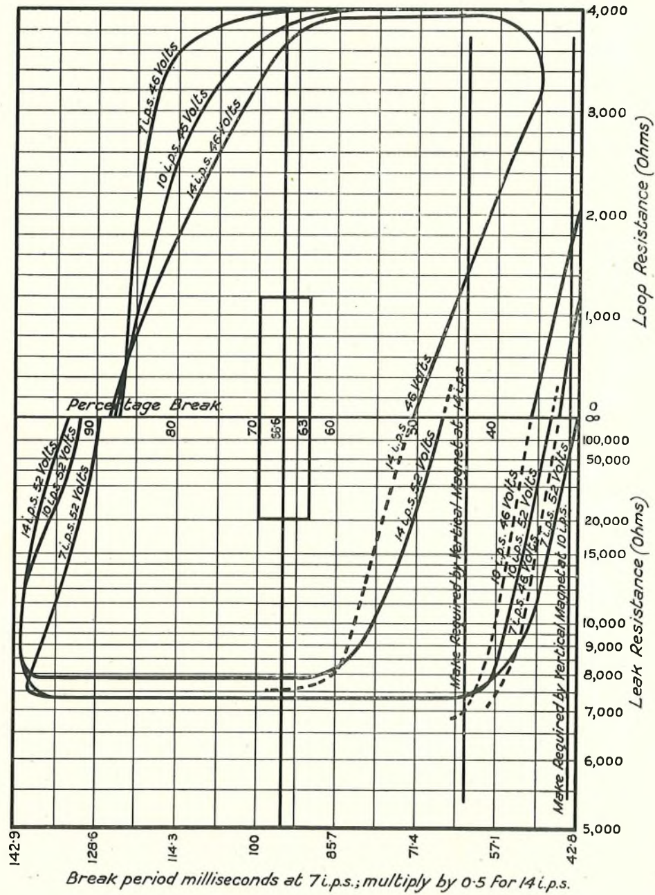
FIG. 3.—SELECTOR PERFORMANCE CHART.
