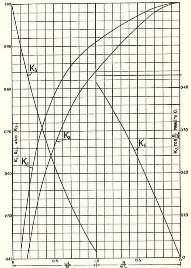
FIG. 1.—CORRECTION FACTORS FOR LOADED LINES.
