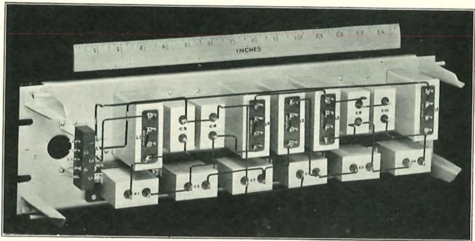
FIG. 4.—RECEIVING-END FILTER.
