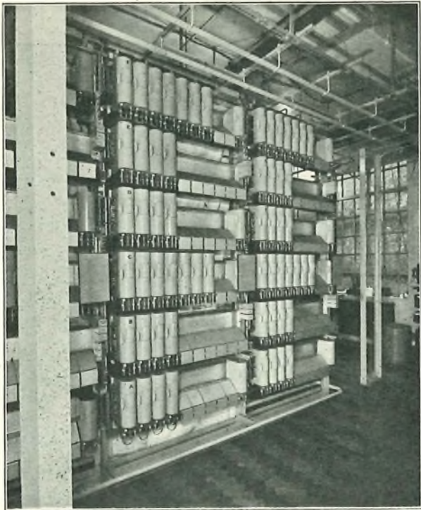
FIG. 4.—3RD SELECTORS, CENTRAL EXCHANGE.
