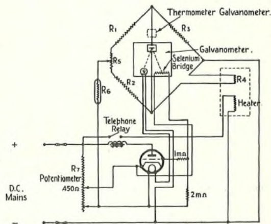
FIG. 2.—CONNEXIONS OF THERMOSTAT WORKED FROM D.C. MAINS.
