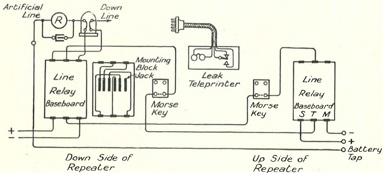
FIG. 3.—REPEATER TERMINATED FOR TELEPRINTER WORKING.
