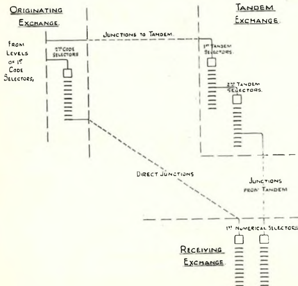
FIG. 4.—APPARATUS REQUIRED FOR DIRECT AND TANDEM-ROUTED TRAFFIC.
