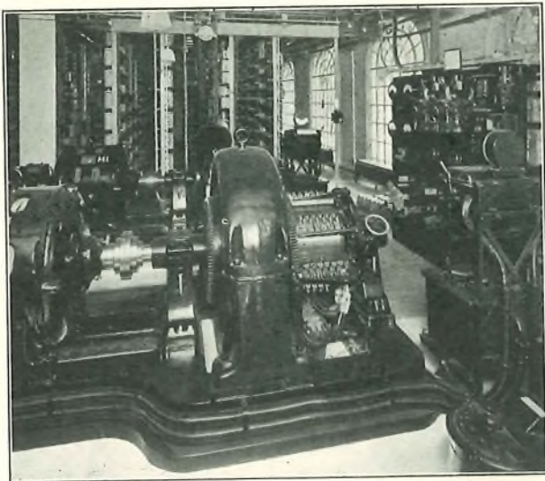
FIG. 9.—POWER PLANT, CENTRAL EXCHANGE.
