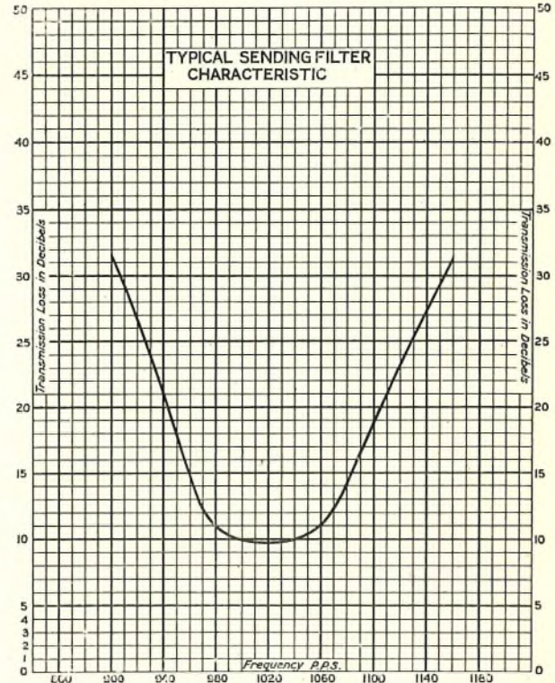
FIG. 2.—TYPICAL SENDING FILTER CHARACTERISTIC.
