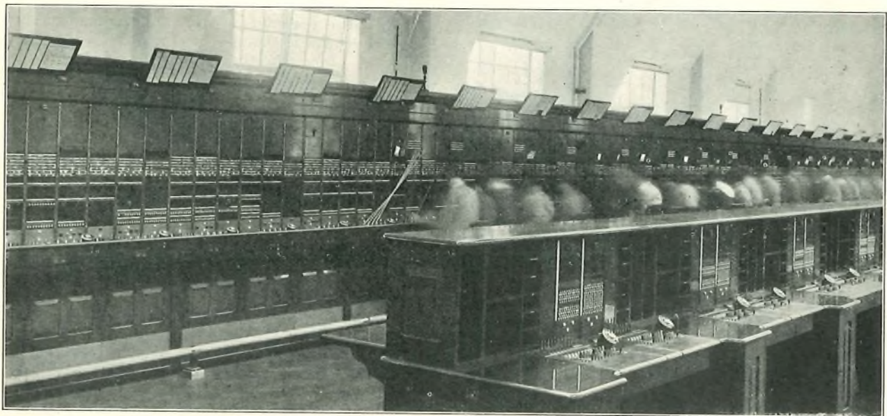
FIG. 10.—AUTO-MANUAL SWITCHBOARD, CENTRAL EXCHANGE.
