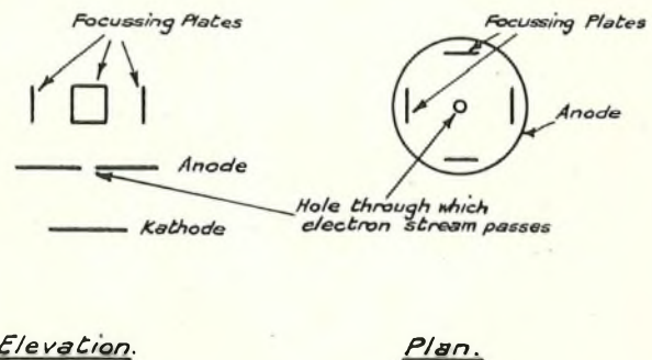
FIG. 8.—ARRANGEMENT OF KATHODE RAY OSCILLOGRAPH.
