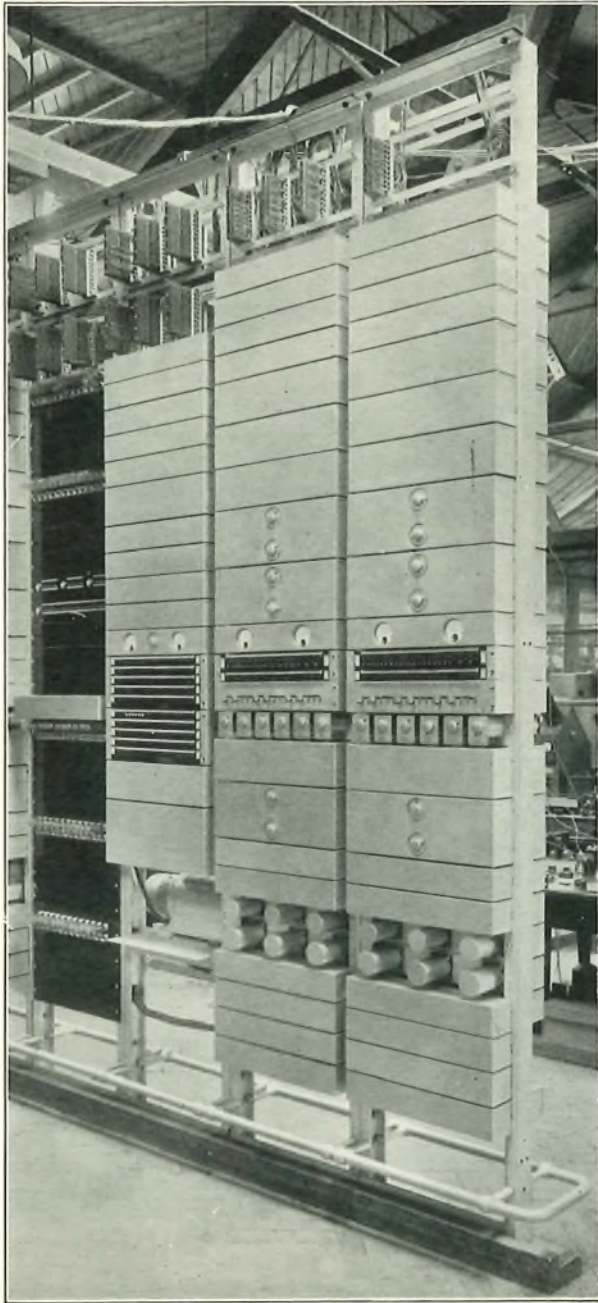
FIG. 8.—TYPICAL 12-CHANNEL EQUIPMENT.
