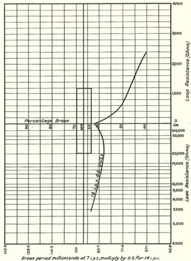
FIG. 4.—PORTION OF PERFORMANCE CURVE.
