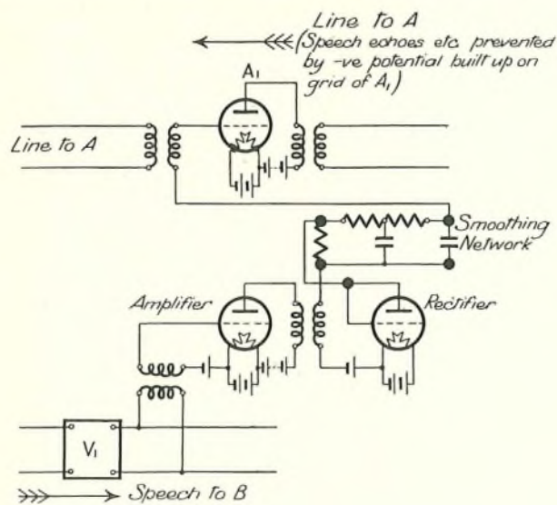
FIG. 51.—PRINCIPLE OF ECHO SUPPRESSOR.
