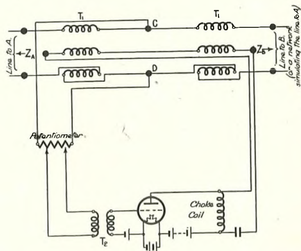
FIG. 48.—PRINCIPLE OF TWO-WAY ONE-ELEMENT "REPEATER" (2-1 TYPE).
