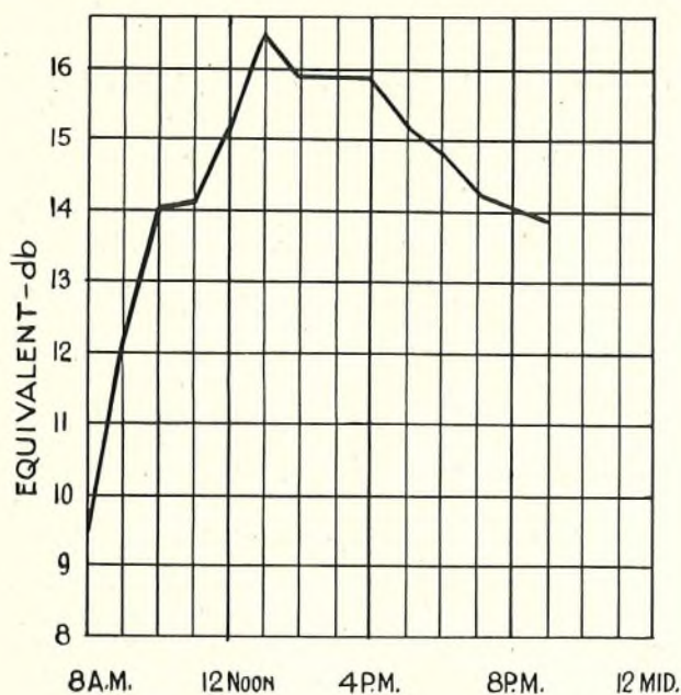
FIG. 9.—VARIATION IN ATTENUATION AT 1,000 C.P.S.
