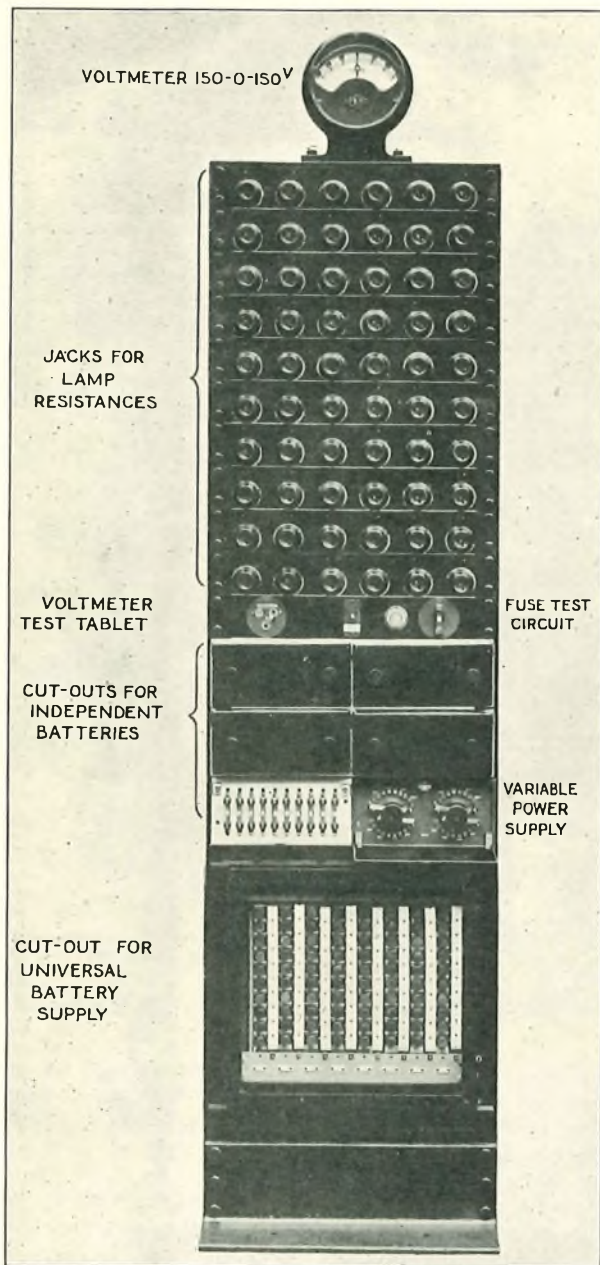
FIG. 6.—POWER BAY.
