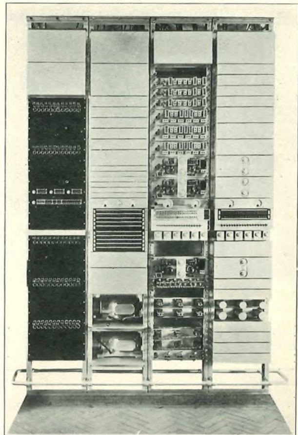
FIG. 9.—FRONT VIEW, SHOWING CHANNEL BAY COVERS REMOVED.
