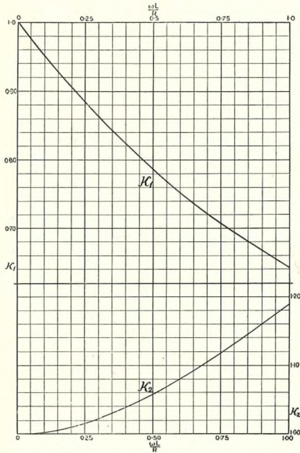
FIG. 2.—CORRECTION FACTORS FOR NON-LOADED LINES.
