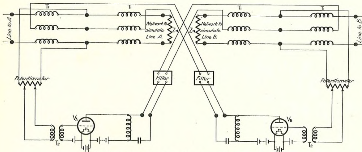
FIG. 49.—PRINCIPLE OF TWO-WAY TWO-ELEMENT "REPEATER" (2-2 TYPE).
