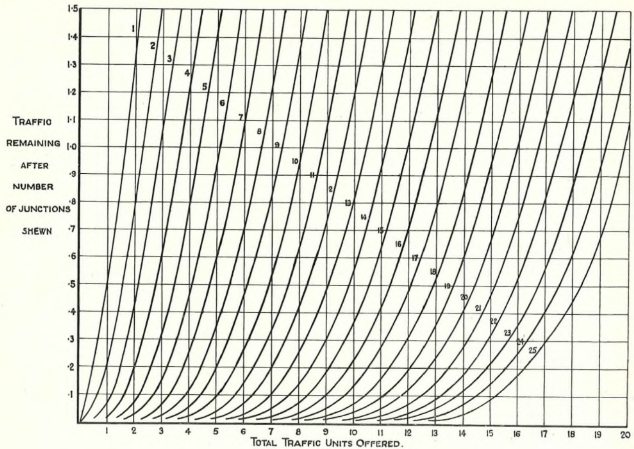
FIG. 6.—TRAFFIC LEFT WHEN PARTICULAR QUANTITIES OF TRAFFIC ARE OFFERED TO JUNCTION GROUPS.
