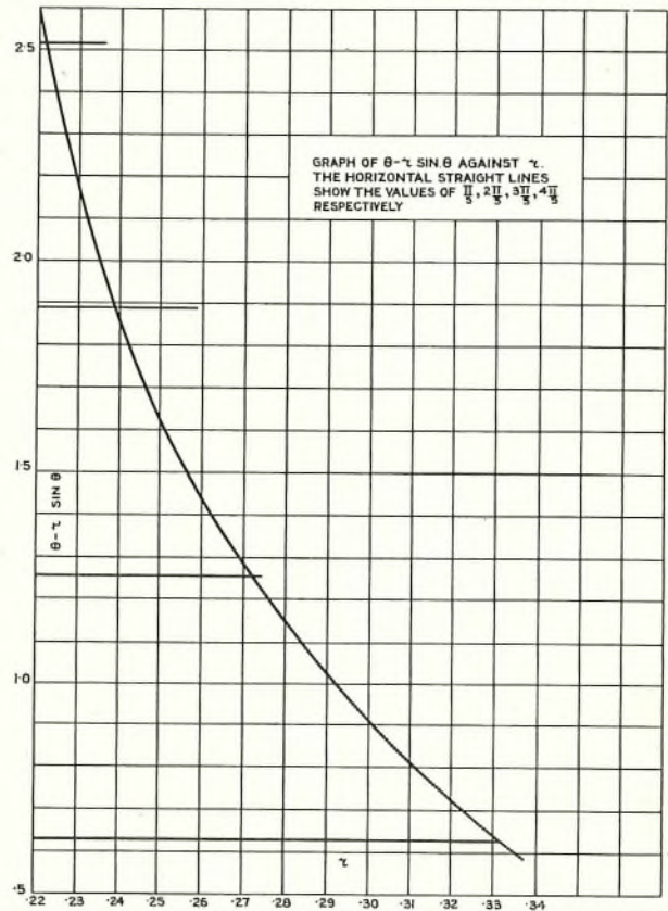
FIG. 1.—CURVE USED FOR OBTAINING THE NUMERICAL SOLUTIONS OF EQUATIONS (5) AND (6).
