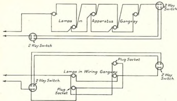
FIG. 10.—WIRING OF GROUP OF THREE PARALLEL SUITES.
