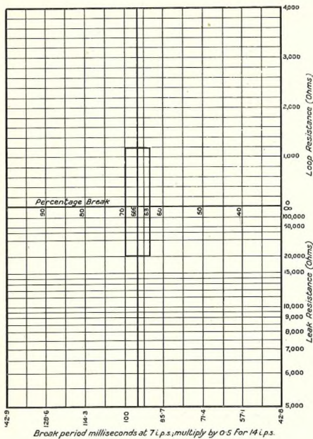
FIG. 2.—PERFORMANCE CHART.
