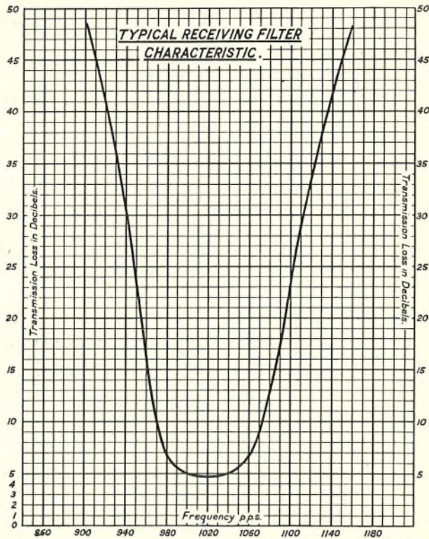
FIG. 5.—TYPICAL RECEIVING FILTER CHARACTERISTIC.
