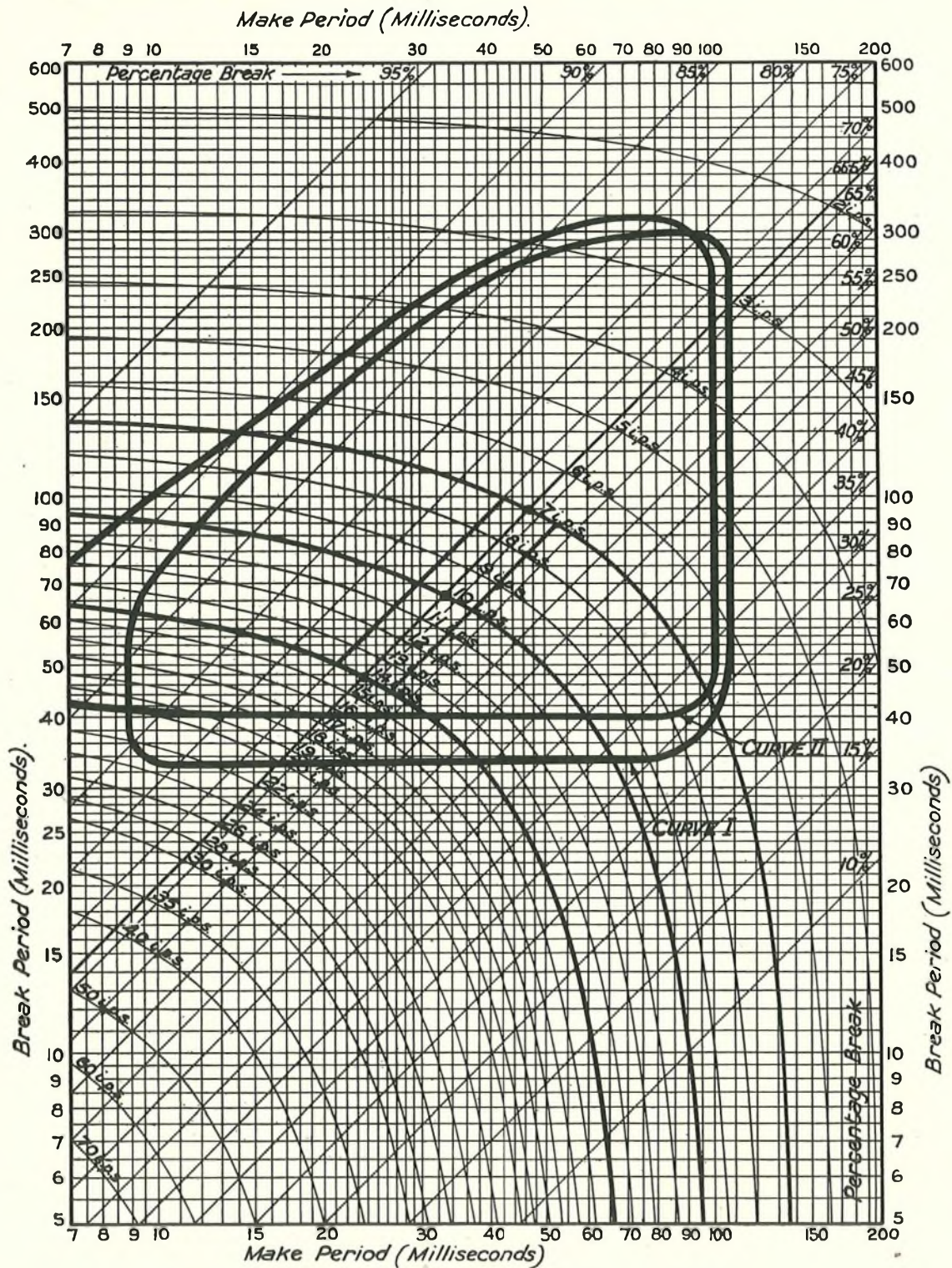
CURVE I. Line Resistance 1800Ω, Leak ∞, 46 Volts. CURVE II. Line Resistance Zero, Leak 20,000Ω, 52 Volts.
