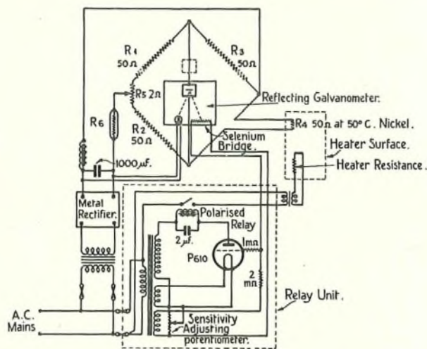
FIG. 1.—CONNEXIONS OF THERMOSTAT WORKED FROM A.C. MAINS.
