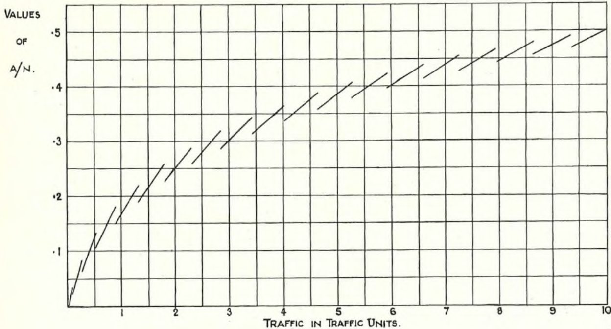
FIG. 3.—RELATION BETWEEN TRAFFIC PER JUNCTION AND TOTAL TRAFFIC.
