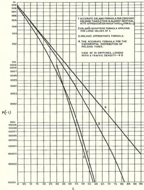
FIG. 2.—CURVES SHOWING THE PROBABILITIES FOR DELAYS, EXCEEDING VARIOUS SPECIFIED TIMES.
