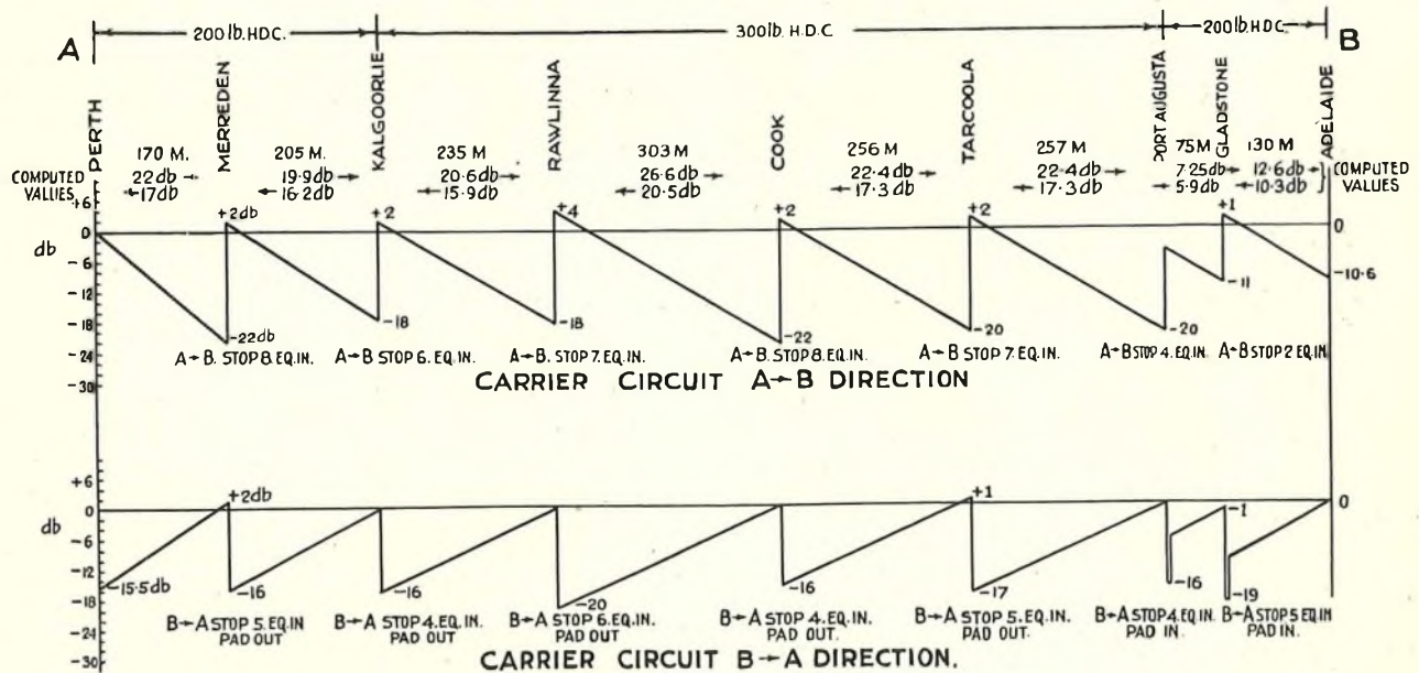
FIG. 8.—POWER LEVEL DIAGRAM.
