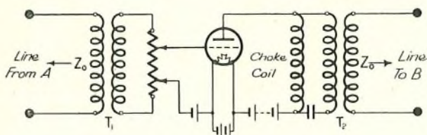
FIG. 47.—ONE VALVE AMPLIFICATION—ONE WAY—ONE ELEMENT "REPEATER."
