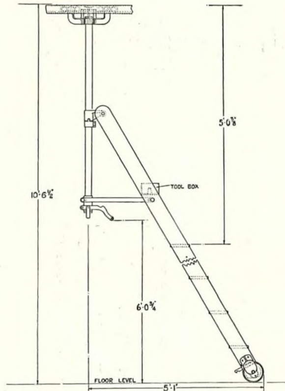
FIG. 1.—SIDE VIEW OF LADDER READY FOR USE.
