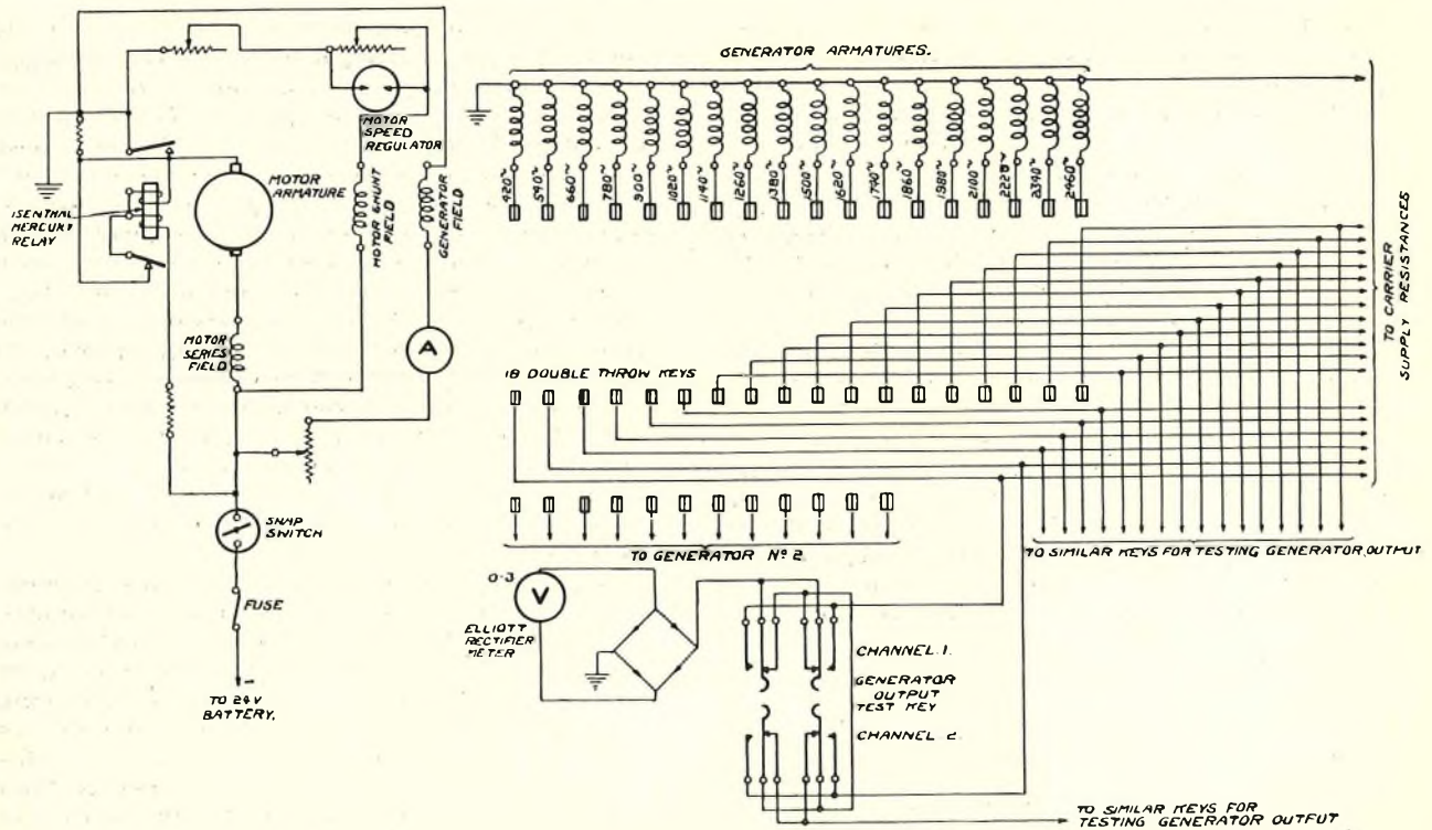
FIG. 1.—SCHEMATIC DIAGRAM OF CARRIER CURRENT SUPPLY.
