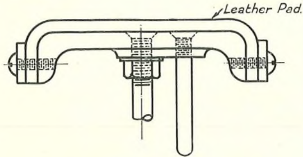
FIG. 3.—BRAKE SHOE.
