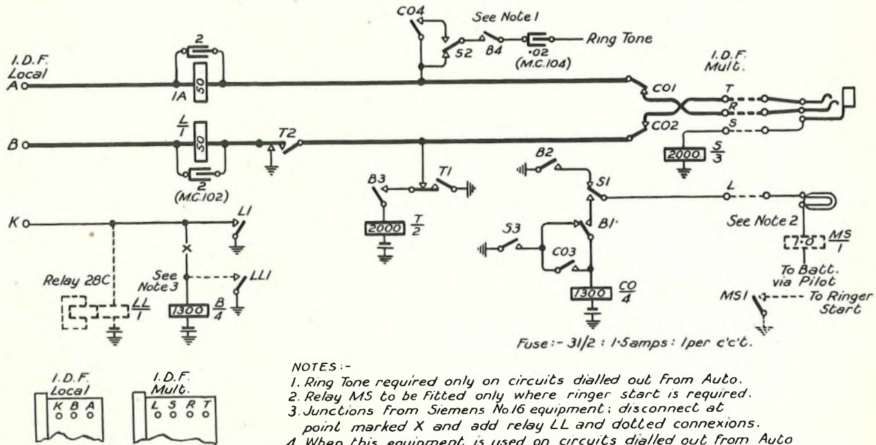
FIG. 2.—JACK-ENDED JUNCTION CIRCUIT WITH CALLING SIGNAL ARRANGED FOR FOLLOWING-ON CALL.
