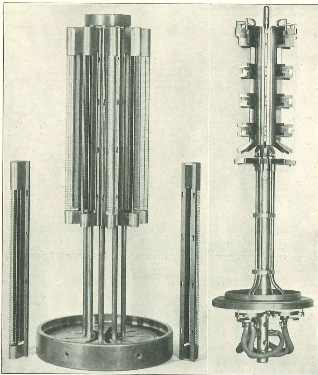
FIG. 2.—GRID STRUCTURE.
