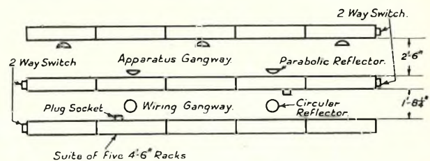
FIG. 9.—PLAN OF APPARATUS AND WIRING GANGWAYS.
