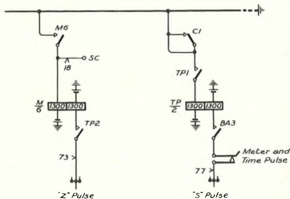
FIG. 1.—PART OF DIRECTOR CIRCUIT.
