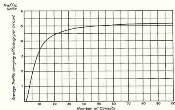
FIG. 1.—TRAFFIC CARRYING EFFICIENCY OF LARGE GROUPS.
