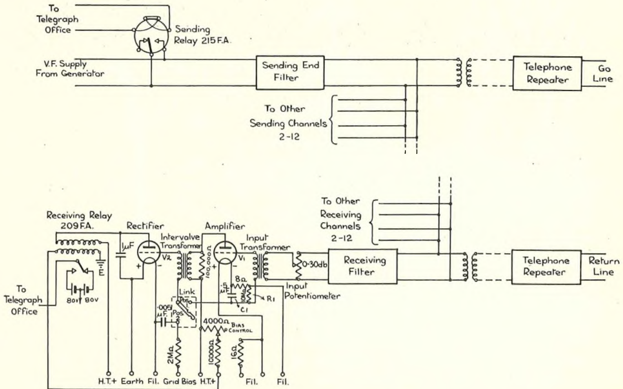
FIG. 6.—SCHEMATIC DIAGRAM OF A SENDING AND RECEIVING CHANNEL.
