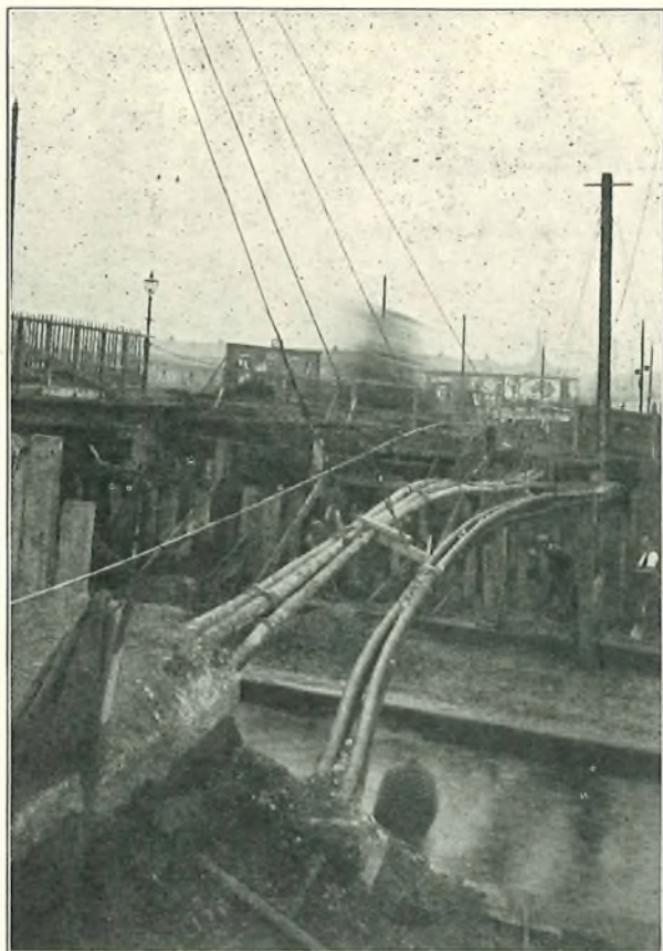
FIG. 2.—PIPES SUPPORTED BY SLINGS AND STAYS.
