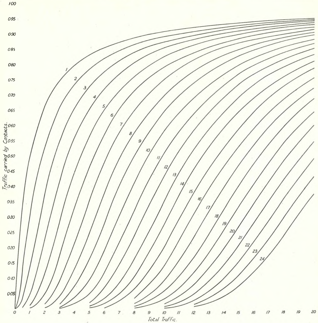
FIG. 5.—TRAFFIC CARRIED BY EACH CONTACT IN A FULL AVAILABILITY GROUP.
