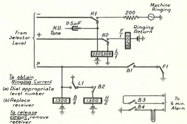
FIG. 3.—FAULTSMEN'S RINGING-BACK CIRCUIT.
