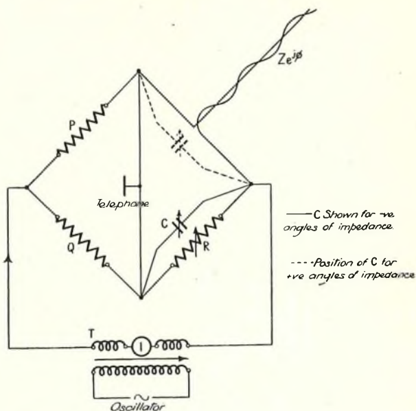
FIG. 52.—A.C. BRIDGE FOR LINE IMPEDANCE MEASUREMENT.
