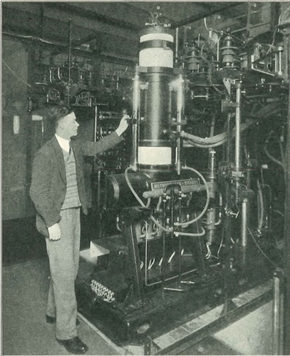
FIG. 1.—500 KILOWATT DEMOUNTABLE VALVE. The attendant is holding a receiving valve for comparison.
