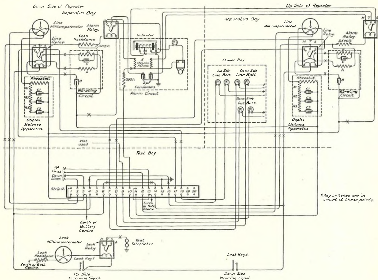
FIG. 8.—CIRCUIT CONNEXIONS—REPEATER THROUGH.
