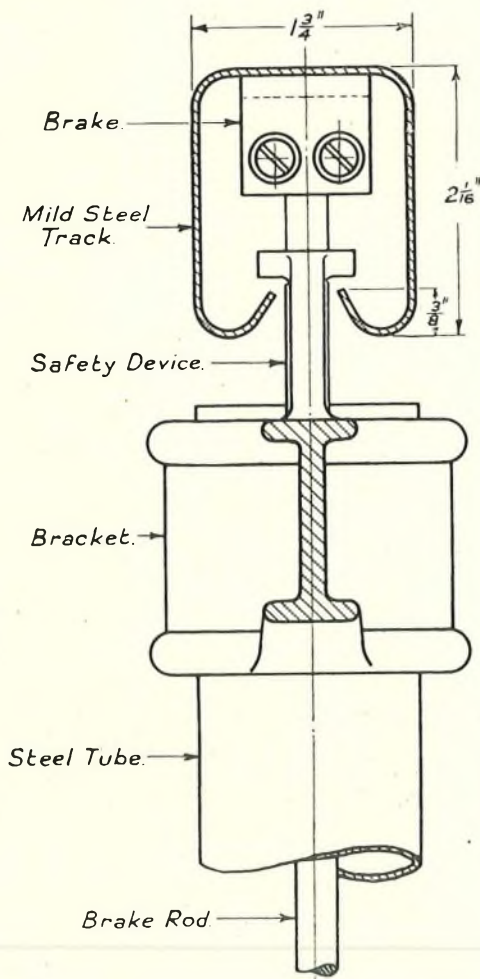
FIG. 4.—SECTIONAL VIEW OF TRACK AND BRAKE.
