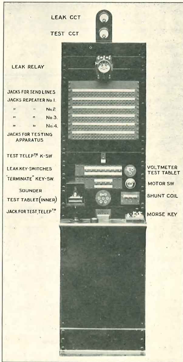
FIG. 5.—TEST BAY.
