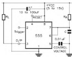
Monostable Mode
