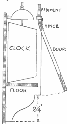
Fig. 2—Side section
