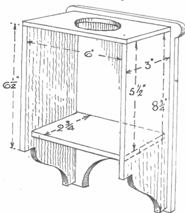
Fig. 3—Constructional details
