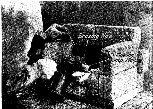
USE OF FIRE-BRICKS IN BRAZING
