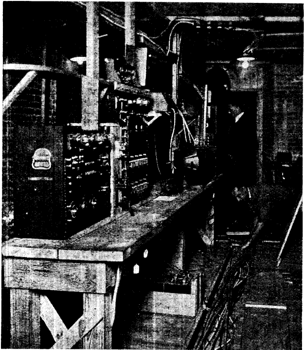
Fig. 3. Broadcasting by land-line relay is carried out by using an apparatus of this kind. Here the instruments for amplifying are seen installed beneath a theatre
