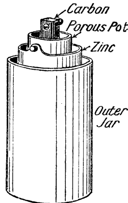
BUNSEN CELL
