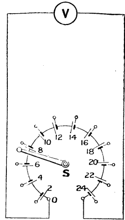
Fig. 4. Voltmeters may be calibrated by the above arrangement, employing a battery of accumulators
