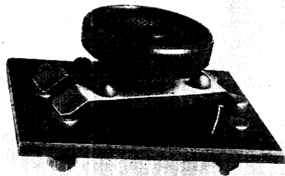
Fig. 4. For commutation purposes this type of double-brush switch is used. The brushes bear simultaneously on opposite contact studs
