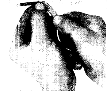
Fig. 3. Eyes are made in the end of a coiled brass wire spring with round-nosed pliers
