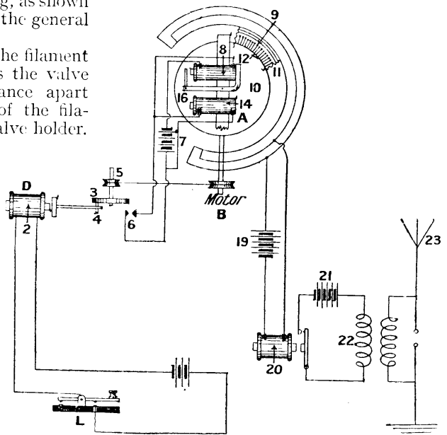
BULL TRANSMITTER WORKED ON MECHANICAL PRINCIPLES Fig. 1. Operation of the spark coil in the old Bull transmitter was conducted through a disperser, the arrangement of which is seen in the above diagram
