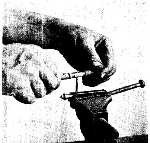
BRASS SCREW CUTTING AND TAPPING BY HAND
