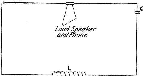
THEORY OF BY-PASS CONDENSER
