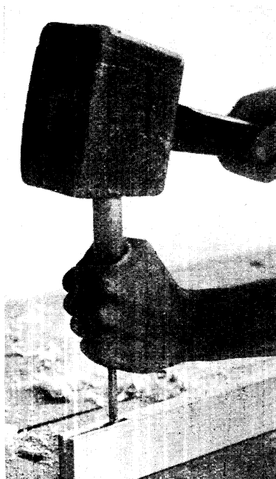
Fig. 46. Cutting out a mortice for a framework. The chisel is driven with a mallet
