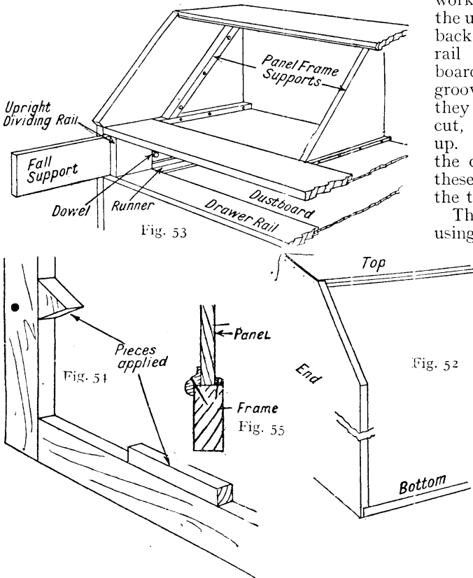
CONSTRUCTIVE DETAILS FOR JACOBEN CABINET CONSTRUCTION Fig. 52. Flush joints at the top of the main body of the cabinet. Fig. 53. Parts for the top of the cabinet and the arrangement for the accommodation of the panel. Fig. 54. Shaping is formed in this manner, and small blocks are glued to the frame before attaching the moulding. Fig. 55. Back panel beading attachment
