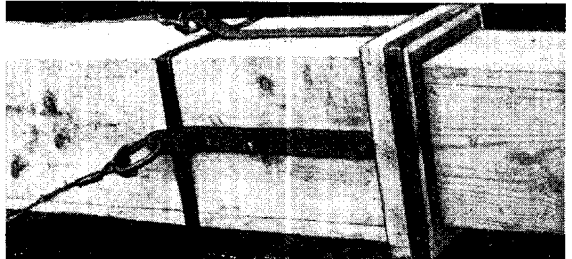
Fig. 4. Shows how one section fits into the next, also position of straps and supporting battens
