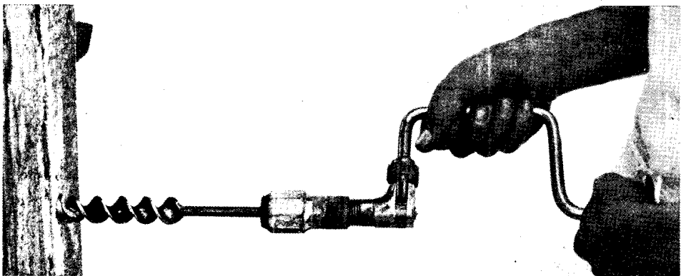
Fig. 6. Manipulation of the brace when boring in an horizontal position is accomplished by holding the tool as shown, applying the pressure from the hip
