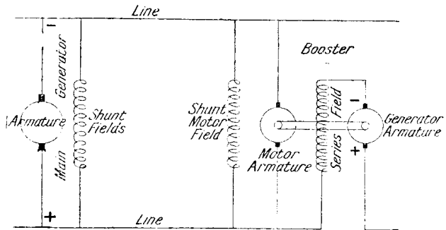
CIRCUIT DIAGRAM OF A BOOSTER
