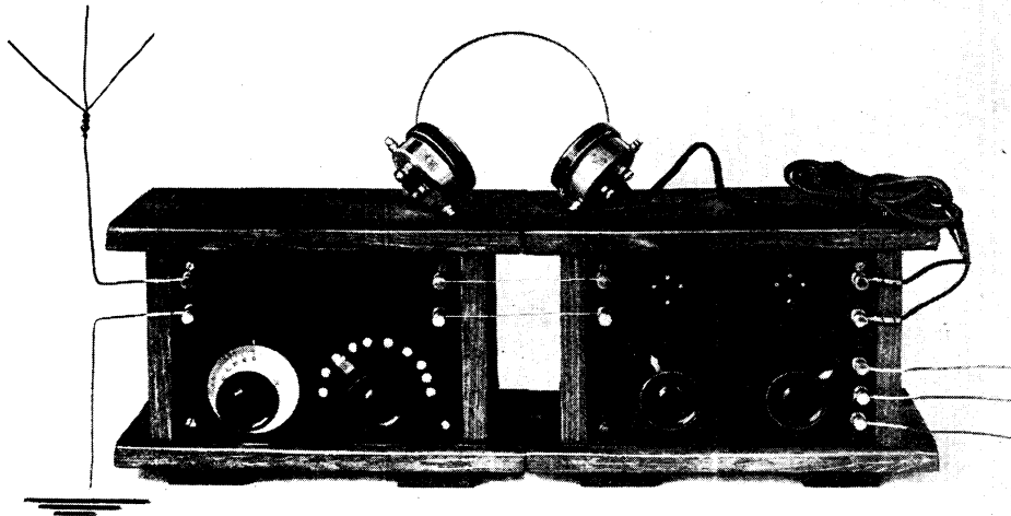
Fig. 23. When high- and low-frequency units are added to a set, cabinets suitable for the purpose may be made as here illustrated. The two units are uniform in design and dimensions
