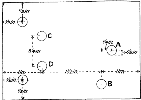
LAY-OUT OF BUZZER PANEL
