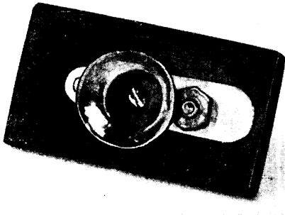
Fig. 2. In this view the centre contact screw is seen, also the flat plate on right to which the holder is joined. How the contact screw is connected to the valve leg on the underside is seen in Fig. 1
