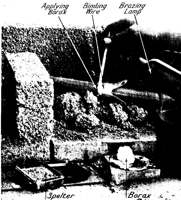
PREPARATION FOR BRAZING
