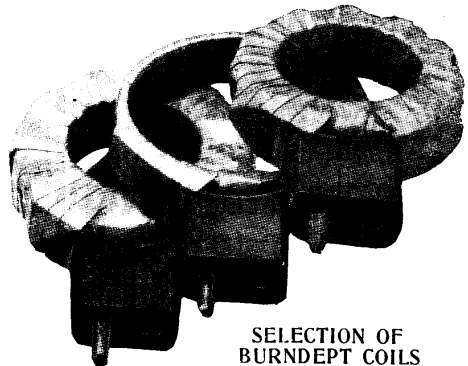
Fig. 2. Burndept coils are in various sizes. Those illustrated are, left, No. 300, centre, No. S1, and right, No. 150. These coils are extensively used in tuned anode circuits
