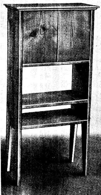
Fig. 42. Carcase and doors of cabinet assembled
