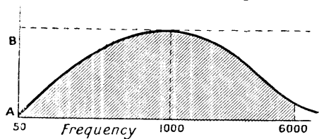
Fig. 1. Limiting amount of amplitude is represented by AB, and the overall amount of microphone control the cross-hatched area
