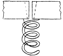
Fig. 2. Fine wire coil bridging brass blocks in calibrated resistance
