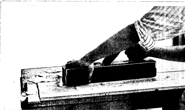
Fig. 38. Planing up the outside of the side. Note the method of holding the plane
