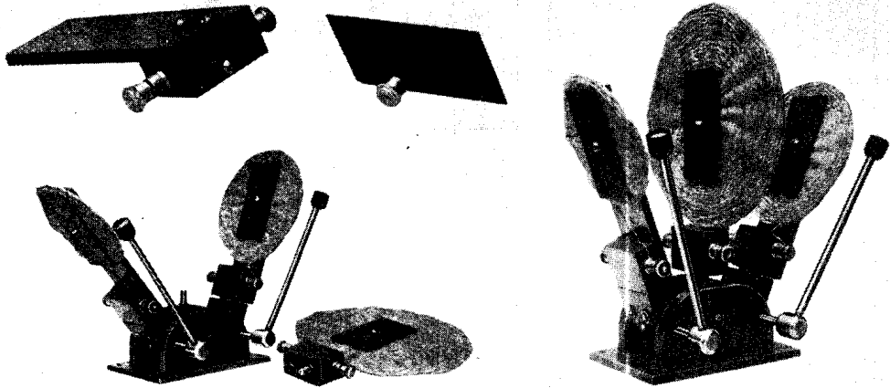
Fig. 10. Mounts are made for adapting standard types of coil holders as used for Igranic, Burndept and other makes of plug-in coils, to take basket coils. In this photograph the mounts shown are made by Will Day & Co. Fig. 11. Another example of the same principle applied to a standard form of holder is here given. Fig. 12. Shows the method of attaching and detaching the coils to standard holders employing adaptors
