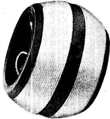
Fig. 6. A common type of reactance ball coil is as the one illustrated. This is a spherical form of inductance coupling, which is more economical in space than many other types of coil effecting the same purpose
