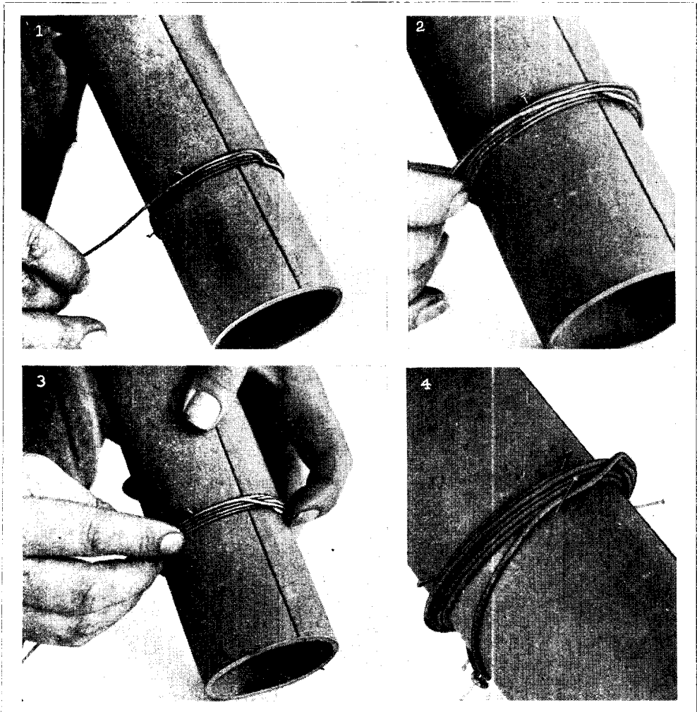
FOUR STAGES IN MAKING A BANK-WOUND COIL
