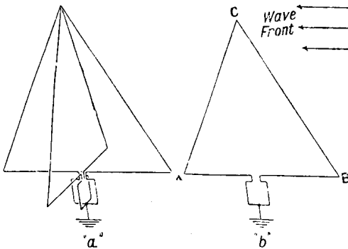
BELLINI-TOSI AERIAL
