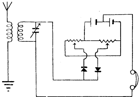
CIRCUIT FOR BALANCED CRYSTALS
