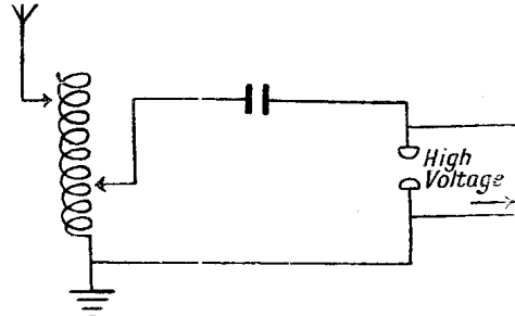
AUTO-TRANSFORMER COUPLING
