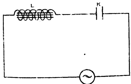
CONDENSER TO BALANCE INDUCTANCE
