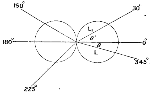
PLOTTING CURVE FOR BELLINI-TOSI AERIAL
