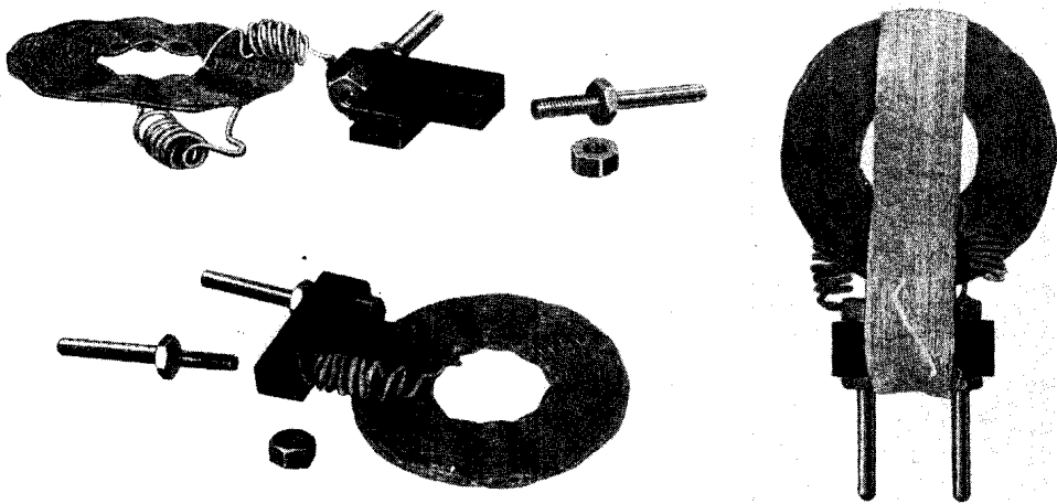
Fig. 13. After the T-shape piece of ebonite has been cut as shown in this photograph, the arms of the T are drilled to provide for the fixture of two valve legs. A longitudinal saw cut to enable the coil to be inserted is then made, and this simple but efficient device is almost complete. Fig. 14. Gives a clear idea of how contact is made between the coil and the valve legs. Fig. 15. Shows the coil mounted
