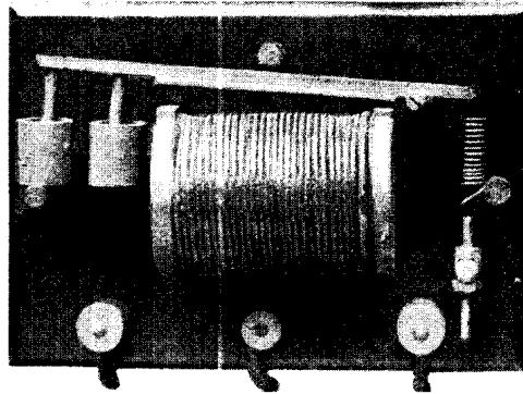
AUTOMATIC CUT-OUT
