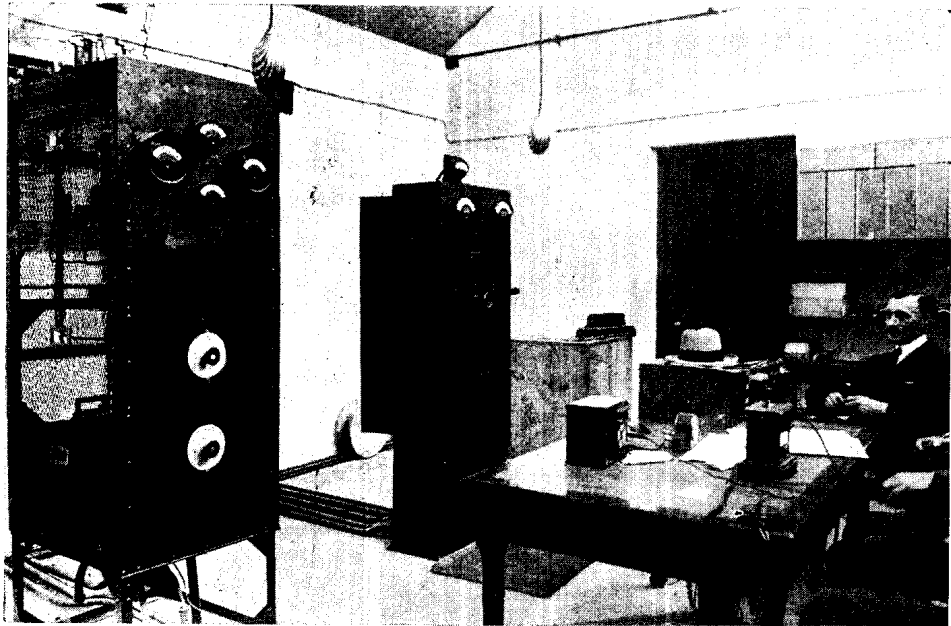
Fig. 2. Transmitting valves are used for broadcasting from the Birmingham station, 5 I T, with a plate current voltage of 1,600 and a filament current supplied at 14.5 volts. The control panels are shown in this photograph
