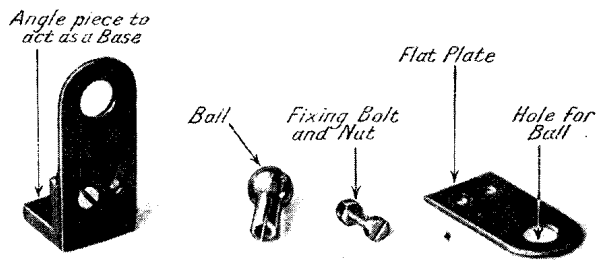
BALL-BEARING COMPONENTS
