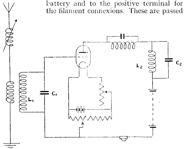
AUTO-HETERODYNE RECEPTION
