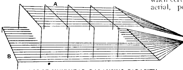
LODGE-MUIRHEAD BALANCING CAPACITY
