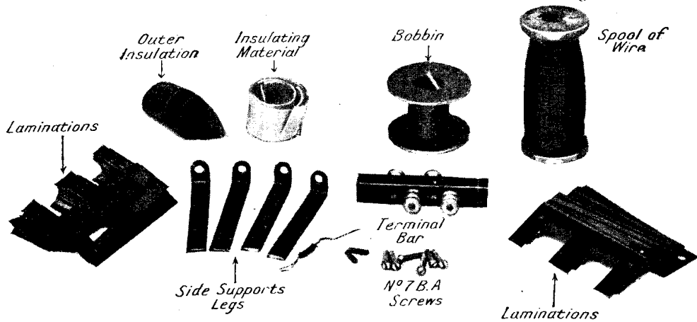
PARTS OF AN AUDIO-FREQUENCY TRANSFORMER BEFORE BUILDING UP
