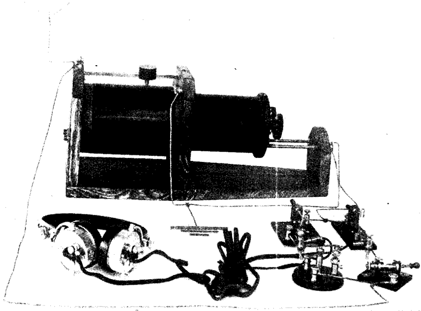
QUADRECTOR CIRCUIT ARRANGEMENT FOR REDUCING INTERFERENCE
