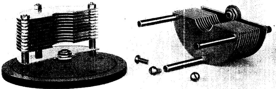
REARRANGEMENT OF PARTS TO MAKE A BALANCED CONDENSER
