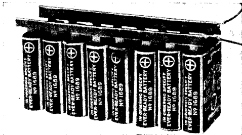
Fig. 4. Parallel connexions may be made with the same kind of batteries as used in Fig. 3, but in this case it will be noted all the positive terminals are connected together and all the negative together
