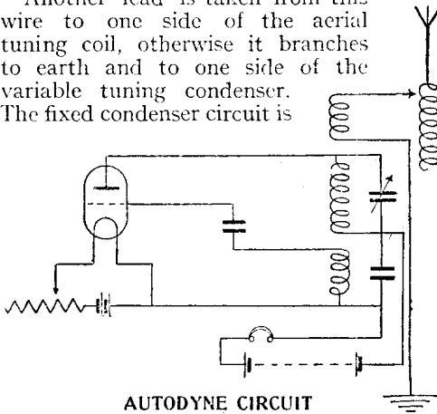
Fig. 2. Many variations of design of circuit are possible in autodyne reception. Above is an example
