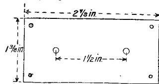
CONDENSER BASE
