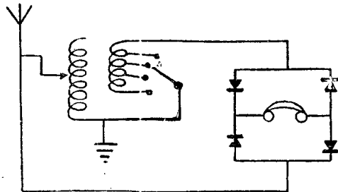
QUADRECTOR, OR FOUR-CRYSTAL, CIRCUIT
