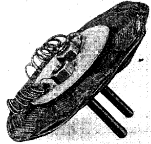
BASKET COIL MOUNT
