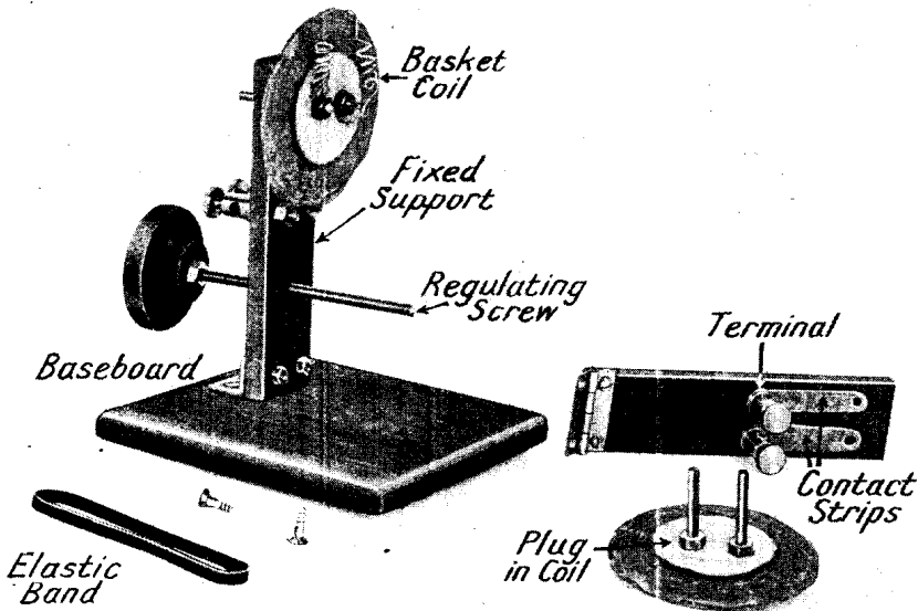
COMPONENTS OF HOME-MADE BASKET COIL HOLDER
