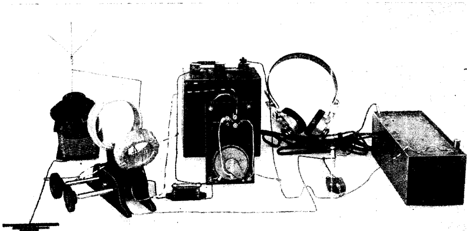
PHOTOGRAPHIC LAY-OUT OF AN EXPERIMENTAL AUTODYNE RECEIVER
