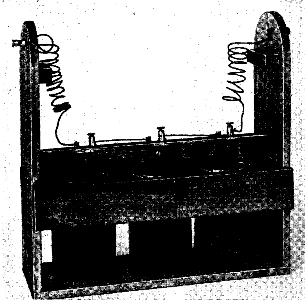
BICHROMATE BATTERY FROM JAM JARS
