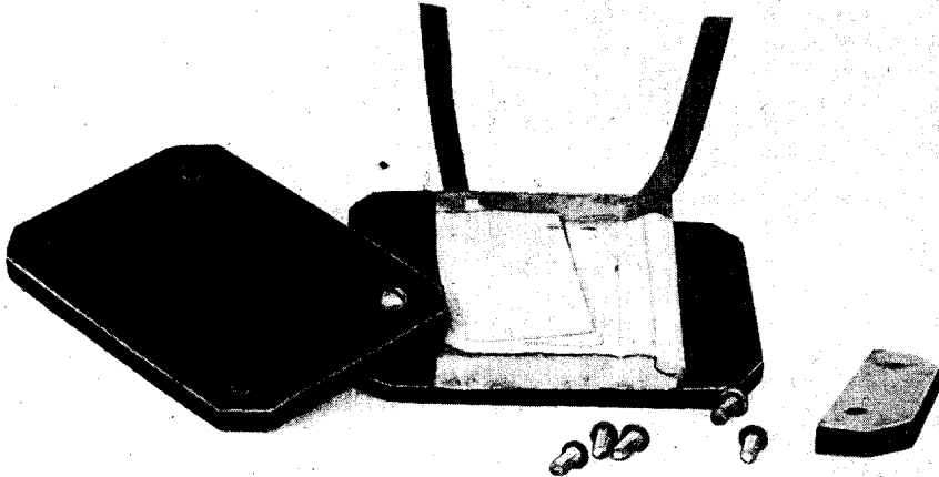
Fig. 5. Tinfoil and waxed paper layers may be seen in this photograph. A blocking condenser has been dissembled to show the various parts and general construction. Note the contact strips
