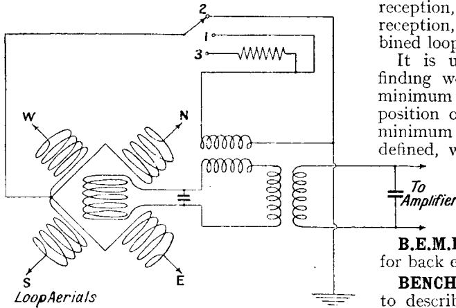
BELLINI-TOSI AERIAL
