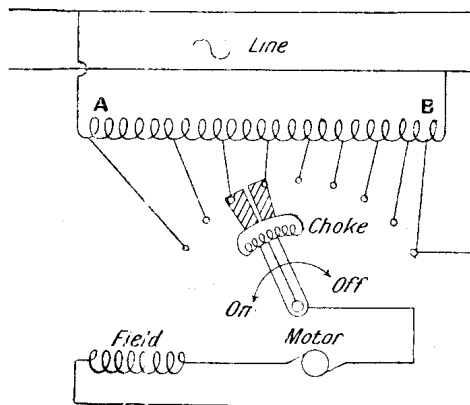
AUTO-STARTER FOR ALTERNATING MOTORS Fig. 1. Connexions are shown of a single-phase commutator with auto-starter
