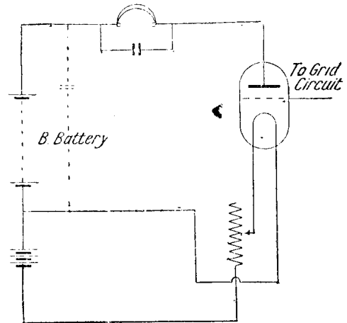
HIGH-TENSION OR B BATTERY CIRCUIT
