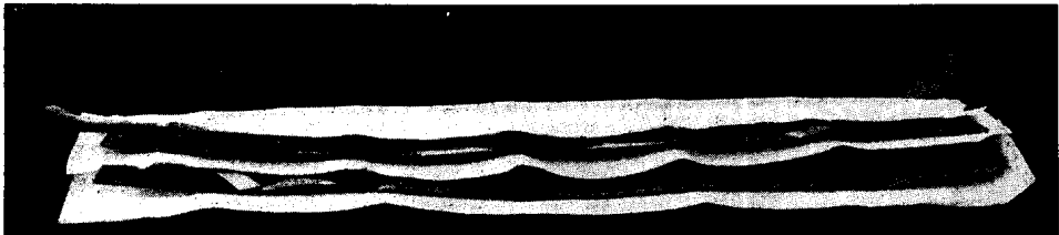
Fig. 6. Paraffin-waxed paper is here seen insulating the strips of tinfoil in the order in which they are placed in the blocking condenser. The contact strips may also be seen in position
