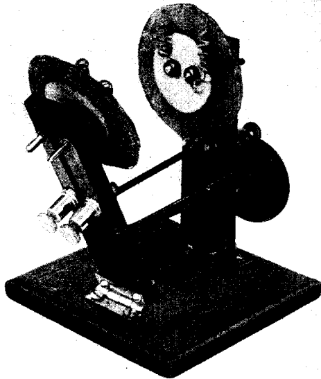
HOLDER FOR TWO BASKET COILS
