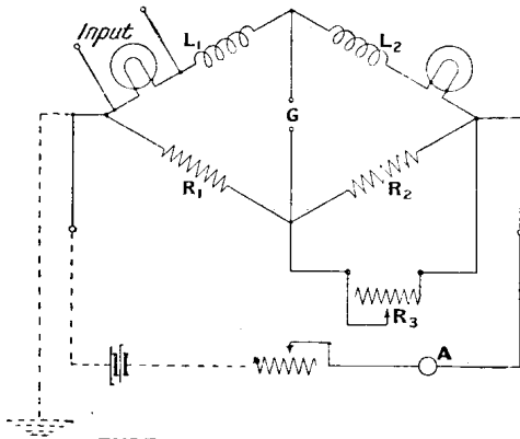
EXPERIMENTAL BOLOMETER
