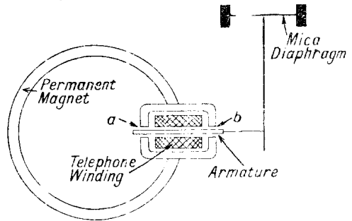
BALDWIN TELEGRAPHY RECEIVER
