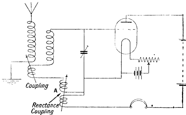
Fig. 7. Reactance coupling by ball-type coils is effected in this circuit diagram. The method of coupling the two windings will be seen, as well as the general wiring arrangements
