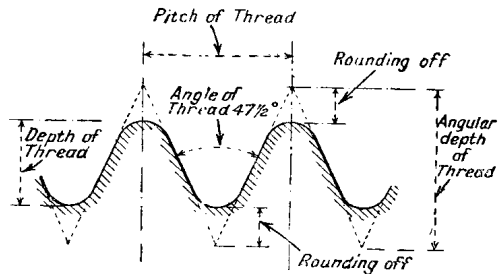
SCREW THREADS
