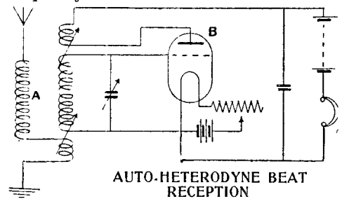
Fig. 4. Detection and generation of local oscillations are carried out in the auto-heterodyne method as shown in the above diagram
