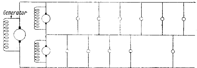
BALANCER ON THREE-WIRE SYSTEM
