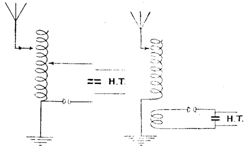
Fig. 1. An auto-coupled aerial
