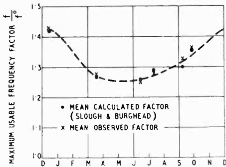
Fig. 6. Mean seasonal variation of m.u.f. factors; near noon; calculated and observed. D = 715 km.
