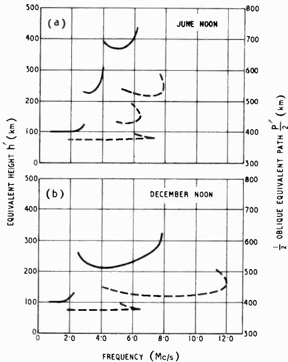
Fig. 1. Equivalent height/frequency curves for normal (—) and oblique (----) incidence; D = 715 km.
