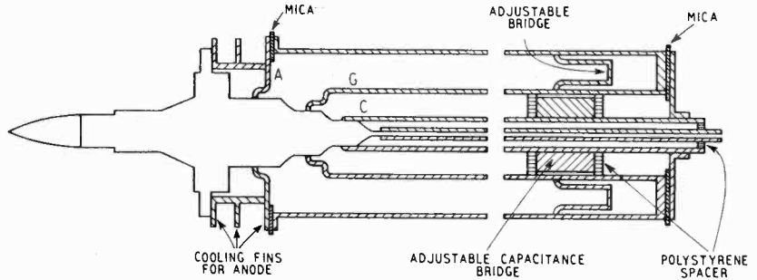
Fig. 4. Common-grid earthed-anode circuit for use with valve Type E1274.
