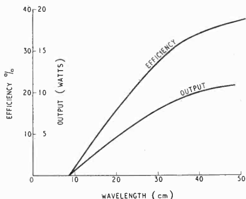
Fig. 5. Performance of valve Type E1274 at a constant input of 30 watts.
