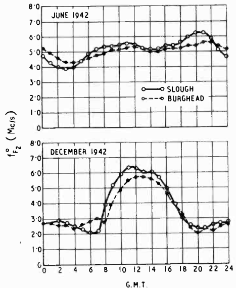
Fig. 5. Mean diurnal variation of region F_2 critical frequencies Slough and Burghead.
