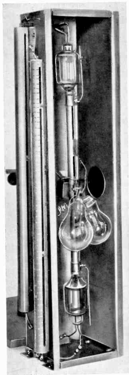
Fig. 6. Original double-ended concentric oscillator using two experimental triodes with ring seals of eight wires for the anode leads. The wavelength is 90 cm and the scale is shown by the engravings on the cathode lines which are 1 cm apart.
