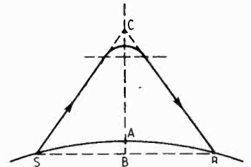
Fig. 2. Method of allowing for the earth's curvature.
