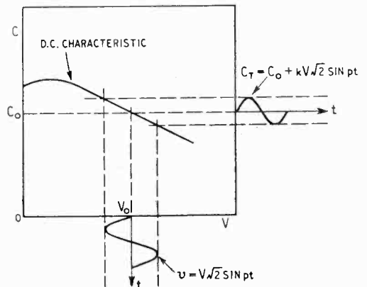
Fig. 3. Illustrates cyclic capacitance variation using alternating polarizing voltages.
