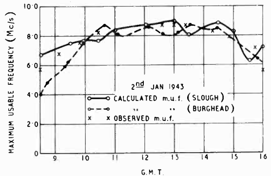
Fig. 7. Calculated and observed maximum-usable frequencies (ordinary ray component).
