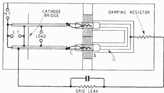
Fig. 7. Push-pull common-anode earthed-anode oscillator derived from the type of oscillator shown in Fig. 4 by bending the half-wave resonator into U-shape.
