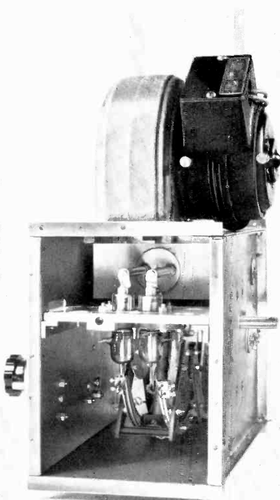
Fig. 9. Two CV55 triodes in a push-pull common-anode earthed-anode oscillator with parallel-wire lines between the grids and between the cathodes. The cathode line is in the form of an arc to give longer tuning adjustment. The output is taken by means of a loop coupled near the cathode bridge and connected to a co-axial feeder which ultimately comes out at the side of the box. The circuit as shown is for a wavelength of about 60 cm.
