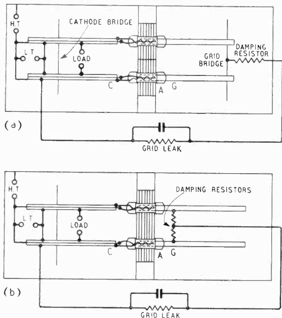
Fig. 8. Longer-wave versions of the push-pull common-anode earthed-anode oscillator. In (a) both grid and cathode circuits are parallel-wire lines tuned by shorting bridges. In (b) an open-ended grid line is used and the d.c. grid leads are attached at the voltage node. Circuit (b) will operate at a higher frequency than (a).
