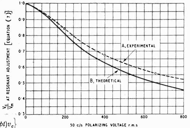
Fig. 11. Variation of height of resonance curve with 50-c/s polarizing voltage [Equation (7)].
