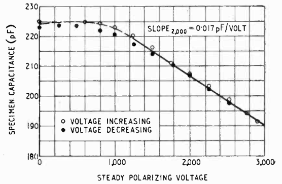
Fig. 2. D.C. capacitance/voltage characteristic of (70:30) (BaSr) \text{TiO}_3 at 1 Mc/s; temperature 21.5^\circ\text{C} .
