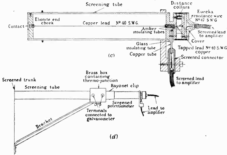
Fig. 3.—Details of screened potentiometer for supplying known potential differences to a wireless receiver.
