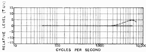
Fig. 12.—Response of glow-lamp recorder ———; response with electrical resonance - - - - -.
