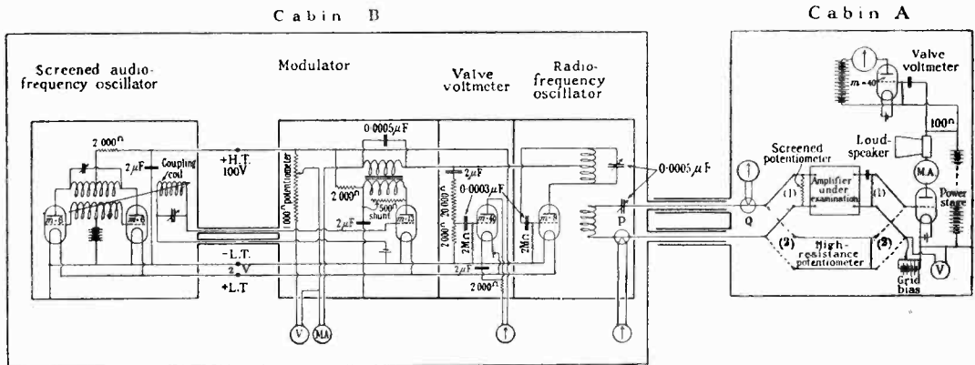
Fig. 5.—Circuit diagram of apparatus for testing the performance of radio receivers.
