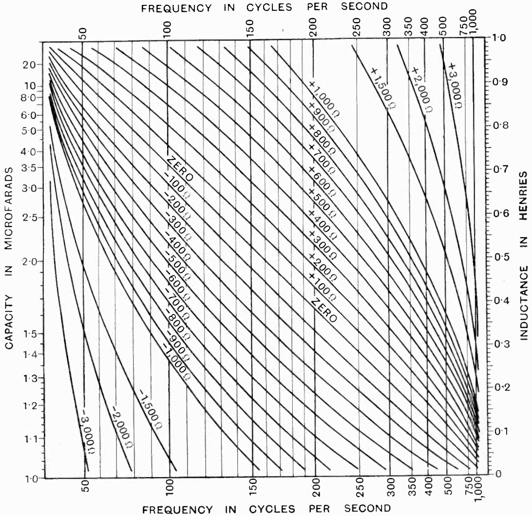
Fig. 4.—Reactance of series combination (audio-frequencies). Copyright by Author.
