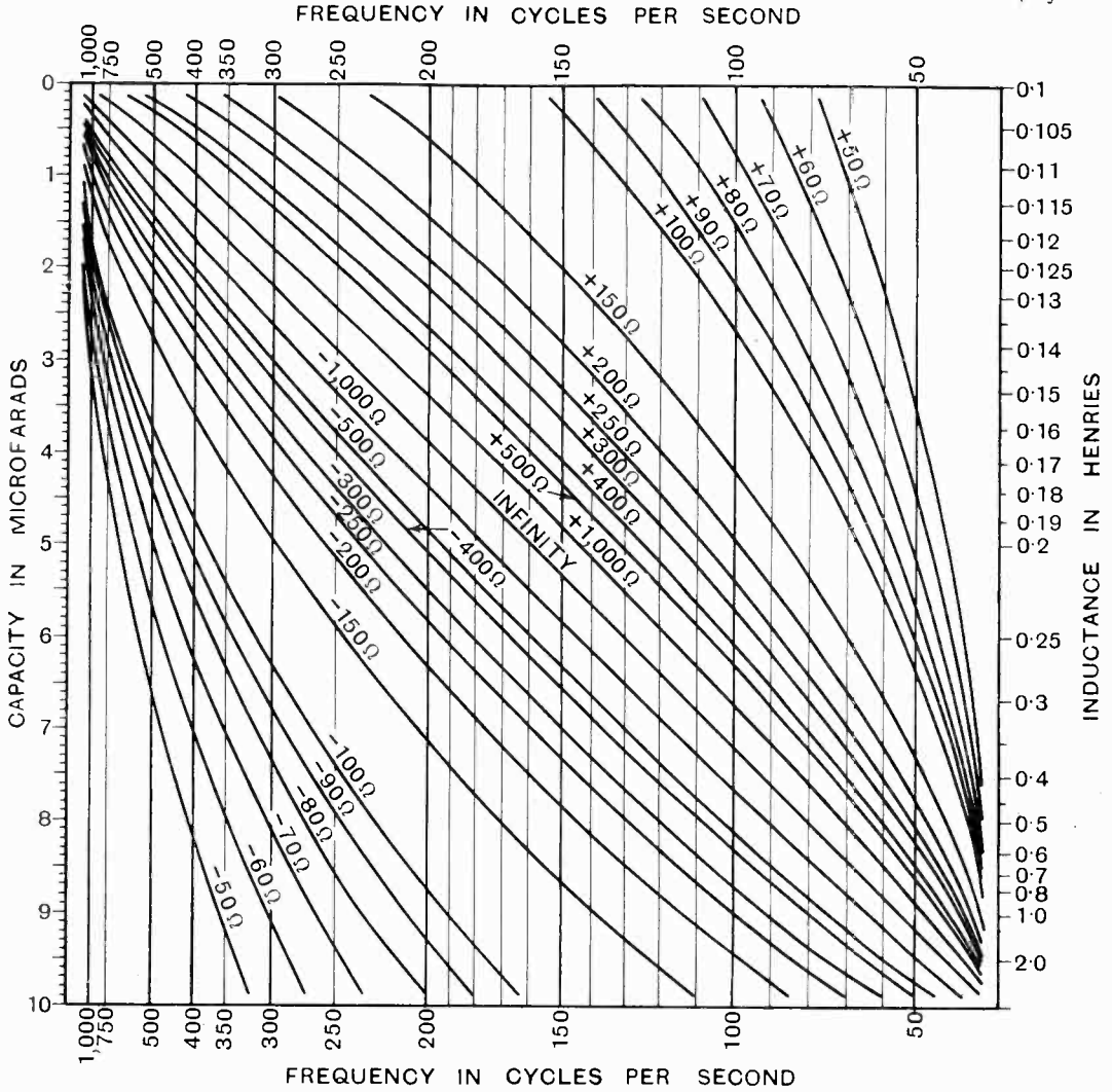
Fig. 5.—Reactance of parallel combination (audio-frequencies). Copyright by Author.
