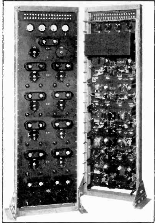
Marconi frequency doubling circuit for tuning fork drive.
