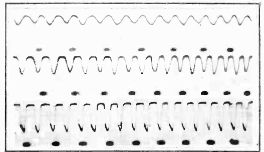
Fig. 5.—Output valve overloaded.
