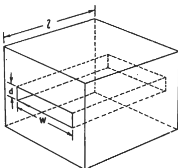
Fig. 4.2—NARROW SLOT HAVING SIMILAR ACOUSTICAL IMPEDANCE TO NARROW TUBE
