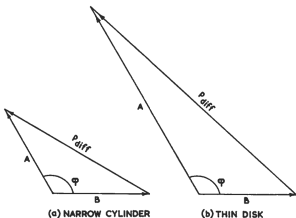
Fig. 5.2—DIFFERENTIAL-PRESSURE VECTORS
