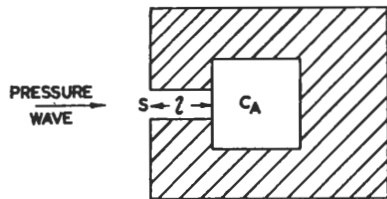
Fig. 4.4 — ACOUSTICAL SYSTEM SIMILAR TO HELMHOLTZ RESONATOR
