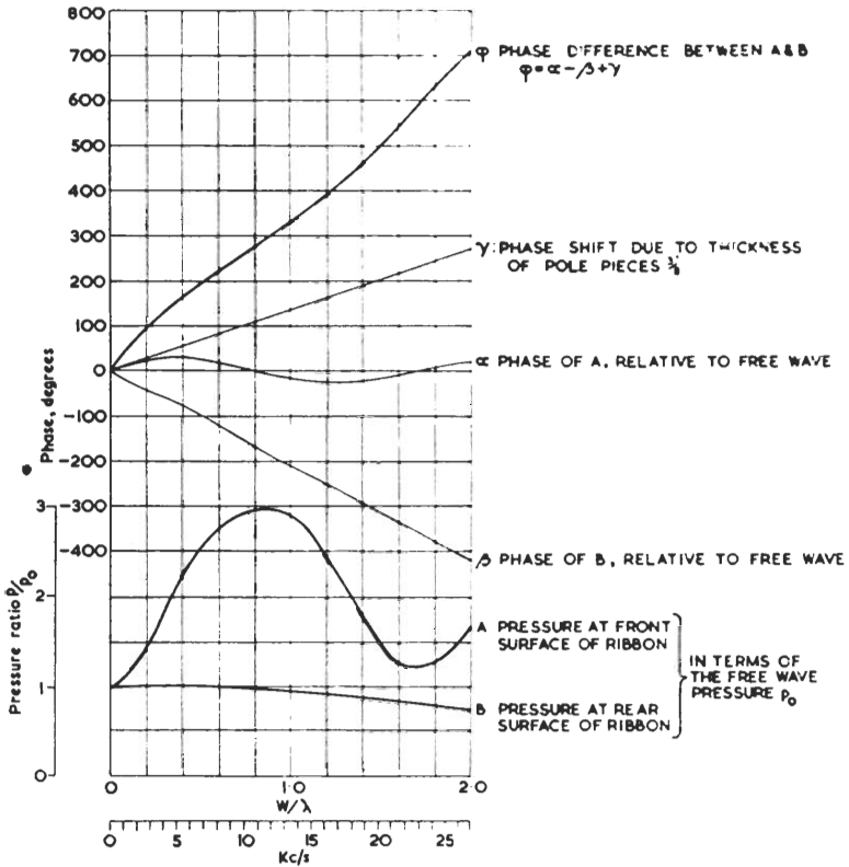
Fig. 40—MAGNITUDE AND PHASE OF PRESSURES
