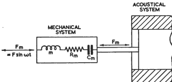
Fig. 4.5—COUPLING OF MECHANICAL SYSTEM TO ACOUSTICAL SYSTEM
