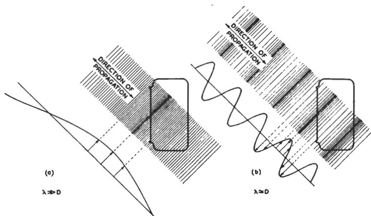
Fig. 28—EFFECT OF PHASE DIFFERENCE ACROSS DIAPHRAGM
