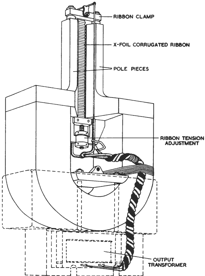
Fig. 37.—BBC-MARCONI RIBBON MICROPHONE
