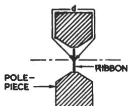
Fig. 15—CROSS-SECTIONAL REPRESENTATION OF RIBBON MICROPHONE : SHOWING EFFECTIVE PATH LENGTH, d , FOR VERY LOW FREQUENCIES
