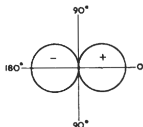
Fig. 34—POLAR DIAGRAM FOR DIFFERENTIAL-PRESSURE MICROPHONE AT LOW FREQUENCY
