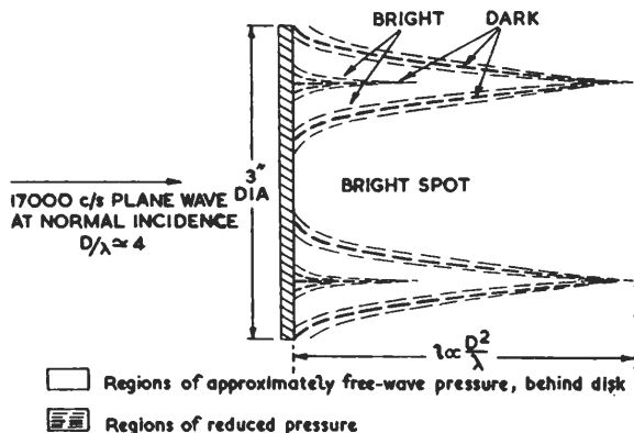
Fig. 25—APPROXIMATE CROSS-SECTIONAL REPRESENTATION OF SOUND SHADOW BEHIND A RIGID DISK
