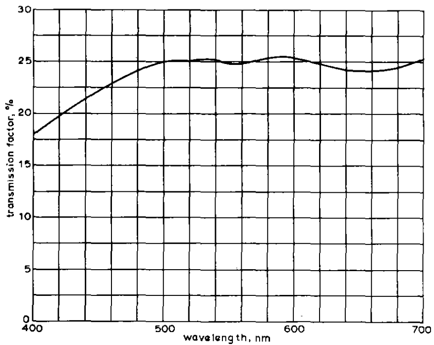
Fig. 6 — Transmission characteristic of typical gelatine neutral density filter ( ND=0.6 ) as a function of wavelength
