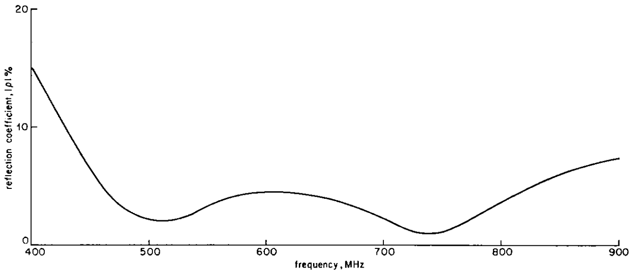
Fig. 3 Reflection coefficient of four-way transformer
