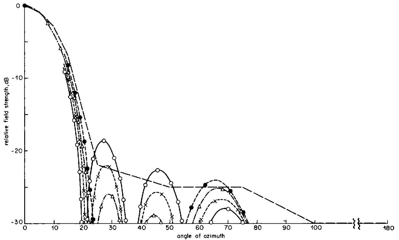
Fig. 5 Effect of current ratio on side-lobe level ○— 1:1.5:1.5:1 x--- 1:1.75:1.75:1 ▲—•— 1:2.0:2.0:1 ●— 1:2.25:2.25:1 — Directivity assumed in calculating co-channel interference
