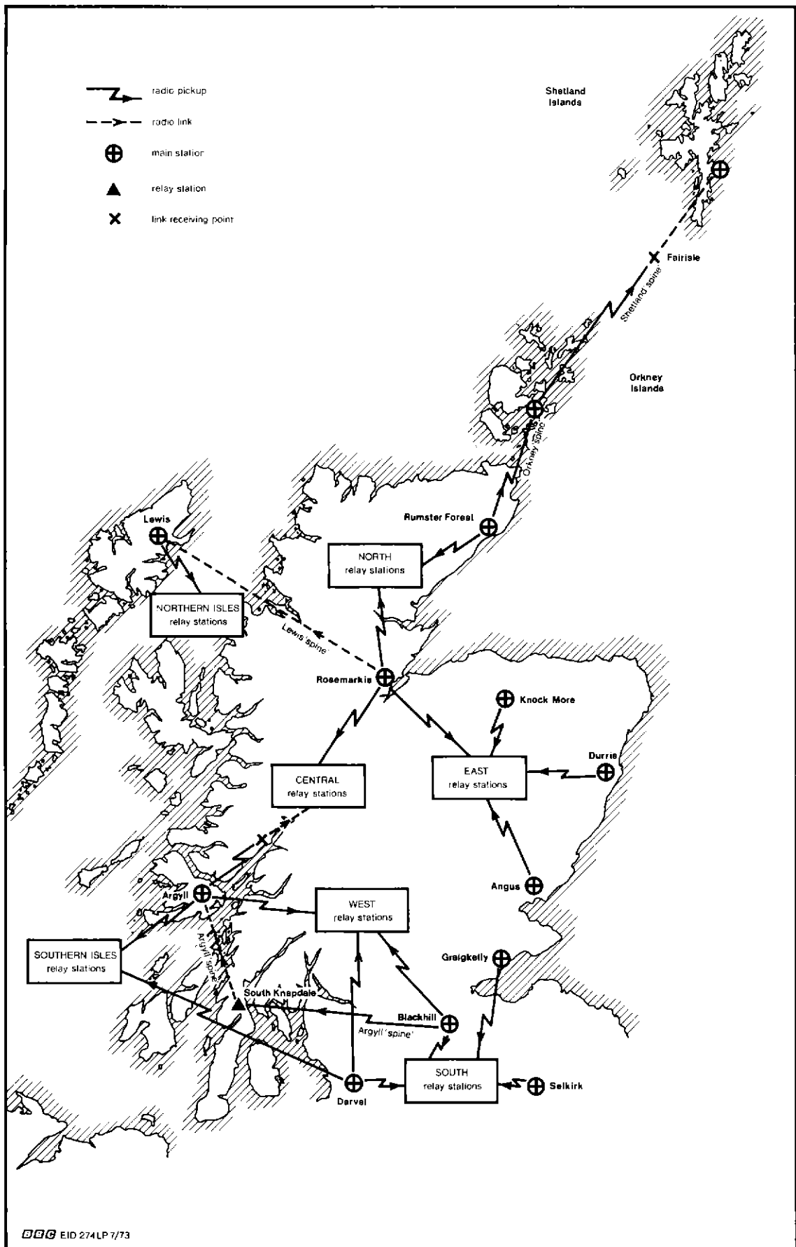
22 Fig. 1 UHF Coverage Plan for Scotland
