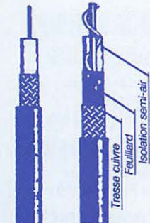
RG 213 H 1000
