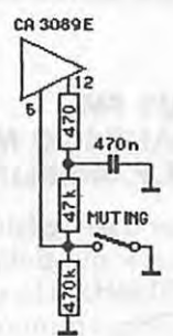
Figure 15 : Circuit "Muting".
