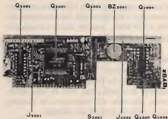
CONTROL UNIT
