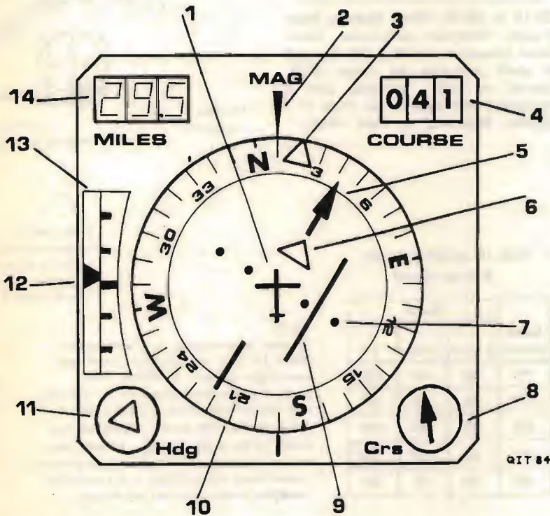
HSI - Horizontal Situation Indicator
