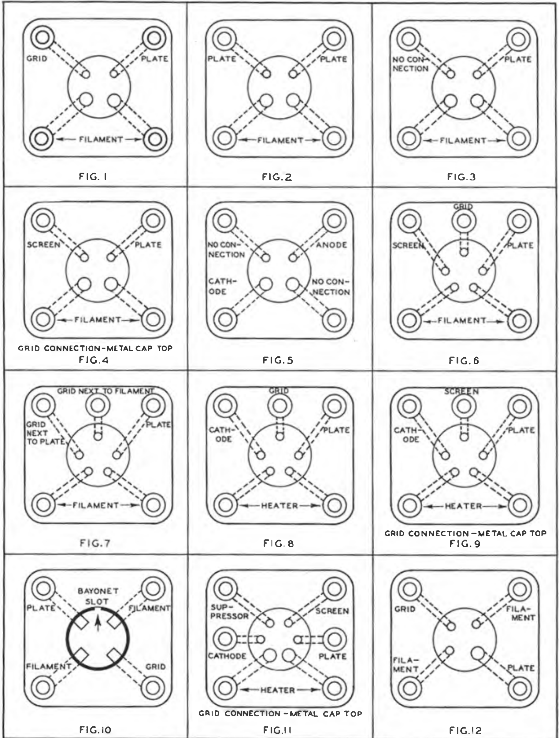
TOP VIEWS OF SOCKETS
