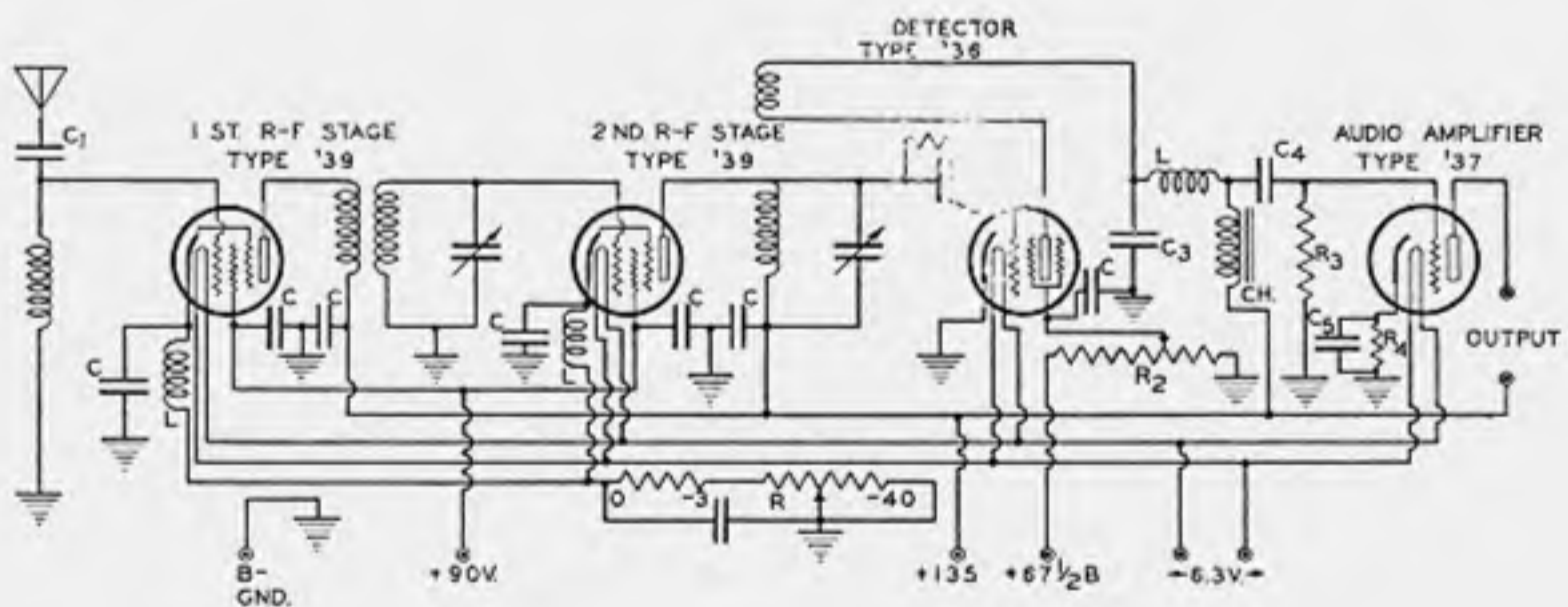
DIAGRAMMATIC SHORTWAVE RECEIVER 6.3-VOLT HEATER TYPE TUBES
