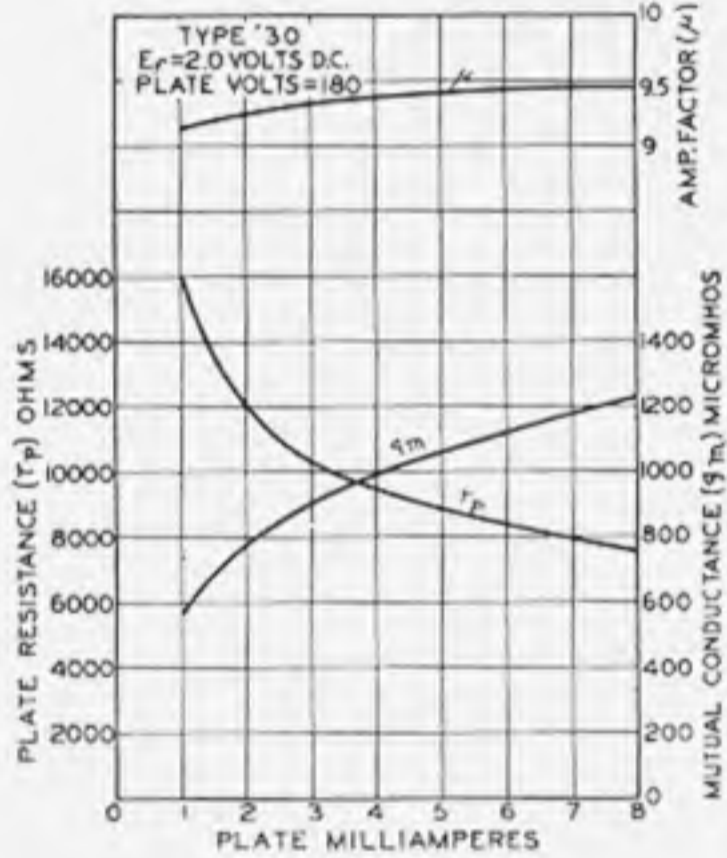
AVERAGE PLATE CHARACTERISTICS
