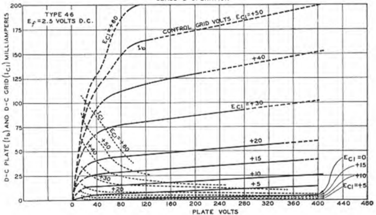
OPERATION CHARACTERISTICS CLASS B OPERATION
