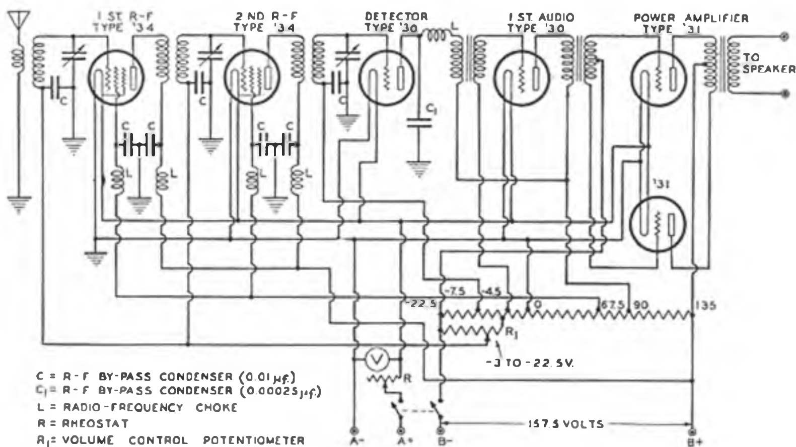
TYPICAL TUNED RADIO-FREQUENCY CIRCUIT 2-VOLT FILAMENT TYPES
