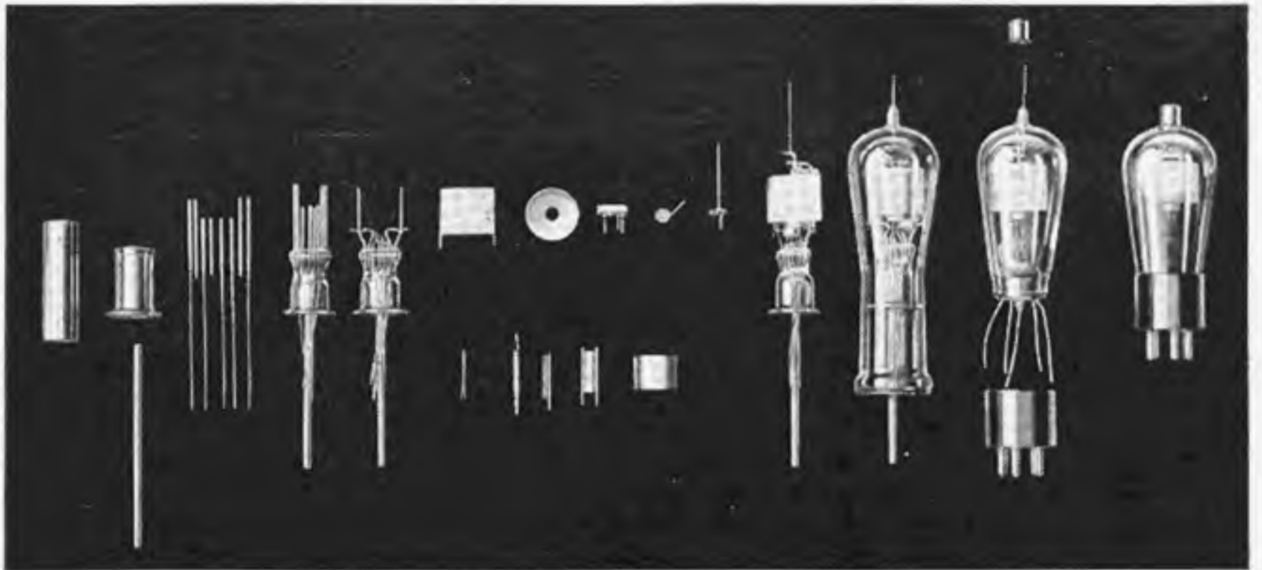
Parts Assembly of the '24-A
