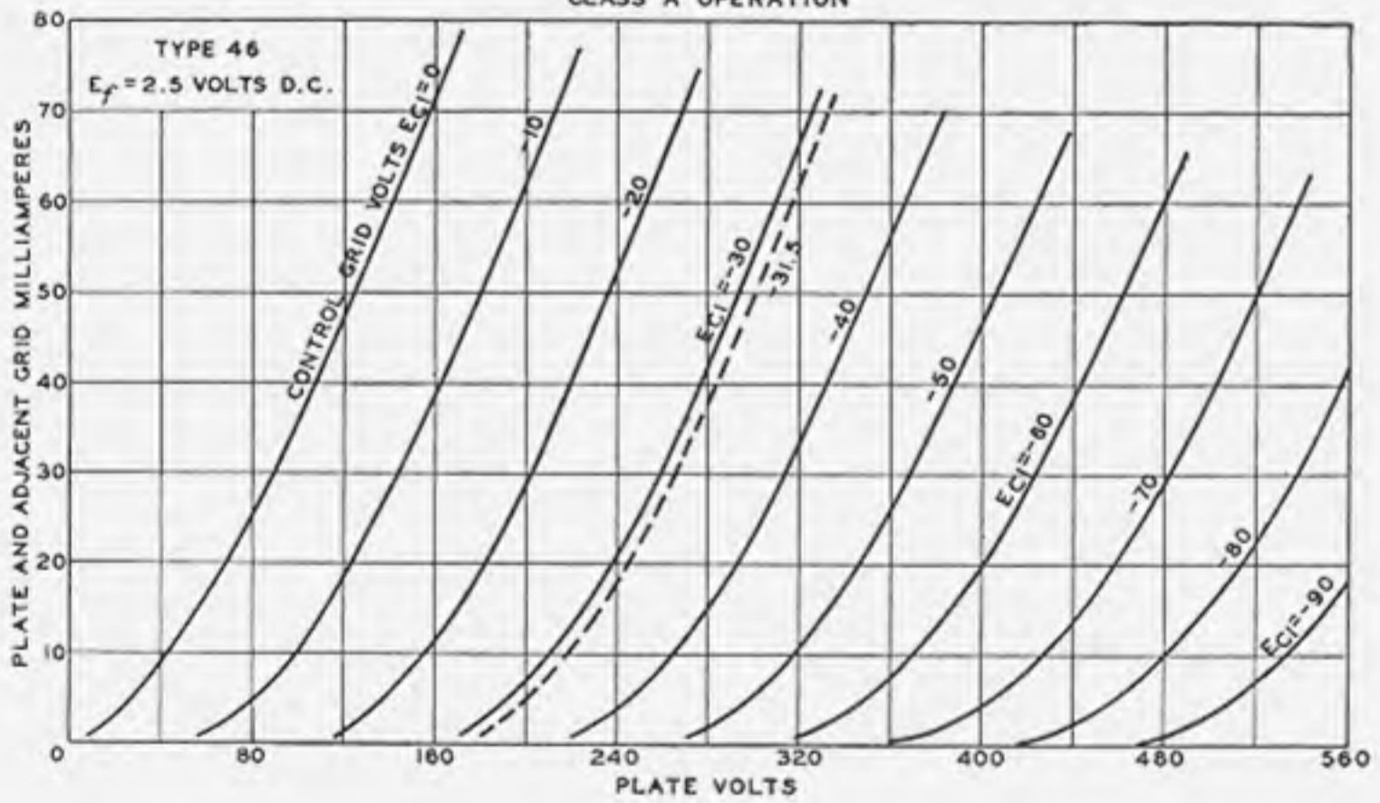
AVERAGE PLATE CHARACTERISTICS CLASS A OPERATION
