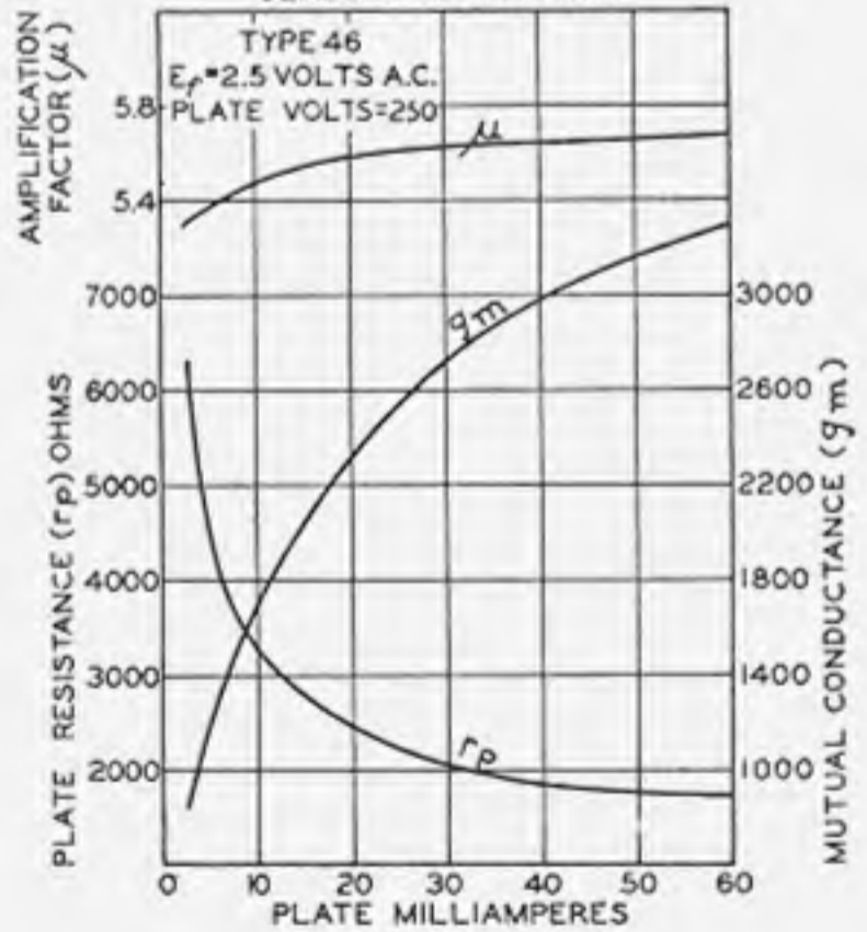
AVERAGE CHARACTERISTICS CLASS A OPERATION
