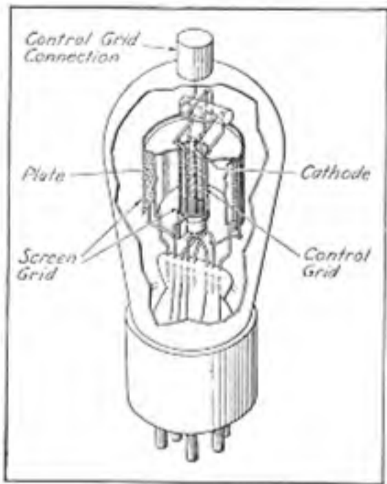
Interior View of '24-A
