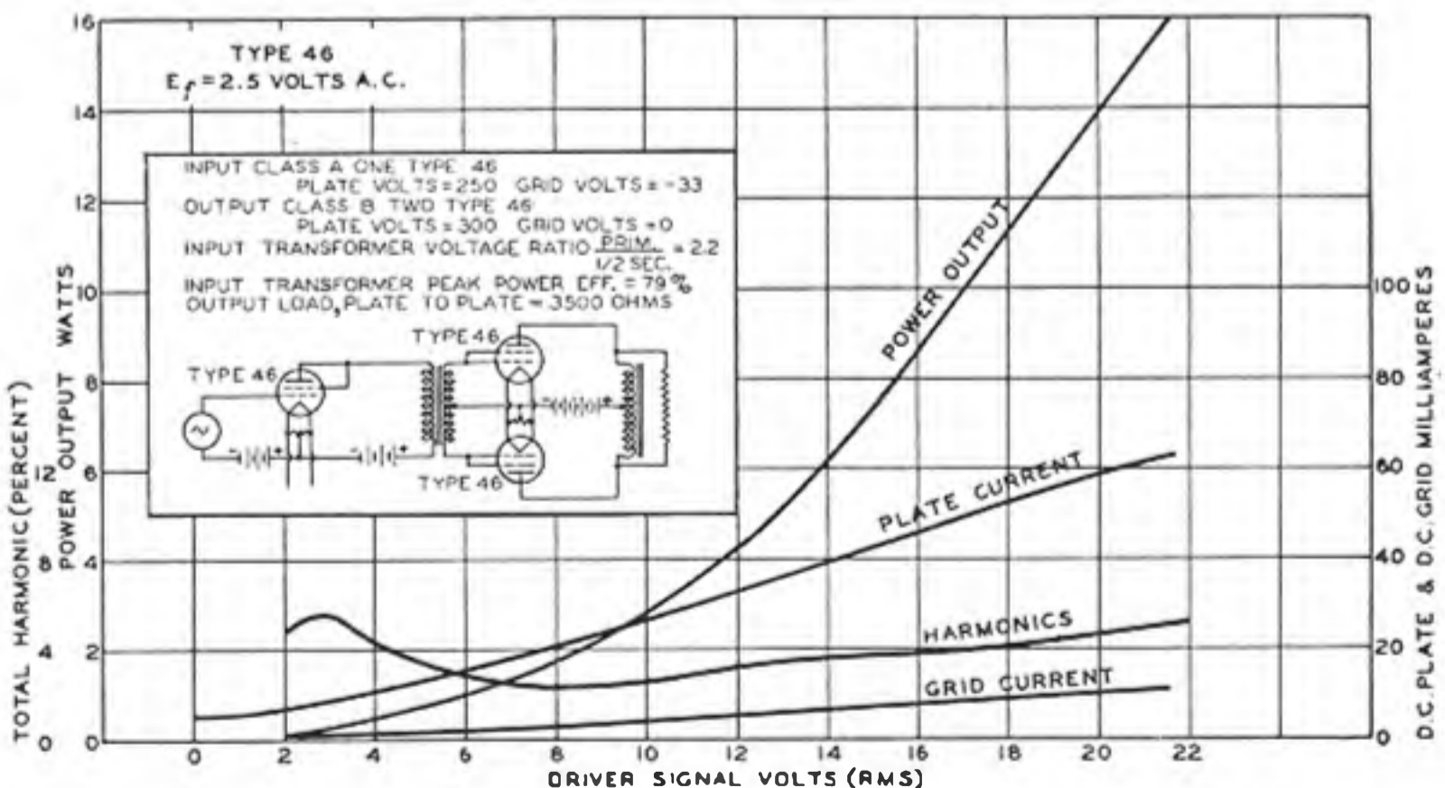
OPERATION CHARACTERISTICS CLASS B OPERATION
