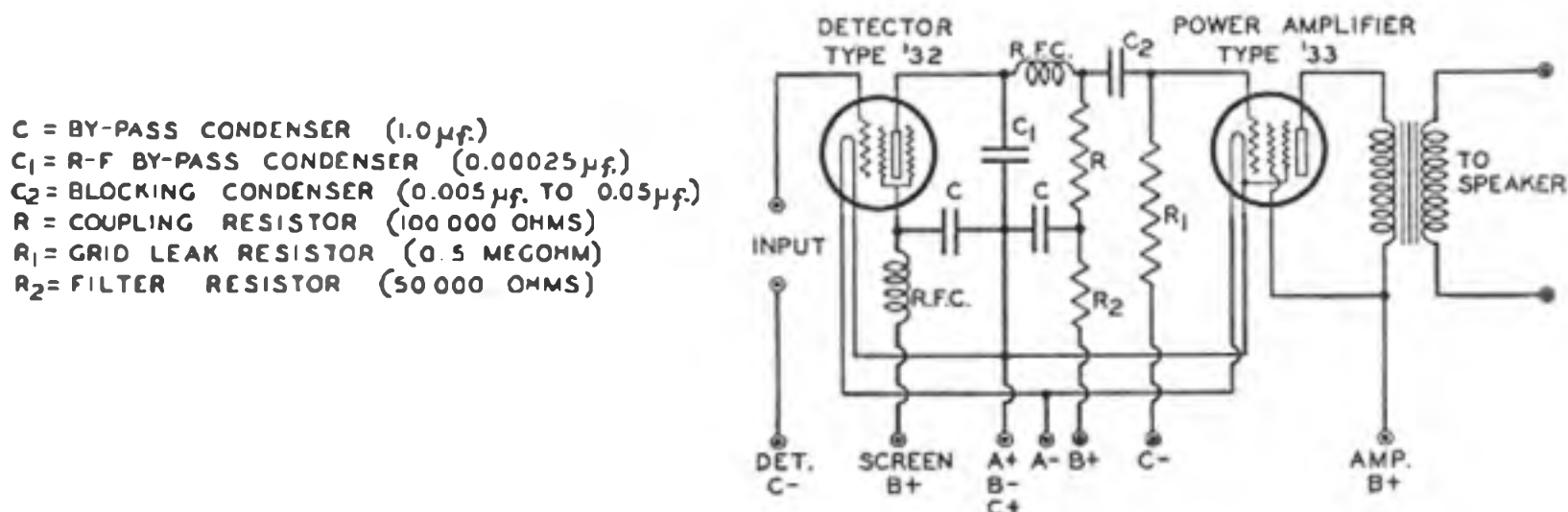
OPTIONAL DETECTOR AND AMPLIFIER—2-VOLT FILAMENT TYPES
