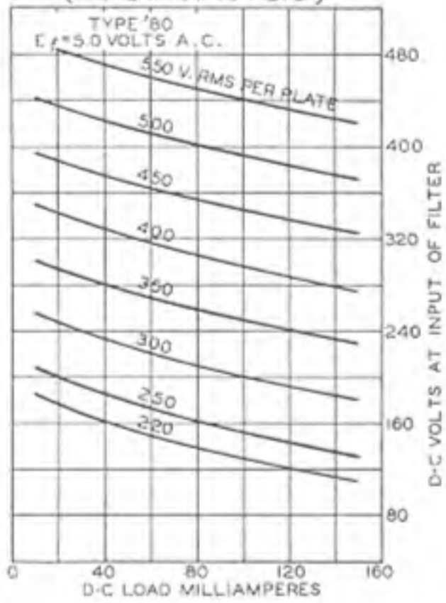
OUTPUT CHARACTERISTICS (CHOKE INPUT TO FILTER)
