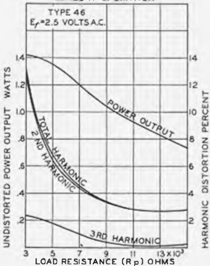
AVERAGE CHARACTERISTICS CLASS A OPERATION
