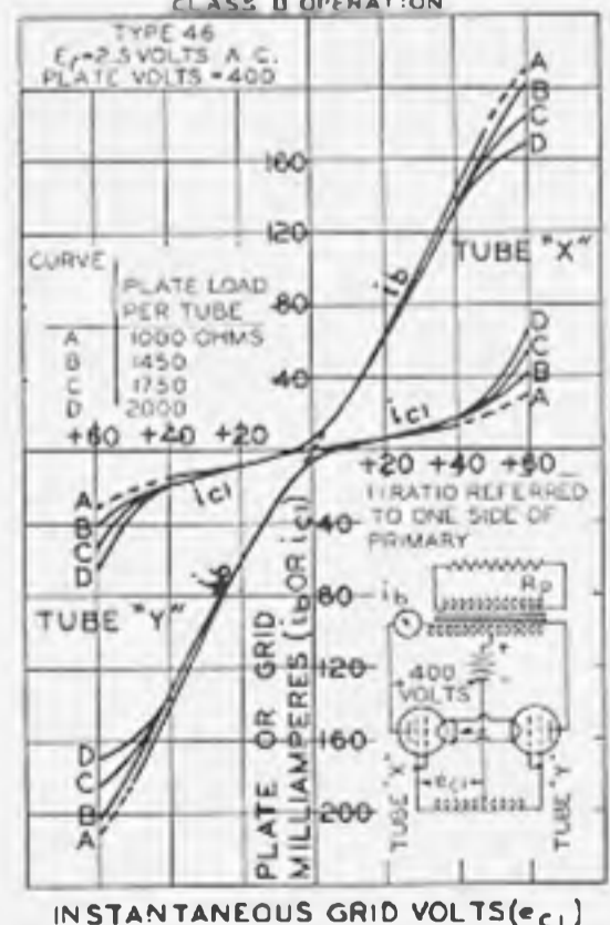
DYNAMIC TRANSFER CHARACTERISTICS CLASS B OPERATION
