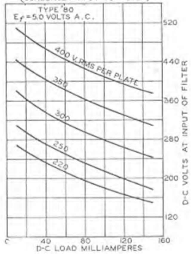
OUTPUT CHARACTERISTICS (CONDENSER INPUT TO FILTER)
