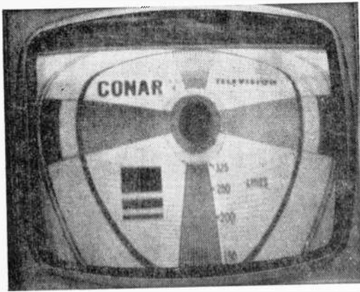
Fig. 24. Flat-topped circle can be made round again by adjusting both the vertical linearity and the vertical height controls together.
