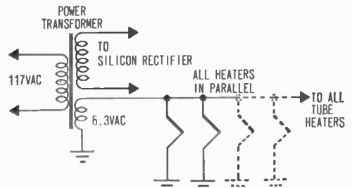
Fig. 11. In transformer type set, one or two filaments may not light up indicating tube or associated heater wiring is defective. If no tubes light up in this type of set, check the power transformer, fuses in AC or filament line or circuit breaker, and AC switch.
