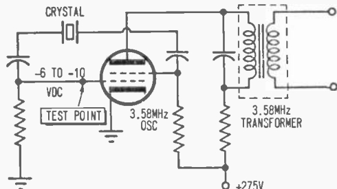
Fig. 7. Circuit of typical 3.58 MHz oscillator. A voltage check with a VTVM will determine if it's OK.
