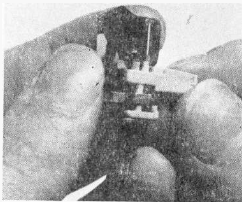
Fig. 7. To remove the stylus assembly from this type cartridge, position the turnover lever as shown.
