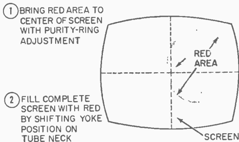
Fig. 8. The red area of the TV screen has to be centered and then expanded to fill the screen.
