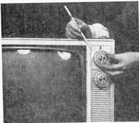
Fig. 25. Final tune-up consists of adjusting tuner slugs to center range of fine-tuning.
