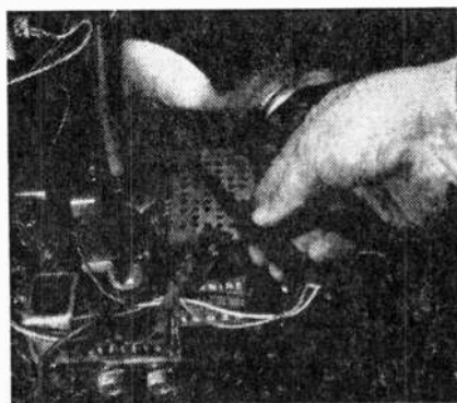
Short circuit voltage stored in picture tube by touching insulated screwdriver to anode and chassis a few times.
