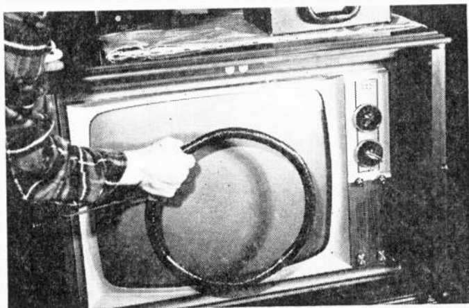
Fig. 14. (right) Degauss the CRT even if there is a built-in degaussing coil.
