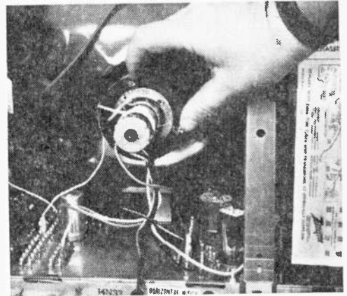
Fig. 18. Magnetic rings on picture tube behind yoke are used to center picture. The two tabs are rotated around neck for both correct horizontal and vertical centering.
