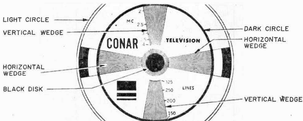
Fig. 8. Test pattern transmitted by most TV stations before and after regular programming is invaluable for adjusting set's controls. Important elements are labeled above.
