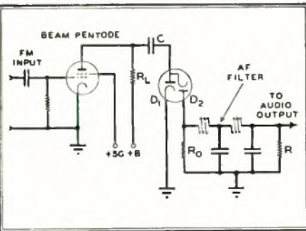
FIG. 65. COUNTER CIRCUIT TYPE OF FM DETECTOR
