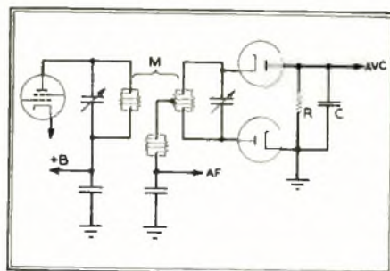
FIG. 65C. RATIO DETECTOR CIRCUIT
