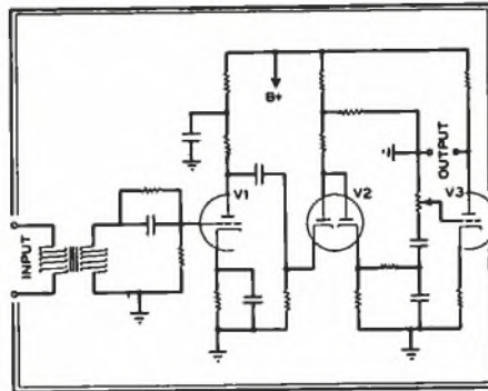
Fig. 8. The basic Motorola IDC circuit
