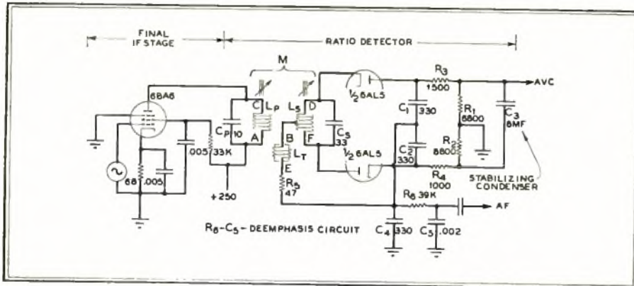
FIG. 65i. RATIO DETECTOR WITH BALANCED PHASE-SHIFT TRANSFORMER, FEEDING 6AL5
