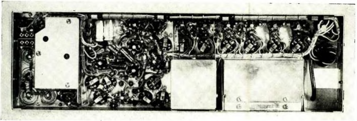
This picture of the under side of the complete receiver section can be more readily understood by comparing it with Fig. 2, which shows the chassis and separate decks. In this view, the RF tuner is at the left, and the meter socket at the right
