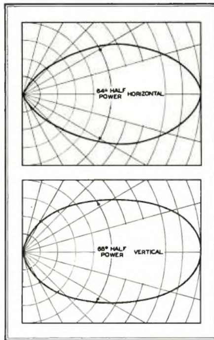
Fig. 29. Stacked array radiation patterns
