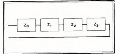
Fig. 20. Equivalent of series-fed colinear
