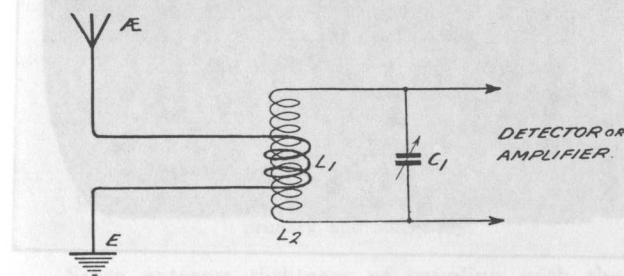
Fig. 43. A typical circuit employing the aperiodic aerial system.
