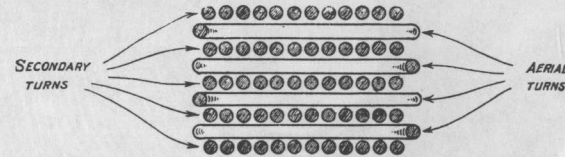
Fig. 45. A section of a lattice winding containing both primary and secondary.
