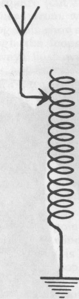
Fig. 3. The wrong way to connect a tapped or slider coil in circuit.
