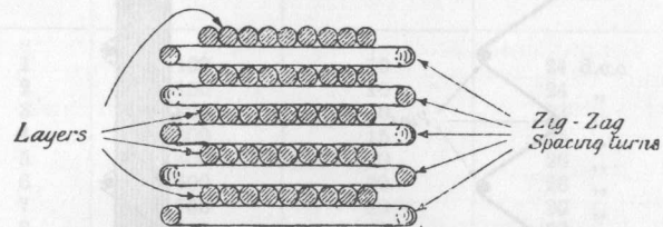
Fig. 27. Section of a lattice winding.
