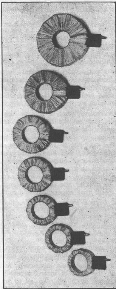
Fig. 2. Seven coils of the Burndepth series. The coils are designed with a progressive increase in turn numbers, as may be seen from their size, so that they cover a wide range of wavelengths without gaps.
