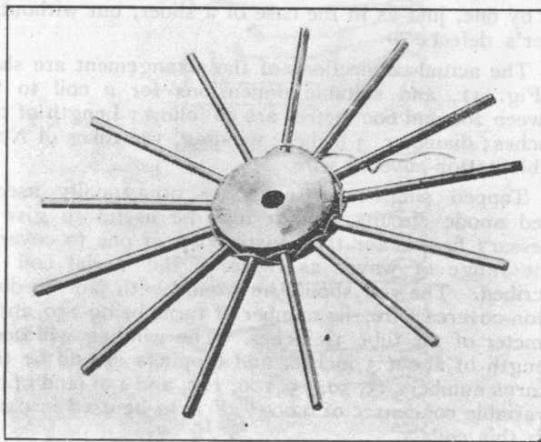
Fig. 12.—A "spider" for the winding of basket coils. Two complete turns are shown in position.
