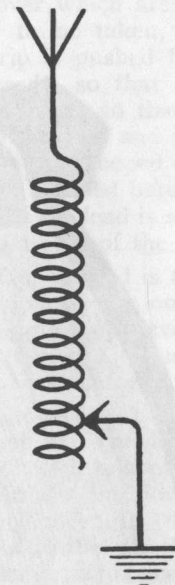
Fig. 4. How to arrange a coil to reduce dead-end effects.
