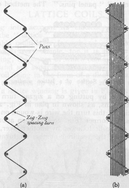
Fig. 29. Stages in the winding of a lattice coil.
