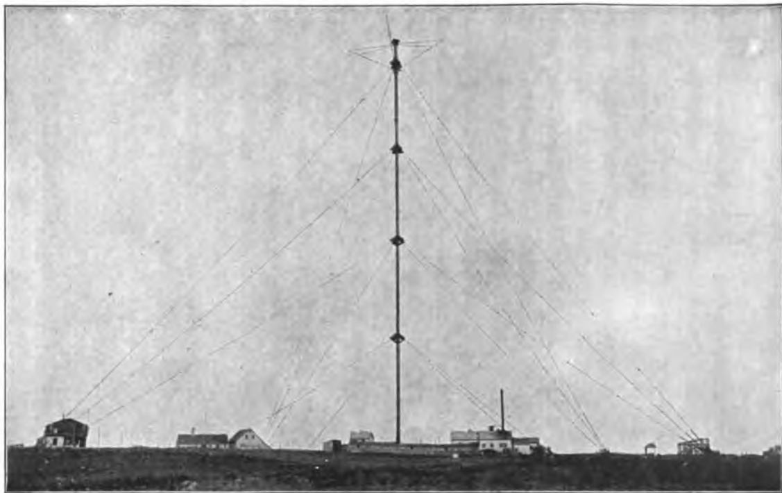
FIG. 9.—MAST FOR SUPPORTING ANTENNA, FESSENDEN TRANS-ATLANTIC STATION, BRANT ROCK, MASS.
