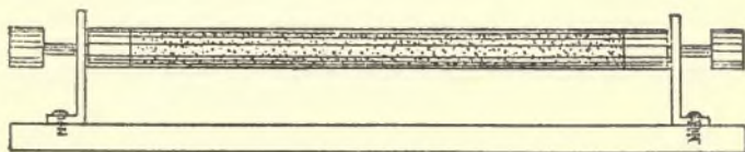
FIG. 135.—LODGE COHERER.
