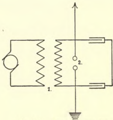
FIG. 127A.—FLEMING OSCILLATOR.
