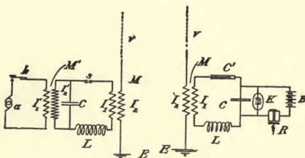
FIG. 302.—STONE MULTIPLEX SYSTEM.
