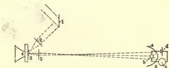
FIG. 313.—BELL RADIOPHONE.
