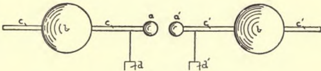
FIG. 54.—HERTZ'S ADJUSTABLE OSCILLATOR.
