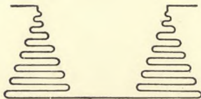
FIG. 234c.—MARCONI LOW-POTENTIAL TRANSFORMER. (Third Form.)
