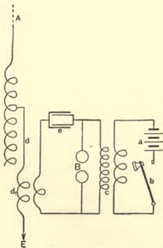
FIG. 297.—MARCONI SYNTONIC SYSTEM. (Second Form.)
