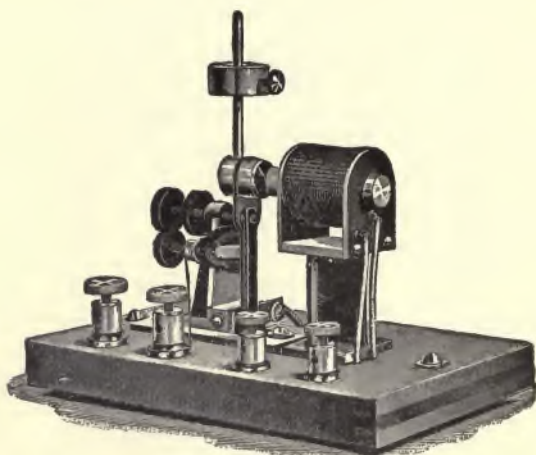
FIG. 107.—INDEPENDENT INTERRUPTOR.
