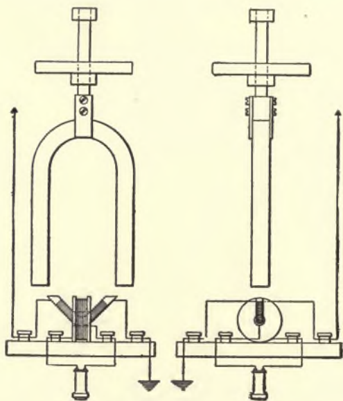
FIG. 152.—MARCONI MAGNETIC DETECTOR. (First Form.)
