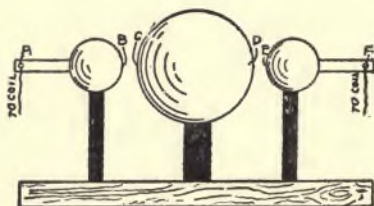
FIG. 56.—LODGE'S OSCILLATOR.
