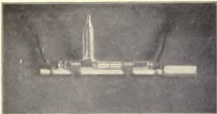
FIG. 141.—MARCONI COHERER.
