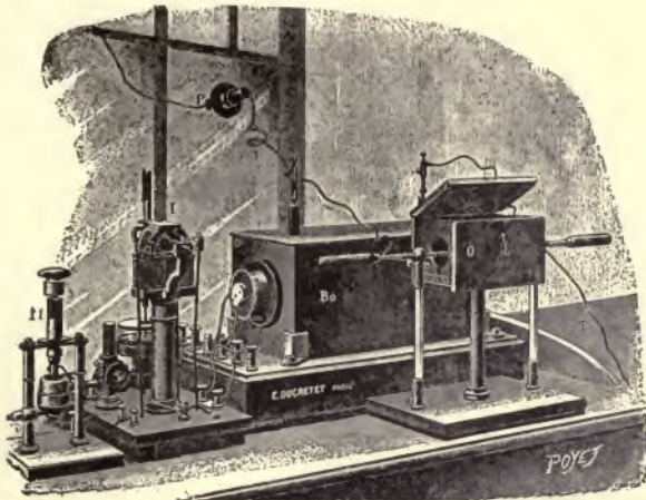
FIG. 179.—POPOFF-DUCRETET TRANSMITTER.
