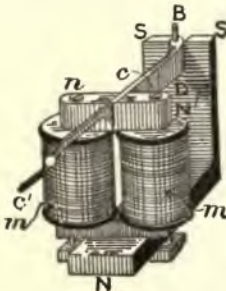
FIG. 240.—POLARIZED RELAY.
