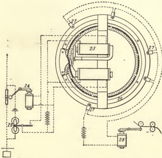
FIG. 307.—BULL SYNCHRONIZED SYSTEM. THE COLLECTOR.
