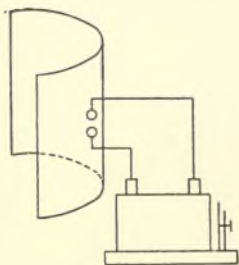
FIG. 162.—MARCONI TRANSMITTER. (First Form.)
