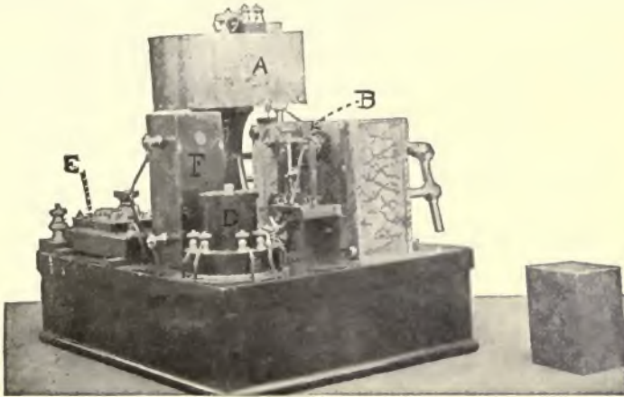
FIG. 216.—LODGE-MUIRHEAD RECEPTOR.
