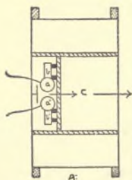
FIG. 26a. HERTZ OSCILLATOR AND RESONATOR.
