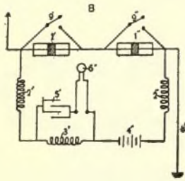
FIG. 208.—DEFOREST RECEPTOR.
