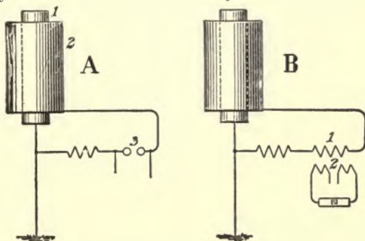
FIG. 296.—MARCONI SYNTONIC SYSTEM.
