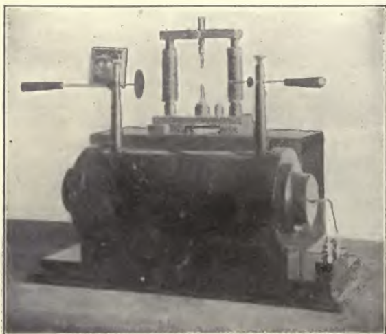
FIG. 99.—LODGE-MUIRHEAD COIL.
