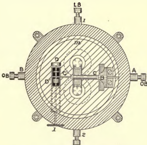
FIG. 241.—POLARIZED RELAY. (Top View.)
