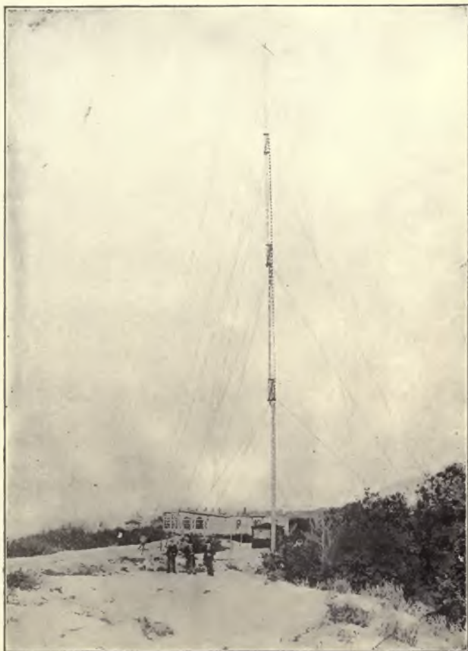
FIG. 267.—SLABY-ARCO AERIAL AND MAST.
