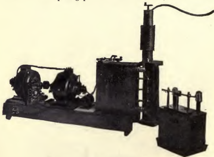
FIG. 181.—DE FOREST TRANSMITTER.
