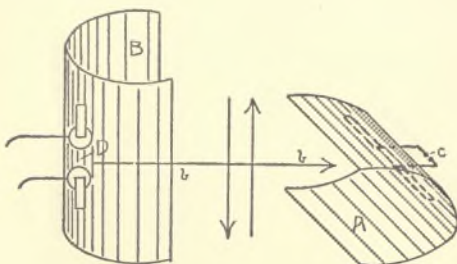
FIG. 31.—POLARIZING ELECTRIC WAVES.
