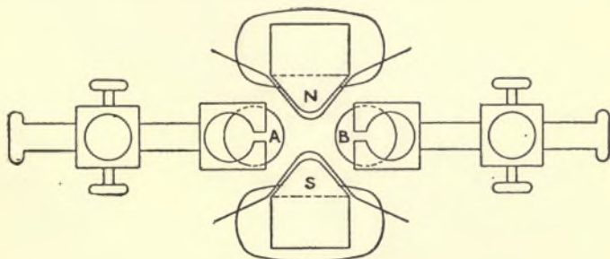
FIG. 221.—MAGNETIC BLOWOUT.
