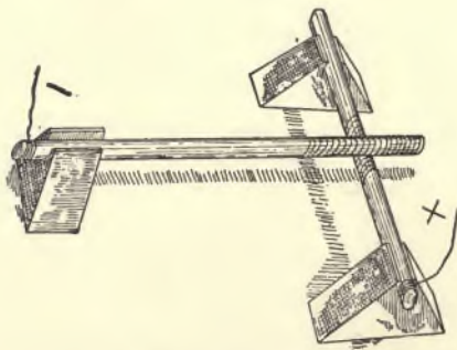
FIG. 134.—OXIDIZED RADIO-CONDUCTOR.
