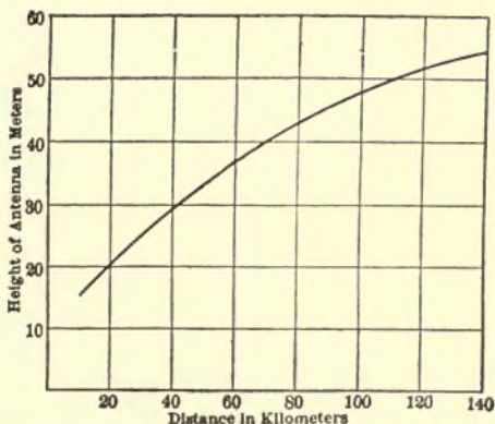
FIG. 251.—CURVE OF ELECTRIC WAVE RADIATION.
