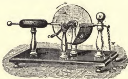
FIG. 125.—FRICTIONAL MACHINE.
