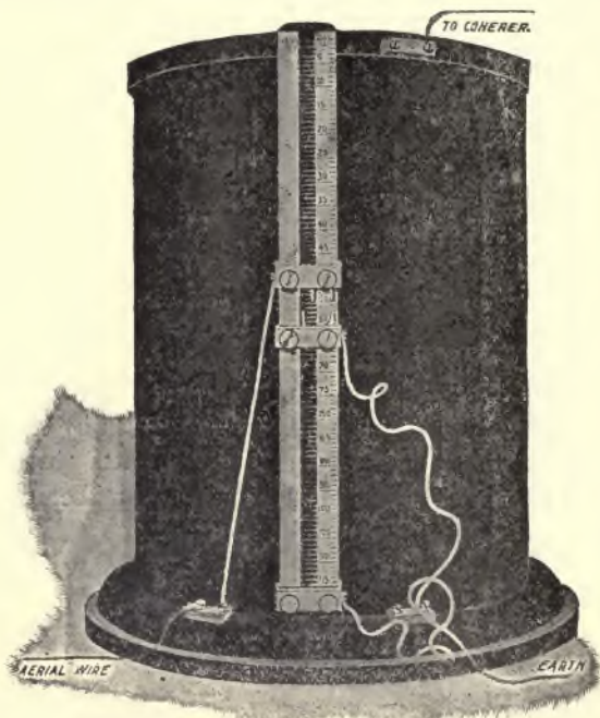
FIG. 248.—SLABY-ARCO TUNING COIL.
