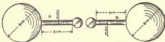
FIG. 60.—EXPERIMENTAL OSCILLATOR.
