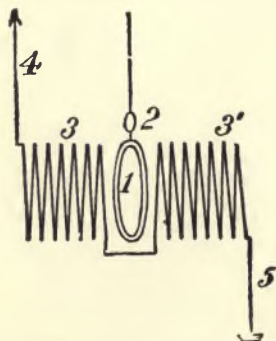
FIG. 150a.—FESSENDEN MAGNETIC DETECTOR. (Side Elevation.)
