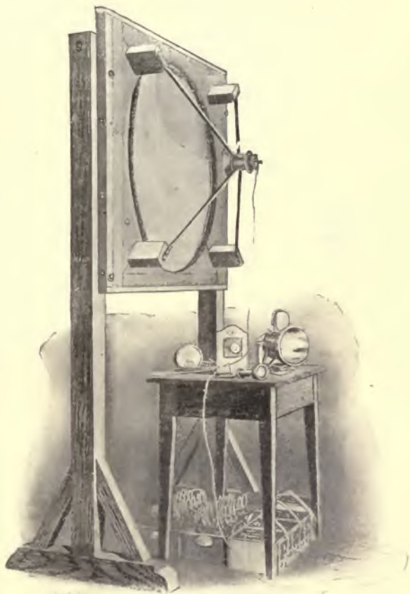
FIG. 315.—RUHMER PHOTO-ELECTRIC RECEIVER.
