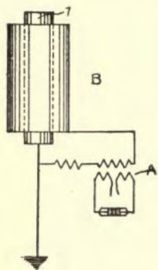
FIG. 200.—MARCONI RECEPTOR. (Third Form.)
