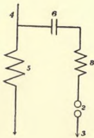
FIG. 169.—GRAPHIC REPRESENTATION OF SLABY-ARCO TRANSMITTER.
