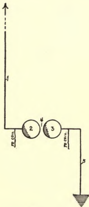
FIG. 61.—MARCONI RADIATOR.
