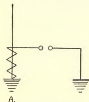
FIG. 260.—SLABY-ARCO DIRECT EARTHED AERIAL.
