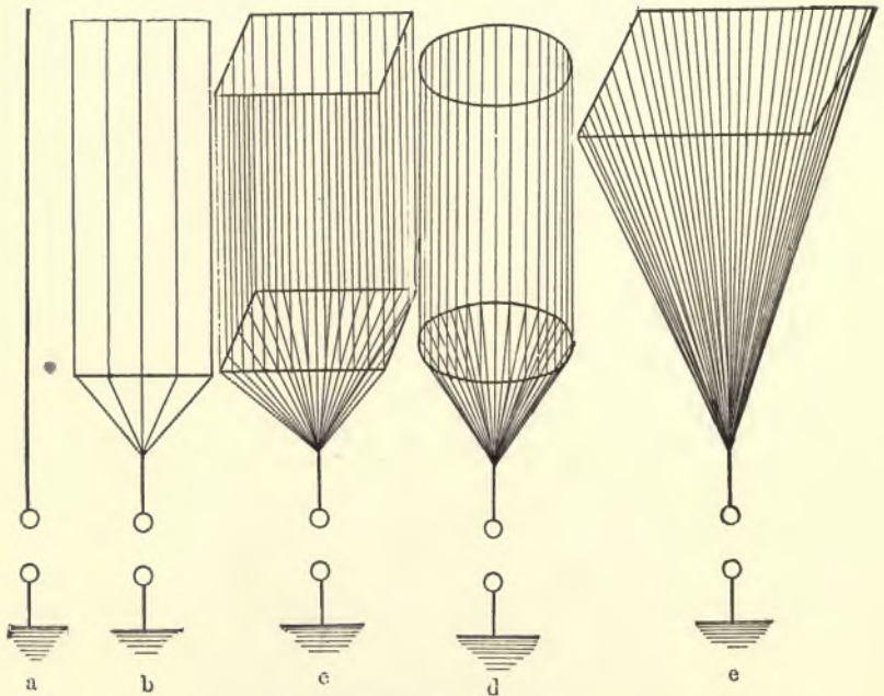
FIG. 255.—FORMS OF AERIALS.
