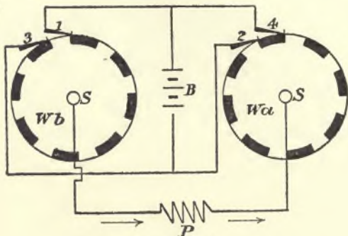
FIG. 118.—ROTARY INTERRUPTOR.
