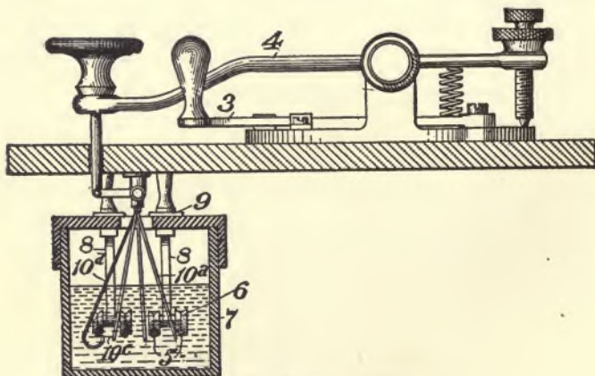
FIG. 223.—FESSENDEN KEY.
