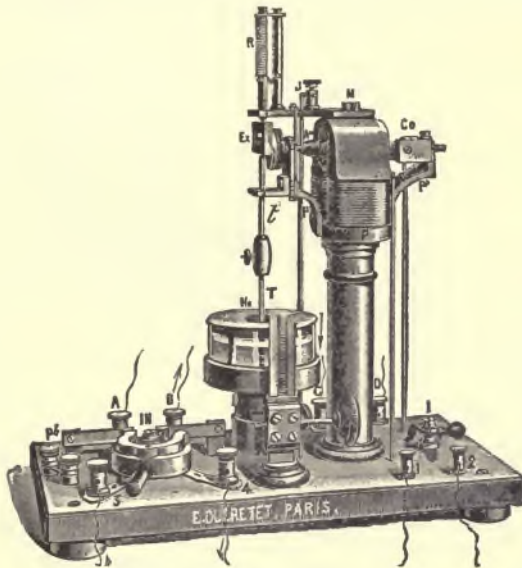
FIG. 111.—ROTATING INTERRUPTOR.
