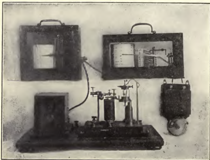
FIG. 213.—BRANLY-POPP METEOROLOGICAL APPARATUS.
