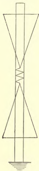
FIG. 256. LODGE CAPACITY AERIAL.
