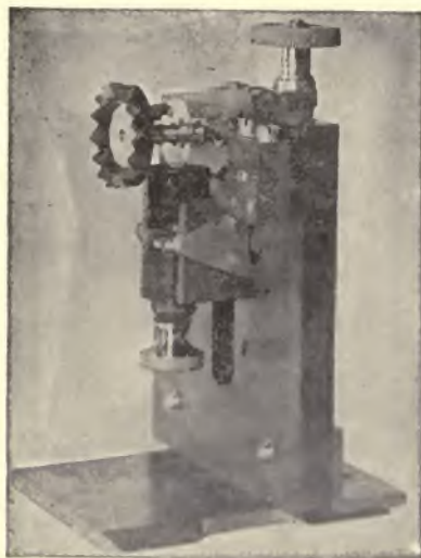
FIG. 154.—LODGE MERCURIAL COHERER.
