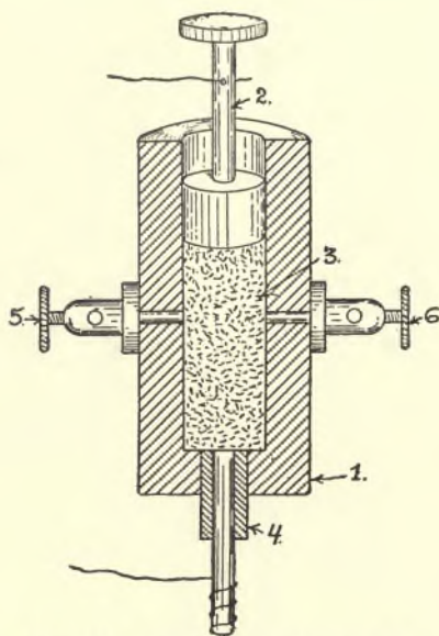
FIG. 133.—BRANLY RADIO-CONDUCTOR.
