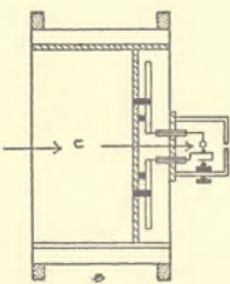
FIG. 26a. HERTZ OSCILLATOR AND RESONATOR.
