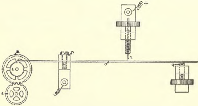
FIG. 137.—POINT AND DIAPHRAGM COHERER.
