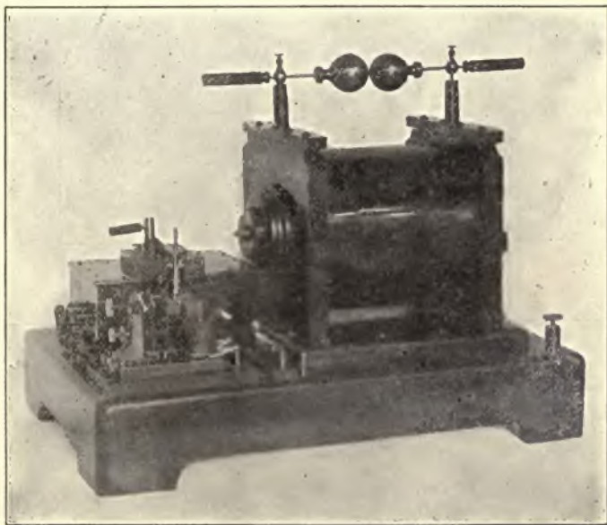
FIG. 98.—FOOTE-PIERSON DELTA COIL.
