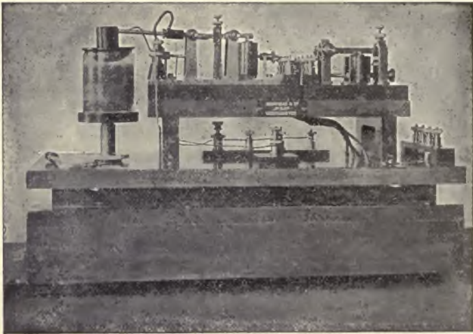
FIG. 227.—LODGE-MUIRHEAD BUZZER.
