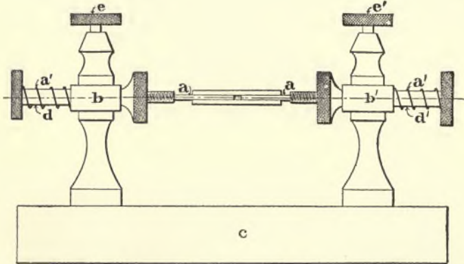
FIG. 143.—EXPERIMENTAL COHERER.
