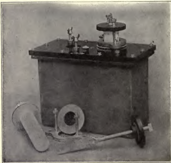
FIG. 116.—DOUBLE ELECTROLYTIC INTERRUPTOR.
