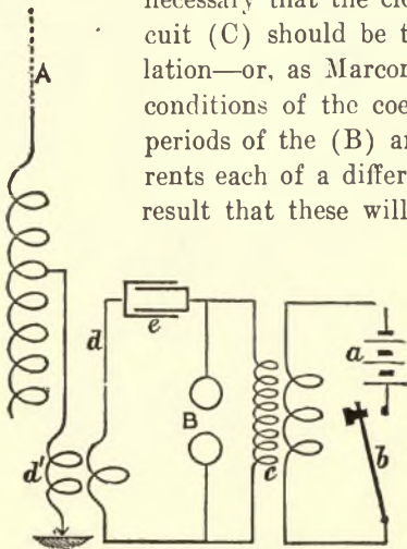
FIG. 178.—MARCONI TRANSMITTER. (Fourth Form.)
