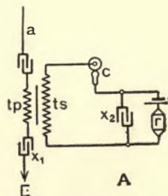
FIG. 215.—LODGE-MUIRHEAD RECEPTOR. (Second Form.)
