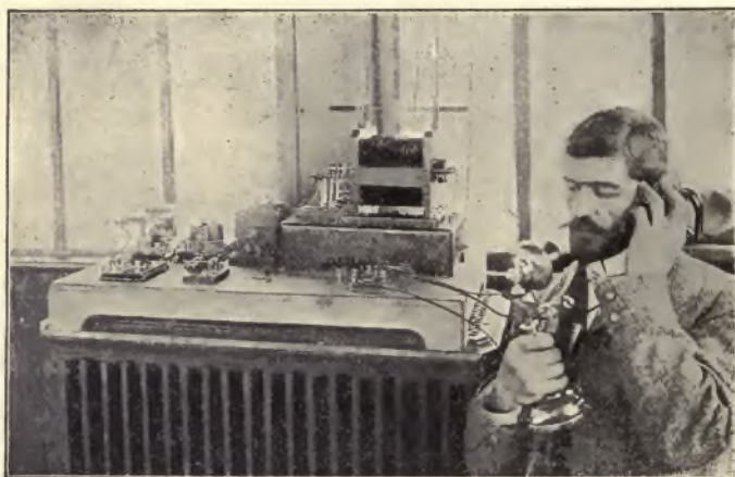
FIG. 332.—COLLINS WIRELESS TELEPHONE.
