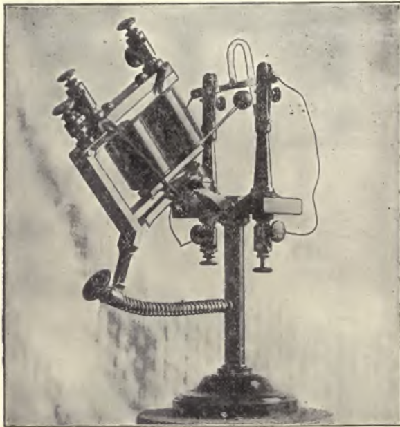
FIG. 237.—GUARINI DE-COHERER.
