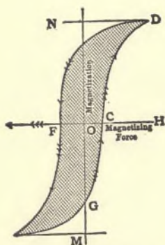
FIG. 83.—HYSTERESIS CURVE.
