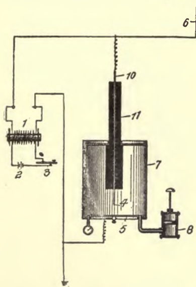
FIG. 44.—COMPRESSED AIR SPARK-GAP.
