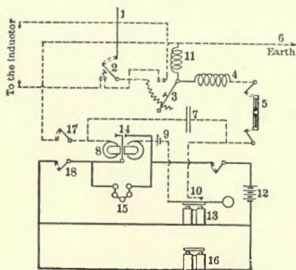
FIG. 196.—INTERNAL CIRCUITS.
