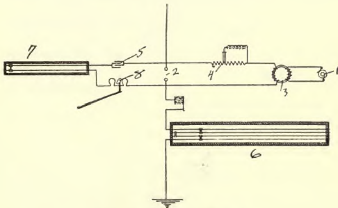
FIG. 182.—FESSENDEN TRANSMITTER.
