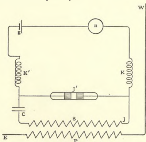
FIG. 234a.—MARCONI LOW-POTENTIAL TRANSFORMER.
