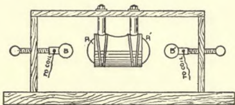
FIG. 55.—RIGHI'S OSCILLATOR.
