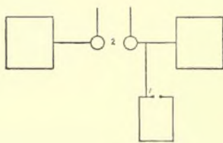
FIG. 21B.—OSCILLATOR WITH RESONATOR ATTACHED AT UNSYMMETRICAL POINT.
