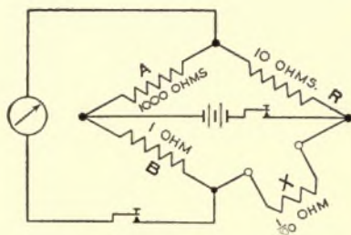
FIG. 75.—RESISTANCE MEASUREMENTS.
