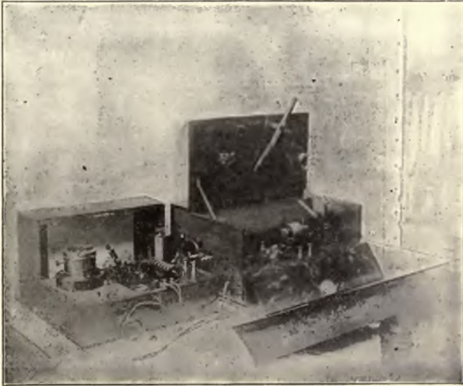
FIG. 206.—FESSENDEN PORTABLE EQUIPMENT.
