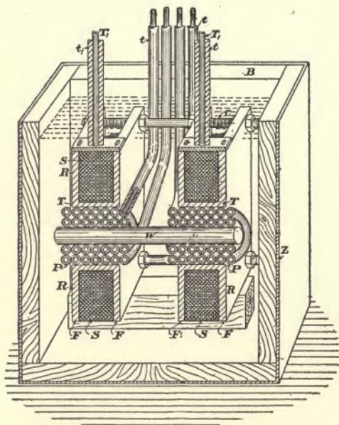
FIG. 128.—TESLA COIL.
