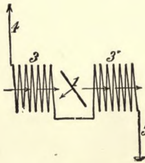
FIG. 150b.—FESSENDEN MAGNETIC DETECTOR. (Top Elevation.)
