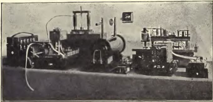
FIG. 188.—LODGE-MUIRHEAD SYSTEM.
