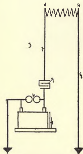
FIG. 166.—SLABY-ARCO TRANSMITTER. (First Form.)
