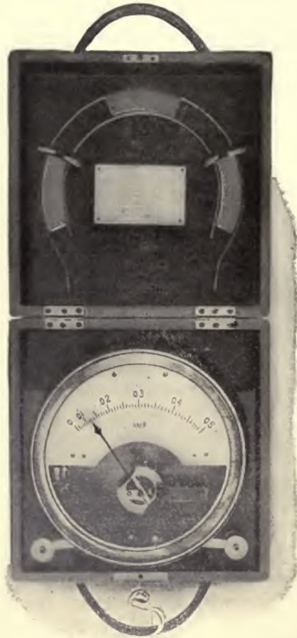
FIG. 290.—HOT-WIRE AMMETER.
