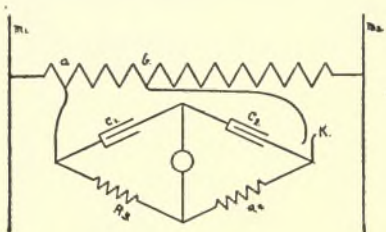
FIG. 70.—POTENTIOMETER METHOD.
