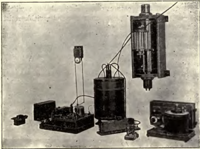
FIG. 170.—SLABY-ARCO SYSTEM.
