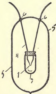
FIG. 158 — FESSENDEN HOT-WIRE BARRETTER.
