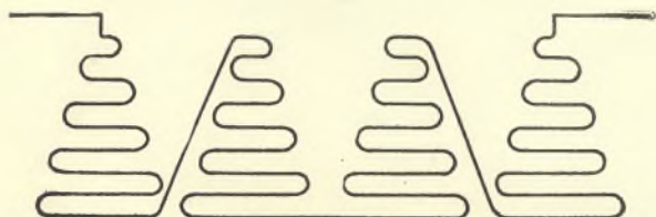
FIG. 234b.—MARCONI LOW-POTENTIAL TRANSFORMER. (Second Form.)
