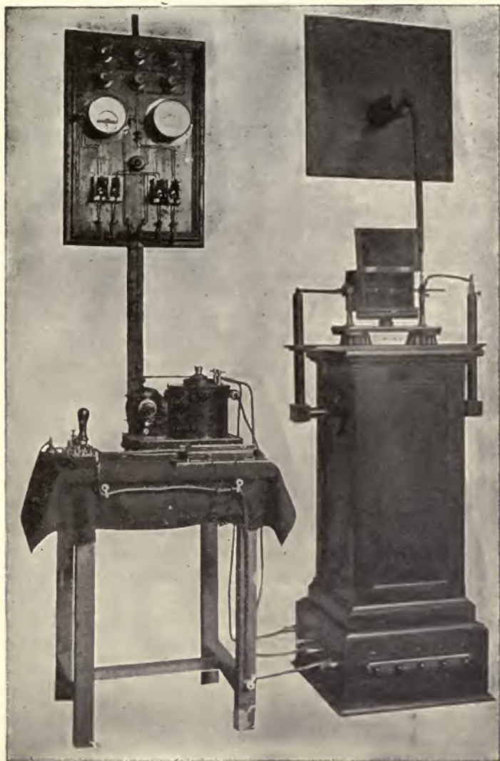
FIG. 184.—POPP-BRANLY TRANSMITTER.
