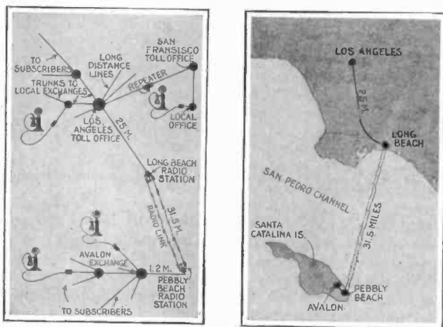
Map and diagram showing the radio link between the California mainland and Santa Catalina Island, and the wire systems at either end, all of which function as a single unit when connected together in this manner.
