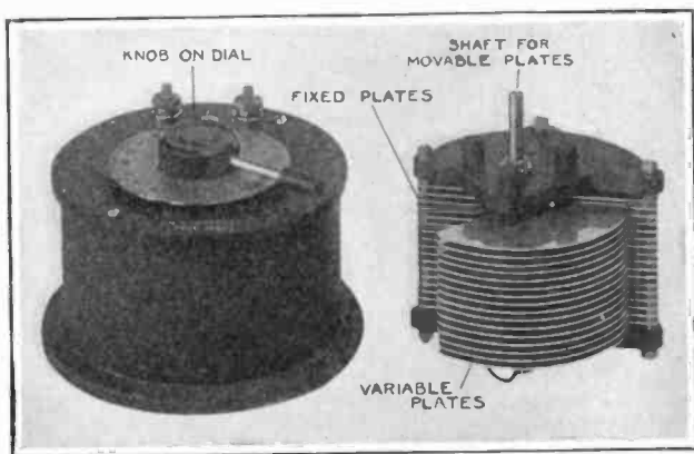
Outside and inside views of a variable condenser, showing its simple mechanism for varying capacity.
