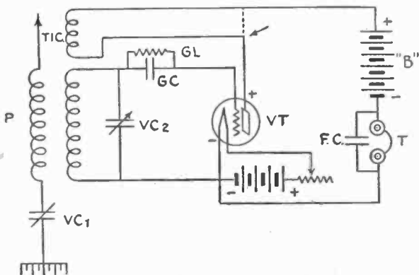
Regenerative set making use of tickler coil. P—primary of vario-coupler; TIC—tickler coil; VC1—variable condenser for varying antenna-ground wave length; VC2—variable condenser for varying secondary of vario-coupler; GL—grid leak; GC—grid condenser; VT—vacuum tube detector; B—high voltage or plate battery; FC—fixed condenser; T—'phones. The dotted line indicates how wiring would run for an ordinary, non-regenerative set.
