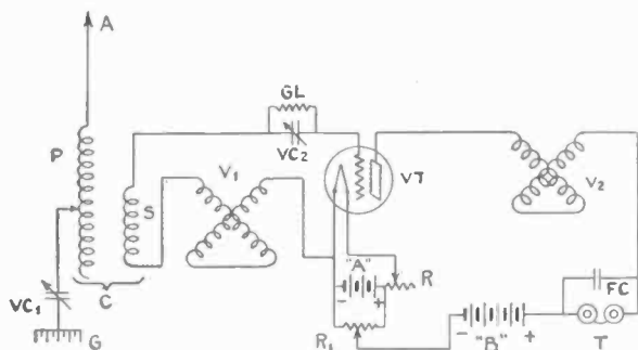
Another method of obtaining regenerative results. A—antenna; P—primary; S—secondary, of the vario-coupler C; VC1—variable condenser in antenna-ground circuit; V1—varlometer; GL—grid leak; VC2—variable condenser as grid condenser; VT—vacuum tube detector; V2—plate variometer for feed back; FC—fixed condenser; T—telephones; "B"—high voltage or plate battery; R—filament rheostat; R1—high voltage battery rheostat.
