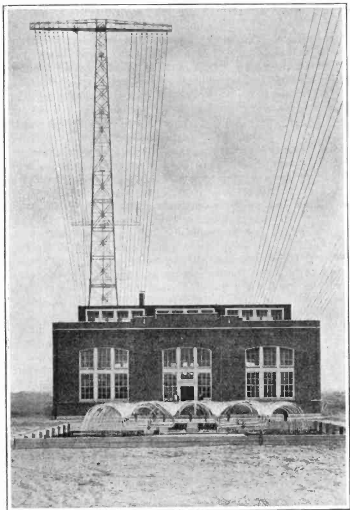
The power plant and station building of the Radio Central wireless station. In the foreground are the «sprays and cooling basin for cooling and condensing purposes, forming part of the power plant operation.
