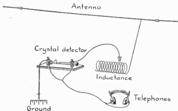
The essentials of receiving radio signals, comprising the antenna, inductance coil for tuning, crystal detector, telephones, and the ground.
