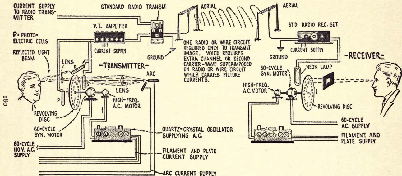
Fig. 68.—Showing how a quartz crystal oscillator is connected to a special high-frequency synchronous motor. Two oscillators tuned to the same frequency are used, one at the transmitter and one at the receiver. (Courtesy Experimenter Publishing Co.)
