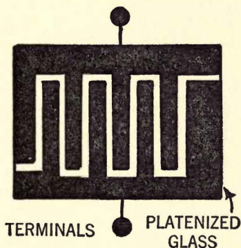
FIG. 52.—Wein selenium is constructed from a platinized piece of glass, the electrodes being formed by separation of the platinum surface into two parts. A thin film of selenium occupies the space between the two surfaces.
