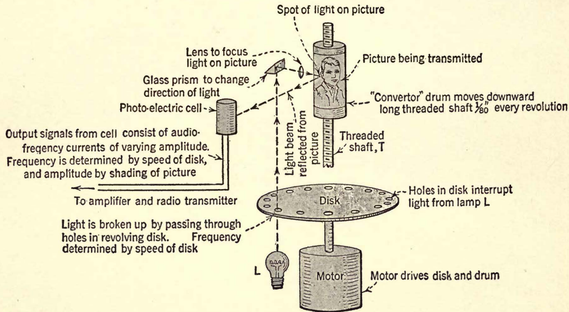
FIG. 8.—Principal parts of the Cooley Rayfoto transmitting system. The operation of this is more or less conventional, the picture which is wound upon a drum being explored by a beam of light which is reflected to a photo-electric cell. (Courtesy "Radio Broadcast.")
