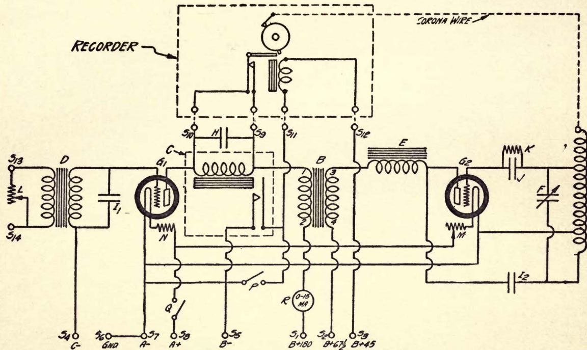
FIG. 10.—More conventional diagram of the connections used in the Cooley Rayfoto receiver. This apparatus is connected to the output of a standard broadcast receiver. This is really the printing apparatus which is controlled by the signal received from a broadcast outfit. The high-voltage discharges appears at the point of the needle which is shown resting upon the cylinder.
