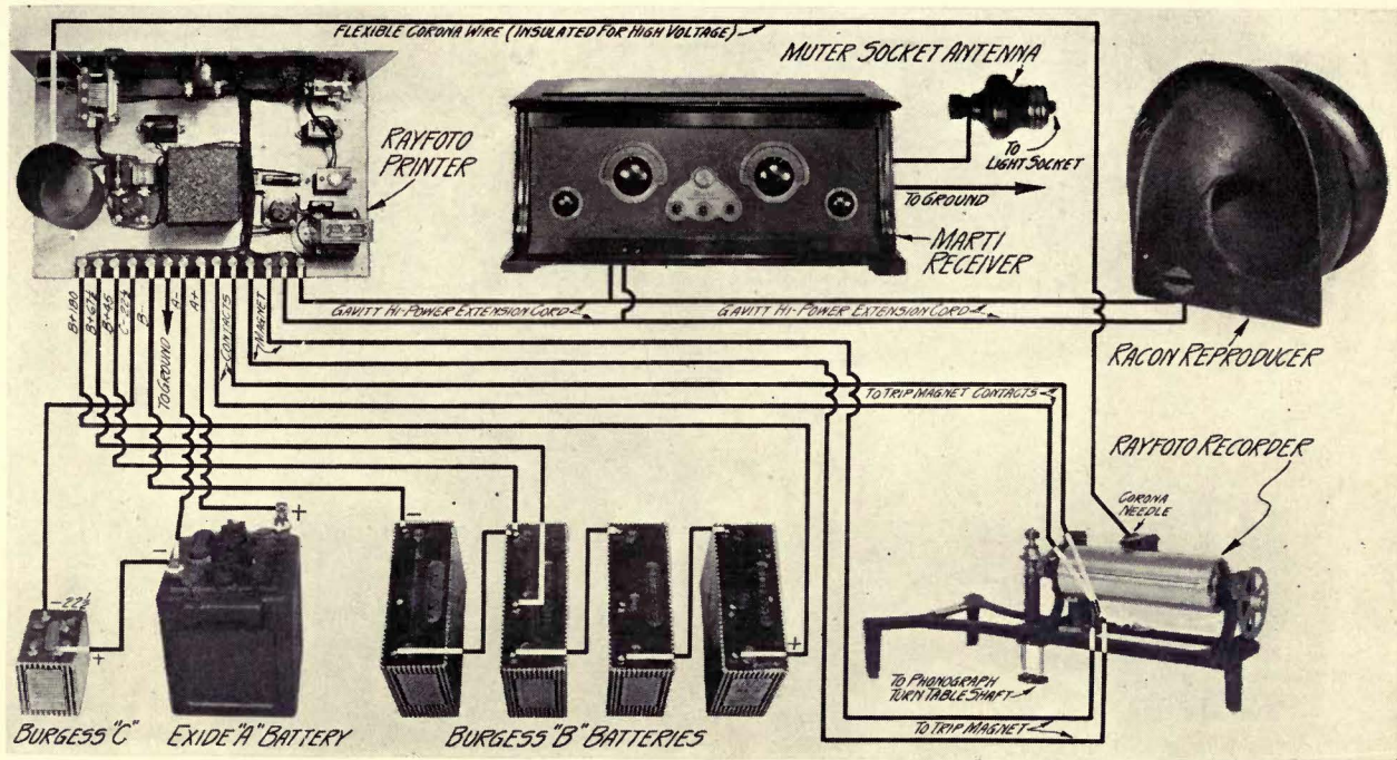
How the Cooley Rayfoto picture receiver is connected to an ordinary radio set for the reception of "still" pictures, either photographs or drawings.
