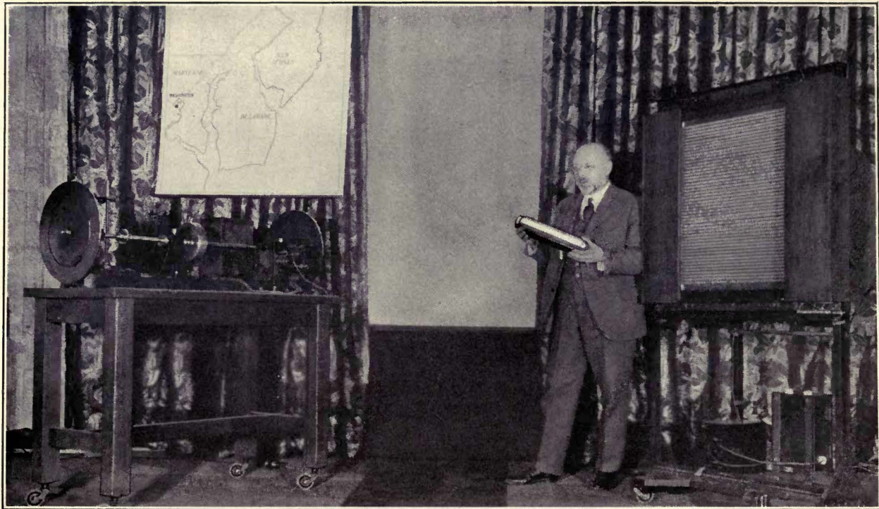
Dr. Herbert Ives of the Bell Telephone Laboratories beside the great neon lamp with its 2500 electrodes. The received picture appears upon this glass screen in the form of 2500 spots of light of varying intensity. Dr. Ives is holding one of the large photoelectric cells used at the transmitter. (Photo Courtesy Bell Telephone Laboratories, Inc.)
