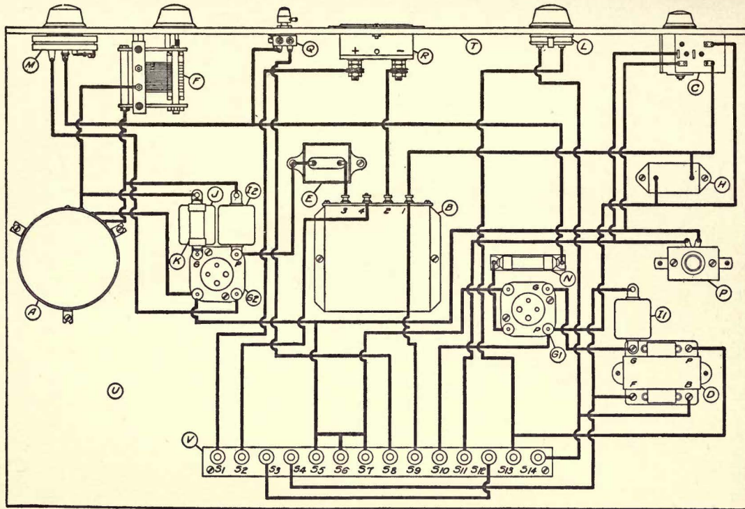
FIG. 9.—Layout and connection necessary for a receiver of the Cooley type. At A there is shown the "corona coil" which generates the high-voltage used in exposing the photo-sensitive paper wound upon the receiving cylinder.
