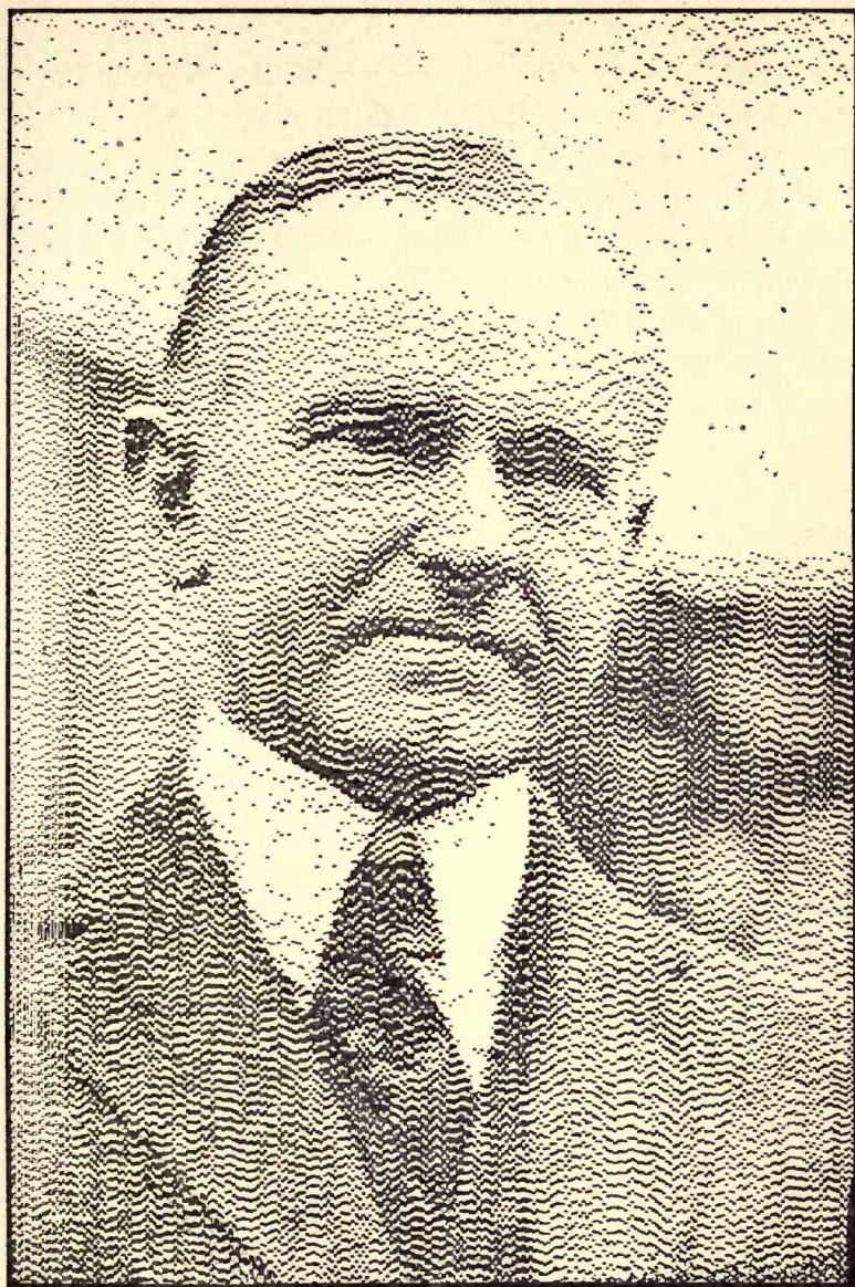
FIG. 4A.—Photograph of President Coolidge transmitted by the Ranger telephotographic apparatus. Although lacking in detail, the general effect is quite pleasing.
