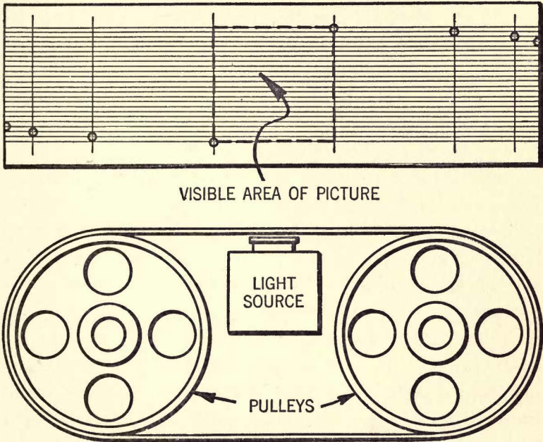
FIG. 55.—How scanning may be provided with a belt. The holes, in place of being drilled in spiral fashion, are simply drilled along the line of an angle.
