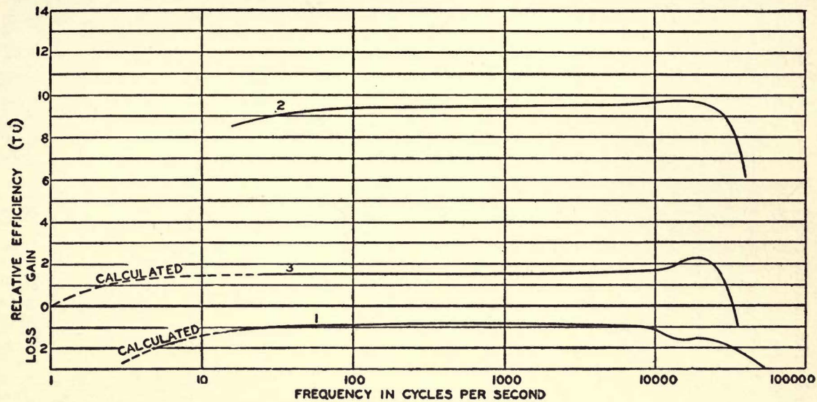
FIG. 36.—Curves showing transmitting characteristics of iron core audio-frequency transformers.
