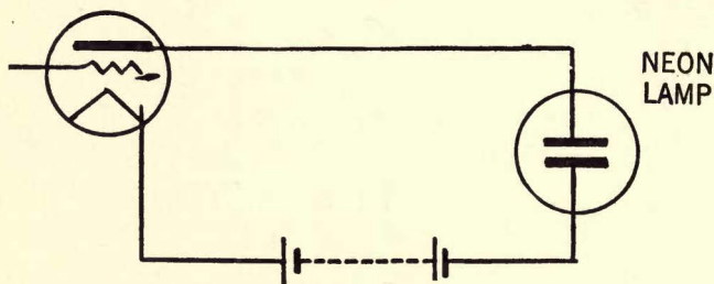
FIG. 43.—One way of connecting a neon lamp of a television receiver to the last or output tube of an amplifier. The plate voltage of the last tube should be larger than the striking voltage of the neon lamp.
