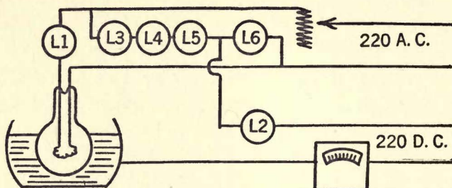
FIG. 25.—Another method of depositing sodium in the construction of photoelectric cells. The drawback of this system, as far as the amateur is concerned at least, is the necessity of having two sources of 220-volt current.
