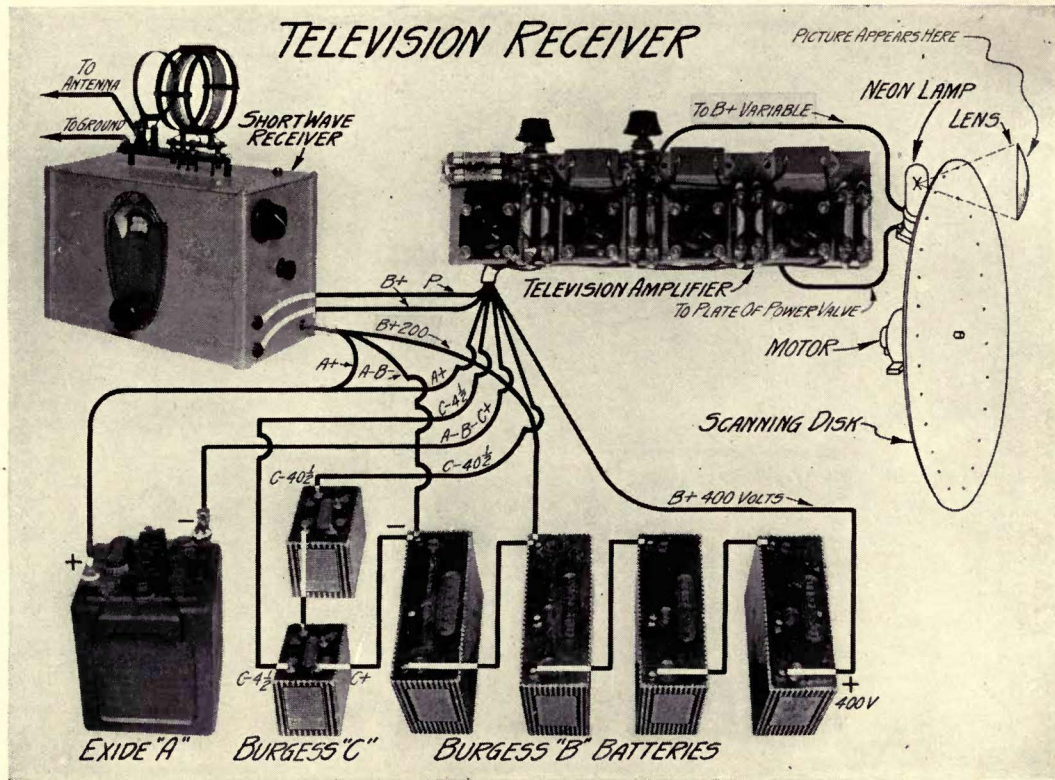
The diagram of connections showing how the short wave tuner, the resistance-coupled amplifier, and the neon tube are connected for the reception of television signals. The amplifier is the same as that described in the last of Chapter V.
