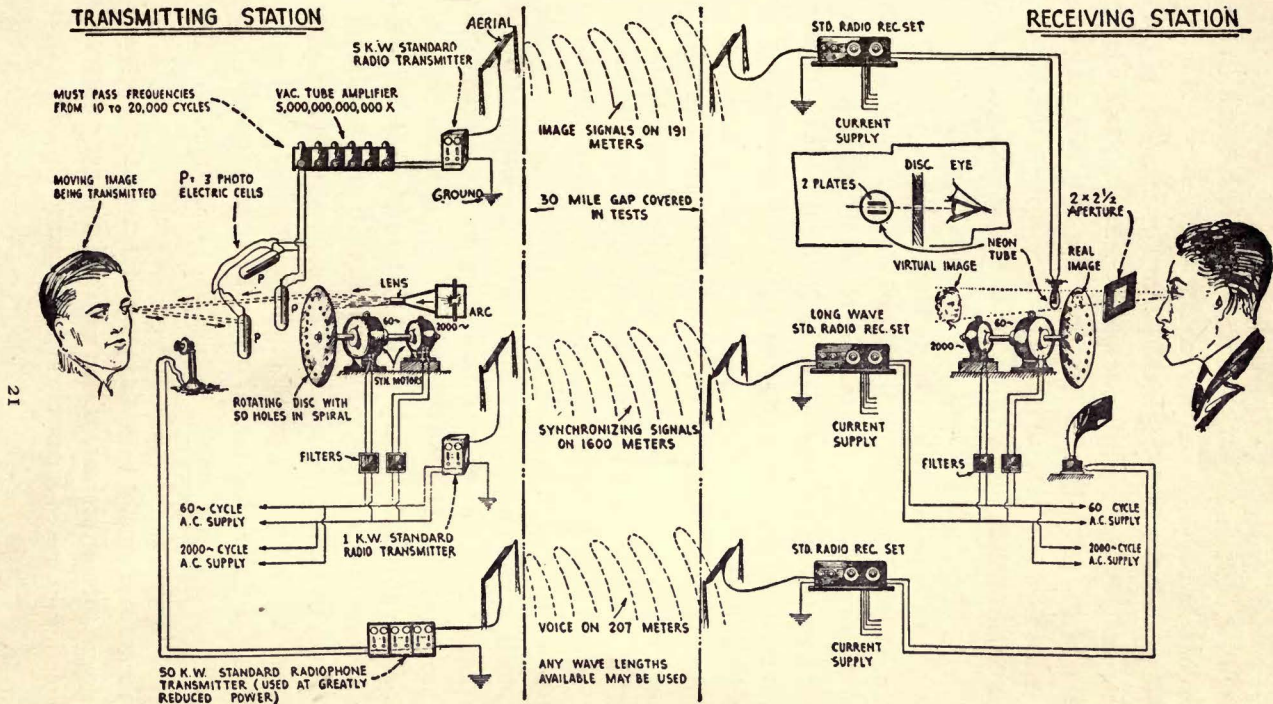
FIG. 1.—Simplified diagram of a complete television and telephonic broadcasting system. Three different wave-lengths are employed, one for the transmission of the picture of the living image, one for the voice or music, and one for the synchronism of the television scanning discs. (Courtesy Experimenter Publishing Company.)
