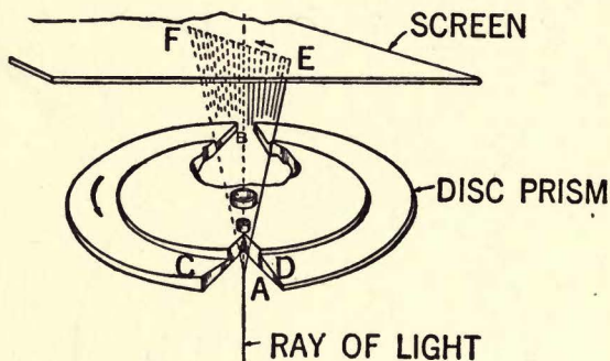
FIG. 59.—Revolving glass prism used for scanning in the Jenkins system of picture transmission. (Courtesy Q S T.)
