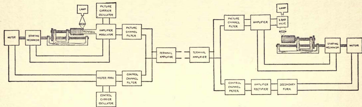
FIG. 15.—Complete layout of all accessory devices used in the Bell system of phototelegraphy. (Courtesy Bell Telephone Laboratories, Inc.)
