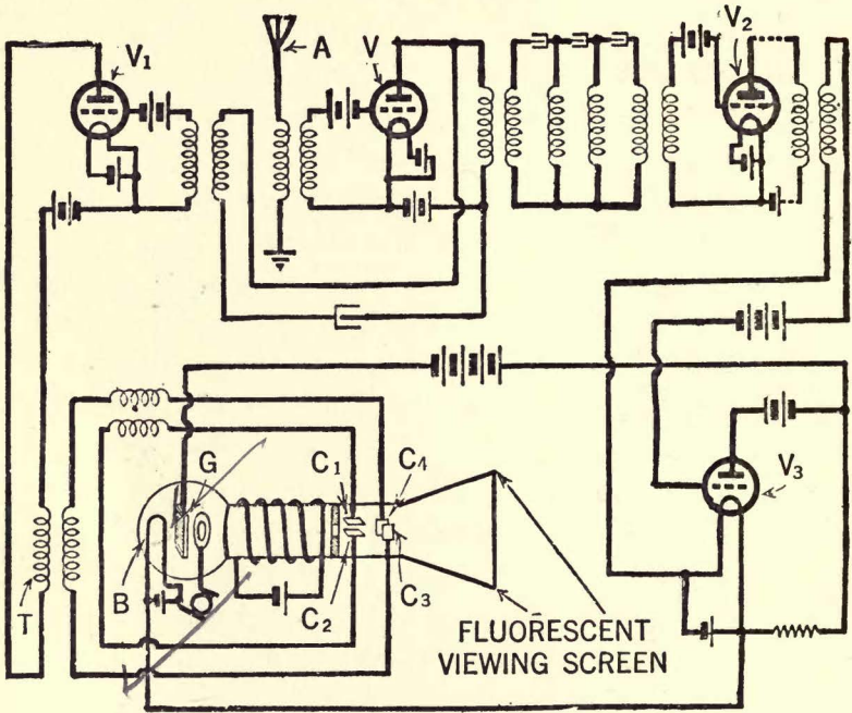
FIG. 4.—Diagram of a television receiver employing the cathode ray tube. The picture, which is formed by the controlling of a pure electron stream, appears on the fluorescent screen at the end of the cathode ray tube. A standard vacuum tube radio receiver is used to tune in the picture-laden waves.
