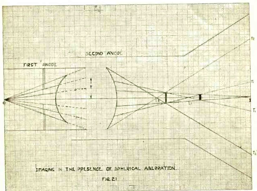
Fig. 21—Imaging in the Presence of Spherical Aberration.
