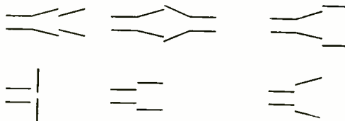
Fig. 3—Axial cross sections of focusing electrode combinations.
