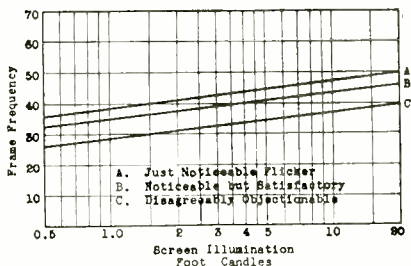
Fig. 5—Kinescope tests.
