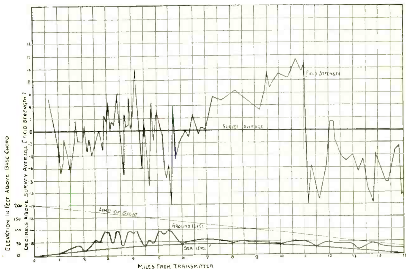
Fig. 12—Thirty-megacycle profile—Burlington Turnpike.
