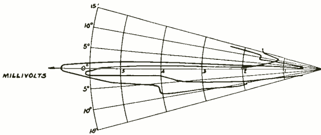
Fig. 3—Directivity of Arney's Mount transmitting antenna, plane flying at 700 feet altitude, 11.5 miles distant.
