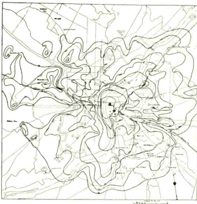
Fig. 5—One-hundred-megacycle contour map. Contours of equal field intensities in microvolts per meter.
