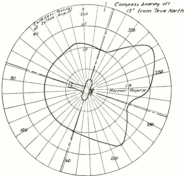
Fig. 1—Directive diagram of airplane antenna, 61 megacycles.
