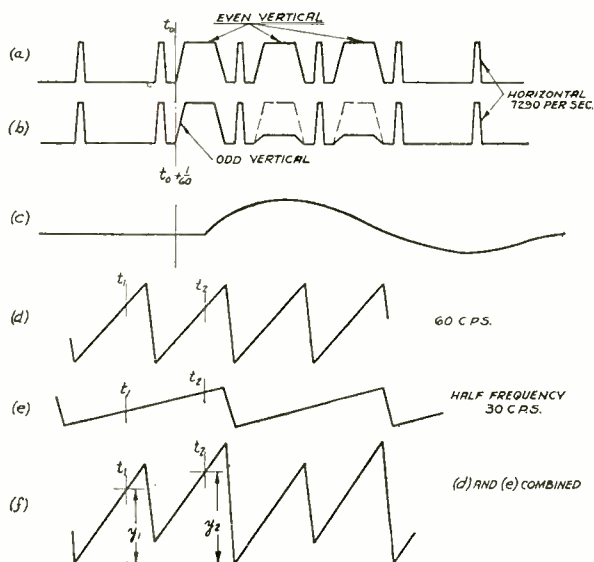
Fig. 12—Even-line interlacing.
