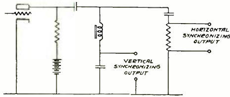
Fig. 11—Circuit for separation of vertical and horizontal synchronizing signals.
