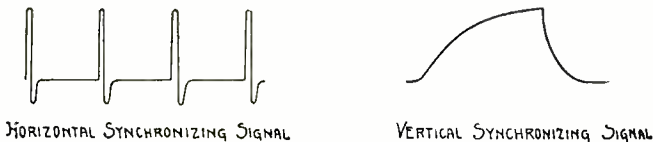
Fig. 13—Synchronizing signals after passing through separating circuit.
