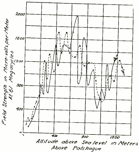
Fig. 12—Field strength vs. altitude at Patchogue, 85 kilometers from Empire State 61-megacycle transmitter. Radiation 1 kilowatt.
