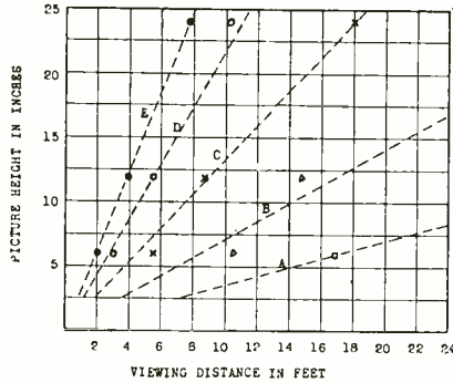
Fig. 11 A— 60 scanning lines B—120 scanning lines C—180 scanning lines D—240 scanning lines E—projection print
