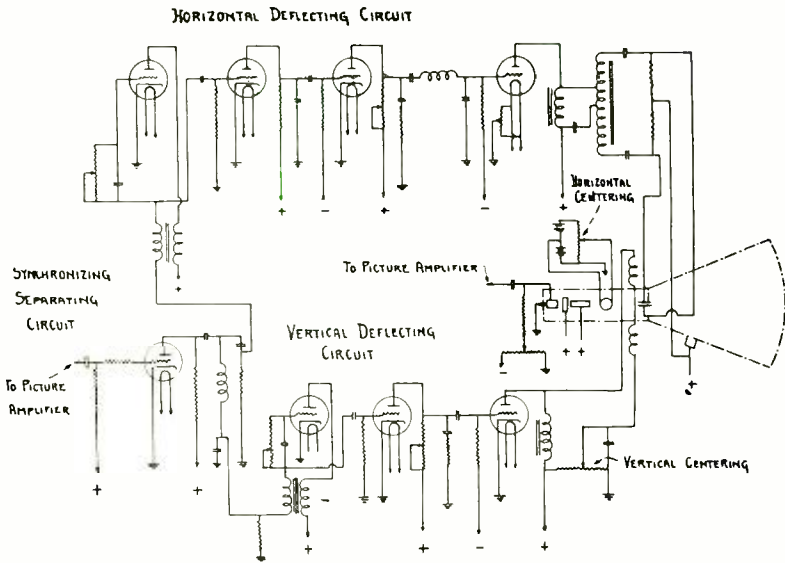
Fig. 21—Schematic arrangement of kinescope deflecting circuit.
