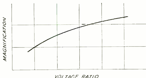
Fig. 21—Variation of optical magnification with voltage ratio keeping image distance constant.
