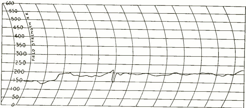
Fig. 21—Field strength at Twenty-fourth Street, 9 P.M., superior location.
