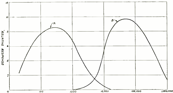
Fig. 12—Response characteristics of circuit shown in Fig. 11.
