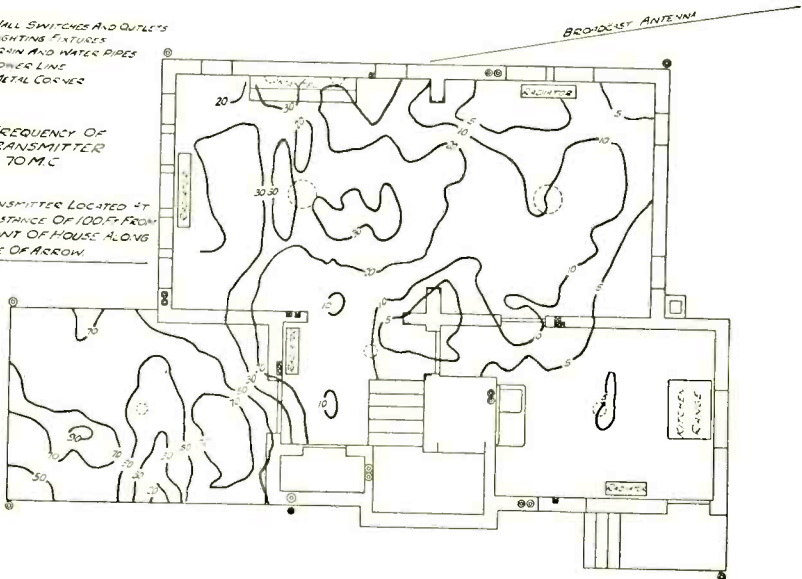
Fig. 17—Field strength within a residence, 70 megacycles.
