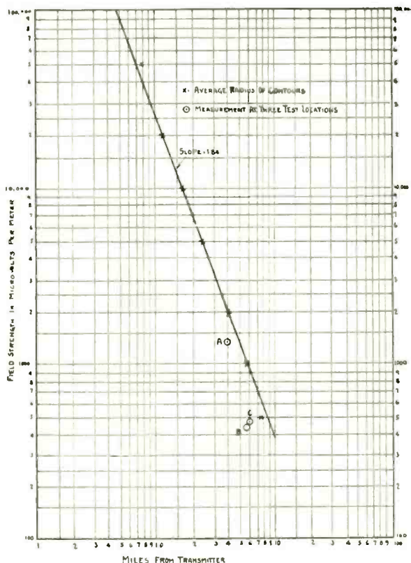
Fig. 6—Thirty-megacycle survey average.
