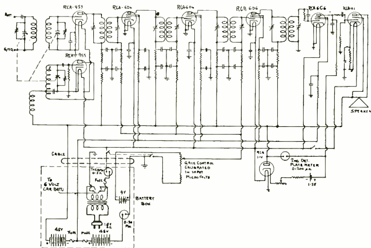
Fig. 3.—Circuit of field strength measuring receiver.
