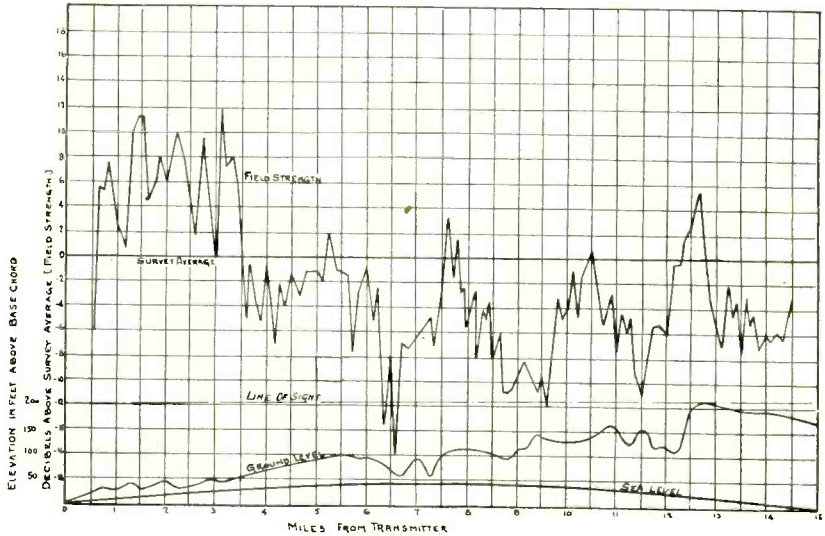
Fig. 10—Thirty-megacycle profile—Berlin Road.
