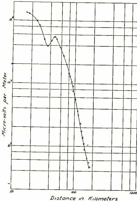
Fig. 8—Field strength vs. distance at 300 meters altitude—Empire State 44-megacycle transmitter. Radiation 2 kilowatts.
