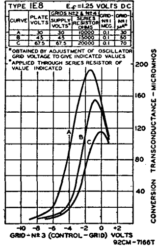
OPERATION CHARACTERISTICS WITH SEPARATE OSCILLATOR EXCITATION
