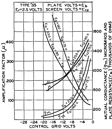
AVERAGE CHARACTERISTICS
