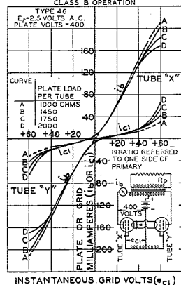
DYNAMIC TRANSFER CHARACTERISTICS CLASS B OPERATION
