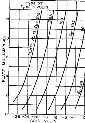
AVERAGE CHARACTERISTICS
