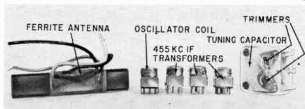
Fig. 339. A matched-coil kit consisting of if's, oscillator coil, antenna and tuning capacitor. Note the size of the units.
