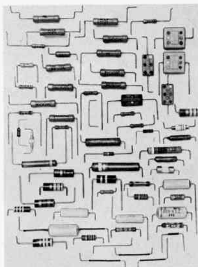
Fig. 389. Types of component lead shapes produced by pig-tailing. (Bruno-New York Industries)
