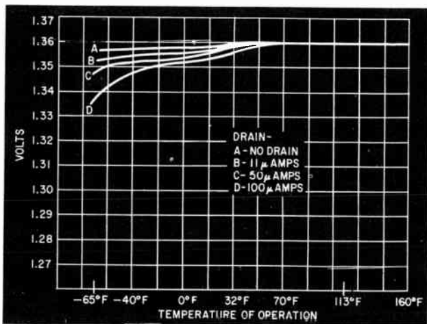
Fig. 404. Typical voltage-vs-temperature curve for a mercury cell.
