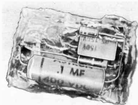
Fig. 654. Preliminary steps in potting a simple R-C circuit.
