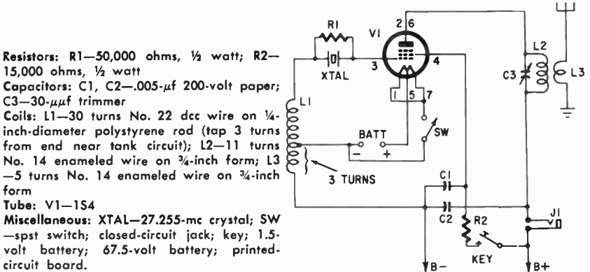
Fig. 638. The printed-circuit pattern and schematic of the transmitter shown in Fig. 637.
