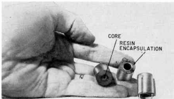
Fig. 336. The plug-in type if coils are extensively used in TV. These units are potted. (Courtesy Essex Electronics Co.)
