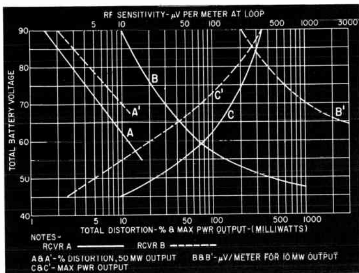
Fig. 412. Curves for B-battery rf performance. (Courtesy National Carbon Co.)
