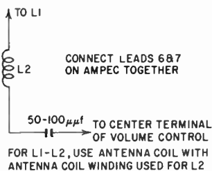
Fig. 624. A simple circuit which converts the receiver of Fig. 623 into a regenerative type.
