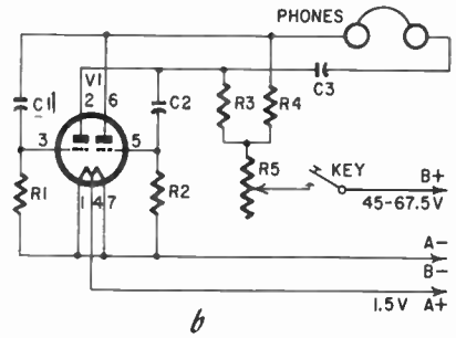
Fig. 634. Printed-circuit board and circuit diagram of a twin-triode oscillator. Pin 6 has a crossover on the opposite side of the board which goes to the phones. All component leads should be insulated with spaghetti. The ground lug on the tube socket is soldered to the A-bus for support. The key and batteries are external to the board.
