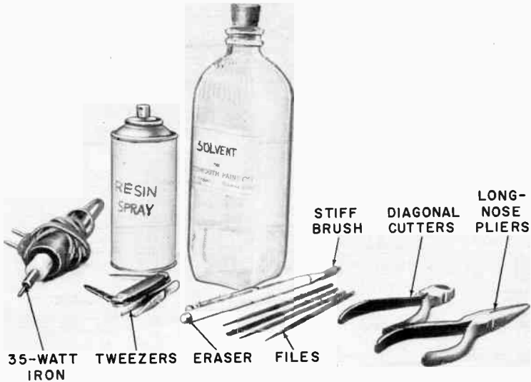
Fig. 504. Some typical tools used in printed-circuit repair.
