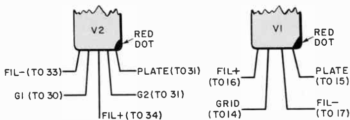
Fig. 720. Printed-circuit board arrangement (a) for the Little Gem duo-diode receiver.
