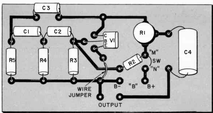
Fig. 631. A phase-shift audio oscillator which uses printed-circuit techniques.
