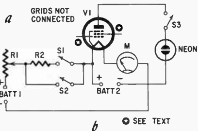
Fig. 526. Layout of the printed-circuit board and circuit diagram for a subminiature tube tester.
