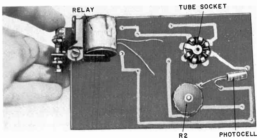
Fig. 616. A light-beam relay which uses a 15-watt lamp for filament dropping and as a light source.
