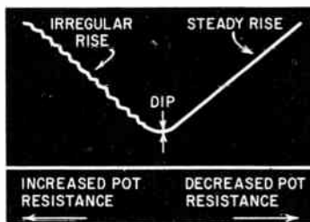
Fig. 723 (continued). Circuit of the Gazistor receiver. The graph represents the plate current of the RK-61 for different settings of the potentiometer.
