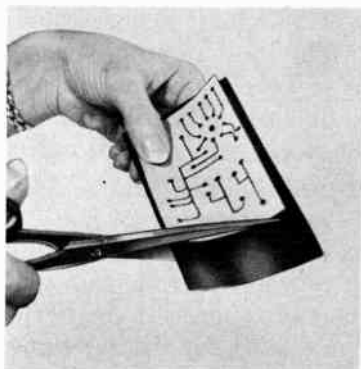
Fig. 215. The first step in the preparation of a silk-screen pattern is to cut a piece of presensitized gelatin film, slightly larger than the pattern to be reproduced.
