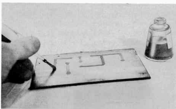
Fig. 221. Fingernail polish can be used as a resist.
