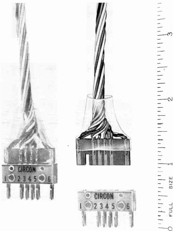
Fig. 358. Some of the special multiple circuit connectors used in miniature work. (Courtesy Circon Component Co.)
