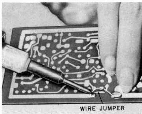
Fig. 512. Using a wire jumper to repair a broken printed-circuit conductor.
