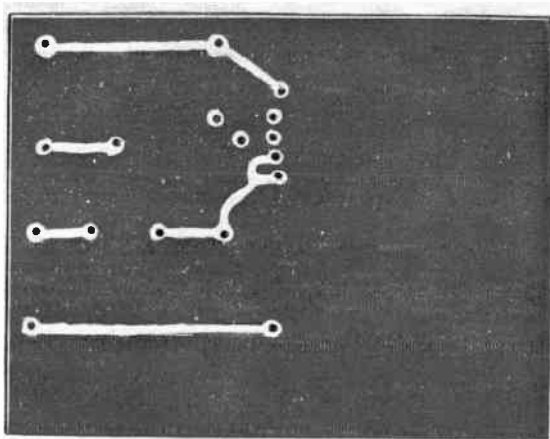
Fig. 635. Printed-circuit board for a Pierce crystal oscillator.
