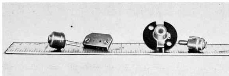
Fig. 370. Extremely small jacks and plugs are needed for compact circuitry.
