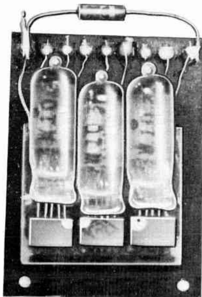
Fig. 620. By connecting a suitable resistor across the input circuit, the Ampec can be used as the heart of a hearing aid.
