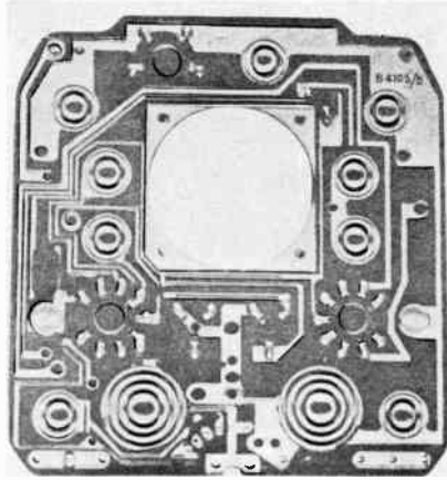
Fig. 101. Circuit plate used in an early British two-tube ac-dc receiver. (Courtesy Sargrove Electronics, Ltd.)
