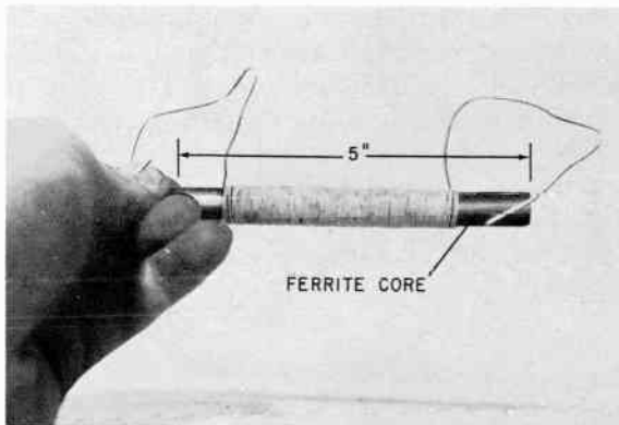
Fig. 337. One type of ferrite-loop antenna used in miniature circuitry.
