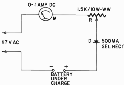
Fig. 414. Setup for rejuvenating dry cells. The table supplies the charging rate and time for various types of cells.
