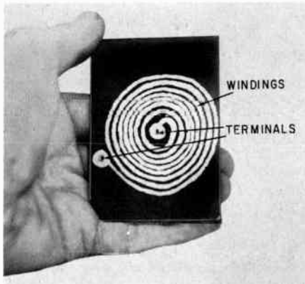
Fig. 342. Example of a flat-spiral inductor.
