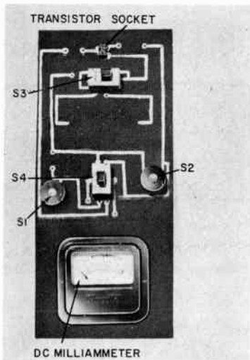
Fig. 528. Photo of the transistor checker. The arrangement shown here follows the circuit diagram fairly closely.
