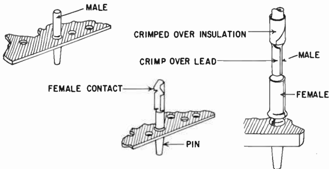
Fig. 708. Tubular pin connectors are used for making snap-on connections.
