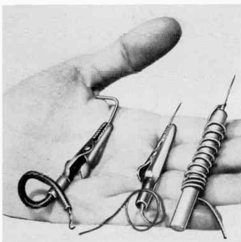
Fig. 506. An assortment of 'home-made test prods.
