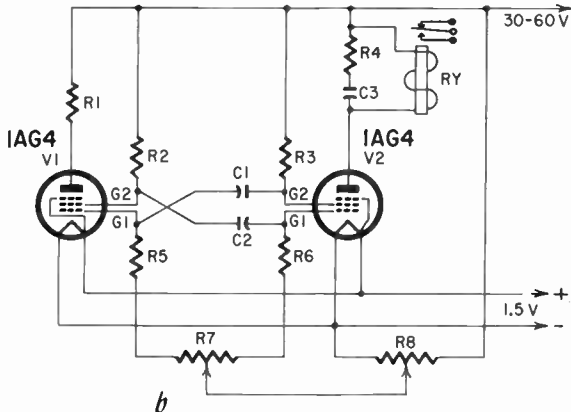
Fig. 717. The upper illustration (a) is a drawing of the printed-circuit board for the subminiature multivibrator. The circuit (b) is shown below. Conductors run from 11 to B+ on the underside of the board, and also from 12 to 13. Crossovers are made by through-soldering with a piece of No. 20 tinned hookup wire. A- also has a conductor on the opposite side from 5 to 10. A+ runs on the opposite side from 3 to 14. Also, through-solder at points 5, 8, 10 and 14.
