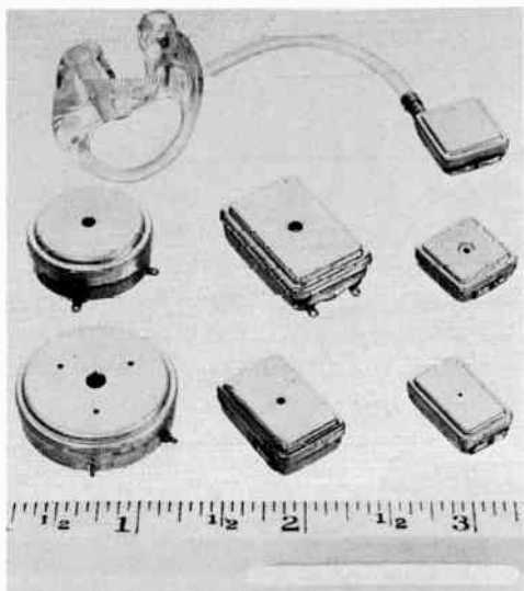
Fig. 372. A variety of "flat" earphones made primarily for hearing aids. (Courtesy Knowles Electronics.)
