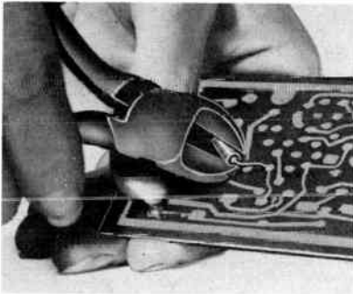
Fig. 507. Replacing a capacitor on a printed-circuit board.
