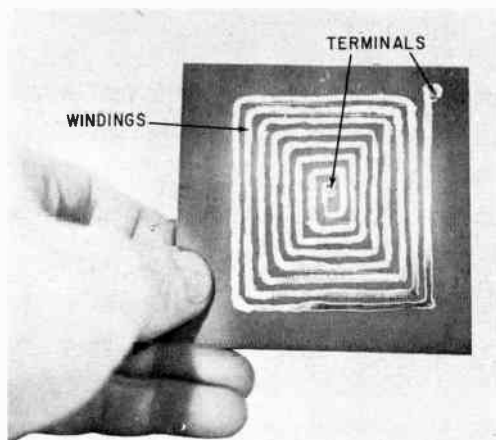
Fig. 344. The flat square is another form of inductor.
