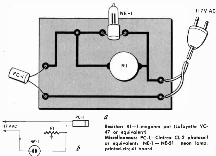
Fig. 615. The printed-circuit pattern and schematic of the light meter shown in Fig. 614.
