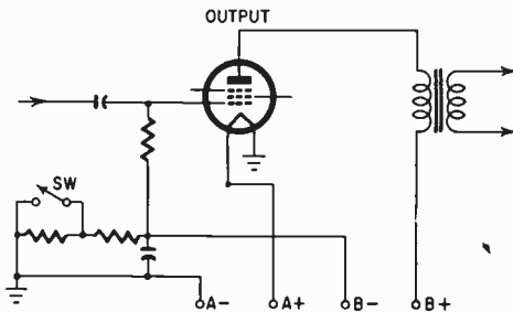
Fig. 413. Economizer circuit used to prolong B-battery life.
