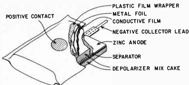
Fig. 401. A reversed-construction dry cell. (Courtesy National Carbon Co.)
