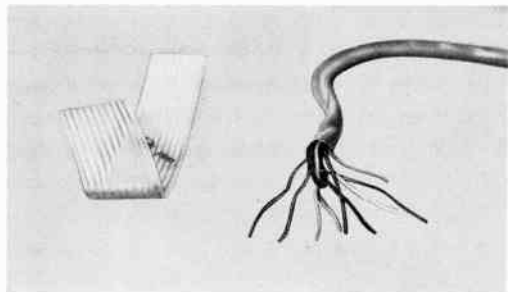
Fig. 227. Conventional multiconductor cable and cable made with printed-circuit techniques.
