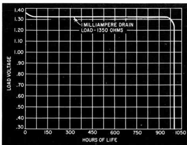
Fig. 405. Typical voltage-us-time curve of a mercury cell.
