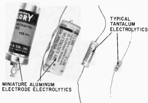
Fig. 320. Quite a departure from the familiar electrolytic, the miniature capacitors shown are about the size of ordinary tubular capacitors.
