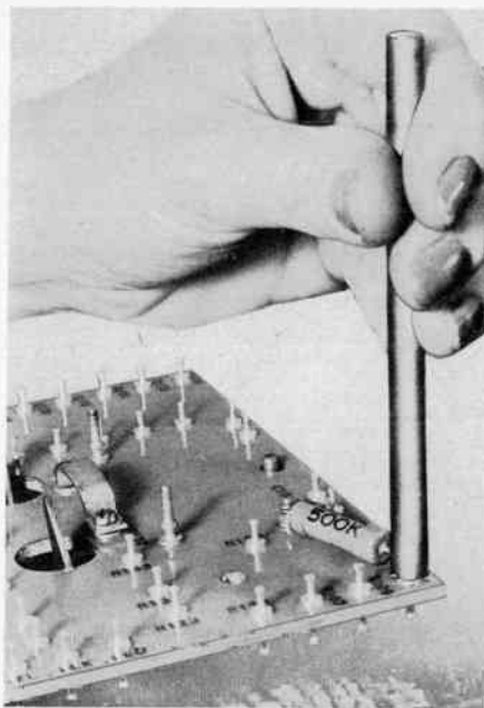
Fig. 388. A spinpin is used for wrapping component leads around turret-type terminals. (Bruno-New York Industries)
