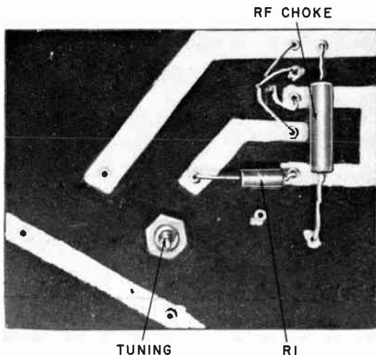
Fig. 603. Underchassis view of a one-tube thyratron receiver.
