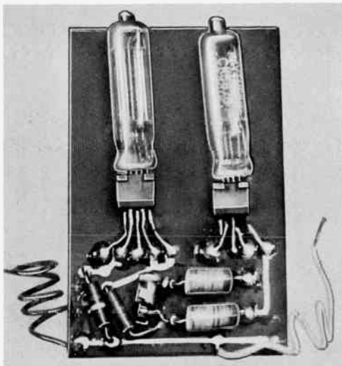
Fig. 711. Inside view of the wristwatch transmitter.
