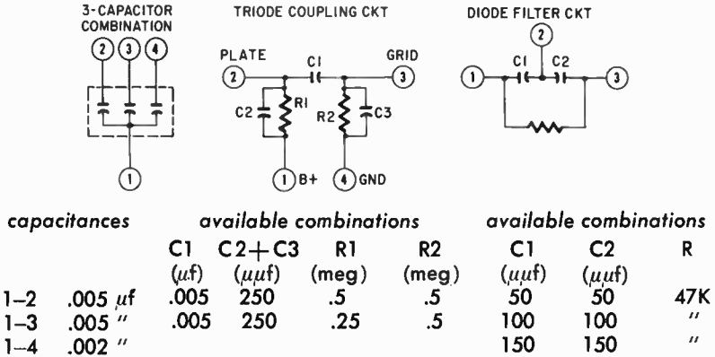
Fig. 384. "Packaged circuit" schematics are available in various combinations. (Courtesy Sprague Electric Co.)
