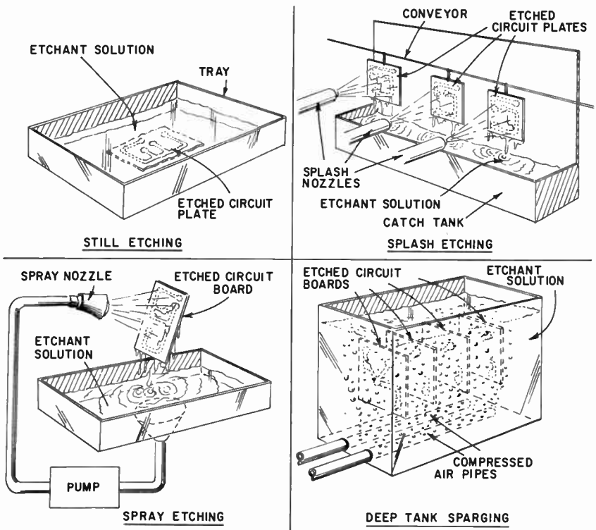
Fig. 213. A variety of etching techniques are used to prepare printed-circuit boards.
