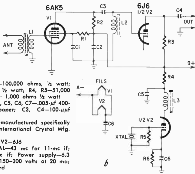
Fig. 709. The upper illustration (a) shows the printed-circuit board for the crystal-controlled converter. The drawing shows the approximate positioning of the parts. The circuit for the converter (b) is shown below.
