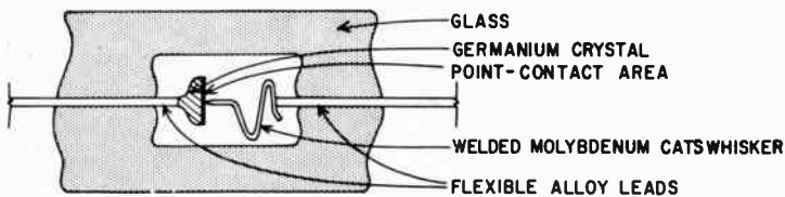
Fig. 376. Internal construction of a germanium diode. (Hughes Electronics)
