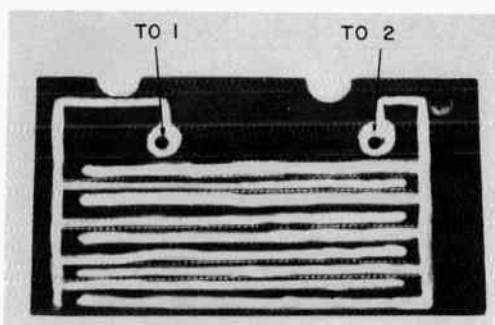
Fig. 608. This printed-circuit maze is used as the sensing element of a rain detector.
