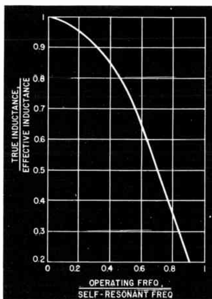
Fig. 347. Chart shows the relationship between inductance and frequency. (Chilton Publishing Co.)
