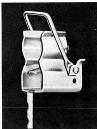
Fig. 365. The locking type component holder gives a positive grip. The large surface area of the holder helps heat dissipation. (Atlas E-E Corp.)
