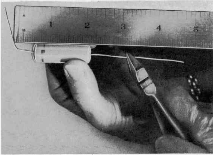
Fig. 385. Preparation of component leads for use in printed circuitry.
