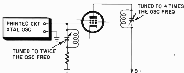
Fig. 704. The circuit following the crystal oscillator can be a frequency multiplier.
