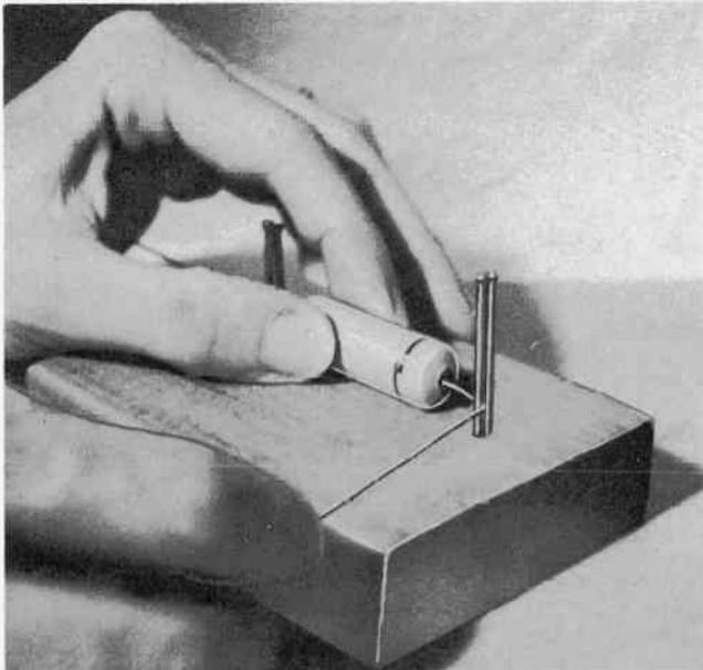
Fig. 386. Some nails and a board make a convenient jig for shaping component leads.
