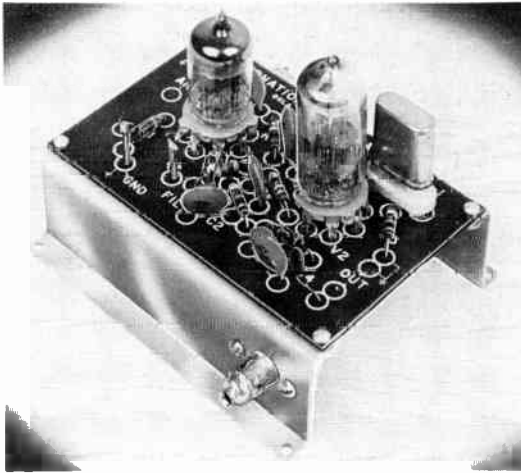
Fig. 707. Two-tube crystal-controlled converter.
