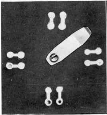
Fig. 642. In this switch the rotary member is independent of the controlled circuits.
