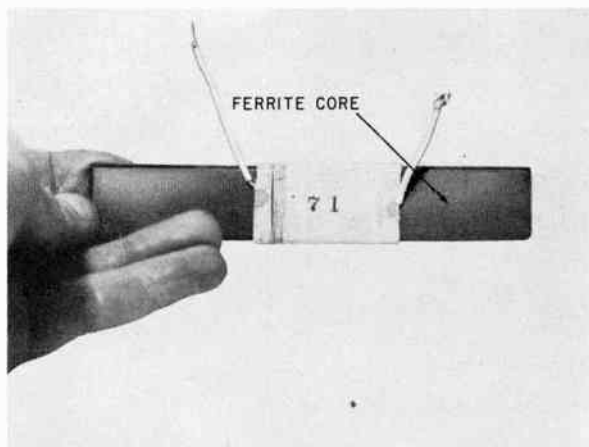
Fig. 338. Flat ferrite rods are also used in loop antenna designs.
