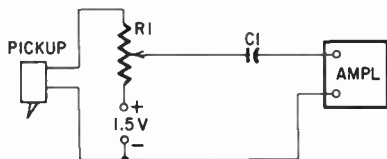
Fig. 640. Circuit of the printed-circuit phono pickup.
