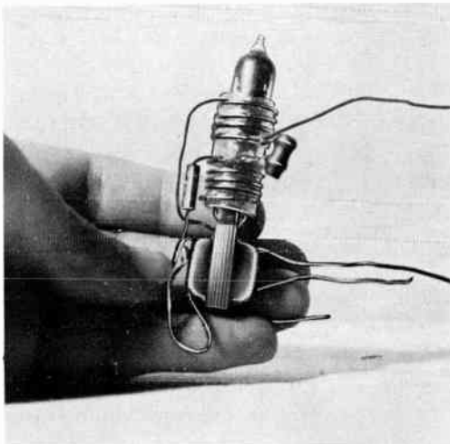
Fig. 713. Single-tube transmitter in which the tube acts as a form for the oscillator coil.
