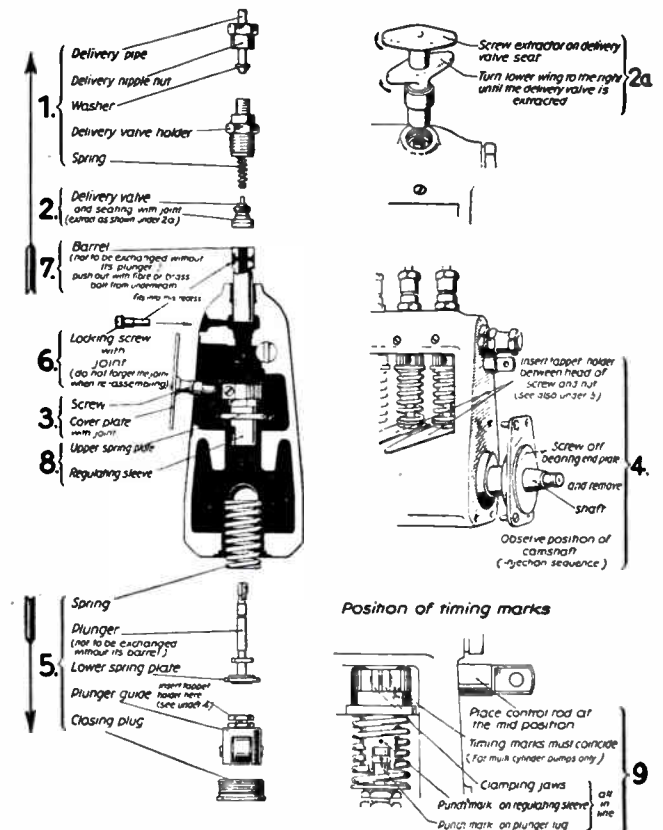
Fig. 39. This figure shows the proper steps in dis-assembling a Bosch fuel injection pump for cleaning and repairs. Carefully note the instructions printed at the various steps. (Courtesy United American Bosch Corp.)
