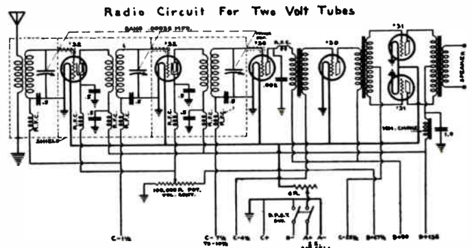
Fig. 138. A modern 6 tube battery operated set designed for use with an air cell "A" battery.
