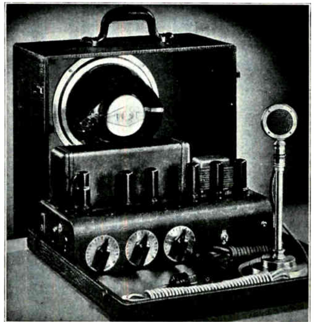
Fig. 228. Compact portable public address unit showing amplifier, speaker, microphone and connecting cables all neatly arranged in a convenient carrying case. Courtesy Montgomery-Ward.
