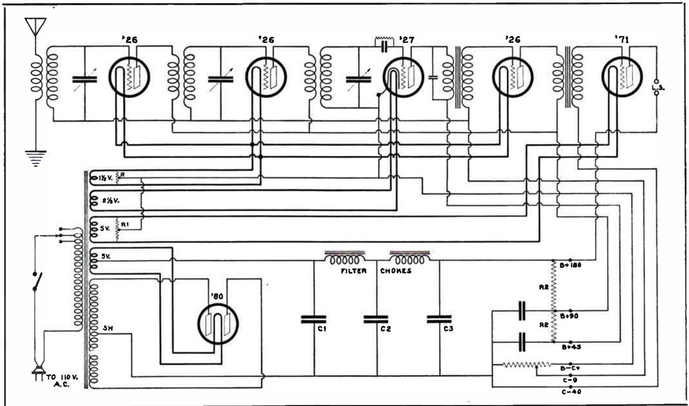
Fig. 142. Complete circuit diagram of a simple five tube A. C. receiver and its "power pack" or power supply unit.
