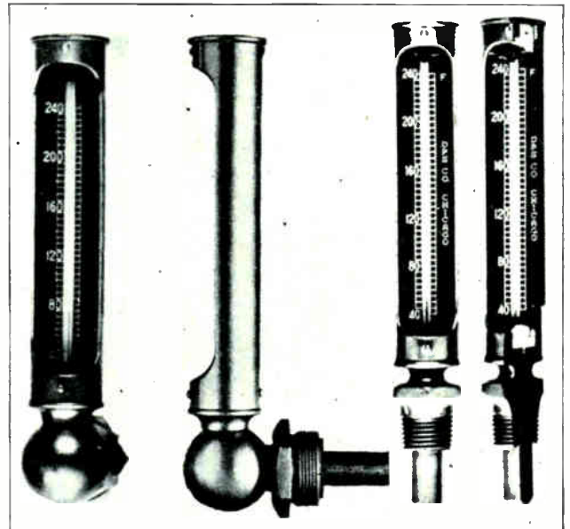
Fig. 117. Several types of mercury column thermometers used to indicate the temperature of Diesel engine cooling water. (Courtesy Diesel Specialties Corp.)
