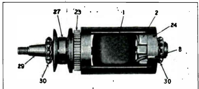
Fig. 49. Magneto armature removed from housing to show bearings, slip ring, armature core, windings, and condenser.
