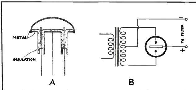
Fig. 92. On the left is shown a sketch of the anode and cathodes of a full-wave gaseous rectifier tube. On the right is shown a connection diagram for a tube of this type as used in the power supply of A. C. receivers.
