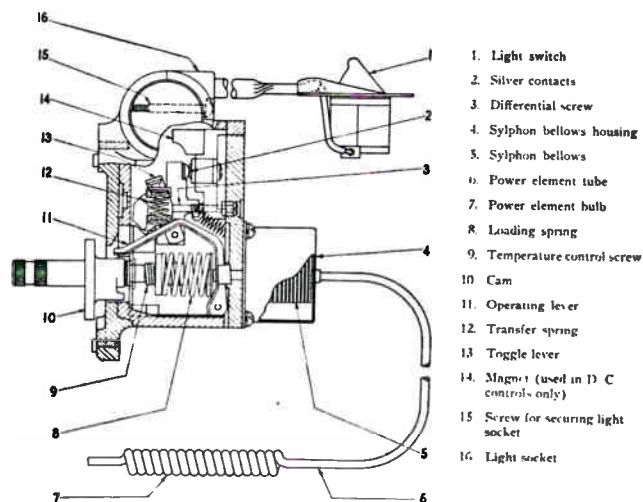
Fig. 104. Sectional view of a refrigerator control switch showing the contacts, springs, pressure bellows and power bulb. Examine each of these parts carefully while studying the instruction on control switch repairs. Courtesy Stewart-Warner Corporation.
