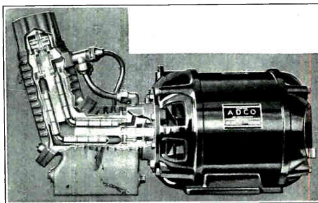
Fig. 44. Sectional view of a unique combination rotary and reciprocating compressor used in one type of refrigerator and air-conditioning unit. As the rotary blocks revolve in the angular chambers the small pistons are caused to move back and forth in the cylinders, thus obtaining compression action. Courtesy Air-Conditioning Devices Corp.
