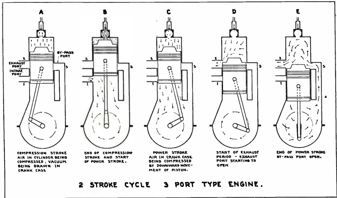
Fig. 18. The diagram on the right illustrates the operation of a two-stroke cycle Diesel engine. Note carefully the operation of the cylinder ports and the admission of air and fuel, and also the power and exhaust strokes.
