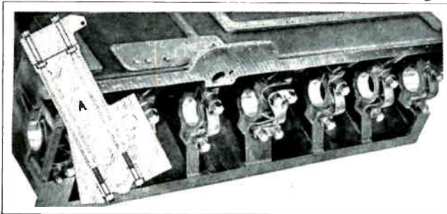
Fig. 142. Photograph showing the arrangement of the bearings in a six cylinder Diesel engine. Note the bottom ends of the through bolts which are shown full length in the insert at "A." These bolts run clear through from the crank shaft bearings to the cylinder head.
