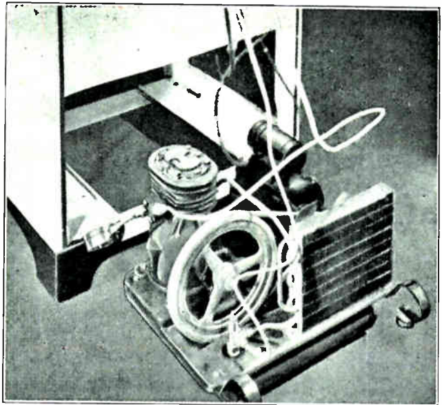
Fig. 97. Here the condensing unit is shown completely removed from the cabinet and in convenient position for adjustment and servicing. On some refrigerators, the tubing is not long enough to permit removal of the condensing unit without pumping down the system and disconnecting the tubing. Courtesy Stewart-Warner Corporation.
