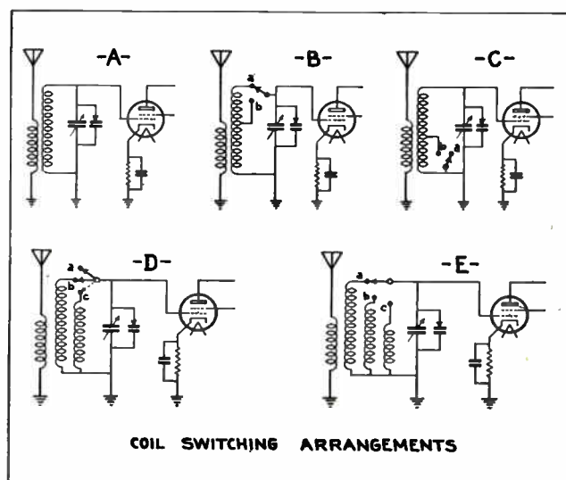
Fig. 180. The above sketches show several different methods of using tapped coils or separate coils, with different inductance values, for changing the frequency bands or wavelengths of receivers.
