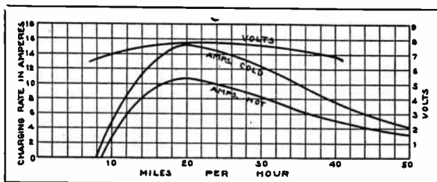
Fig. 76. These curves show the variation in generator voltage and charging current with changes of car speed and variations in generator temperature.
