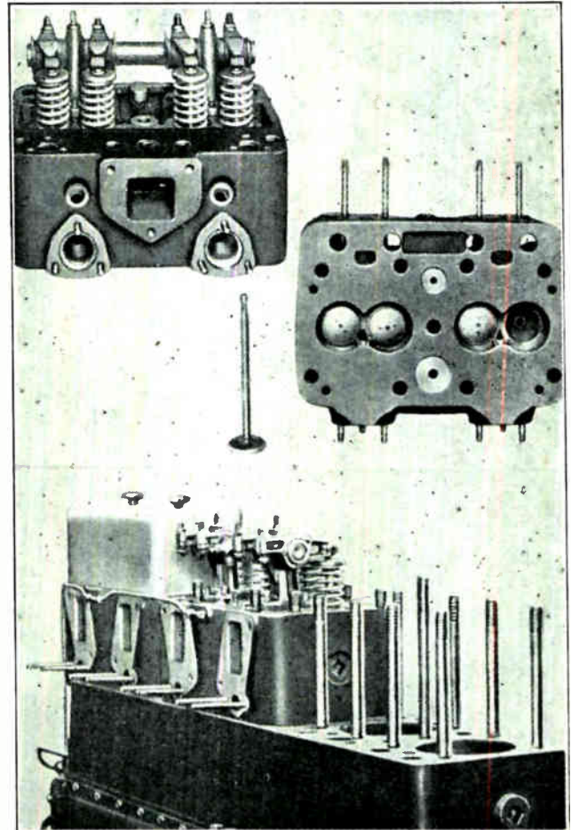
Fig. 141. In the lower view is shown a six cylinder Diesel engine from which one section of the cylinder head has been removed. Note that each cylinder head section covers two cylinders and is equipped with the intake and exhaust valves which are located right in the cylinder head.
