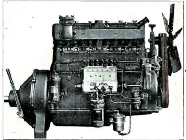
Fig. 6. This photo shows a modern six cylinder automotive type Diesel-engine. Note the similarity to the ordinary gasoline engine except for the fuel pump and the injectors which replace the ordinary carburetor and spark plugs. (Courtesy of the Buda Company.)
