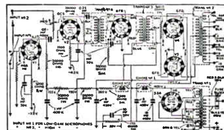
Fig. 234. The above three diagrams show circuits of popular type P.A. amplifiers. The top circuit is for a 36 watt amplifier such as made by Radolek Company, Chicago. The middle diagram shows the circuit of a 15 watt P.A. amplifier, while the lower diagram shows the circuit of a compact six tube amplifier with its power supply unit and two input circuits. Courtesy RadioCraft Magazine.
