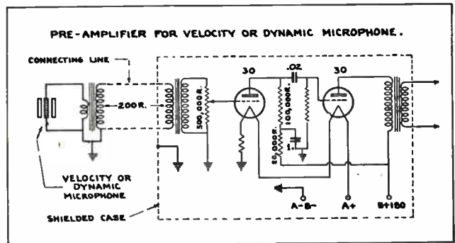
Fig. 244. This diagram shows the connections of a pre-amplifier which can be used for either velocity or dynamic type microphones. The output of this pre-amplifier feeds the first stage of the public address amplifier.
