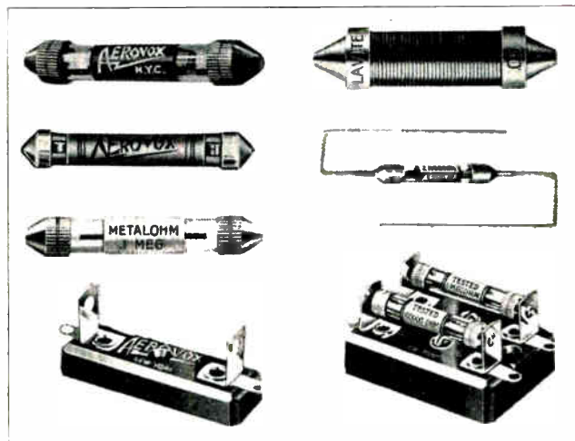
Fig. 122. Photos of several styles of fixed resistor units and mountings, for use in resistance coupled amplifiers, and for grid leaks, and other purposes in radio receivers. (Photo courtesy of Aerovox Wireless Corp.)
