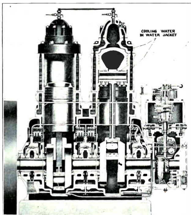
Fig. 107. This sectional view shows the cooling water in the water jacket around the cylinders, cylinder head and pre-combustion chamber of a Diesel engine. Also note the oil lines which carry lubricating oil to the bearings and piston surfaces. (Courtesy Venn-Severin Engine Company.)
