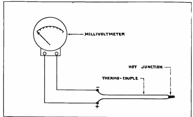
Fig. 101. Diagram showing the connections of a thermo-couple and millivolt-meter used for indicating exhaust gas temperatures on Diesel engines.
