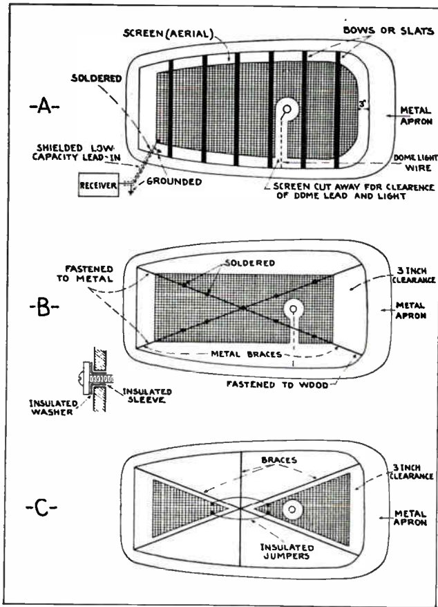
Fig. 215. The above views show several different methods of installing antennas in the roofs or tops of automobiles. Each of these methods is fully explained on the accompanying pages.
