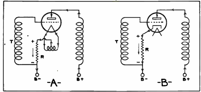
Fig. 72. Diagrams showing method of obtaining negative bias voltages for grids of amplifier tubes of the filament and heater element types, by means of the voltage drop across resistor "R."
