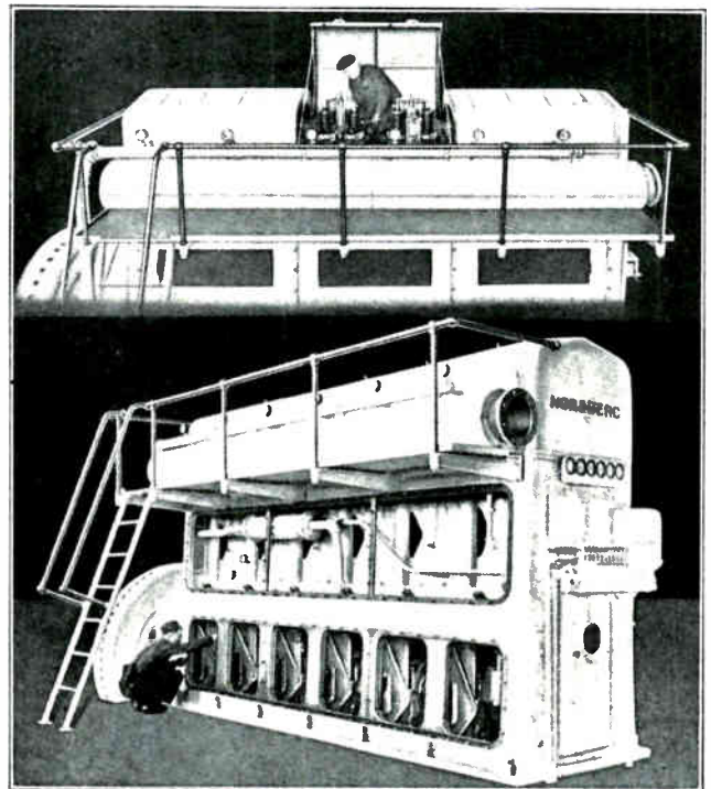
Fig. 143. Some Diesel engines are equipped with covers or housings such as shown above and which make them neater in appearance and quieter in operation. Note in the upper view how the top covers can be conveniently opened for access to the valve mechanisms and cylinder heads. Note in the lower view how the side plates can be removed for access to connecting rod and crank shaft bearings.
