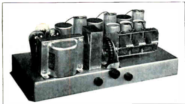
Fig. 189. This photo shows another view of compact, factory made receiver with the power unit located on the left. Note the arrangement and shielding of parts. The wiring, A. F. transformers, and some other small parts are located beneath the sub-panel.
