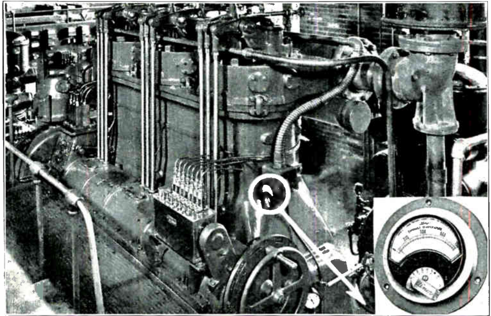
Fig. 103. This photograph shows the pyrometer indicating meter located on the right end of the engine and marked by the white circle. The wiring runs from this meter through the flexible tubing shown, to the thermo-couples located in the exhaust outlet of each cylinder. The insert on the lower right shows a larger view of the meter and the selector switch which is used for taking readings of the temperatures of individual cylinders.
