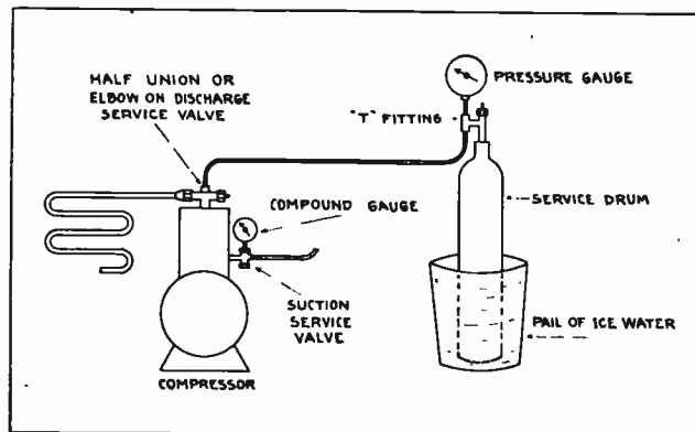
Fig. 106. The above diagram shows the method of connecting a refrigerant service drum to a compressor for discharging the refrigerant from the unit. Observe this diagram carefully while reading the explanation in article 81.
