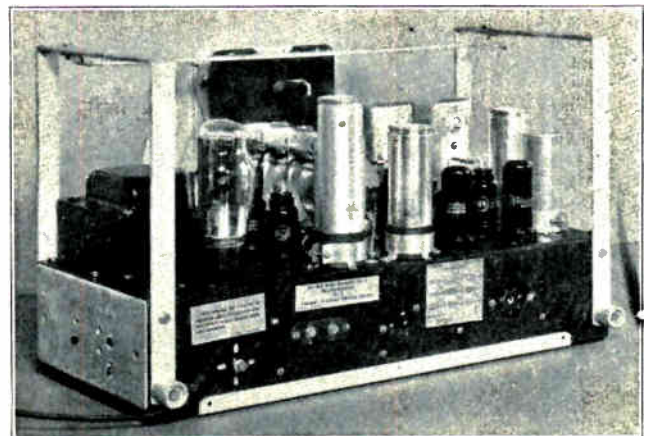
Fig. 143. Photo of a modern A. C. receiver chassis showing power transformers, rectifier tube, tuning condenser, detector and amplifier tubes, and shielded condensers and R. F. transformers. Courtesy Stromberg Carlson Co.
