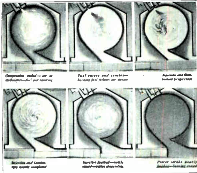
Fig. 58. The above illustrations show the fuel injection, turbulence and combustion, in a pre-combustion chamber of the Waukesha Comet Diesel engine. Examine each view carefully and note the various stages through which the fuel oil passes during ignition and combustion, all within a small fraction of a second.
