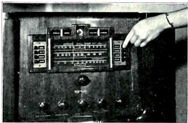
Fig. 176. Note the push buttons for automatic tuning on this console type receiver, and also the kilocycle and megacycle scales for the broadcast and short wave stations, the cathode ray tuning indicator above the scales, and the manual tuning knob below the scales. Courtesy R.C.A. Victor Corporation.
