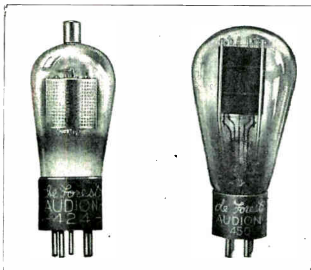
Fig. 82. On the left is shown a screen grid amplifier tube, and on the right a power amplifier tube. (Photo courtesy of DeForest Radio Co.)
