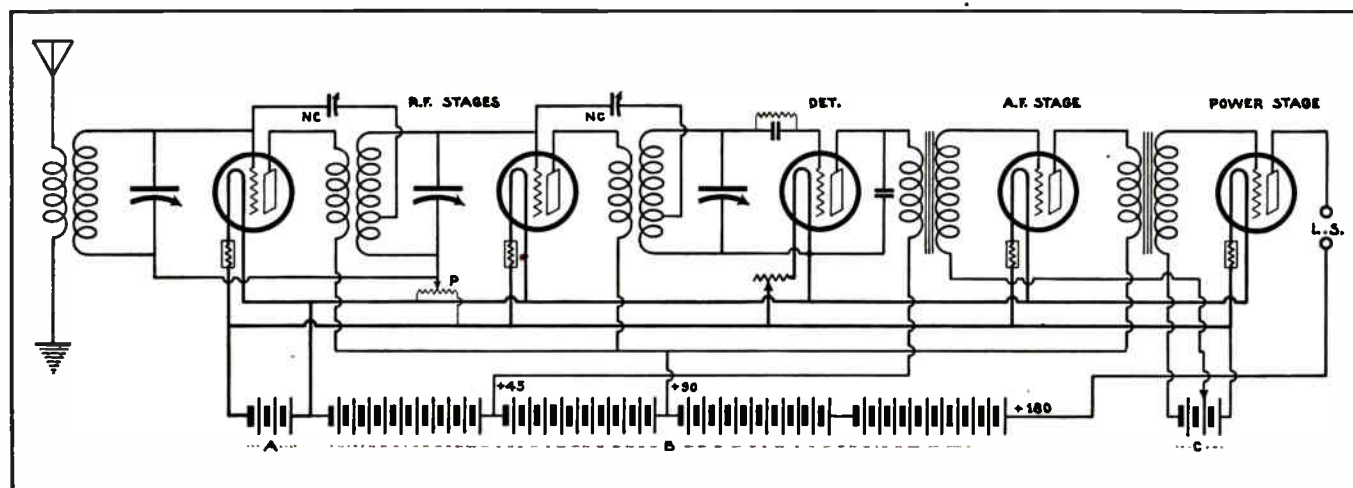
Fig. 124. Circuit diagram of a five tube neutrodyne receiver. Note the two neutralizing condensers N. C. connected across the R. F. amplifier tubes for balancing out the effect of the tube capacity. Also note the tapped secondaries of the special R. F. transformers or "neutroformers," to which one lead from each neutralizing condenser connects.
