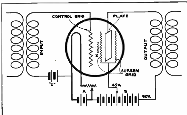
Fig. 76. Diagram of a screen-grid tube showing the connection of the screen grid, and illustrating the manner in which it reduces the capacity between the control grid and plate.
