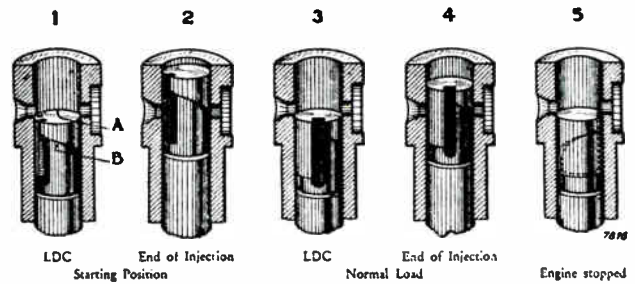
Fig. 31. The above sectional views of Bosch fuel pump cylinders and plungers show the plungers in five different positions of the stroke, and rotated at different angles to illustrate the variable discharge feature of this type of pump. (Courtesy United American Bosch Corp.)
