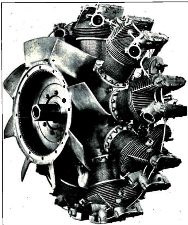
Fig. 151. Another view of Buda-Guiberson Diesel engine, Model T-1040 radial aircooled type. Note air fan for cooling cylinders.
