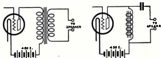
Fig. 118. The sketch on the left shows the transformer method of coupling a loudspeaker to the output or plate circuit of the last tube. On the right is shown the impedance method of speaker coupling.
