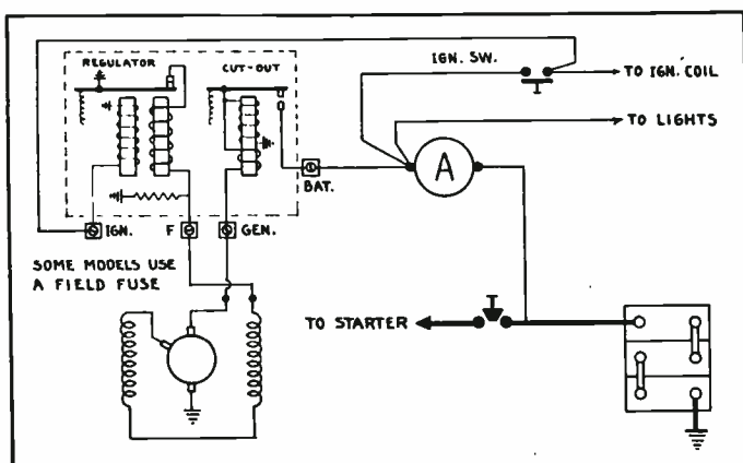
Fig. 80. Circuit diagram of a vibrating type generator control.
