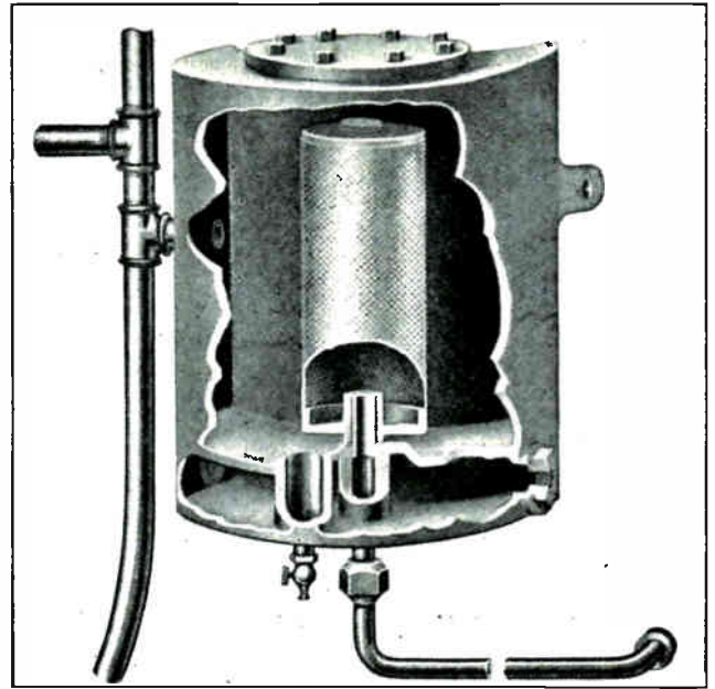
Fig. 50. Cut-away view of auxiliary fuel oil tank, showing filter screen, water sump and valve, and hot water chamber for pre-heating heavy fuel oils. (Courtesy Venn-Severin Co.)
