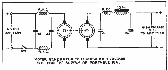
Fig. 232. Diagram showing the connections of battery operated motor generator power supply units such as were shown on the right in Fig. 231. Note the filter circuits used to provide smooth D.C. for the tube plates and also to eliminate commutator hum or interference.
