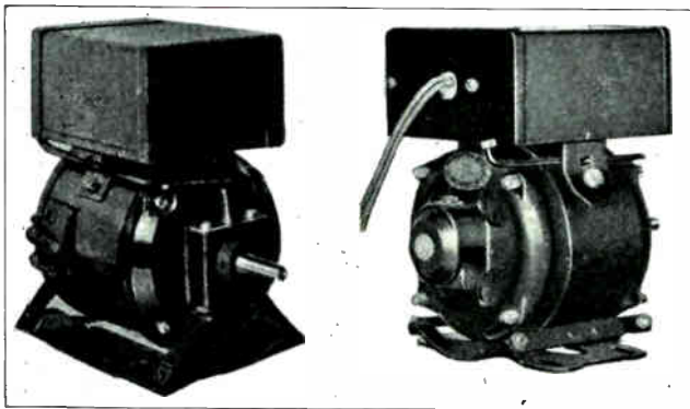
Fig. 113. Two popular types of capacitor motors such as are used by the millions on domestic refrigerators. Note the condensers on top of the motors.
