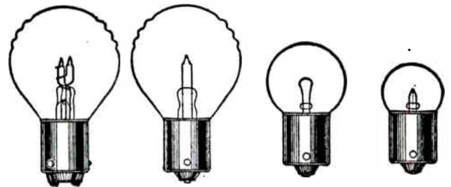
Fig. 83. Several types of double and single filament bulbs used for headlights and other lights on automobiles.
