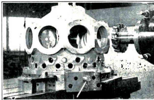
Fig. 152. Complete crankcase in process of machining. Note large openings to which cylinders will be attached and small openings for valve rods and fuel pump barrels.
