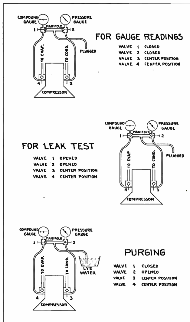
Fig. 108. The above diagrams show proper methods of connecting valve manifold and service gauges for testing and purging refrigerator systems. Carefully observe the position of all valves for each test and refer to these diagrams when making any such tests on refrigerators.
