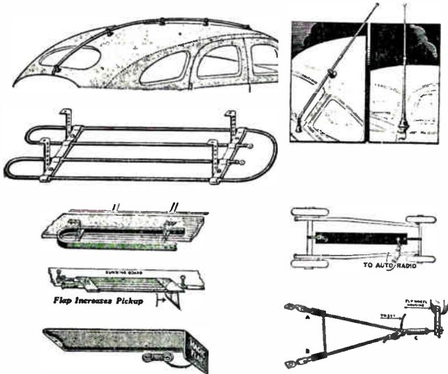
Fig. 217. The above views show several different types of car top, running board, and under-car auto radio antennas and their methods of installation.
