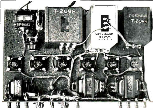
Fig. 115. This photograph shows the wiring and arrangement of parts in a complete power amplifier without the tubes. Two number "210" power tubes are used in push-pull in the last stage of this amplifier. It also contains its own power supply unit. (Photo courtesy of Thordarson Electric Mfg. Co.)
