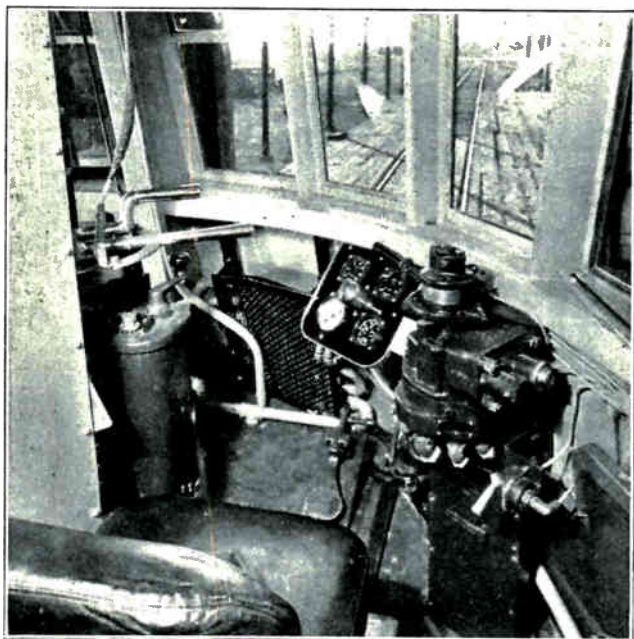
Fig. 90. Photo of the inside of the engineer's cab of a Diesel-Electric locomotive showing the engine and generator controls. (Courtesy Burlington Railway Co.)
