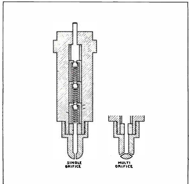
Fig. 46. Sketch showing a sectional view of single orifice and multi-orifice open type injector nozzles. Note the series of spring loaded ball check valves.
