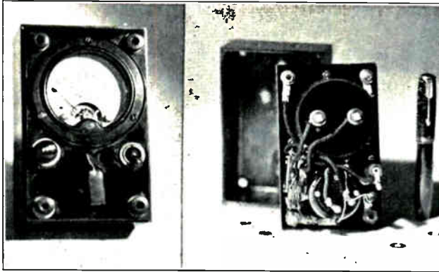
Fig. 198. This photograph shows two views of a very compact and convenient ohmmeter or multi-range meter for radio testing. On the right is shown a view of the back of the instrument opened up so the meter terminals, selector switch, rectifier and resistors can be seen. Note the fountain pen standing on the right to give an idea of the compact size of this unit.
