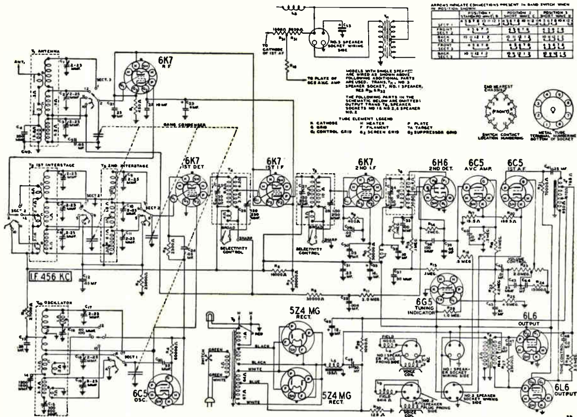
Fig. 183. Wiring diagram of another type of all-wave superheterodyne receiver, showing multiple band coils and selector switches. This is a good circuit to observe and trace carefully.
