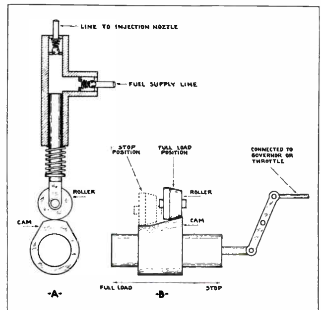
Fig. 36. The above diagrams illustrate the variable stroke type of Diesel fuel injection pump. Note how the amount of fuel charge is controlled by shifting the tapered cam.
