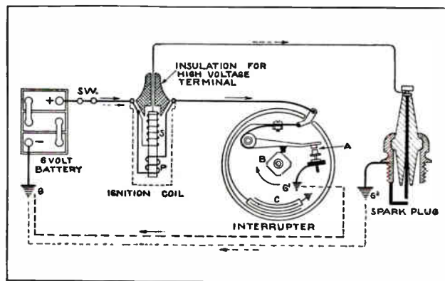
Fig. 24. This simple sketch shows both the primary and secondary circuits of a battery type ignition system. Trace the primary current through the heavy wire and ground connections, and the secondary current through the light wire, spark plug, and ground connections.
