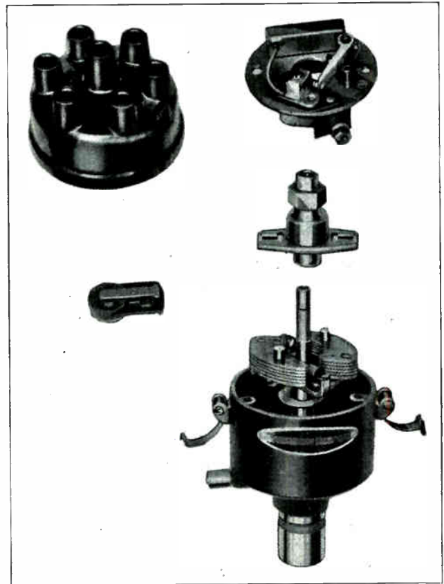
Fig. 37. Disassembled view of a distributor with automatic spark advance, showing the governor weights in the view at the lower right.
