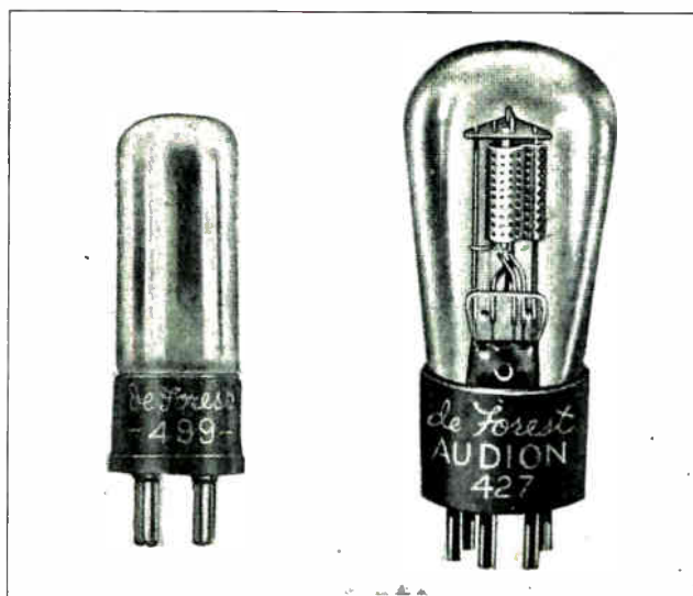
Fig. 81. Photo showing two different types of vacuum tubes for use in radio receivers. The filament of the small tube on the left can be operated on dry cells thus making it very good for use in portable sets. (Photo courtesy of DeForest Radio Co.)
