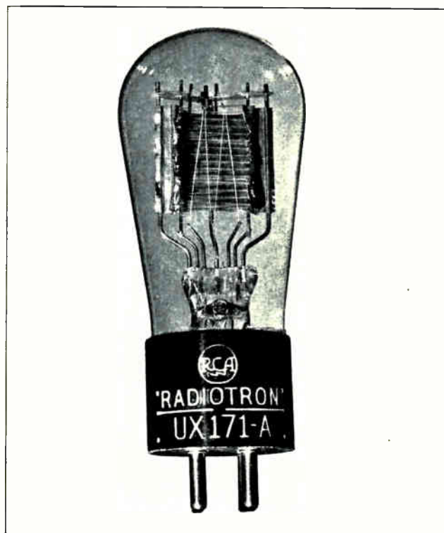
Fig. 55. Photograph of a vacuum tube with the plate opened up on one side to show the location of the grid and filament which are surrounded by the plate.
