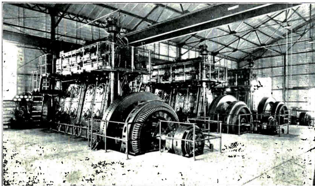
Fig. 70. Modern Diesel-Electric power plant showing three 500 kilowatt, 2300 volt, 3-phase alternators, driven by direct connection to 180 R.P.M. Diesel engines. (Courtesy Allis-Chalmers Manufacturing Co.)
