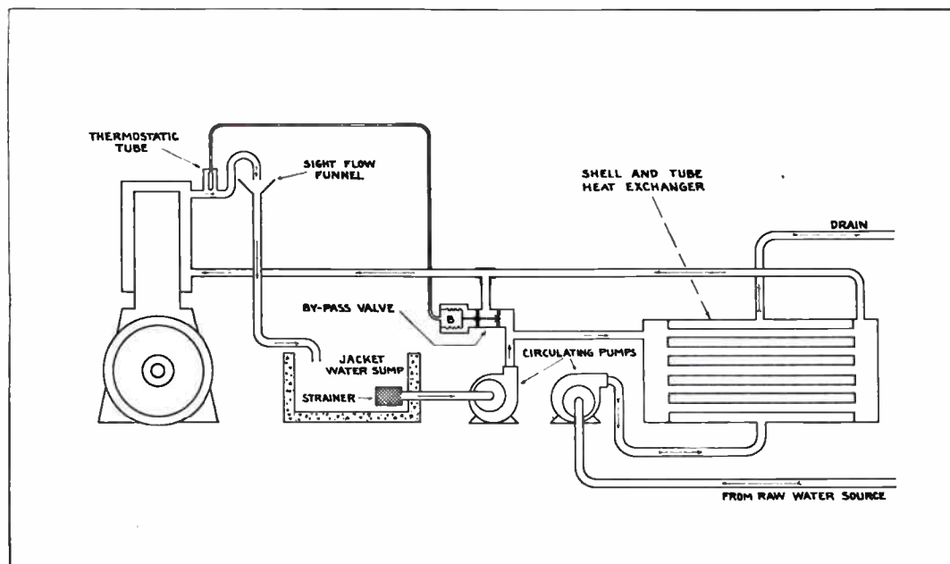
Fig. 113. This illustration shows the piping and water circulating arrangement of a closed type cooling system using a shell and tube heat exchanger and automatic temperature regulating valve.
