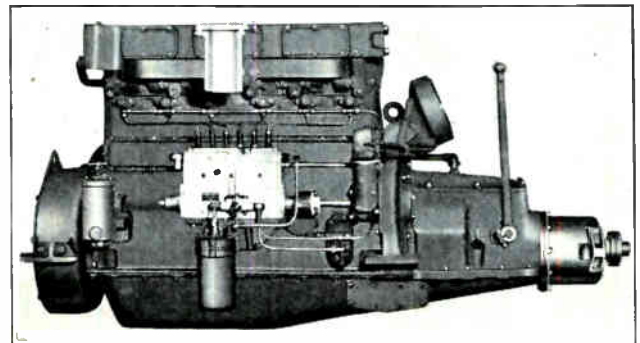
Fig. 14. Photograph of a modern marine type Diesel-engine such as used in pleasure craft and small service boats. Note the oil filter, fuel pump, and fuel lines running to the injector nozzles. (Courtesy of the Buda Engine Company.)
