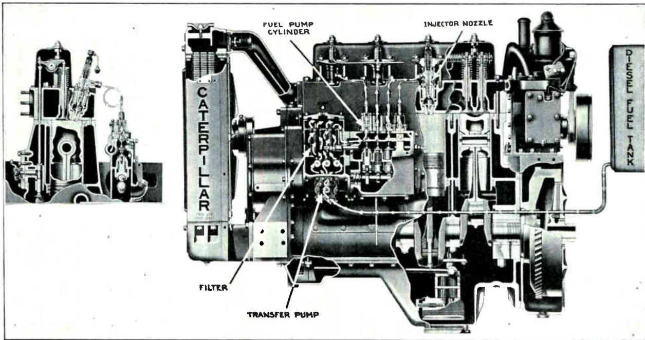
Fig. 28. This illustration shows a sectional view of a Diesel engine including the important parts of the fuel system. Note the fuel tank, fuel line, transfer pump, filter, fuel injection pump, and injector nozzles, and trace the path of the fuel oil through the system. (Courtesy Caterpillar Tractor Company.)
