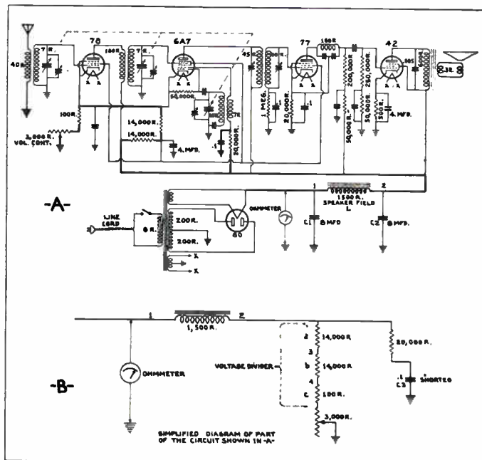
Fig. 209. The diagram at "A" shows the circuit of a modern radio receiver, with the correct values of various resistors and condensers marked. Observe this diagram carefully while reading the instructions on various service tests for this receiver. The sketch at "B" shows a simplified view of part of the wiring of the complete circuit at "A". Compare the lower sketch with the same section of the circuit above.
