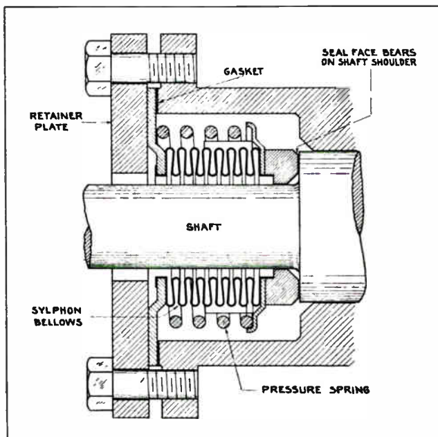
Fig. 39. Carefully examine all details of the syphon bellows type shaft seal shown in the above diagram. This type of seal is extensively used in domestic type refrigerators.
