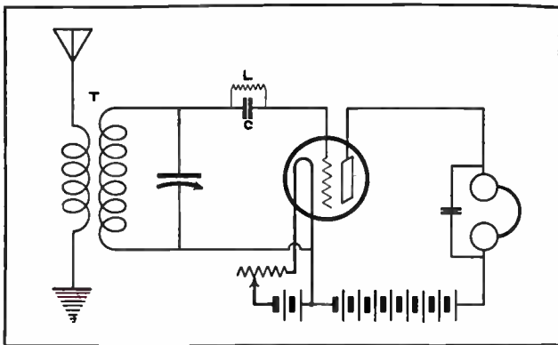
Fig. 62. Diagram of a simple single tube detector circuit using a grid leak and condenser to obtain detector action.
