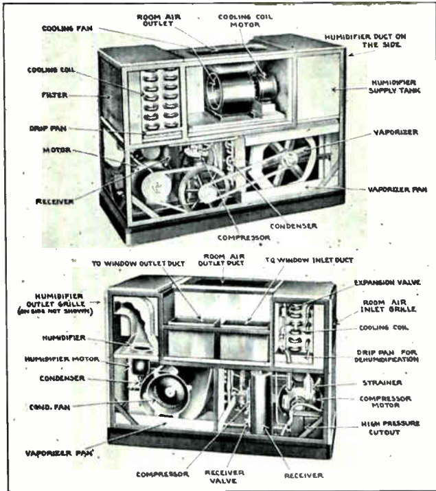
Fig. 145. Two excellent views of a room cooler unit with cover removed to show all working parts. Note the location and names of all the parts as marked on the photos. Courtesy Pacific Mfg. Corp.
