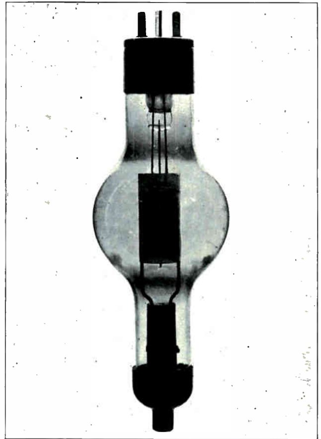
Fig. 14. Photo of a large vacuum tube such as commonly used in radio transmitters.
