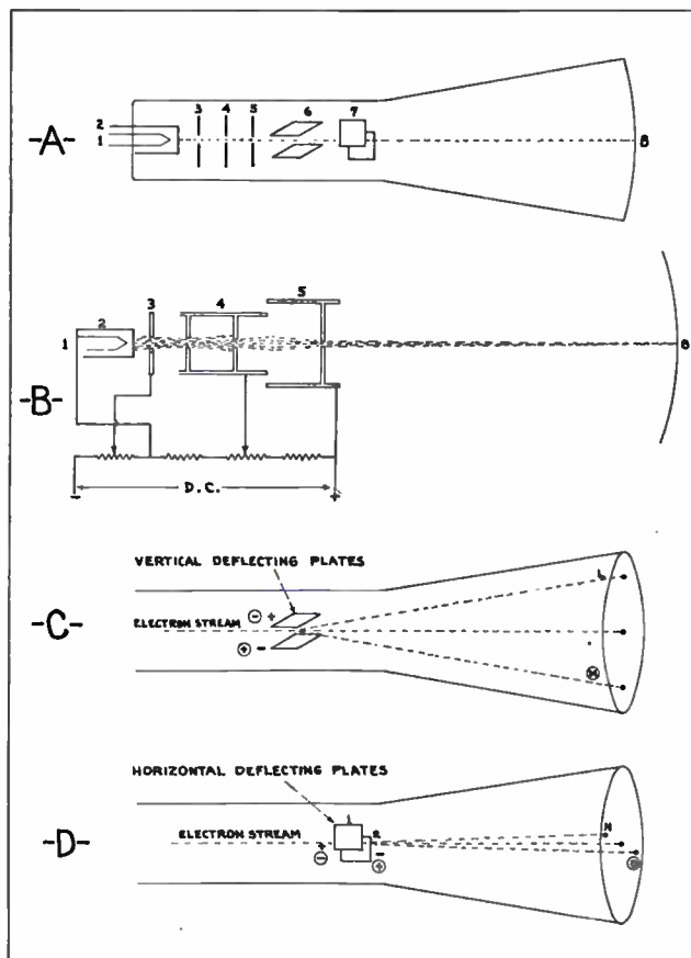
Fig. 248. The above diagrams show several views of cathode ray tubes and illustrate the principle of operation of the electron beam which traces the image of voltage or current waves on the fluorescent screen. Carefully note the various important parts of the tube which are numbered and explained in the instruction material on these pages.
