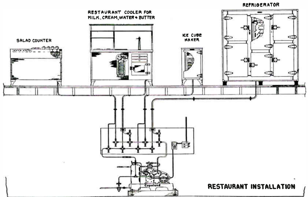
Fig. 123. Diagram showing arrangement and connections of a commercial refrigeration system in a restaurant. Note the separate liquid and suction lines running from the valve manifold panel to each cabinet.
