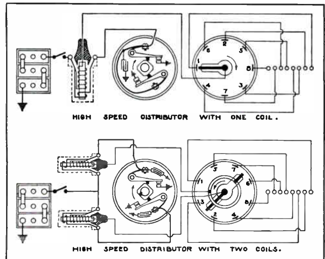
Fig. 42. The top diagram shows the connections for a high-speed distributor using one coil on an eight-cylinder engine. Below is shown the same type breaker using two coils and a slightly different arrangement of the secondary rotor arms and distributor cap contacts.
