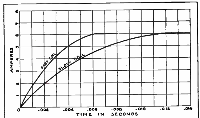
Fig. 26. The above curves show the difference in time required for different types of coils to build up their full primary current after the breaker points close.
