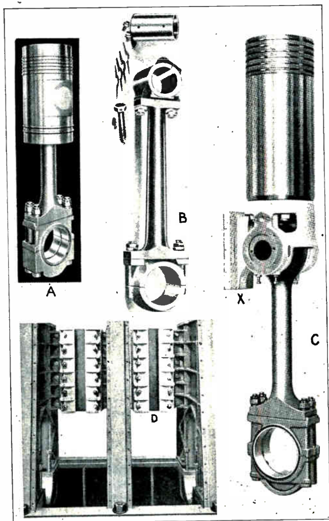
Fig. 129. A trunk type Diesel engine piston is shown at "A" and a crosshead type piston at "C". Note the crosshead pad at "X" which slides up and down in the guides shown at "D". At "B" is shown a connecting rod for a large Diesel engine. Note the provision for adjustments to compensate for wear at both the top and bottom of the bearings of this rod.
