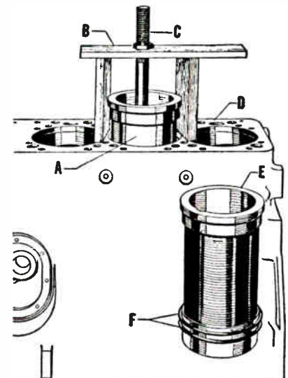
Fig. 148. This illustration shows a convenient method of removing cylinder liners from a Diesel engine. Note the printed explanation above.
