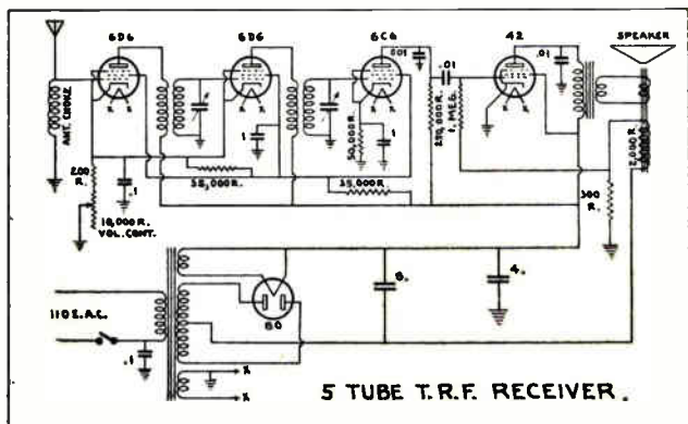
Fig. 148. Circuit diagram of a popular type 5 tube A. C. midget receiver. Note the pentode tubes used for two R. F. amplifiers, detector and one A. F. amplifier. Carefully trace the receiver and power pack circuits, and note the ground connections to the chassis, which completes various circuits.
