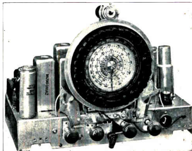
Fig. 175. A good view of the push button dial of the manual automatic tuning system used on another modern type of radio. Courtesy Wells-Garnder Company.
