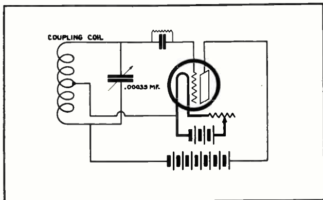
Fig. 200. Circuit diagram of an inexpensive portable modulated oscillator which can be easily made, and which is very useful for testing, balancing and neutralizing radio receivers.
