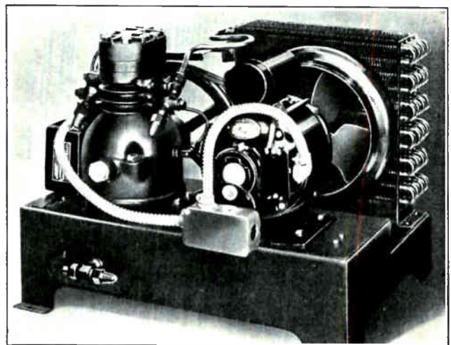
Fig. 23. This photograph shows a modern electric refrigerator condensing unit. Note the compressor and driving motor which are connected together by means of a "V" belt and pulleys. Also carefully note the construction of the condenser which is located behind the fan on the motor pulley. Courtesy General Electric Co.
