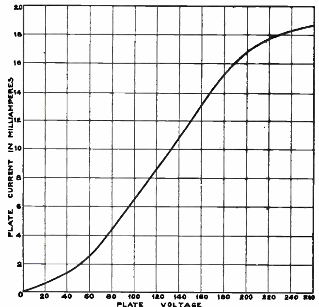
Fig. 59. Curve showing the manner in which the plate current of a vacuum tube varies with changes of the plate voltage.
