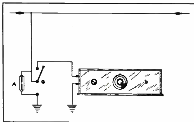
Fig. 33. This diagram shows the method of connecting a lightning arrester and a grounding switch to the lead-in of a radio receiver.
