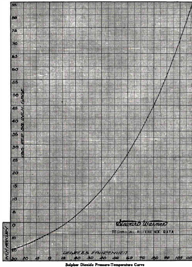
Fig. 15. Chart showing the boiling point of sulphur-dioxide (SO 2 ) refrigerant at various pressures and vacuums. Refer to this chart often while studying about pressures and evaporation. Courtesy Stewart-Warner Corporation.
