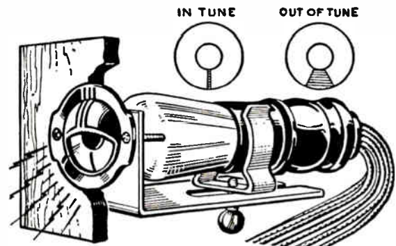
Fig. 93. Sketch of a cathode ray tuning indicator tube mounted in its support behind a shadow shield on the panel of a radio set. Courtesy Radolek Company.
