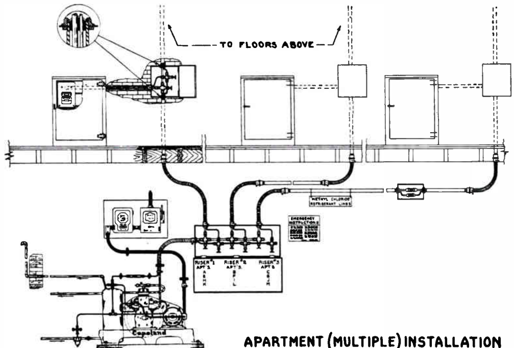
Fig. 33. On the right is shown a diagram of the general arrangement of electrical connections and refrigerant connections for a multiple refrigeration system. Courtesy Servel Manufacturing Co.
