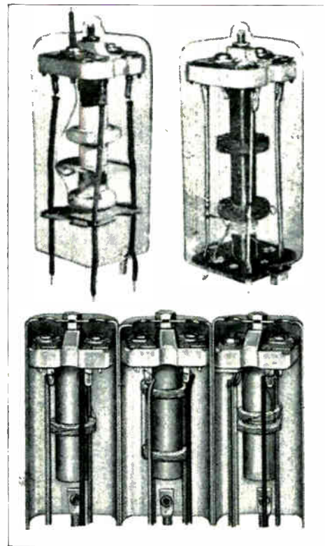
Fig. 166. Several more types of I. F. transformers, showing coils and trimmer condensers. The trimmers are located underneath the adjusting screws on top of the porcelain sections.
