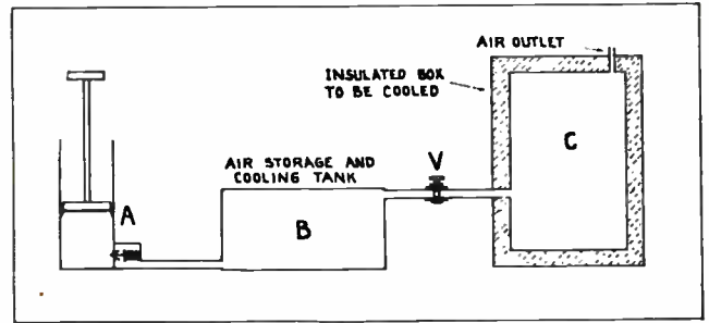
Fig. 16. Diagram illustrating a simple method of accomplishing heat transfer and refrigeration by means of compressed air.
