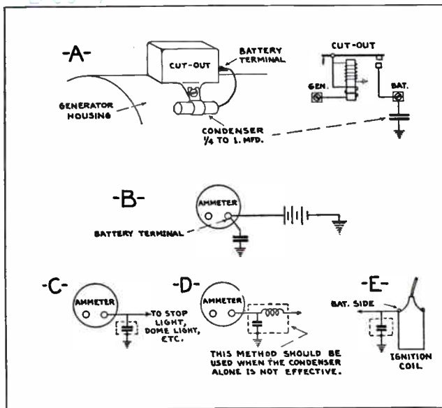
Fig. 223. These sketches show various places where filter condensers may be connected to eliminate radio interference from different sources on the automobile.
