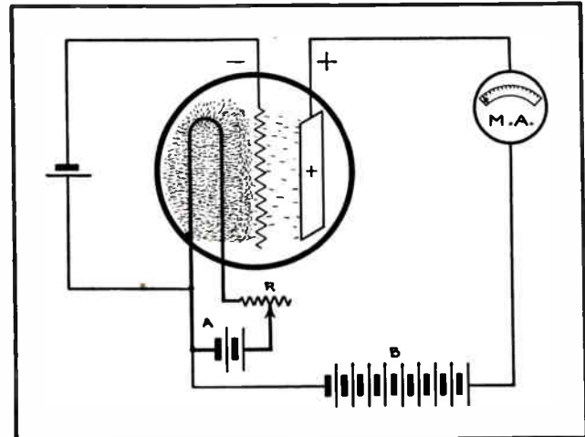
Fig. 61. The above diagram shows the manner in which the electron flow from filament to plate is almost entirely shut off when the grid of the tube is negatively charged. Compare this sketch with those in Figs. 58 and 60.
