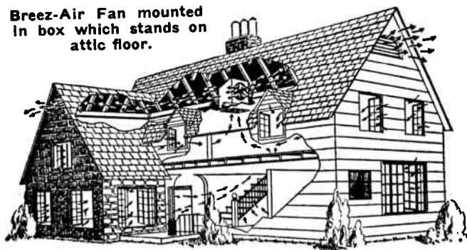
Fig. 162. These two diagrams show how attic ventilator fans can be used to remove heat from attics and draw cool night air into all the rooms of the home.
