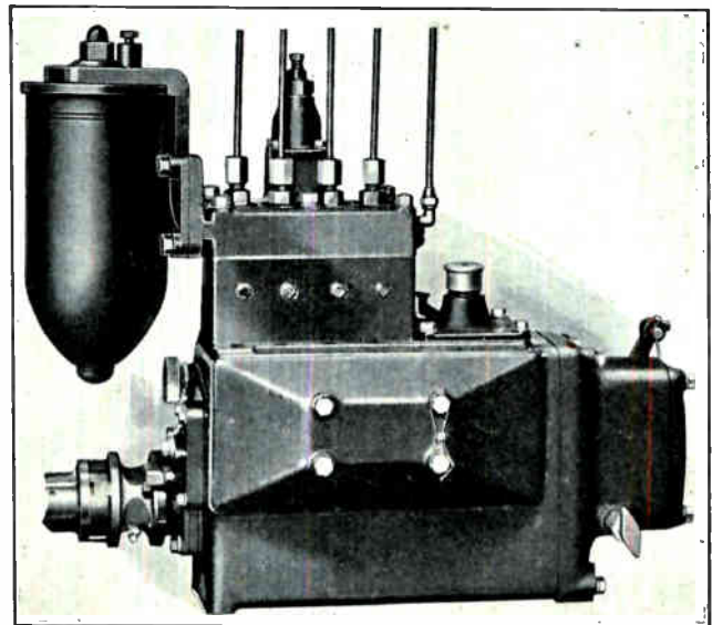
Fig. 29. Photograph of a Diesel engine fuel injection pump, governor and filter assembly for a four cylinder engine. (Courtesy International Harvester Company.)
