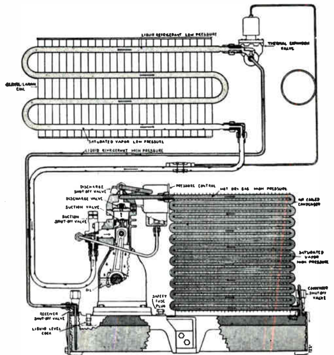
Fig. 27. Cycle diagram of a Servel refrigerator using a dry type evaporator, thermal expansion valve, air-cooled condenser, and reciprocating compressor. Courtesy Servel Corp.
