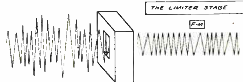
THE LIMITER STAGE IS USED IN F.M. RECEIVERS TO REMOVE VARIATIONS IN AMPLITUDE OF THE FREQUENCY-MODULATED WAVE. LOW PLATE AND SCREEN VOLTAGES ARE EMPLOYED SO THAT THE LIMITER OVERLOADS EVEN WHEN THE INPUT SIGNAL IS WEAK. THE OUTPUT AND TO THE DISCRIMINATOR IS THEREBY MAINTAINED CONSTANT REGARDLESS OF VARIATIONS IN THE STRENGTH OF THE INCOMING SIGNAL DUE TO NOISE OR OTHER CAUSES. THE LIMITER IS NOT USED IN A.M. RECEIVERS.
