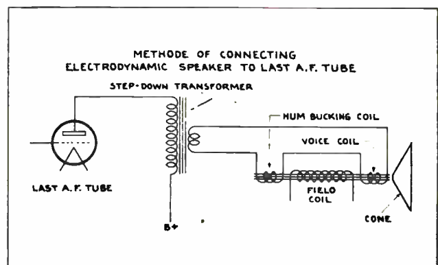
Fig. 134. This figure shows a dynamic speaker connected to the last stage of a Radio receiver. Note how the hum bucking coil is connected in series with the voice coil.
