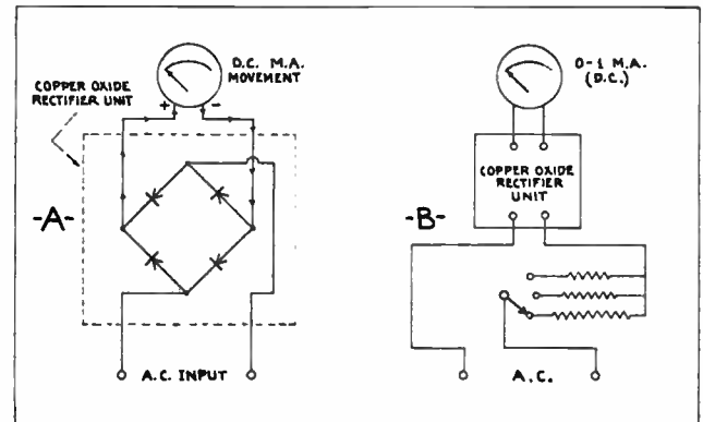
Fig. 204. This diagram shows two methods of connecting rectifiers to radio test meters for taking either D.C. or A.C. readings. The circuit at "B" shows how a milliammeter can be used as a multi-range A.C. voltmeter, by use of the rectifier and proper resistors.
