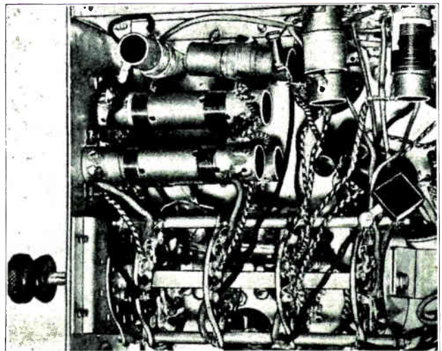
Fig. 182. This view of the under side of a radio chassis shows the gang selector switch and multi-wave coils of an all-wave receiver. Note that the four sections of the rotary multi-point switch are all ganged together on one shaft, for operation by the single knob shown on the left. Courtesy Short-Wave Craft.
