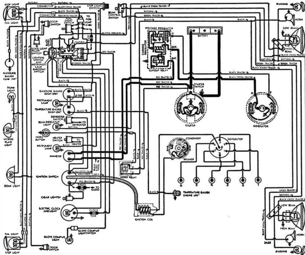
Fig. 90. Wiring diagram of 1941 Oldsmobile car. Note the current-voltage regulator used for controlling generator output, and also the lighting switch and instrument lamp rheostat. Courtesy National Automotive Serv. Co.
