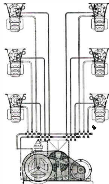
Fig. 124. Diagram of a multiple system with six evaporators and separate liquid and suction lines from each evaporator to the valve manifold at the condensing unit.
