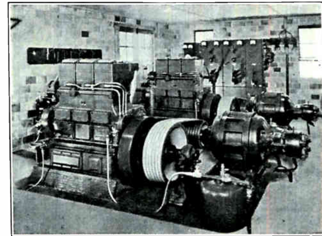
Fig. 11. Two Diesel-Electric generating units in a small town municipal power plant. Note the neat compact arrangement of this plant. (Courtesy of the Cummins Engine Company.)
