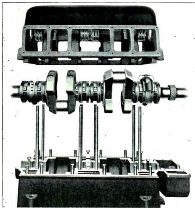
Fig. 137. This view shows the upper and lower sections of a two cylinder Diesel engine crank case with the crank shaft and bearings removed. Note the various bolts which hold these parts in place. (Courtesy Fairbanks Morse Co.)
