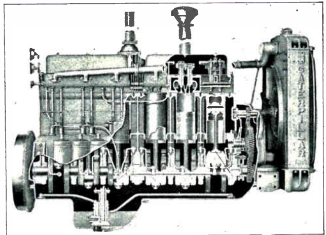
Fig. 120. The above sectional view of a Diesel tractor engine shows the lubricating oil lines and the holes drilled in the crank shaft and connecting rods for conveying oil to the various bearings. In the lower part of the crank case can be seen the gear type oil pump, which feeds oil under pressure to the oil lines and bearings. (Courtesy Caterpillar Tractor Co.)
