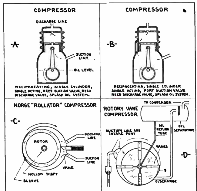
Fig. 35. The above diagrams show several types of reciprocating and rotary refrigeration compressors. Examine and check every operation carefully while reading the lesson material.
