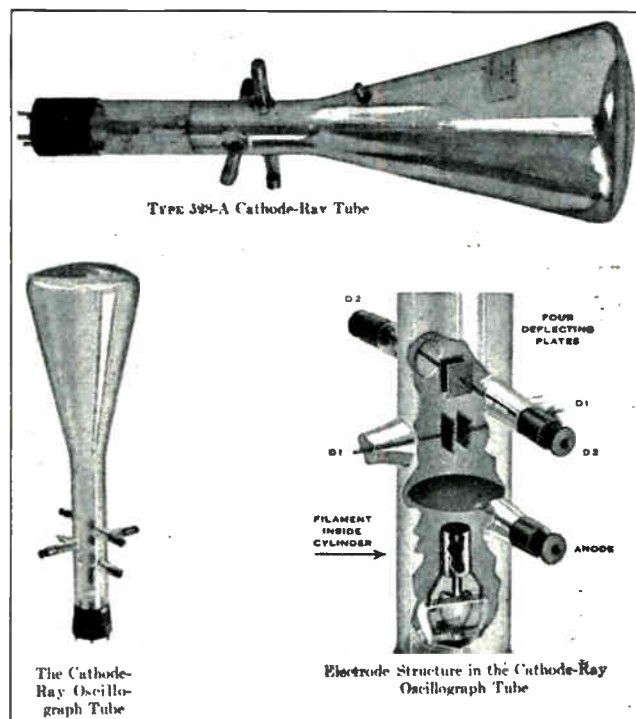
Fig. 247. These views show the construction and parts of a common type of cathode ray tube such as used with oscilloscopes. Note the tube elements and deflector plates, and also the fluorescent screen on the end of the tube. Tubes of a similar type are also used for television equipment. Courtesy General Radio Corporation.
