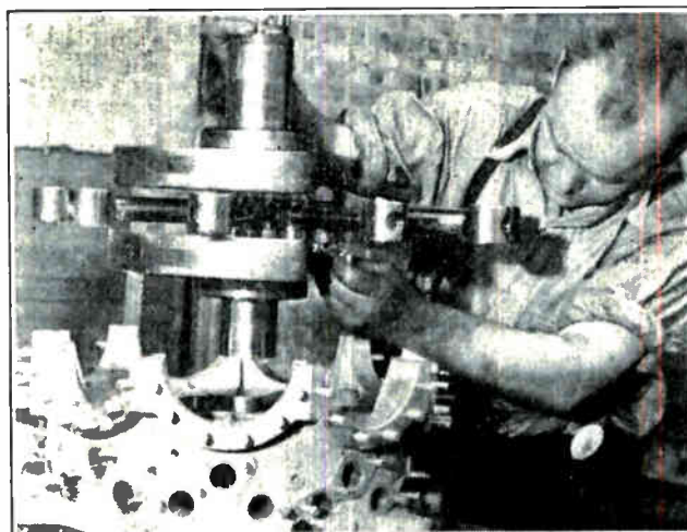
Fig. 154. Assembly of crankshaft and connecting rods in rear half of crankcase of Guiberson radial Diesel engine.
