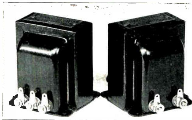
Fig. 114. Photo showing opposite sides of two push-pull A. F. transformers. Note the three terminals on the side with the center-tapped coil. (Photo courtesy of Thordarson Electric Mfg. Co.)
