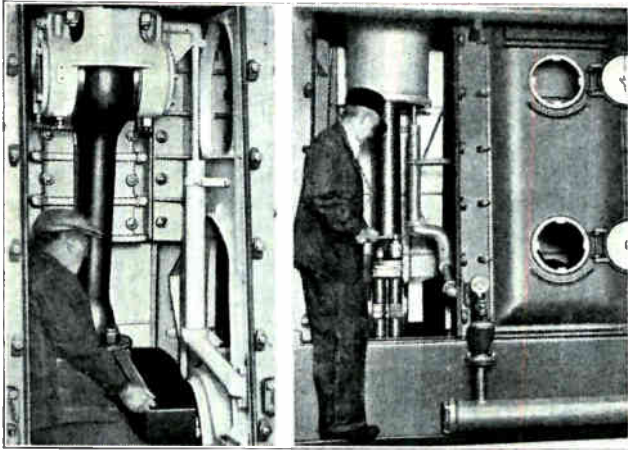
Fig. 144. These photos show how the side plates can be removed from a large heavy duty Diesel engine to permit the operator or repair man to get at the connecting rod and crank bearings to adjust them for wear. Note in the left hand view the crosshead between the top of the connecting rod and the bottom end of the piston to which it is bolted. Also note the guide bearing directly behind the crosshead and connecting rod.
