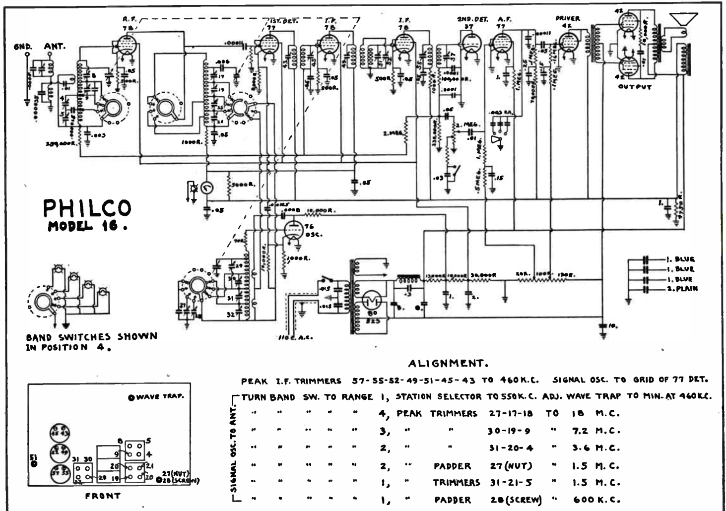
Fig. 159. Circuit diagram of an all-wave "super". Carefully examine all stages, and the oscillator and power pack circuits.
