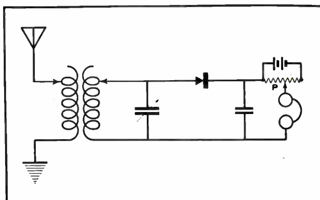
Fig. 46. Sketch of a crystal detector circuit using a battery and potentiometer for applying voltage to the crystal and obtaining slight amplification of the received signal.
