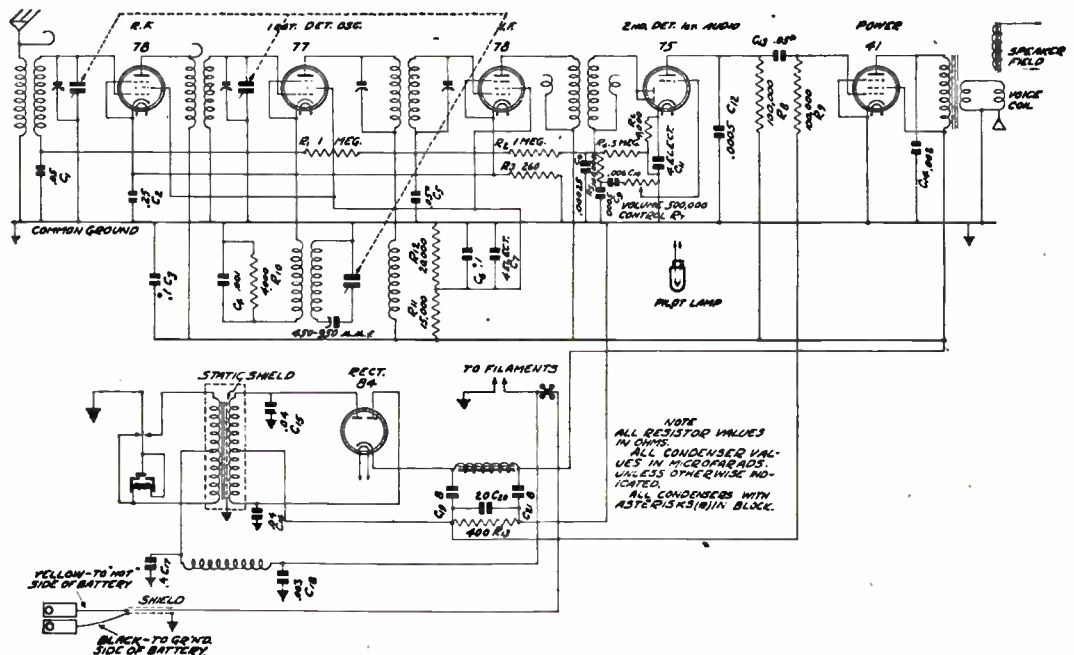
Fig. 225. Circuit diagram of a popular six tube superheterodyne auto radio receiver. Examine this circuit carefully to become familiar with all of the important parts of such receivers. Note the similarity to household radio receivers and also note the vibrator and rectifier circuit. Courtesy Wells-Gardner Company.
