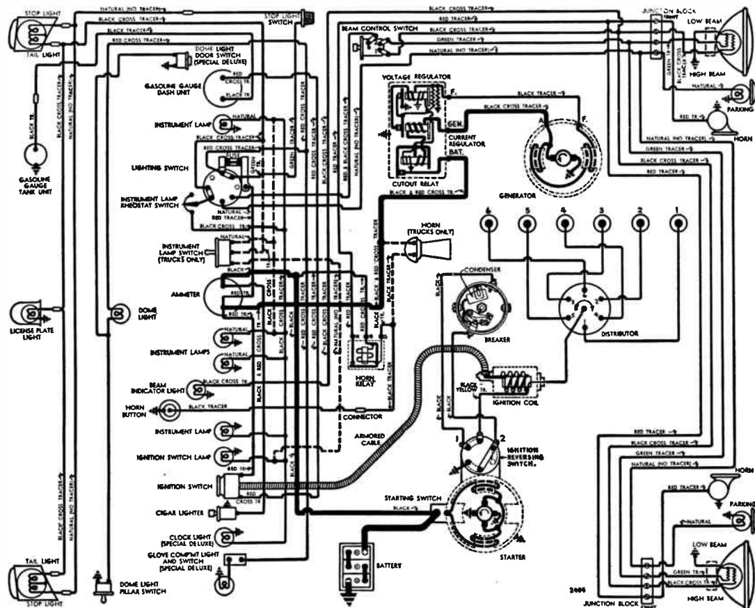
Fig. 88. Complete wiring diagram of 1941 Chevrolet. Note carefully the location and arrangement of all of the electrical devices. Trace the circuits one at a time to become thoroughly familiar with the common types of automobile wiring systems. Courtesy National Automotive Service.
