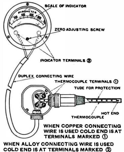
Fig. 102. The above view shows several different types of thermo-couple pyrometers for measuring Diesel exhaust gas temperatures.
