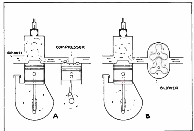
Fig. 22. The above sketches illustrate the operation of air compressors and blowers for charging and scavenging Diesel-engines.
