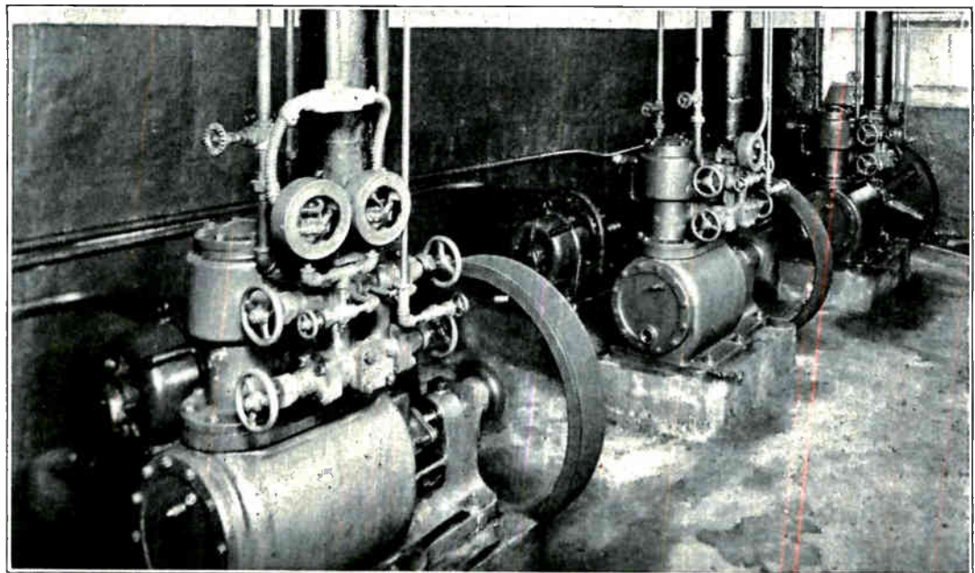
Fig. 58. This photo shows three twin-cylinder refrigeration compressors, all driven by "V" belts connected to electric motors and supplying refrigeration for a large commercial installation. Courtesy Carrier Co.
