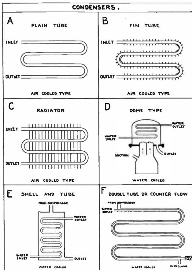
Fig. 45. The above diagrams show the construction of several different types of air-cooled and water-cooled condensers such as used in electric refrigerators.
