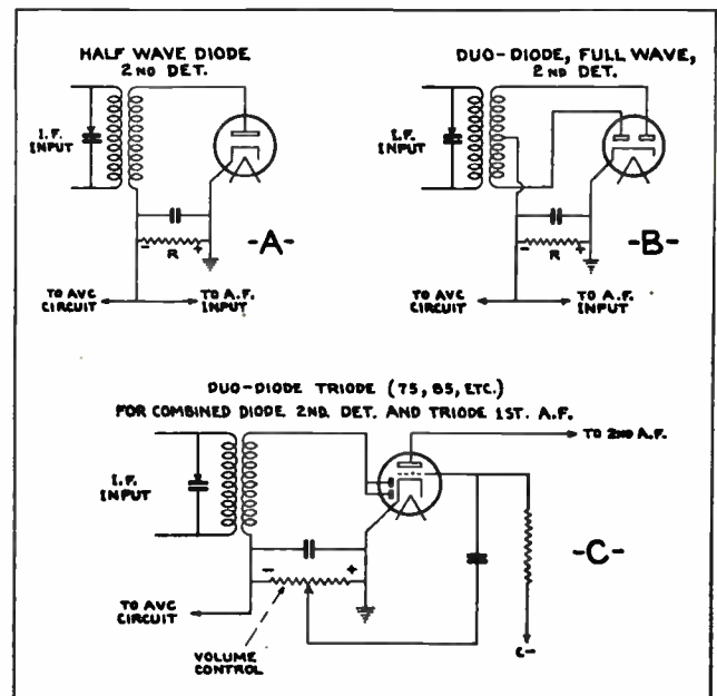
Fig. 162. The above sketches show connections for half-wave and full-wave rectifier type detectors at A and B, and for a double purpose combination detector and first A. F. amplifier tube at C.
