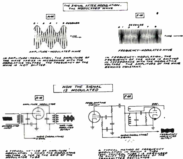
Fig. 191A. This diagram illustrates the difference between A.M. and F.M. modulated waves above, and modulating circuits below.
