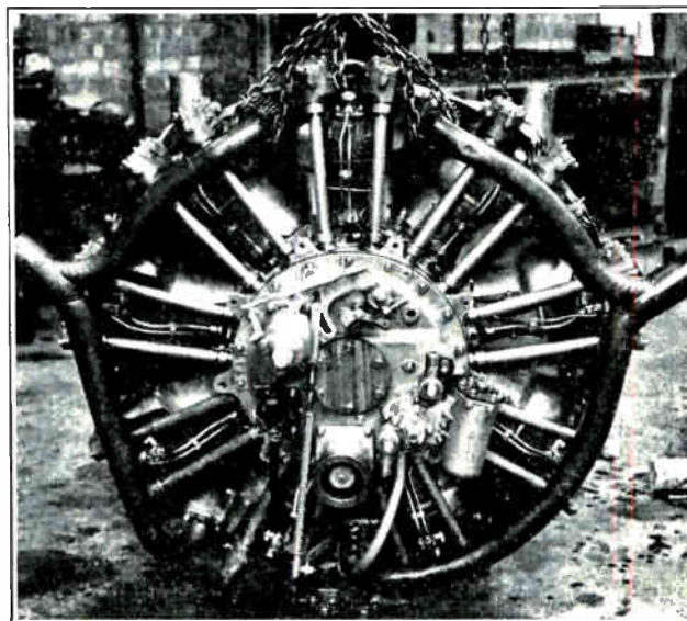
Fig. 150. Buda-Guiberson Diesel engine for tanks and aircraft. Note arrangement of cylinders, valve push rods, injectors and control auxiliaries.
