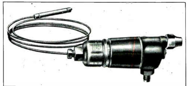
Fig. 51. Photo showing a thermostatic expansion valve with its power bulb and connecting capillary tubing. Courtesy Detroit Lubricator Co.
