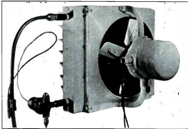
Fig. 171. Compact unit type evaporator or air cooling unit and fan. Note control valve and power bulb on the liquid and suction lines. Courtesy Iig Electric Ventilating Co.
