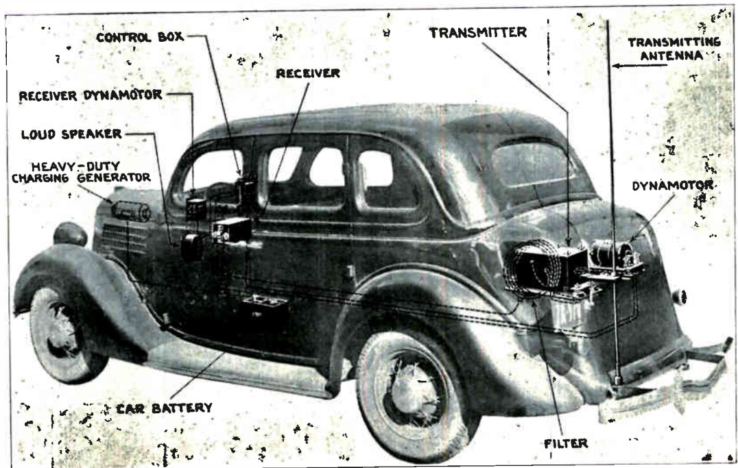
Fig. 211. Photo diagram showing the installation of a complete radio transmitter and receiver in a police car. Thousands of police cars are now being equipped with such two-way radio communication. Installation and servicing of such equipment provides good jobs for many trained radio men. Courtesy General Electric Company.
