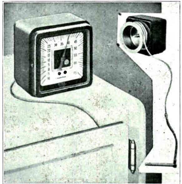
Fig. 122. A very convenient type of thermometer for checking refrigerator cabinet temperatures without repeatedly opening the door, after making adjustments.
