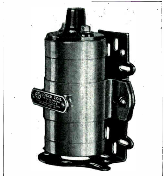
Fig. 22. High-tension ignition coil such as used for supplying high voltage impulses to the spark plugs on the ignition systems of automobiles. The heavily insulated bushing on the top of the coil is where the high voltage lead connects.
