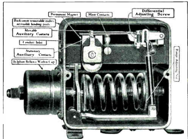
Fig. 53. This view shows the construction and parts of a pressure type electric control switch such as used to start and stop the motor in electric refrigerators and thereby maintain proper operating temperatures. Courtesy Penn Electric Switch Co.
