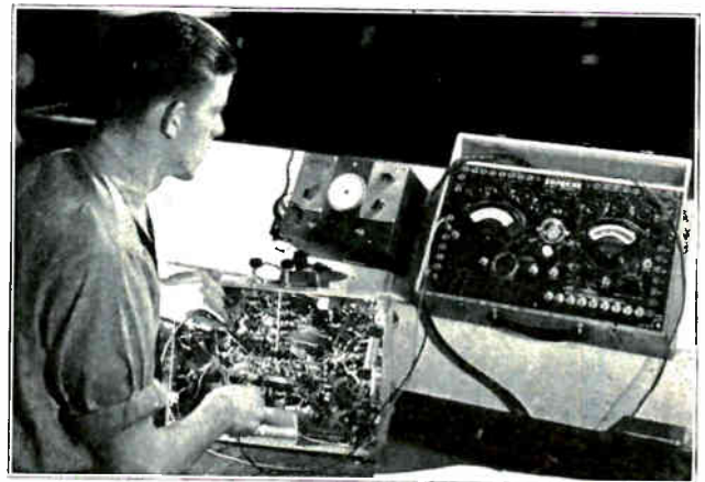
Fig. 199. This view shows an analyzer in use for testing parts and circuits on the under side of a radio chassis. Note the meters, selector switches, pin jacks and tube sockets on this complete analyzer, and also the oscillator or signal generator on the left. The operator is using a pair of test prods for checking resistances and continuity of various parts of the receiver circuit.
