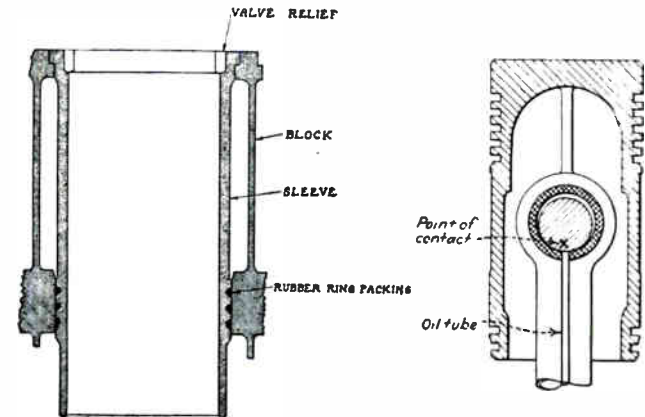
Fig. 133. On the left is shown a cylinder liner pressed into the skeleton cylinder block of a Diesel engine. Note the water space between the liner and the block. This type of liner is known as "wet type" because the water is in direct contact with the outside surface of the liner. Note the rubber packing rings to prevent leakage of cooling water into the crank case. On the right is shown a sectional view of a piston and wrist pin bearing showing how the constant pressure on the lower side of the bearing causes the greatest wear at this point and also tends to prevent proper flow of lubricating oil.
