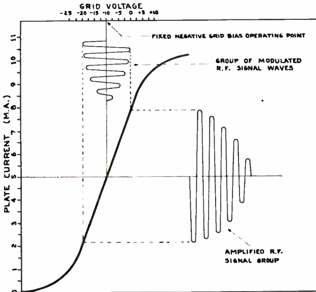
Fig. 71. Curves illustrating amplifier action of a vacuum tube. Note that the grid voltage impulses are greatly amplified or increased in the plate current impulses, but are kept in the same form instead of being rectified.
