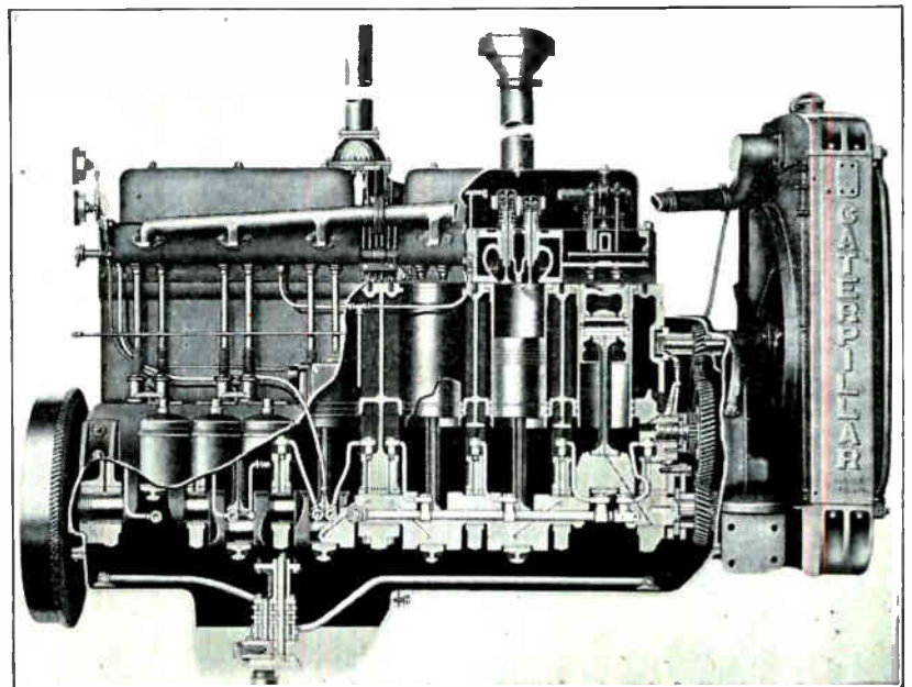
Fig. 7. This excellent sectional view of a modern six cylinder Diesel-engine clearly shows many important construction features. Note the pistons, connecting rods, crank shaft, timing gears, valves, and cylinder liners. (Courtesy Caterpillar Tractor Company.)
