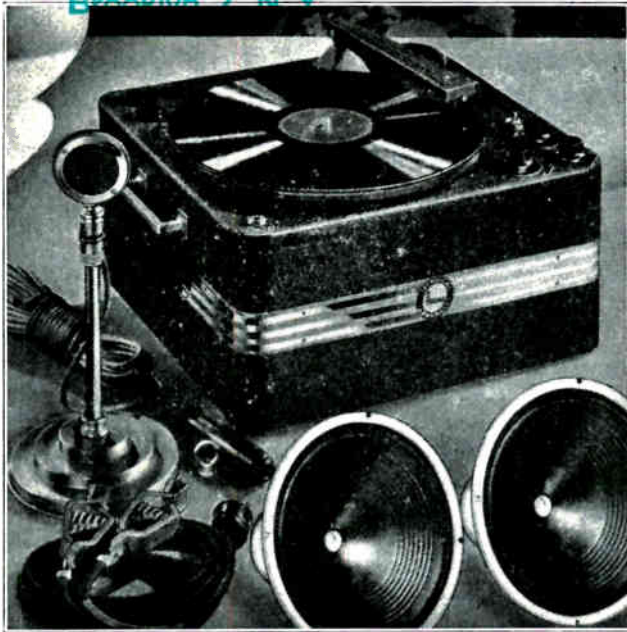
Fig. 229. Phonograph or record turn table and pick-up head with amplifier enclosed in the same compact cabinet. Note the microphone and dynamic speakers which are used with this unit. Courtesy Montgomery-Ward.
