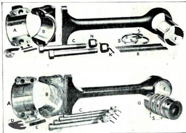
Fig. 134. The above connecting rods are equipped with quill type roller bearings at the right hand or wrist pin ends. Plain split type bearings are used on the crank ends at the left. The split feature allows convenient adjustments to take up the slack due to wear.
