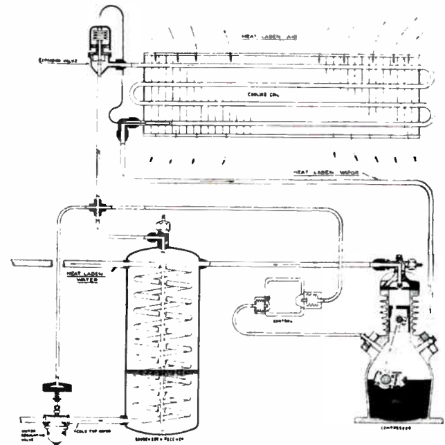
Copeland Commercial Refrigeration Cycle
