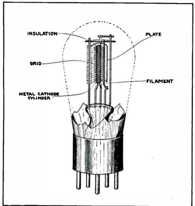
Fig. 79. This sketch gives a sectional view of an A. C. tube and shows the construction of the heater element, its insulator, the cathode, grid, and plate of the tube.
