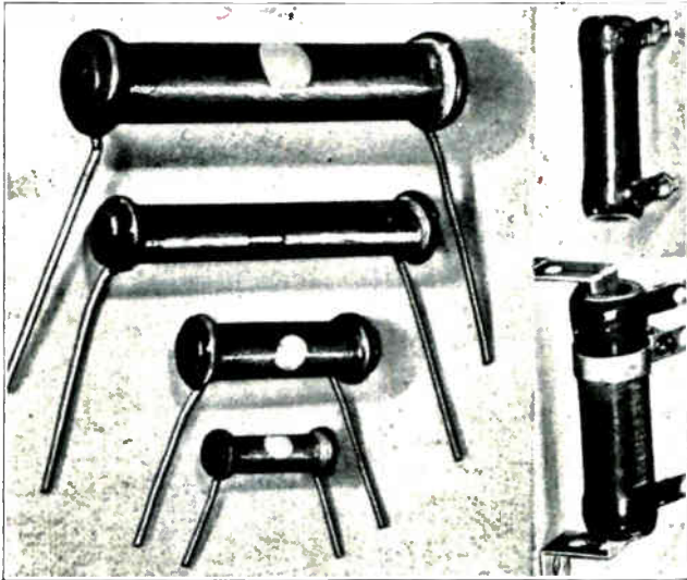
Fig. 151. Several composition type resistors of 2 watt, 1 watt, \frac{1}{2} watt, and \frac{1}{8} watt sizes on the left; and two wire wound resistors on the right.
