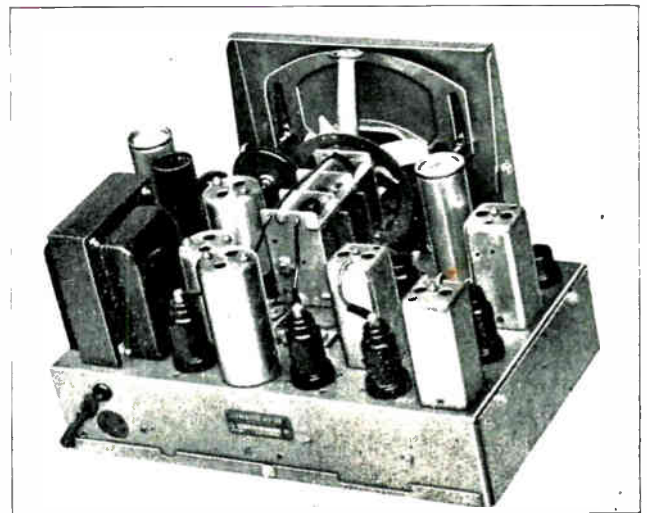
Fig. 194. This view shows the chassis of a radio receiver and illustrates how the serviceman can easily get at the tubes, R.F. and I.F. transformers, tuning condenser and tuning mechanism, and the power transformer. To reach the resistors, condensers and circuit connections on the under side of this set, the chassis must be removed from the cabinet and turned on its side or up side down.
