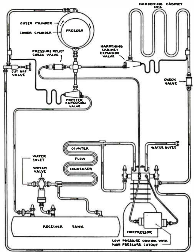
Fig. 133. Cycle diagram of a commercial refrigerating unit used in an ice-cream freezing machine and hardening cabinet. Courtesy Mills Novelty Co.
