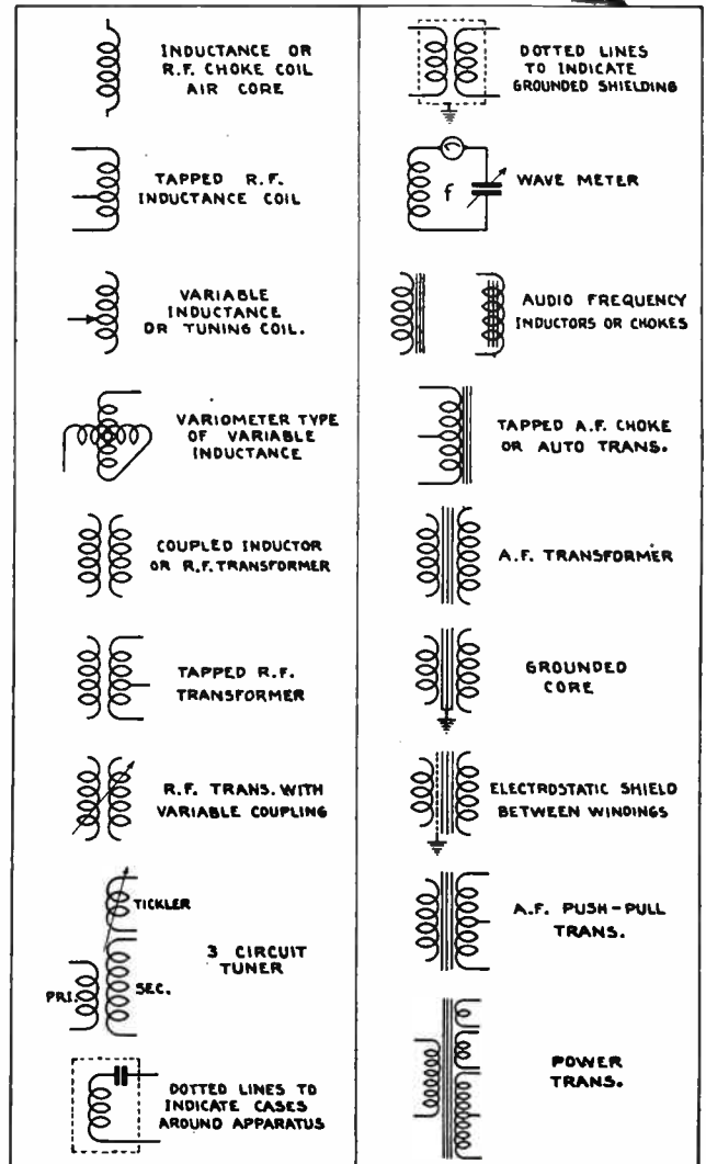
Fig. 48. Radio coil and transformer symbols.
