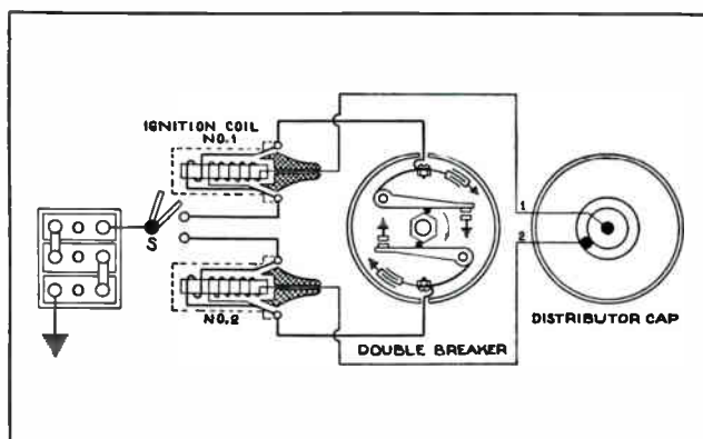
Fig. 38. This diagram shows the parts and connections of a dual ignition system used for firing two plugs in each cylinder. See the rest of this system in Fig. 39.
