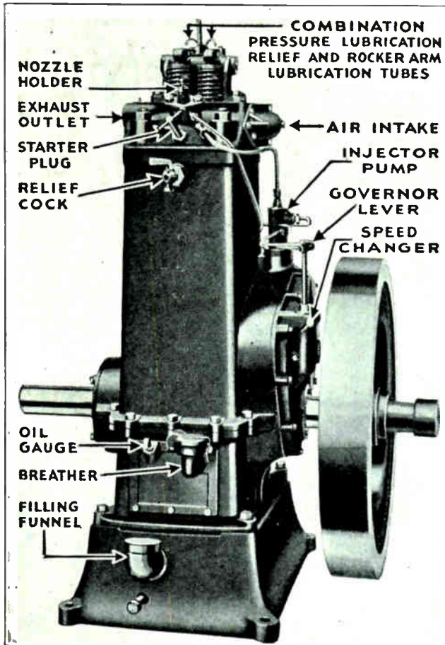
Fig. 3. This illustration shows a popular type of vertical, single-cylinder, 10 h.p. Diesel-engine for stationary use. Note the names and locations of the various parts shown on this engine. (Courtesy of the Stover Engine Company.)
