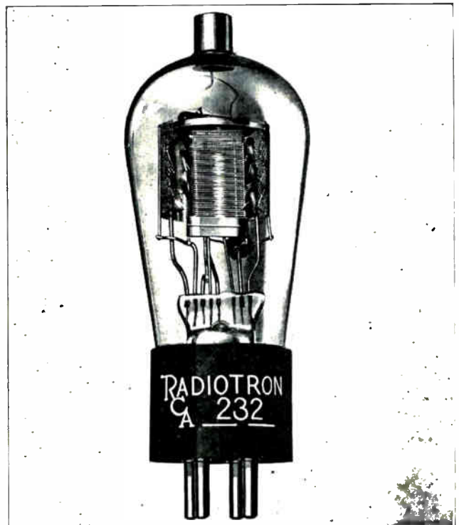
Fig. 77. This excellent photograph shows a vacuum tube with part of the outer screen grid and part of the plate removed, to clearly show the inner screen grid in its position between the control grid and plate. (Photo courtesy of R. C. A. Radiotron Co., Inc.)
