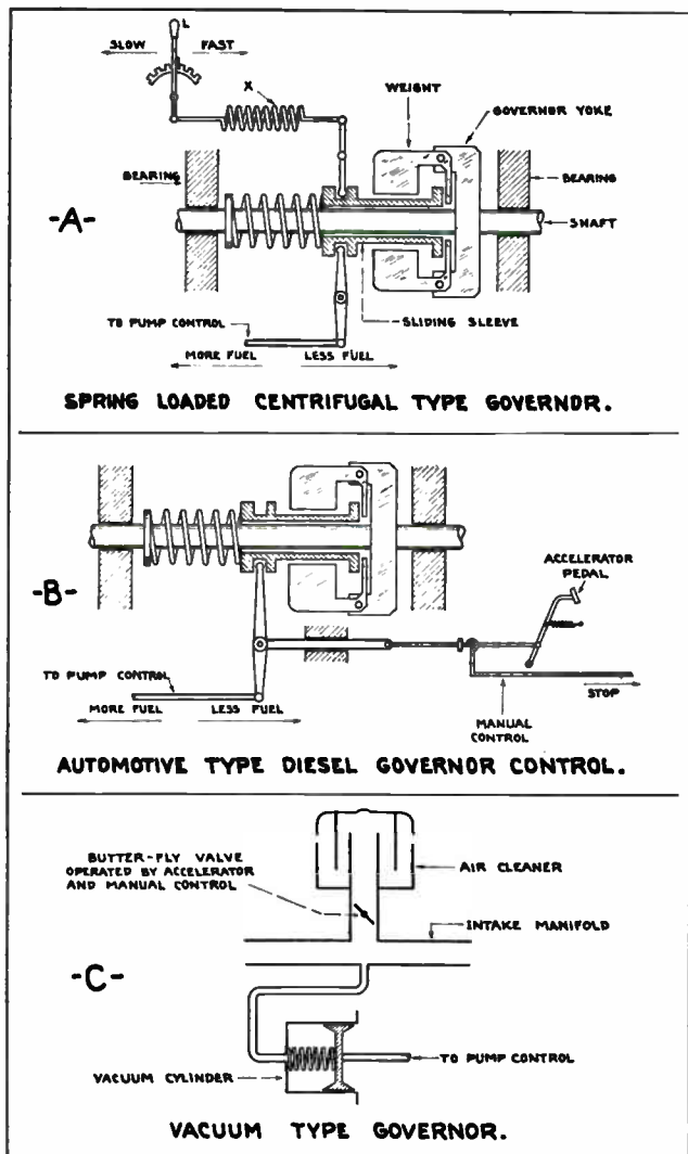
Fig. 53. The above three diagrams show the construction and operation of centrifugal type and vacuum type Diesel engine governors.
