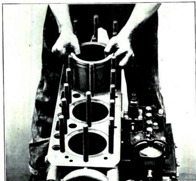
Fig. 135. Photograph showing how cylinder liners can be conveniently removed and replaced on Diesel engines of this type of construction. (Courtesy International Harvester Co.)
