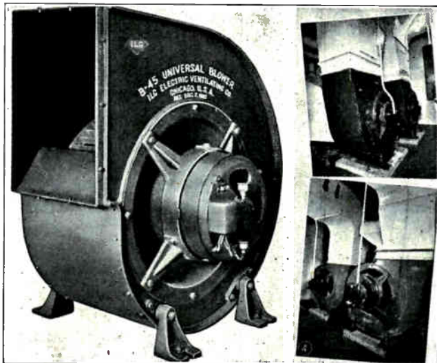
Fig. 164. Large centrifugal fans or blowers of the type shown above are used to circulate air through ducts of air-conditioning systems. Courtesy Ilg Electric Ventilating Co.
