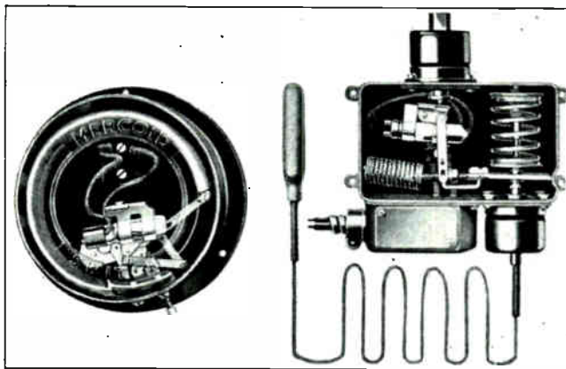
Fig. 130. Two different types of mercury switch controls. Note the mercury tubes with flexible wire leads attached. The tubes can be tilted by pressure bellows and bulb or by thermostat strips.
