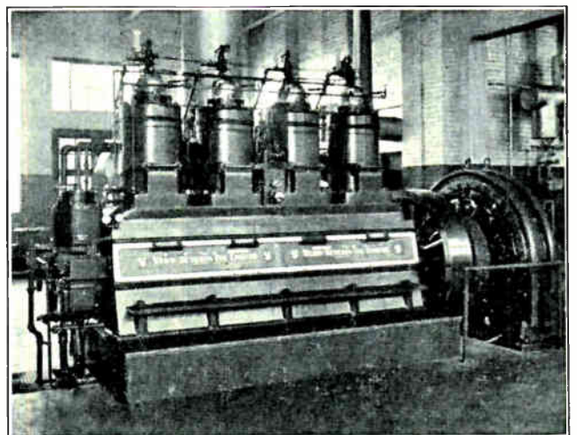
Fig. 10. Four cylinder 300 h.p. engine driving a 200 kw. D.C. generator for electric power supply in a foundry and machine shop. (Courtesy of the Ven-Severin Engine Company.)
