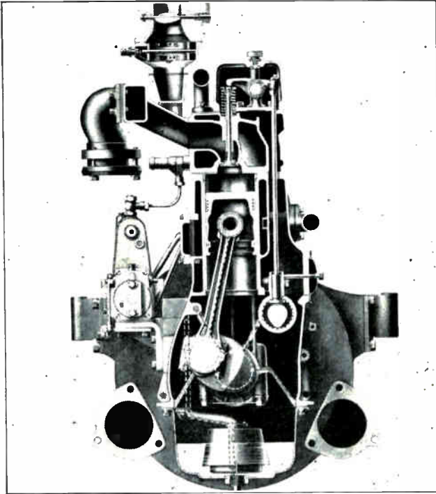
Fig. 121. This end sectional view of one cylinder of a Diesel engine shows by dotted lines the path of the lubricating oil to the main bearings, crank shaft bearings, wrist pin bearings and cam shaft bearings. (Courtesy Buda Engine Co.)
