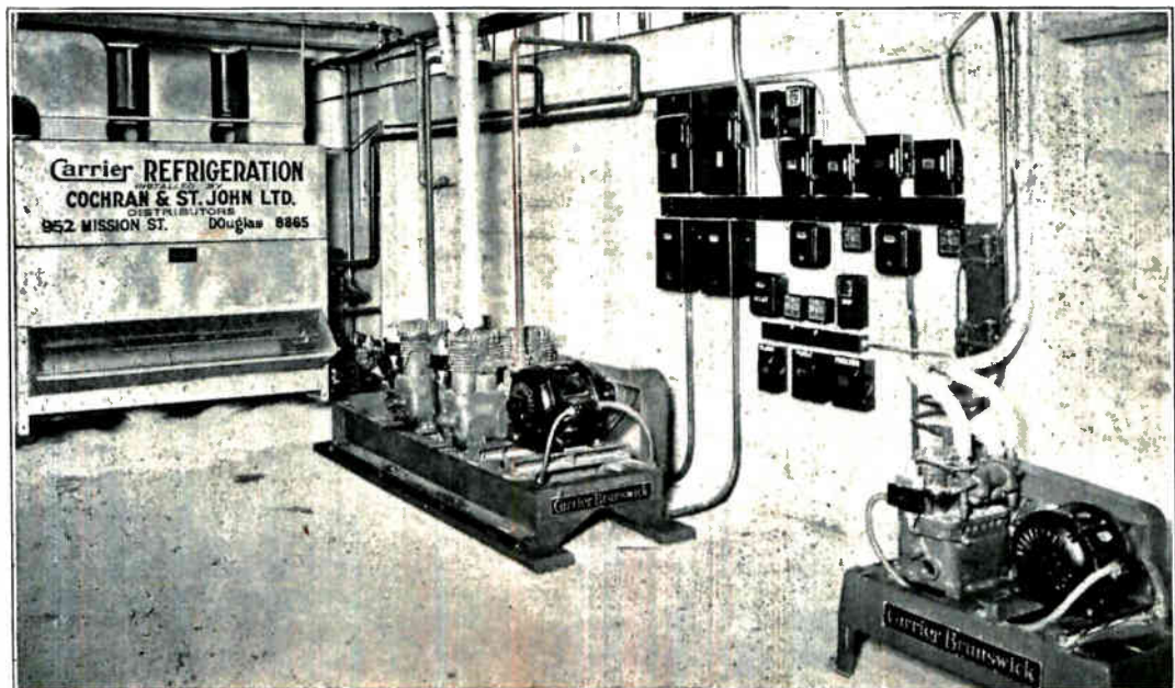
Fig. 91. The above photograph shows a very neat installation of two commercial refrigeration units in the basement of a meat market. The unit on the right is a two cylinder motor driven compressor while the unit on the left has two four cylinder compressors each driven by a separate motor. Note the electrical wiring and switch box installation for these units. Courtesy Carrier Corporation.
