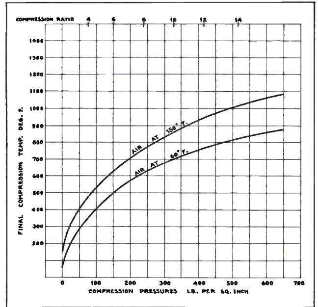
Fig. 27. The above chart shows the relation between compression ratios, air pressures, and temperatures of Diesel-engines.
