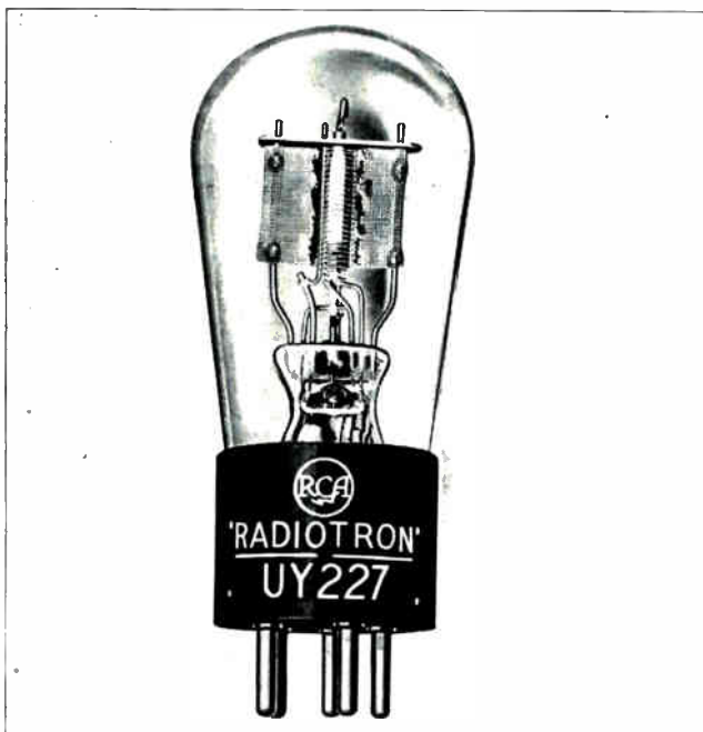
Fig. 80. Photograph of an A. C. heater-element vacuum tube with part of the plate removed to show the grid and the cathode inside of which the heater element or filament, is located. (Photo courtesy of R. C. A. Radiotron Co., Inc.)
