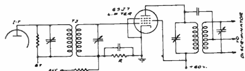
THE LIMITER STAGE IS USED IN F.M. RECEIVERS TO REMOVE VARIATIONS IN AMPLITUDE OF THE FREQUENCY-MODULATED WAVE. LOW PLATE AND SCREEN VOLTAGES ARE EMPLOYED SO THAT THE LIMITER OVERLOADS EVEN WHEN THE INPUT SIGNAL IS WEAK. THE OUTPUT AND TO THE DISCRIMINATOR IS THEREBY MAINTAINED CONSTANT REGARDLESS OF VARIATIONS IN THE STRENGTH OF THE INCOMING SIGNAL DUE TO NOISE OR OTHER CAUSES. THE LIMITER IS NOT USED IN A.M. RECEIVERS.
