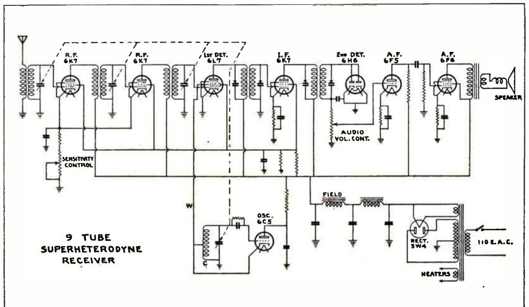
Fig. 158. Circuit diagram of a simple nine tube superheterodyne receiver. Carefully examine and trace all parts of this circuit, particularly the coupling or path of the signals through the R. F. stages, first detector, I. F. stage, second detector, and two A. F. stages. The tube filament or heater circuits are not shown in this diagram.
