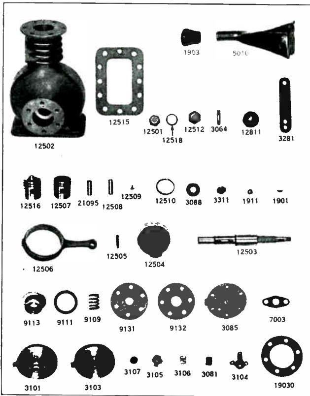
Fig. 92. Above are shown a number of replacement parts for a single cylinder refrigeration compressor. Note the compressor body, pistons, piston pins, piston ring, eccentric rod, eccentric, eccentric shaft, shaft seal, cylinder head, valve plates, gaskets, etc. Courtesy Kelvinator Corporation.
