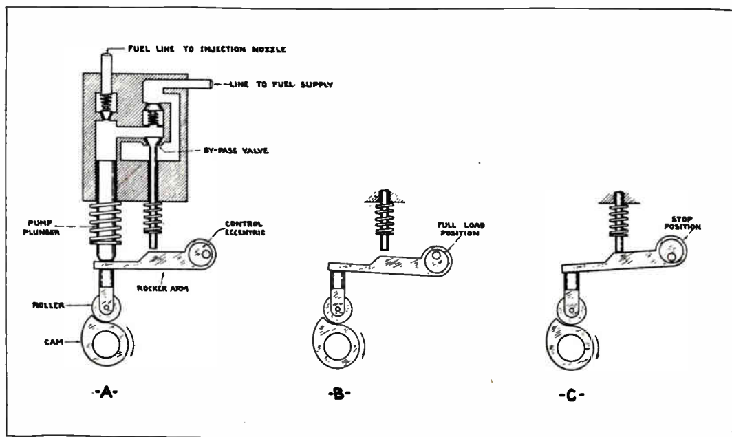
Fig. 34. The figures on the right illustrate the operation of a Diesel fuel injection pump using the by-pass valve method of fuel control. Note how the time of opening of the by-pass valve, and the amount of fuel charge is governed by the position of the control eccentric.
