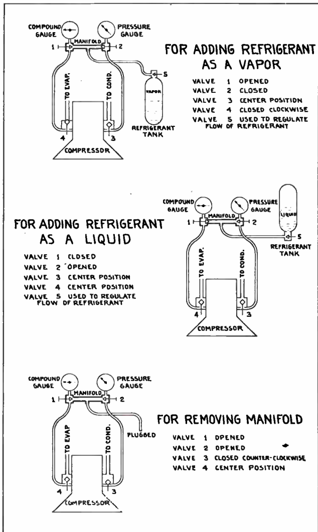
Fig. 109. These diagrams show proper connection of valve manifold, service gauges and the correct valve positions for charging refrigerating systems and for removing the valve manifold.
