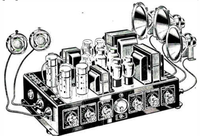
Fig. 230. Another view of a very popular type of P.A. unit showing the power amplifier, power supply transformers, controls, microphones and speakers for a complete installation. Courtesy Radolek Company.
