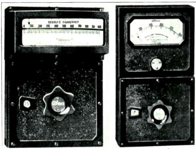
Fig. 105. Two common types of pyrometer meters and switches for panel or switchboard mounting.
