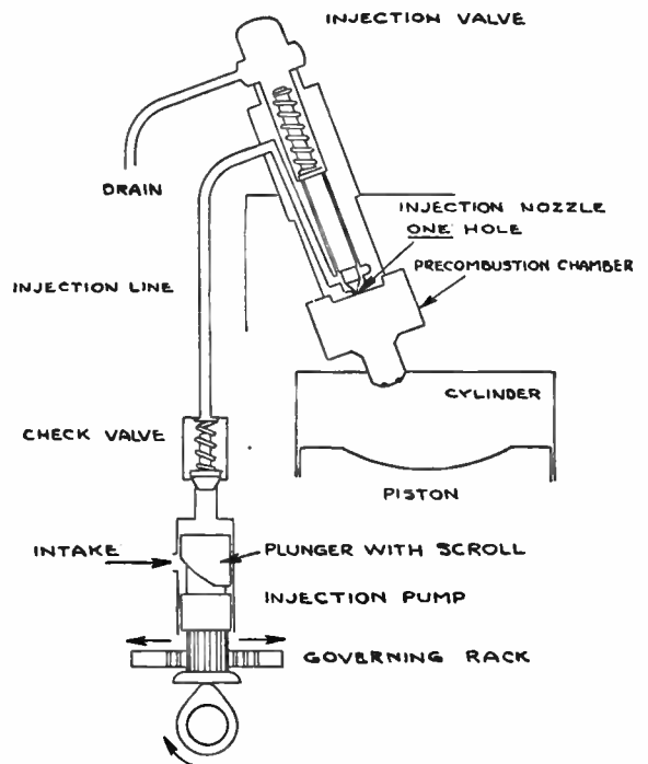
Fig. 32. This sketch shows a single cylinder Bosch constant stroke, variable discharge fuel pump, with check valve, injection nozzle, pre-combustion chamber, and drain line. Refer to this figure often while reading the accompanying explanation. (Courtesy United American Bosch Corp.)
