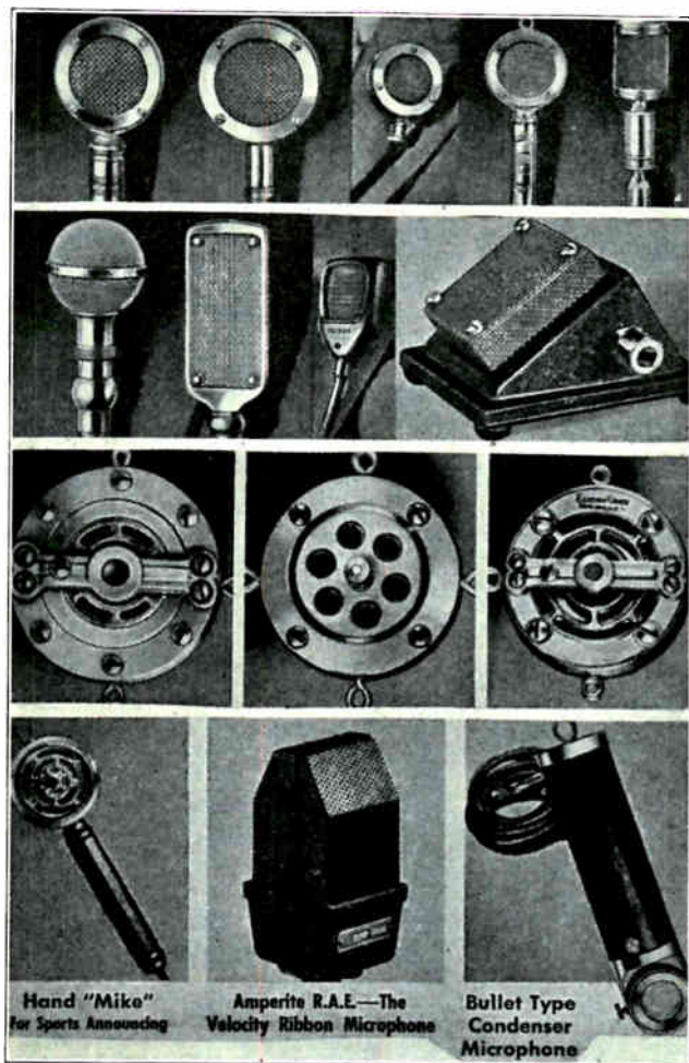
Fig. 242. Above are shown a number of different types of microphones such as commonly used with P.A. systems and in broadcast stations or recording studios. Those in the top row are crystal type microphones, and those in the second row sound-cell crystal type units. The third row shows various views of carbon type microphones and below are shown a portable hand "mike," a ribbon velocity microphone, and a condenser type microphone. Courtesy Montgomery-Ward.
