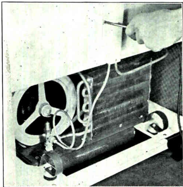
Fig. 94. When removing a condensing unit from the cabinet, be sure to loosen all tubing and wiring so they will not be broken or strained when the condensing unit is pulled out of the cabinet. Courtesy Stewart-Warner Corporation.
