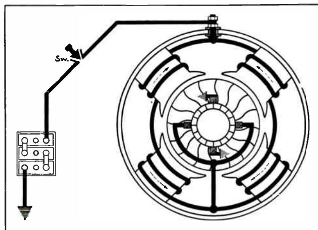
Fig. 63. Diagram showing connections of series wound automobile starting motor. Carefully trace the circuit from the battery through the switch, field coils, armature, and from the grounded brushes back to the battery.
