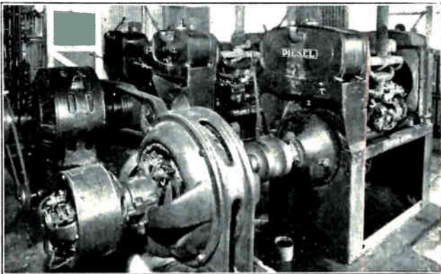
Fig. 68. This photo shows 3 McCormick Diesel engines used for driving electric generators in a small industrial Diesel-Electric power plant. Note the fuel tanks located right on the engine stands. Also note the "V" belt drives used on one generator and the direct shaft coupling on the other unit.
