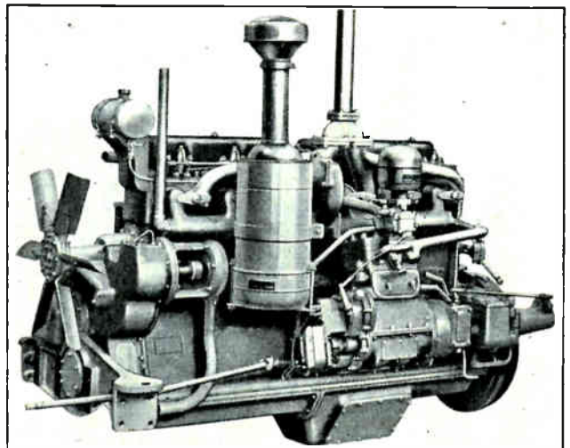
Fig. 74. This view shows a Diesel tractor with a small gasoline engine built right on the side of the Diesel for use in starting. The gasoline engine is first started by hand and then connected to the Diesel engine flywheel by means of a clutch and Bendix drive, thus rotating the Diesel engine until it starts on its own fuel. (Courtesy Caterpillar Tractor Co.)
