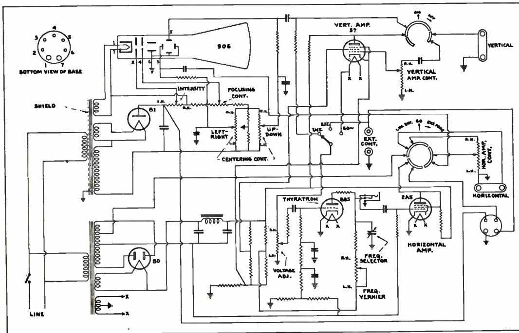
Fig. 252. This diagram shows the complete circuit of a commercial type oscilloscope using a type 906 cathode ray tube. Carefully observe and trace all parts of this circuit including the power supply unit, sweep oscillators, and amplifier.
