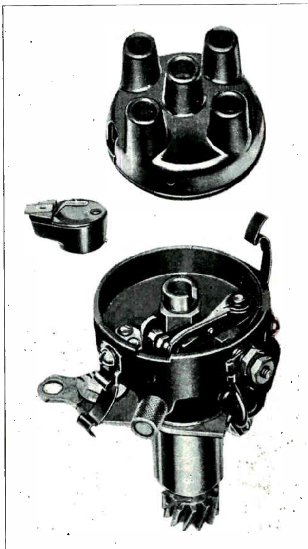
Fig. 34. This view shows a distributor with the high tension cap and rotor removed so that the primary breaker points and cam can be clearly seen in the distributor housing.
