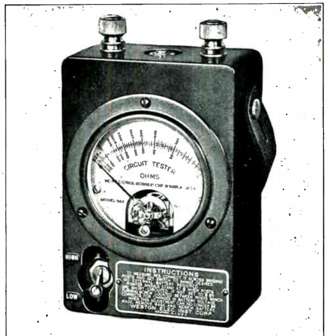
Fig. 197. Convenient Ohmmeter or circuit tester which is also very valuable for continuity testing and radio trouble shooting. (Photo courtesy of Weston Electrical Instrument Co.)
