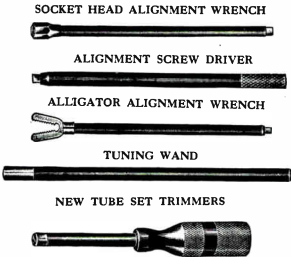
Fig. 170. Several types of aligning wrenches and screwdrivers, and also a tuning wand for aligning "supers."
