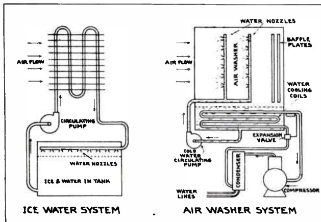
Fig. 150. The diagram on the left shows a simple method of cooling and dehumidifying air by circulating ice water through the finned cooling coil above. On the right is shown an indirect system, using a refrigerator unit to cool water, and then circulating the cold water through spray nozzles to cool and clean the air.
