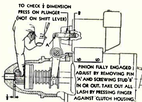
Starter pinion and solenoid plunger adjustment on Delco Equipment.
