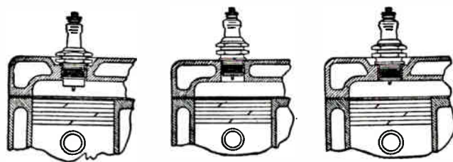
Fig. 31. The above sketches show spark plugs improperly fitted to the cylinder on the left and properly fitted in the cylinder on the right.
