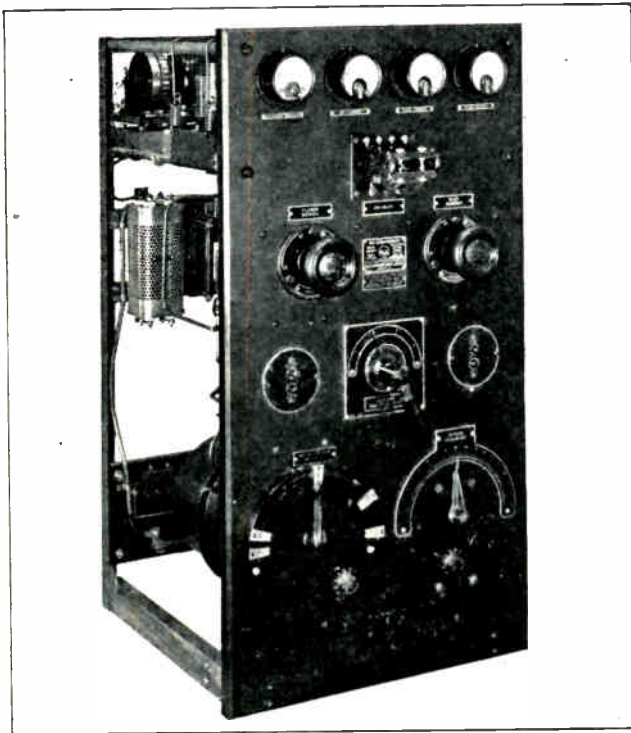
Fig. 272. Front view of a marine type vacuum tube transmitter for use on ships for communication and distress signal uses. Vacuum tube transmitters of this type are rapidly replacing all spark transmitters. (Photo courtesy of Radiomarine Corp. of America.)
