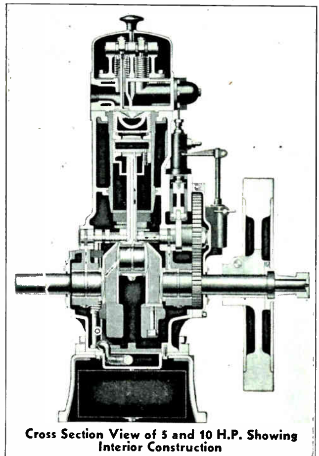
Fig. 4. A sectional view of the same engine shown in Figure 3. Note carefully the construction and arrangement of the cylinder, water jacket, piston, valves, crank-shaft, cam shaft, etc. (Courtesy of the Stover Engine Company.)
