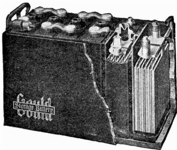
FIG. 4,023—Gould type B storage battery for starting and lighting systems. Plates 4\frac{1}{8} \times 5\frac{3}{4} 7 to 15 plates per cell. Battery units for 6, 8, 12, 16, 18 and 24 volts.
