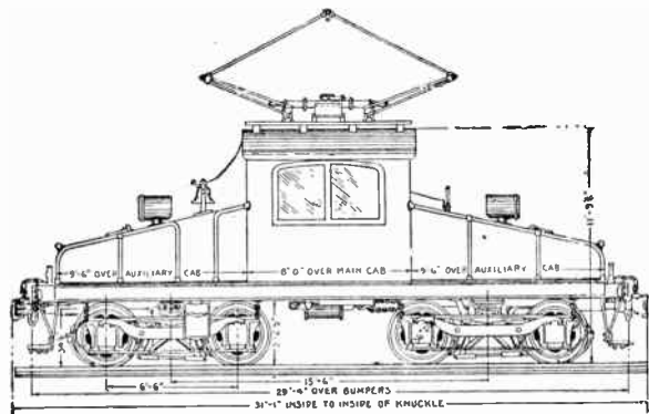
FIG. 3,648.—Baltimore and Ohio 160,000 lb. 0-4-0 locomotive.
