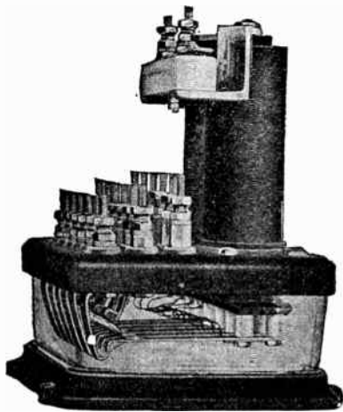
FIG. 3,728. —Slow release neutral relay with six front and back contacts. This relay is equipped with extra large magnets having the slow release feature added as sometimes required by polarized wireless rail circuits when it is necessary to prevent the opening of signal circuits during the reversal of current through the polarized track relay. This slow release relay is also used when line wire circuits controlling annunciators or indicators are used with track instruments or short rail sections to prevent the circuit being opened or closed with the passing of each car.
