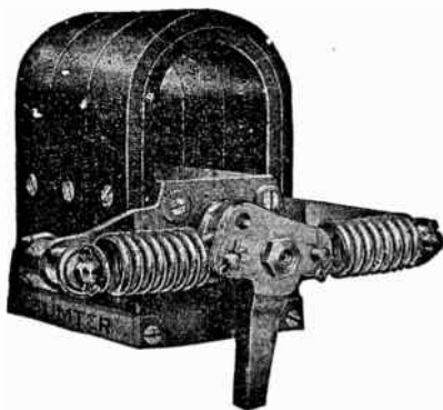
FIG. 3,960. —Sumter low tension oscillating magneto. In this type the armature does not revolve continuously but oscillates back and forth through an angle of about 90°.
