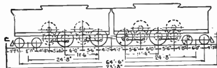
FIG. 3,650.—Combination car and side rod locomotive.
