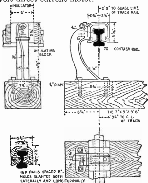
FIGS. 3,509 to 3,512. —Construction details of New York Central Railroad inverted third rail. As shown, the rail is supported from above every eleven feet by iron brackets, which hold the insulation blocks by special clamps. These blocks, which are in two pieces, are 6 \times \frac{3}{4} in., and are interchangeable. Between supporting brackets the upper part of the rail is covered by wooden sheathing, which is applied in three parts and nailed together. At the joints where the third rail is bonded, and at the feeder taps, the wooden sheathing is mortised. This rail is given a little play in the insulators for expansion, except at certain points, where it is anchored. The rail is of special section and composition and has a conductivity of about \frac{1}{2} that of copper. The under, or contact surface is placed 2\frac{3}{4} inches above the top of the service rail, and its center is 4 ft. 9\frac{1}{2} ins. from the center line of the service track, or 2 ft. 5 ins. from the gauge line of the near rail.
