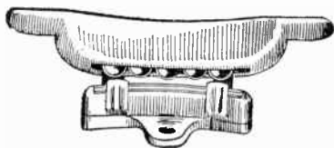
Figs. 3,664 to 3,666. —Center and side bearings. Fig. 3,664 center bearing for city and interurban service; fig. 3,665, side bearing with 9 inch travel; fig. 3,666, side bearing with 12 inch travel for interurban cars operating on short curves. The center and side bearings of a truck form the contact points between itself and the car body. The car body is practically carried on the center plates on the truck bolster and comes in contact with the truck only at this point; but in order to prevent more than a slight displacement of the car body from the vertical, side bearings are placed over the side frames of the trucks, and so adjusted as to leave sufficient space between side bearing top plate and the plate on the car to take up the maximum compression of the springs when the car is fully loaded. It is a fact, however, that owing to a lack of adjustment, or from the displacement of the car body from the vertical when rounding curves due to the excessive elevation of the outer rail, the side bearings on one side may be brought into solid contact with the car body. In order to facilitate the swivelling of trucks when rounding curves ball bearings are frequently used in place of the ordinary bearing plates.
