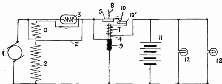
FIG. 4,055. —Diagram showing circuit connection of Rushmore dynamo with automatic cut out. The construction of the cut out is shown on fig. 4,056. The shunt field coil is connected beyond the ballast coil so that it receives current at all times at the constant voltage of the battery, and another winding is added to the field. This is what electricians call a "bucking" coil, that is a coil so connected as to oppose the main shunt field coil. This bucking coil, the effect of which is to reduce the field excitation, is connected as a shunt across the iron ballast coil. Its resistance is considerably greater than that of the ballast coil when the latter is cold or only warm, so that at low engine speeds practically all of the current generated passes directly to the battery and lamps and the machine acts as a simple unhampered shunt dynamo. However, the iron wire will allow only a certain number of amperes to pass, after which it suddenly increases in resistance, so that any excess current cannot pass, but must go through the field bucking coil which thus, only at high speeds, comes into action and chokes down the dynamo excitation. It will thus be seen that the output of the dynamo may be adjusted to any value desired by simply employing an iron wire of suitable diameter in the ballast coil. At car speeds below 15 miles an hour, the dynamo acts as a simple uncontrolled shunt wound machine, while at the higher speeds, owing to the counter effect of the bucking coil, the resultant excitation is less than the excitation due to the main shunt field coil alone. In order to keep the current in the main shunt field coil as nearly constant as possible, it is connected at a point beyond the ballast coil instead of directly across the brushes; then it does not feel the fluctuations of voltage at the brushes. The effect of controlling the bucking coil by the current output is to produce an approximately constant current at the higher speeds. The voltage is determined by the storage battery, and is simply the voltage required to force the specified current against the reverse pressure, plus the small internal resistance of the battery. Assuming the battery to be in good condition, the dynamo voltage will be slightly in excess of the open circuit voltage of the battery, from about 6\frac{1}{4} to 6\frac{1}{2} volts, depending upon the state of charge. The battery is necessary to control the voltage of any automobile lighting dynamo, and must never be disconnected therefrom while the dynamo is in use.
