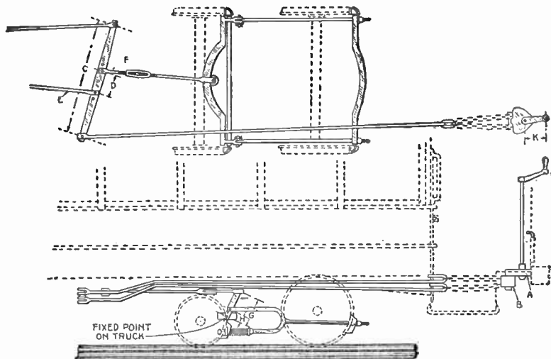
FIG. 3,667.—Geared brake. This apparatus has a pinion A, on the lower end of the brake staff, which engages a gear B, made in one piece with a double sprocket wheel. The two chain loops running through these sprocket wheels engage two hooks formed on the end of the brake rod, or two separate brake rods which are attached at the same point the sway bar. The upper chain is the only one used in braking, the other being left slack and held in reserve for use if the first set fail to work. When the brake is applied to a car mounted on maximum traction trucks as shown, the difference in pressure between the brake shoes on the driving wheels and those on the pony wheels is obtained by means of a spring interposed between the brake system and the pony wheel brake shoes. The dimensions of the different levers are as follows: Length of sway bar C is 48 inches; distance D between pins for the arch bar rods E and F is 9 inches; length truck lever B is 13 inches; and length of horizontal part of brake handle K is 15 inches. With levers of these dimensions a force of 65 pounds applied at the brake handle gives a total braking pressure of 29,000 pounds, or an amount exceeding the weight of an empty car. The best proportion of the lever is secured when, (C + D) \times (G \times H) \times 85k = \text{total weight of the empty car} .
