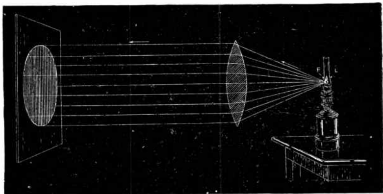
FIG. 3,794.—Effect of placing luminous source at the principal focus of a double convex lens. As the point of light comes near the lens, the convergence of the emergent rays decreases, and the conjugate focus L' (fig. 3,788) becomes more distant. When the source of light L coincides with the principal focus F , as shown above, the conjugate focus is at an infinite distance, that is to say, the emergent rays are parallel. When this condition obtains, the intensity of light decreases slowly, thus, a small lamp can illuminate considerable distance.
