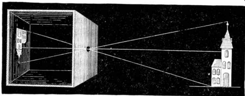
FIG. 3,762.—Images produced by small apertures showing the luminous rays at the aperture causing inversion of the image.
