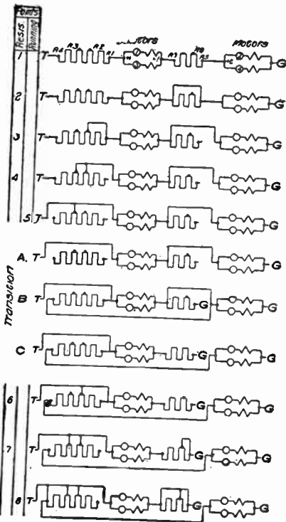
Figs. 3,570 to 3,580.—Diagrams showing control connections of General Electric type K series parallel four motor controller.
