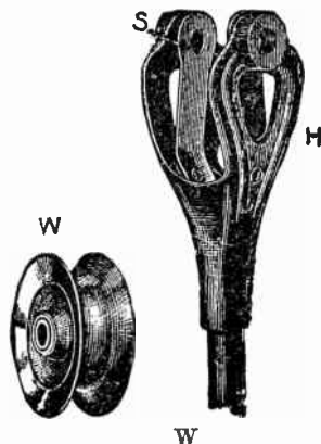
FIGS. 3,501 and 3,502. —Trolley wheel and harp. The word trolley signifies the wheel which is supported at the top of the trolley pole, and which makes rolling contact with the overhead conductor. As shown, the trolley consists of a light wheel W, usually of bronze, supported in a frame or harp H, and revolving freely on a spindle, the latter not shown in the figure. The grooved form given to the wheel not only serves the purpose of securing additional contact surface, but prevents the trolley slipping off the wire. The spring S, pressing against the side of the trolley maintains good electrical contact between the wheel and insulated wire which passes down through the trolley pole to the car. For city service the wheel principally used on the large city systems runs to fairly uniform practice being 4\frac{1}{2} inches outside diameter, with a \frac{3}{4} inch V groove, 1\frac{1}{2} \times 1\frac{1}{2} in., bronze and graphite bushing, and weighing from 2 to 4 lbs.; 1\frac{1}{2} \times \frac{1}{2} in. bushings are largely employed on city roads. For interurban service trolleys of from 4\frac{1}{2} to 8\frac{1}{2} in. outside diameter are used. In general the larger the diameter the greater the mileage. Mr. Chas. A. Ingle, Electric Railway Journal, 1914, states as follows: "For the past year the Rockford & Interurban Railway, Rockford, Ills., has been able to average approximately 10,000 miles on its trolley wheels by getting the maximum possible wear out of them. We use a 6 in., 4 lb. wheel with a \frac{3}{8} in. hollow shaft, for which we pay $1.05. The new wheels are installed in interurban service, and as they wear down are transferred to city car until worn out. We had much trouble at first because the hub would become badly worn before the rim. Now when this occurs we bore out the hub 1\frac{1}{8} inch scant and press in a \frac{3}{8} in. inside diameter, 1\frac{1}{8} in. outside diameter phosphor bronze bushing, which is swaged at both ends with a tapered pin ( \frac{1}{8} in. taper to fit). This makes the bushing tight in the wheel and allows it to run freely on the \frac{3}{8} in. axle. At a cost of 7 cents for labor and material we frequently obtain from 3,000 to 4,000 miles additional life from a wheel, and in all cases we obtain the limit of wear." Other companies report wear from 2,800 miles in interurban service, to 25,000 or 30,000 miles in city service.
