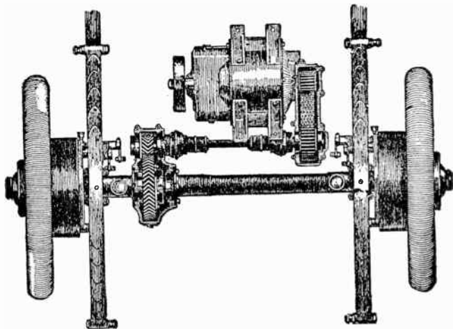
FIG. 4,070.—Waverly double reduction gear or combination herringbone gear and "silent" chain. In construction the motor shaft is parallel to the intermediate or jack shaft and drive shaft. Two universal joints are used, so as to give freedom of motion in any direction. The motor weight is above the springs. The first reduction is by the silent chain enclosed in a casing at end of motor; the second reduction is through the herringbone gear in the axle.
