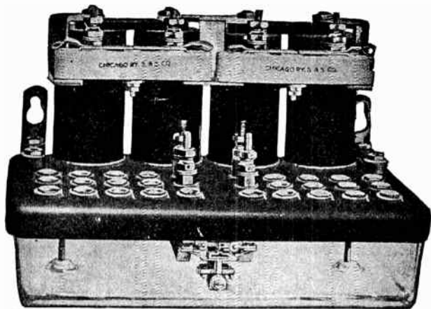
FIG. 3,729. —Glass enclosed interlocking relay; wall type with interlocking contact. Interlocking relays are in reality a combination of two relays in one and are used in connection with two track circuits. The entire operation is actuated by gravity and without springs. Fig. 3,734 shows the interlocking relay connected to the track of an unoccupied block; fig. 3,735 shows the condition of the relay as the train enters it; fig. 3,736 shows the train between the relay connections and fig. 3,737 shows the condition of the relay when the train has passed into a second block
