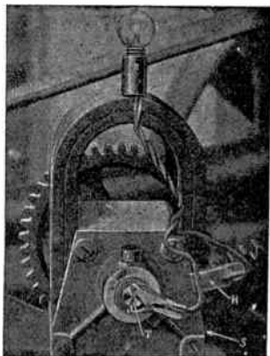
FIGS. 4,012 and 4,014.—Sumter testing device for testing low tension circuits. To test magneto, snap the clips on terminals after disconnecting it from circuit. The condition of magneto is evidenced by the brilliancy of lamp. To test a make and break ignitor, snap one clip on insulated terminal and the other on the engine frame. A little practice enables the conditions to be determined by noting the varying brilliancy of the lamp.
