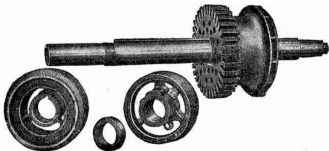
FIGS. 3,534 to 3,537.—Armature construction of General Electric ventilated railway motor. The core is built up of laminations mounted upon and keyed to the armature shaft. The armature is so constructed that the shaft can be removed without disturbing the windings or connections to the commutator. The laminations are punched and assembled with the holes in alignment so as to provide longitudinal holes through the core structure. The pinion end thrust collar has two oil throws, and the commutator end thrust collar, three, so designed as to prevent oil reaching the interior of the motor.
