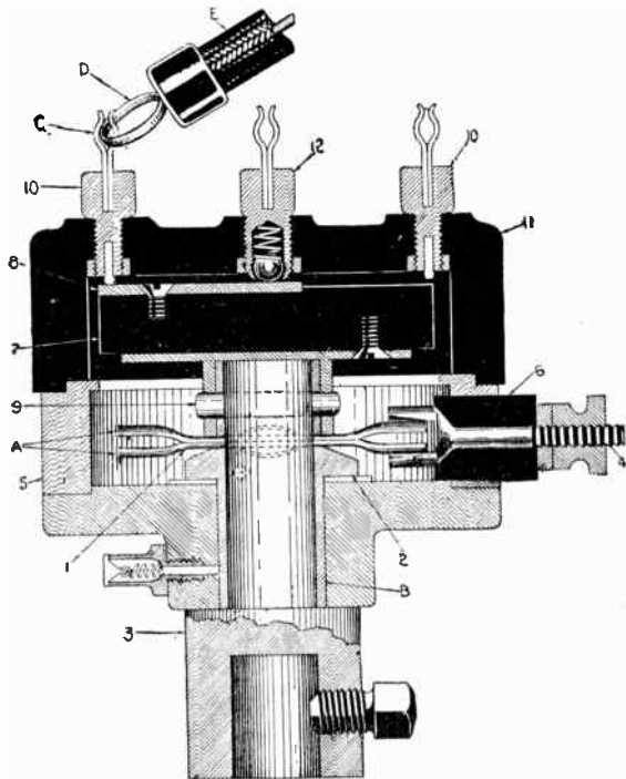
FIG. 3,987.—Sectional view of the Pittsfield distributor. In this device several revolving contacts are employed instead of one; these consist of a double spring making sliding contact at the portions, A. The parts are: 1, contact springs; 2, shaft; 3, bushing; 4, stationary terminal; 5, timer ring; 6, stationary contact insulation; 7, distributor plate; 8, secondary revolving contact segment; 9, taper pin; 10, secondary stationary terminals; 11, casing; 12, secondary terminal for lead to coil; B, slide bearing; C, hook; D, eye; E, secondary cable. The principles of distributor operations are plainly shown in fig. 3,998.
