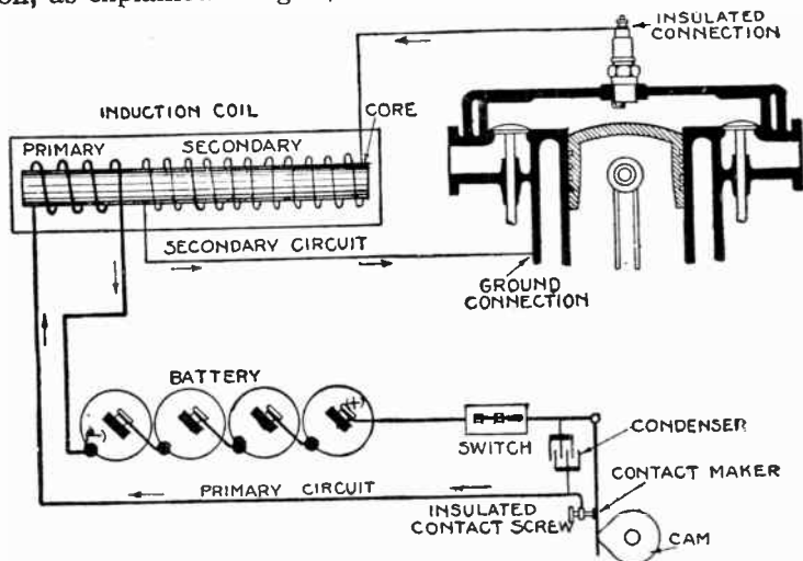
FIG. 3,995. —Diagram illustrating the principles of high tension or jump spark ignition. The nose of the cam in revolving engages the contact maker which completes the primary circuit and allows current to flow from the battery through the primary winding of the coil; this magnetizes the core. The primary circuit is now broken by the action of the cam and magnetic changes take place in the coil which induce a momentary high tension current in the secondary circuit. The great pressure of this current forces it across the air gap of the spark plug and as it bridges the gap a spark is produced. The arrows indicate the paths of the currents. At break, the primary current is "slowed down" by the condenser, thus preventing an arc between contact breaker contacts.
