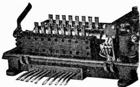
FIG. 3,641. —Westinghouse standard reverser, covers removed. The number of copper fingers mounted on a stationary base, and presence of two sets of movable contact carried on a wooden drum. The forward or the reverse position by one or the other of two pneumatically controlled by a magnet valve similar to those in the switch group. Powering those for operating the switches, are used for moving the reverser on the fingers and firm contacts are thus secured. This construction overload capacity for taking care of heavy current rushes. No reverser cylinders and the drum, when moved to one position by action of the magnets, remains in that position until the circuit of the other. Suitable small fingers mounted upon the reverser frame, and pressing movable contact pieces on the reverser shaft, establish the necessary connections. The reverser parts are built upon a skeleton cast iron frame with sheet iron covers.
