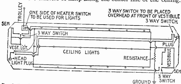
FIG. 3,671. —Car lighting wiring diagram showing head light in series with interior lamps. In this case there are five circuits of four 16 c.p. 110 volt, \frac{1}{2} amp. lamps each, operating on a trolley voltage of 550 volts, therefore, 110 volts from each circuit goes to the head light, thereby giving 2\frac{1}{2} amp. of current which is sufficient for a 80 c.p. incandescent lamp for city cars, or a 2\frac{1}{2} ampere arc lamp for interurban cars. The wiring diagram shows 7 lamps on each side, 4 lamps on the ceiling, one lamp in each vestibule and one lamp for the illuminated sign at each end of the car. A three way switch is located in each vestibule by means of which either the vestibule light, or the sign light at either end may be cut out of circuit, thus keeping only 20 lamps in service at any one time. A three way switch for cutting out either head light is also provided at each end of the car. When neither of the head lights is in use, a small resistance inserted in the ground connection is cut into circuit to take up the 2\frac{1}{2} amperes usually taken by the head light.
