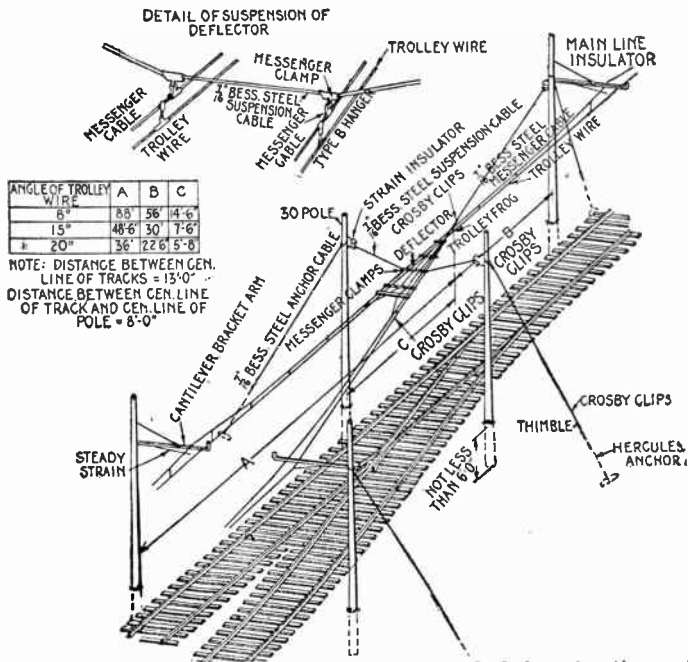
FIG. 3.713. —Trolley deflector construction at switch. The method of construction employed at turnouts and sidings depends upon the type of current collector used. For the wheel trolley, the siding trolley wire is brought to the main line at the switch, and then carried down the main line, parallel to and at a distance of 12 inches from the main line trolley wire, to a distance of about 200 feet. For the pantograph trolley, a so called deflector set is used to prevent the trolley becoming caught. The layout of the poles and line and the construction of the deflector are here shown. The deflector consists of number of trolley wires held in place by ordinary trolley ears which are bolted to cross bars spaced about 3 feet apart and supported by the main line and siding trolley wires. The ends of these rods are raised about 4 or 5 inches above the siding and the main line trolley wires so that no possibility of the ends of the pantograph becoming caught in them. The siding trolley wire is carried over that of the main line to an anchorage on the farther side.
