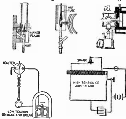
Figs. 3,898 to 3,902. —Various methods of ignition. Fig. 3,898, naked flame; fig. 3,899, hot tube; fig. 3,900, hot ball; fig. 3,901, low tension electric or make and break; fig. 3,902, high tension electric or jump spark.
