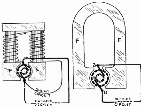
FIGS. 3,949 and 3,950. —Circuit diagrams to illustrate the difference between a dynamo and a magneto. The former has its field magnets FF magnetized by means of a small current flowing around a shunt circuit. In a magneto the field magnets are permanently magnetized. The strength of the magnetic field of a magneto is constant while that of a dynamo varies with the output, hence, a magneto may be run at a widely varying speed and meet ignition requirements, but a dynamo must have its speed maintained approximately constant to keep the voltage within limits.
