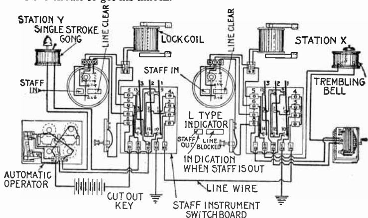
FIG. 3,717. —Wiring diagram of automatic operator system. By using the automatic operator connected as shown, it is possible to operate a staff block without an operator at either station. Twenty dry cells of battery are generally used to furnish current for the operation of each automatic operator. When current is passed through the line the armature is rotated in a direction to cause it to lift the weight on which the normally closed contact is fixed. When current through the line is broken this weight causes the armature to rotate in the opposite direction a sufficient distance to close the other contact and cut in a local battery. Current from this battery passes through a pair of coil holding the armature in this position and releases the staff at opposite ends of the block. When the circuit is again broken, battery is cut off the line.
