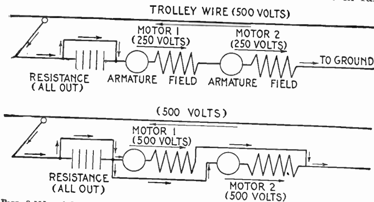
Figs. 3,555 and 3,556.—Diagrams of series parallel two motor control. Fig. 3,555, series running position, all resistance cut out; fig. 3,556, parallel running position, all resistance cut out. When the controller handle is in the series running position, fig. 3,555, the motors are in series, and with a 500 volt trolley circuit, each motor therefore operates at 250 volts. In fig. 3,556, both motors are in parallel under the full 500 volt pressure. The two positives here shown are with resistance all out. A number of intermediate positions may be obtained in both series and parallel positions by progressively cutting out a series resistance. When a rheostatic controller is used with, for example, a two motor equipment, the motors are connected permanently in parallel, and the current divides into two branches, one of which passes through each motor, before they become joined again in a single circuit, passing to the ground. Under this condition the amount of current required by each motor is double that which would be required by one of the motors to move its share of the load. As all this current has to flow through the resistance of the rheostat, the volts dropped in the rheostat constitute a loss, since they do no work, but are wasted in the form of heat. Series parallel operation prevents some of this loss as the motors are in series at starting and the same current which starts one motor passes through and starts the other, thereby taking only one-half as much current from the line as when a rheostatic controller is used. The final or full speed connections are the same in both methods, the motors operating in parallel at the full trolley line voltages with all resistance cut out of the circuit. In selecting a series parallel controller, as in the case of any other similar apparatus, it is important to consider the nature of the circuit, whether wholly metallic or ground return, the number of motor per equipment, and the capacity of each, and the character of the service required of the controller, whether for simple series parallel operation, series parallel control with emergency electric brake, or series parallel control with electric brake for regular operation. The controller should not only be of sufficient capacity, but should be arranged for the number of motor operated. For example: a series parallel controller designed for two 100 H. P. motors is not suitable for an equipment of four 50 H. P. motors, as the reversing switch must have separate connections for each motor. Furthermore, controllers of either the rheostatic or series parallel type for operation with electric brakes for either emergency or regular service should have the necessary contacts and connections for the operation of the brakes.
