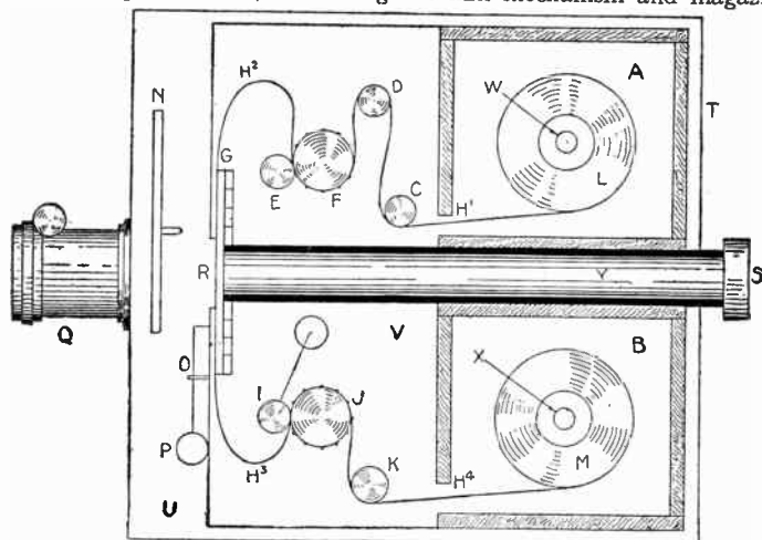
FIG. 3,888. —Diagram of motion picture camera showing the essential parts. Cameras are built for various numbers of picture per turn of the crank; four, six, and eight are common. An eight picture camera should be run at a speed of almost one hundred turns per minute. To operate at this speed, get a watch ticking 300 ticks per minute and learn to count one, two, three; one, two, three, etc., just as fast as the watch ticks, turning the crank one revolution for every one, two, three counted; that is to say, one revolution per every three ticks of the watch.
