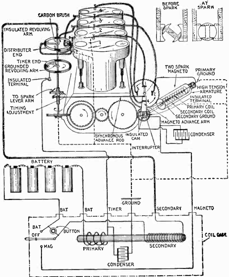
FIG. 3,955 to 3,957. —Double ignition consisting of a two spark high tension magneto system, and a battery synchronous ignition system with engine driven distributor. Fig. 3,955 elementary diagram of connections; fig. 3,956, position of magneto armature just before time of spark; fig. 3,957, position of armature at time of spark.
