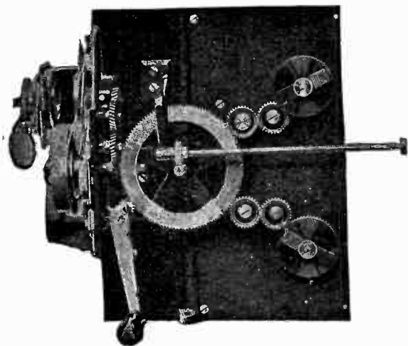
FIGS. 3,893 TO 3895.—Views of Universal motion picture camera. Fig. 3,893 front view showing lens, fly wheel, shutter, and aperture adjustment; fig. 3895, right side showing film channel sprocket wheel and shuttle movement. The adjustable shutter may be set for from 25% to 50% exposure. Under ordinary day light conditions and ordinary speed, 37\frac{1}{2}\% (about \frac{1}{4} th second) is found to be the correct time of exposure; fig. 3,894, left side showing arrangement of take up mechanism and stop picture shaft.
