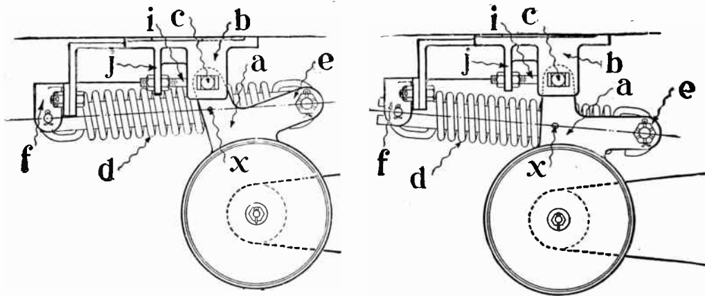
FIGS. 3,674 and 3,675.—Safety Lighting Cc. dynamo suspension. Fig. 3,674, position of dynamo when distance between axle pulley and the suspension is shortened; fig. 3,675, position of dynamo when distance between axle pulley and the suspension is lengthened. In construction there are two carrying lugs a cast on the dynamo frame and which are pivoted to the supporting lugs b on the suspension casting by the suspension bar c . The suspension casting is to be bolted to a suitable plate secured to the car under frame. Belt tension is maintained by the weight of the dynamo and by the tension spring which engages at one end with the lug e on the dynamo frame, and at the other end with the bracket f , fastened to the suspension casting. The parts are so designed that the sum of these two varying factors is constant. When the dynamo is hanging as in fig. 3,675, so that its center of gravity is directly under the supporting bar c , the weight adds nothing to the belt tension, but the spring d has its greatest effect, since the leverage on which the spring acts (the distance between c and x ) is greatest. If the dynamo be swung as in fig. 3,674, the weight of the dynamo is giving tension, but the pull of the spring is decreased as the leverage cx is shortened; the sum of the two tensions being the same as in the first position. Ample latitude is provided between the two extreme positions of the dynamo (figs. 3,674 and 3,675) to take care of belt stretch and the variation in distance between the dynamo and axle when the car is on a curved track. The tension spring is assembled on a carrier under the proper tension, so that to apply it to the suspension it is only necessary to slip the two pins through the holes and in the carrier and corresponding holes in generator lug e and in the suspension bracket f . The arrangement for lining the dynamo with the car axle is simple. The hole in the lug b for the supporting bar c is slotted, and the position of the bar can be adjusted and locked by means of the bolt i which is provided with locknuts on either side of the lug i .
