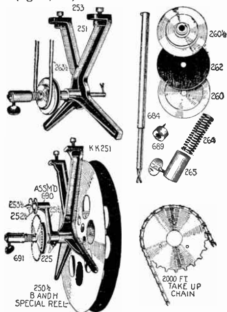
Figs. 3,846 to 3,855. —Simplex take up device. Fig. 3,846 belt drive for small reels; fig. 3,854, chain drive for large reels; figs. 3,847 to 3,853, parts. The take up is the equivalent of the belt drive P, fig. 3,819, that is, it performs the same function, viz.: to rotate at variable speed the lower reel upon which the film is wound. Instead of securing the variable speed by belt slippage, a friction disc clutch is provided. Part 260 is the driving side of the disc and is directly connected to the take up shaft 684. The leather friction washer 262 is 3" diameter by \frac{1}{4} " thick; it operates between friction disc 260 and pulley 260 \frac{1}{2} . The driving pulley 260 \frac{1}{2} , driven by belt 263 \frac{1}{2} , is forced to bear against leather washer 262 by spring 264, which is kept in place by a thimble and set screw 265.
