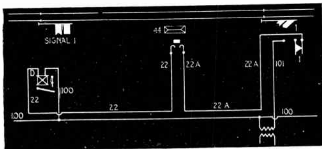
FIG. 3,738.—Advanced block distant signal. In operation when the towerman pulls a lever numbered the same as the distant signal he desires to operate, he completes a circuit between the two springs which causes the distant signal blade to clear.
