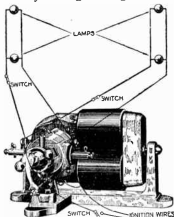
FIG. 3,952.—Motzinger "Auto Sparker" friction drive dynamo. The small friction pulley gives sufficient speed to ignite the charge when engine is turned slowly as in cranking. After the engine is under motion, the governor on the shaft of the dynamo limits its speed so as not to obtain an excessive voltage. This is accomplished by mounting the dynamo on its base so that it can oscillate on an axis, the small friction wheel making and breaking contact with the engine fly wheel. In operation , when normal speed is exceeded, the governor weights fly out and draw the friction wheel away from the fly wheel, one spring serving the double purpose of pushing the friction pulley against the fly wheel and acting as a tension on the governor. By increasing or diminishing the tension on the governor spring by means of a thumb nut provided for the purpose, the speed of the dynamo may be increased or diminished, which in turn increases or diminishes the volume of current and size of spark. By screwing up on this thumb nut the position of the dynamo is not changed, but the contact of the pulley and tension of the governor are increased. Thus, by adjusting the thumb nut, the size of the spark may be regulated at will.
