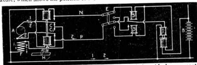
FIG. 3,740.—Diagram illustrating electric interlocking. A switch and lock movement is driven by a direct current motor, the shaft of which is connected by a magnetic clutch to an extension working a cam drum which operates the switch and lock. When the drum is revolved by the motor, first the lock rod and then the switch move in proper operation. After the switch has been moved against the stock rail it is automatically locked and a knife switch throws open the control circuits and closes the indication circuit. The direction of rotation for reversing the switch is controlled by a double field winding in the motor, one part of which is cut out while the other is in circuit.
