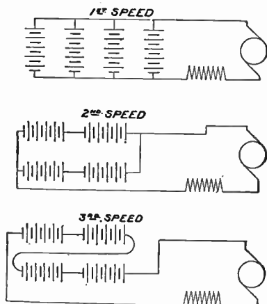
FIGS. 4,105 to 4,107. —Diagrams showing combinations for three speeds in a typical four battery unit, single motor circuit. The only changes made in these circuits are in the battery connections. For the first speed the battery units are in parallel for the second , in series parallel, for the third , in series. The motor connections are not varied.
