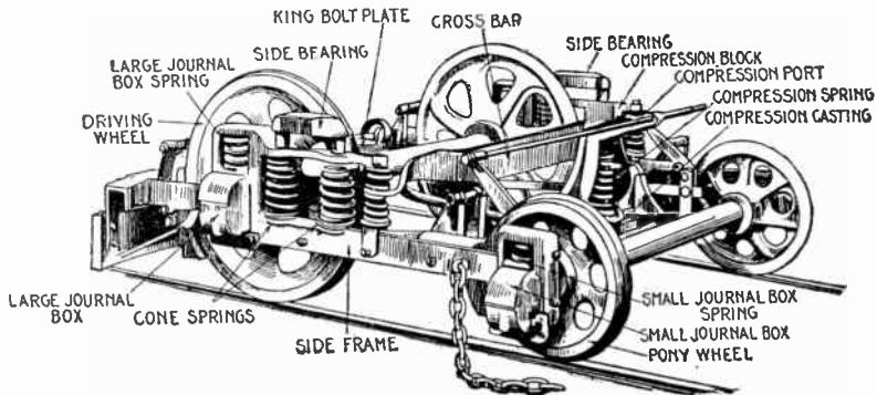
FIG. 3,652.—Brill maximum traction truck. On tangent track 75 per cent. of the weight of this truck comes on the motor axle which has the large wheels. When on a curve, part of this weight is shifted to the trailing wheels. This type is used extensively in city street car service and is not adapted to high speed. One motor is used on each truck.
