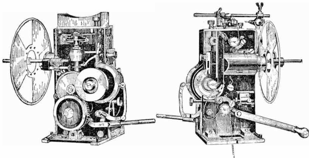
Figs. 3,817 and 3,818.—Simplex motion picture machine. Fig. 3,817 shows the right side with film covers and upper magazine fire valve removed from the top. The valve consists of one large steel roller and two smaller ones which are set at an angle of 45 degrees. They bear against the film top and bottom, and protect the reel from fire. Fig. 3,817 shows also the revolving shutter and shutter mechanism. The three wing shutter shown is used with direct current, but on A. C. circuits of 60 cycles or less a two wing shutter is recommended as it does not intercept the light periods in step with the alternation of the arc. A three wing shutter used with alternating current is liable to get into synchronism with the alternations of the arc and cause a wavy effect in the light similar to a bad flicker. The shutter may be set during operation by turning the knurled knob located alongside the framing handle, thus avoiding ghosts or white streaks. Fig. 3,818 shows right side of machine with fireproof covers removed; it also shows clearly the path of the film through the machine.
