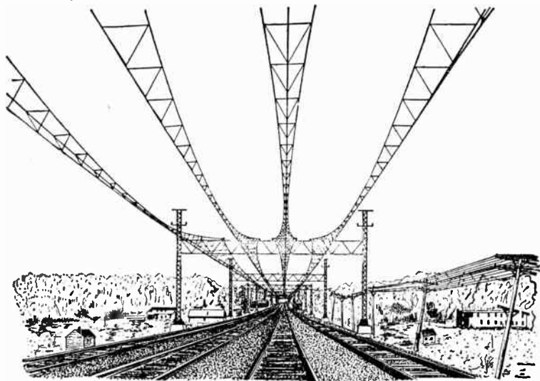
FIG. 3,714. —Four track double catenary construction with bridge supports. In this construction , the trolley wire is carried by two messenger cables supported on bridge of substantial construction spanning the tracks at intervals of 300 feet or more, as here shown. This type of construction represents the highest development of the art of line construction for electric railways. It produces a very rigid structure which is not subject to undue lateral vibration for wind pressure, but is very flexible with regard to vertical pressures exerted by the current collectors. Owing to its great cost, however, it is used only in the electrification of lines of the heaviest class.
