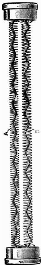
FIG. 3,682.—View showing construction of Gold two coil heater unit. The coils are so designed as to insure a circulation of air. In this heater the coils are wound around wavy metal rods as shown. The smaller coil A provides one-third the heat and the larger coil B, two-thirds, thus making it possible to obtain three variations in the amount of heat furnished, to meet changes in air temperature conditions.
