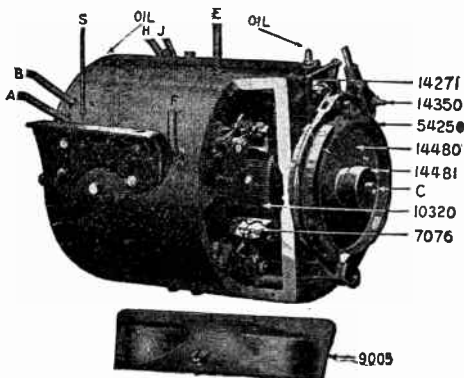
FIG. 4,067. —Raach and Lang electric vehicle motor. Instructions for care of motor: The two oil covers lead to the ball bearings in the motor yokes. A good grade of light cylinder oil is recommended for these bearings. The commutator, 10,320, should be at all times kept clean, free from any gummy or gritty substance. The carbon brushes 7,076 should make perfect contact with the surface of the commutator and should be replaced with new ones when worn out. These brushes are originally 1\frac{1}{8} inches long and should be replaced with new ones as soon as the measurement is reduced to 1\frac{1}{4} inches. It is safer to replace these brushes often, rather than allow them to become too short. Very serious damage may result from using brushes that are too short or ones that make poor contact with the commutator. Brushes that are too short or that are making poor contact will pit, burn and blacken the surface of the commutator. Replacement of brushes should be made only by an experienced person. The motor leads are lead out of motor through insulated holes. These holes, lettered J, H, B, A, S, E and F correspond to the letter contacts on the controller into which they are connected. The motor brake may be adjusted for wear by means of the winged nut 14,350. Clearance between brake jaws and wheel may be adjusted by means of the screw 14,271. To remove brake wheel from armature shaft, take the \frac{1}{8} inch screw C out of the cap 14,481. A \frac{1}{2} inch, 12 pitch bolt, 3 inches or longer, or a cap screw may then be screwed through the threads in the cap and up against the end of the armature shaft. Continue to turn this screw and the pulley will be drawn off the shaft.
