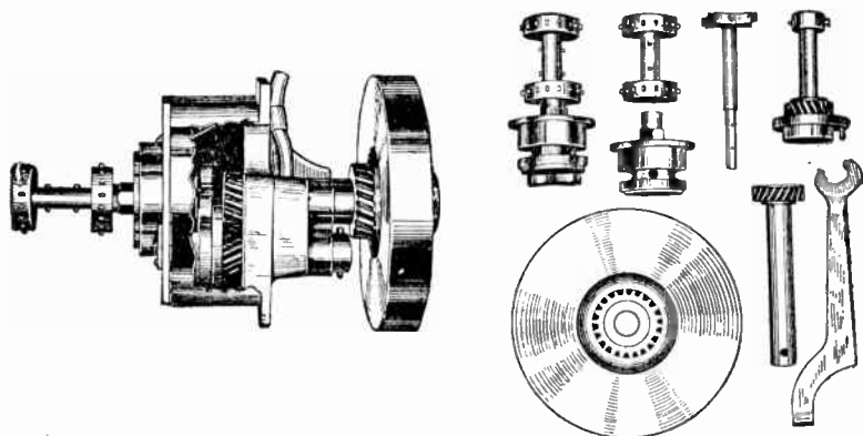
FIGS. 3,827 to 3,835. —Construction details of an intermittent sprocket and intermittent movement. Fig. 3,827, intermittent sprocket and intermittent movement with case broken to show interior; figs. 3,828 to 3,835, parts. The intermittent movement is of the Geneva type arranged to run in oil. The case is in two pieces, consisting of box and screw cover, as shown in fig. 3,827. "Framing" of the film is accomplished by advancing or retarding the intermittent movement by a device for turning the intermittent box forward or backward. The revolving shutter synchronizes automatically by a cam system.
