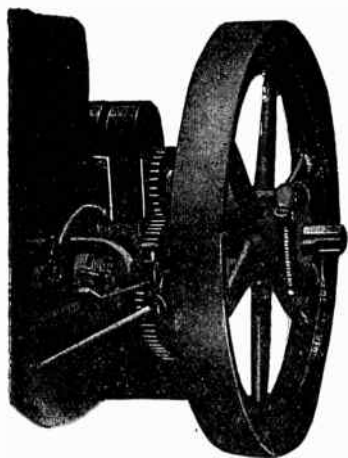
FIGS. 3,961 and 3,962. —Scumter low tension magneto installed on stationary engine, and marking on the ends of shaft and bearing for timing. To time , turn engine over in running direction until igniter snaps; be careful not to turn past this point. With gear on magneto shaft, turn the magneto in running direction until timing mark N on the shaft is in line with mark L, if rotation be left hand, or R, if rotation be right hand. Now mesh the gears, without moving the timing ; this is accomplished by a proper location of the keyway in the magneto gear in relation to a marked tooth on same. The teeth on the engine driving gear meshing with marked tooth on magneto gear should also be marked, and after this marking is once determined all keyways may be cut in proper relation to the marked tooth, thus making all magnetos on the same type of engine interchangeable. These magnetos are usually driven at engine speed, but may be driven at other speeds.
