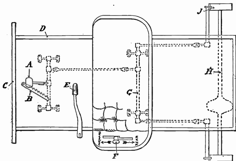
FIG. 4,090. —Diagram of the controlling apparatus of a light electric vehicle. A, brake pedal; B, ratchet retaining pedal in place, operated by left foot; C, dash board; D, body sill; E, steering handle; F, controller handle; G, rocker shaft for setting hub brakes; J, brake band on wheel hub; H, rear axle.
