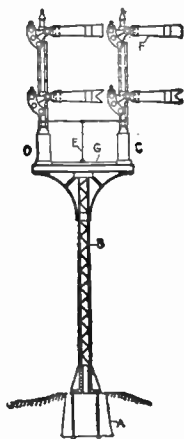
FIG. 3,744. —Three spectacle automatic double route home and distant semaphore signal. The post B consists of two lengths of channel iron strengthened by a lattice structure, the base being bolted to, or incorporated with a foundation of concrete, A. The top consists of a platform G, railing E, semaphores F, being pivoted to short posts and operated by motors and accessories housed in watertight base boxes C D. This arrangement protects two tracks having trains running in the same direction.
