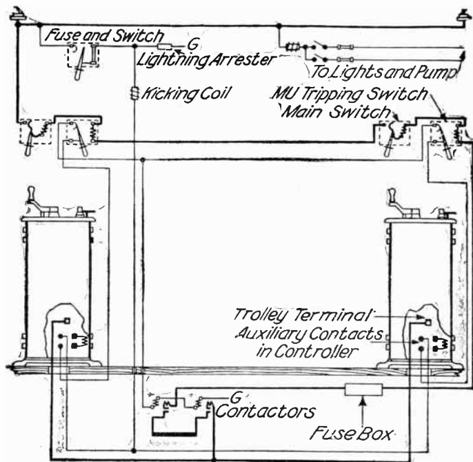
FIG. 3.581.—Wiring diagram of General Electric contactor equipment, designed to eliminate all destructive arcing from the car platform, by opening and closing the main power circuit with contactors located underneath the car body. Two of these contactors are connected in series in the main circuit between the trolley base and the controller and are enclosed in an iron box for protection. Additional contacts are provided in the controller for opening and closing the operating circuit of the contactors when the controller is turned off or on respectively. By this arrangement heavy arcing is avoided at the controller. This equipment also includes overload devices, tripping switches for interrupting the energizing circuit of the contactor coils in case of overload. These switches perform the function of the circuit breakers ordinarily used, and are located in the cab convenient for operation by the motorman. They are adjusted, set and tripped the same as a circuit breaker but only open the small energizing current of the contact coils. A combined switch and fuse is connected in the contactor operating coil circuit. Where the auxiliary contactor equipment is used, the car circuit breakers are usually replaced with non-automatic magnetic blowout switches, for opening the main circuit when desired.
