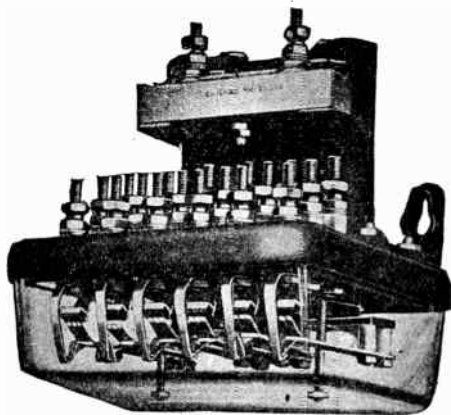
FIG. 3,727. —Polarized relay, wall type, with four front and four back neutral contacts and two front and two back polar contacts. The armature of this relay is itself a permanent magnet and swings back and forth to either pole of the electromagnet as the current attracts and repels it or whenever the polarity of the relay magnet changes.
