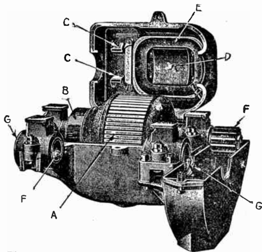
FIG. 3,515.—Direct current railway motor, casing open; as shown, the essential working part of the motor consists of an armature A, with a commutator at B; the brushes C C, which serve to carry the current from the trolley line into and out of the armature; and the four poles between which the armature rotates. One of the poles is shown in the upper half of the casing at D, surrounded by the upper field coil E. The pinion F secured to one end of the armature shaft engages with a gear wheel on the car axle, which passes through the bearings G G, corresponding to the bearings designated E in fig. 3,514.
