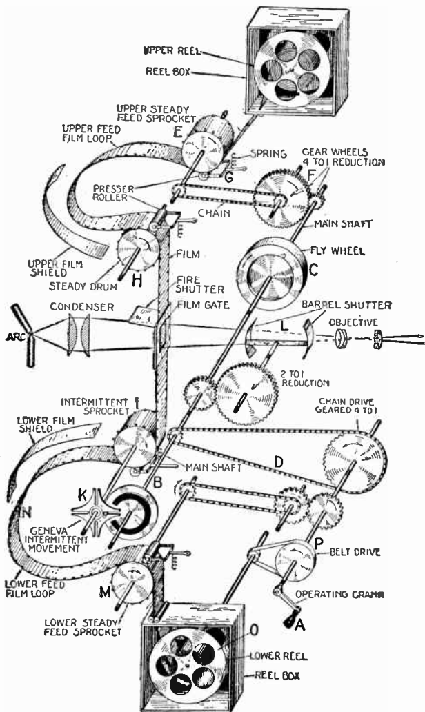
FIG. 3,519.—Elementary moving picture machine without case, showing essential parts.
