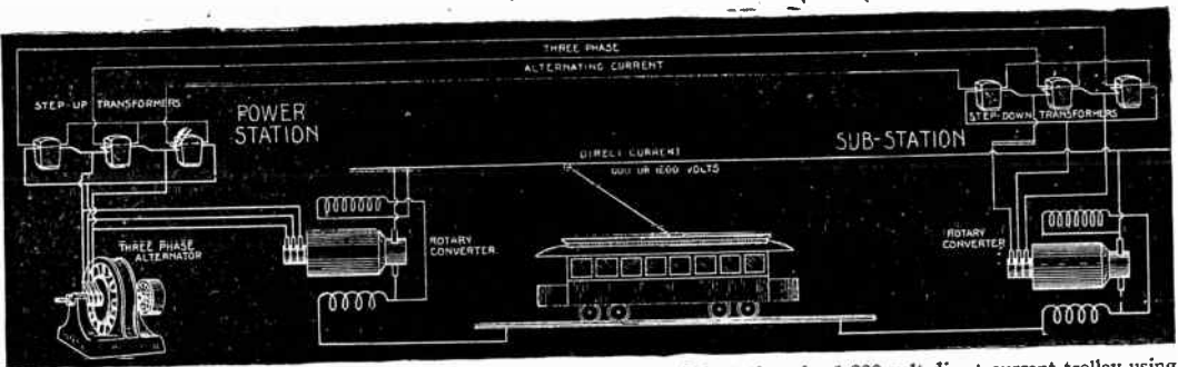
FIG. 3,492.— Alternating current transmission, direct current distribution. Sub-stations for 1,200 volt direct current trolley using two rotaries in series. Alternating current radius depends on the transmission voltage. The system shown consists of three phase 25 cycle alternators, wound for 360 to 390 volts, depending on the direct current voltage desired; step up transformers for raising the generated voltage to the voltage necessary to transmission; sub-stations each having one or more rotary converters, with each converter having a set of three step down transformers for lowering the alternating current voltage to the proper value for reception by the converter for conversion to the proper direct current voltage supplied by it to the trolley, and in some cases the installation of rotary converters in the power station, as shown at A, for taking current directly from the generators without transformation. In cases where a large amount of direct current is required near the power station, and for plants of moderate capacity where the transmission pressure is higher than 13,500 volts it is desirable to have the alternators wound for the low voltage stated; but for cases where the transmission on voltage does not exceed 13,500 volts, the use of the step up transformer may be avoided by winding the alternators for the high voltage; while for cases where the units of power handled at the switchboard exceed 1,500 kilowatts it is almost essential that the generated voltage should be higher than 390 volts. This system may be varied in several ways to satisfy special conditions, for example; 60 cycles may be used where the general lighting circuits are supplied from the same power house, and storage batteries may be installed in the sub-stations for equalizing the demand and reducing the rotary converter capacity necessary to take care of the load. The primary elements of all such installations are practically the same, however, and the sub-stations are usually placed from 10 to 15 miles apart, depending on the character of the road and the traffic.
