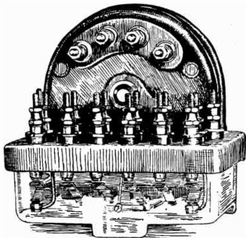
FIG. 3,733. —Interlocking relay for alternating current. The contact springs are glass enclosed. Each armature may be equipped with as many as three extra front and back contacts in addition to interlocking contacts, of which there may be as many as four. It is an improved type of polyphase relay.
