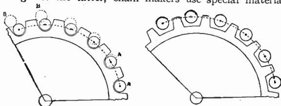
Figs. 4,071 and 4,072. —Diagrams showing the behavior of a chain on a sprocket of equal pitch, and on one of properly unequal pitch. The following quotation from an English authority explains the action: "A chain can never be in true pitch with its sprocket. A pair of spur gears tend, to a certain extent, to wear into a good running fit with each other, but a chain, if made to fit its sprocket when new, does not continue do to so a moment after being made, as wear at once throws it out. This being so, it must be put up with, and involves the consequence that a chain can only drive with one tooth at a time, supplemented by any frictional 'bite' the other links may have on the base of the tooth interspaces. If the chain be made to fit these accurately (taking a roller chain for illustration), it is obvious that the least stretch will cause the rollers AA to begin to ride on the teeth as at BB. If, however, the teeth be made narrow compared with the spaces between the rollers, a considerable stretch may occur without this taking place. The roller interspaces, then, should be long, to permit the teeth to have some play in them, while retaining sufficient strength, as shown in fig. 4,072. In order that the driving sprocket may receive each incoming link of the chain without its having to slide up the tooth face, it should be of a somewhat longer pitch than its chain, the result being that the bottom tooth takes the drive, this being permitted by the tooth play shown in fig. 4,072. This difference, of course, gradually disappears as the chain stretches. The back wheel sprocket, on the other hand, should take the drive with its topmost tooth, and hence should be of slightly less pitch than the chain, but as the pitch of the latter constantly increases, it may be originally of the same pitch. The only remaining point with regard to design, and one which the owner of a car may easily ensure, is that the number of teeth in the sprockets should be prime to that of the links in the chain."
