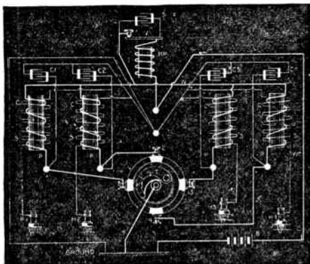
FIG. 3,997. —Circuit diagram of a master vibrator coil. B, is the battery; C, the unit coils; C1, C2, etc., the condensers; P, the primary windings and S, the secondary windings; H1, H2, etc., the spark plugs; T, the timer; MP, the master primary; V, the vibrator; W, the common primary connection; 1, 2, etc., the stationary contacts of the timer. The primary windings are all united in parallel at the top by a wire W, and with the lower winding ends connecting respectively with the segments of the timer T. The primary winding MP which operates the vibrator V is in series with this winding, the wire WT connecting from the battery and passing directly through the master primary MP. The four condensers, C1, C2, C3 and C4, are in parallel with the primary windings. Each of the secondary windings S connects direct to the spark plugs, designated respectively H1, H2, H3 and H4.
