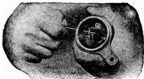
FIG. 3,999. —Filing slot for cleaning platinum contacts of Connecticut magneto interrupter. The cup holding the interrupter or primary circuit breaker may be withdrawn from its housing. The slot serves as a guide for a small flat file for cleaning and squaring the contact points. By means of an adjustable gauge furnished with the magneto, the correct opening of the contact points may be determined. The interrupter is provided with a single roller bearing against the cam pins, thus insuring accurate timing at any speed and unaffected by centrifugal force. The advance lever can be connected at either side of the magneto as the interrupter housing is reversible. The cams are renewable by a half turn with a screw driver.
