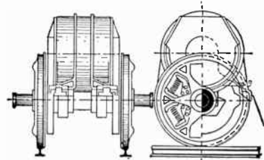
FIGS. 3,529 to 3,533.—Various motor suspensions. Fig. 3,529, New Haven geared motor; fig. 3,530, New Haven gearless motor; fig. 3,531, New Haven topgeared motor; fig. 3,532, Pennsylvania gearless motor with connecting rods; fig. 3,533, geared motors with yoke, or erroneously called Scotch yoke.
