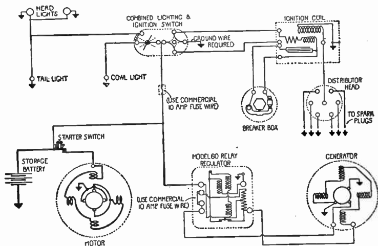
FIG. 3,953.—Wiring diagram of Remy ignition, lighting and starting system as installed on Oakland automobiles. The 6 volt dynamo is a four pole shunt wound machine driven at 1\frac{1}{2} crank speed. A discriminating cut out controls its connection with the battery in charging. The ignition distributor which is a part of the dynamo distributes the high tension current to the cylinders in proper sequence. The interrupter contact points are made of silver.
