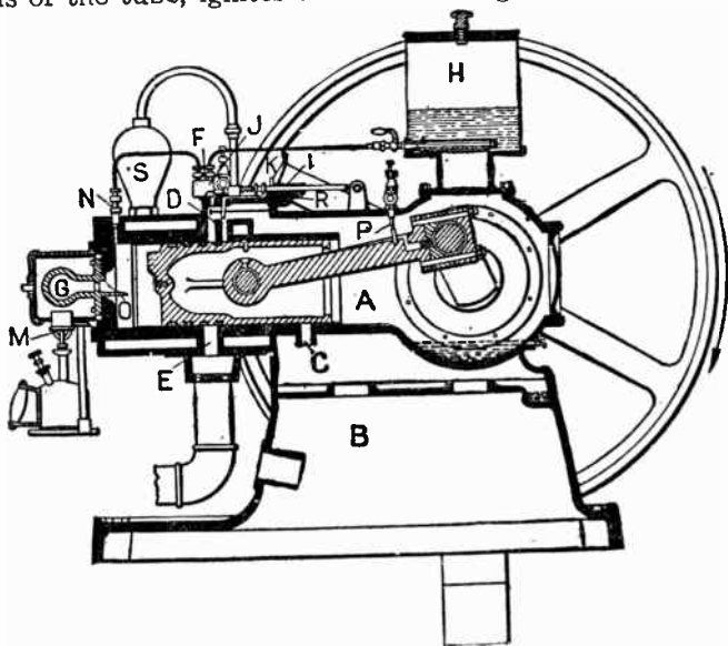
FIG. 3,905. —Meitz and Weiss two cycle oil engine with hot ball igniter. In operation , air is drawn into the closed crank chamber A, from the interior of the base B, through the port C, in the lower part of the cylinder. On the outward stroke of the piston, this air is compressed, and the opening of a port D, by the piston, allows the air, together with the steam generated in the water jacket, to pass into the combustion space of the cylinder. At the same time, the exhaust port E, having been overrun, and thus opened by the piston, discharges the products of combustion of the previous charge into the exhaust pipe. The fuel is injected into the cylinder by the pump F, and mixes with the air and steam previously admitted from the crank chamber, so that on the compression stroke, the charge is automatically ignited by contact with the heated walls of the hollow igniter ball G. This ball, made of cast iron, is located in the projection attached to the cylinder head, as shown. A charge is compressed at every revolution of the crank shaft, and compressed by the piston into the compression space of the cylinder and the interior of the igniter ball where it is ignited. Before starting , the igniter ball is heated for a few minutes by a small oil jet from the burner M. The oil jet from the injection nozzle N, strikes the projection O, extending from the igniter ball and is sprayed, vaporized and mixed with the air and steam in the compression space. The igniter ball is maintained at a dull red heat by the heat of the explosives.
