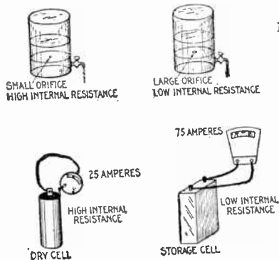
FIGS. 3,942 to 3,945.— Hydraulic analogy of internal resistance. Figs. 3,942 and 3,943 show two tanks (cells) both having discharge pipes (external circuits) of practically no resistance. The internal resistances of the tanks are represented by a large and small orifice through which the tanks must discharge. It is evident that the flow in one case will be high, and in the other case low, corresponding to initial currents of cells of low and high internal resistances. It is certain that on ordinary work either of these tanks would give equally good service if the flow required be less than the initial flow of the high resistance tank. This is true of dry cells. The required drain in any kind of work is less than the lowest initial current; hence, a low current cell may give just as good or better service results than a very high current cell.
