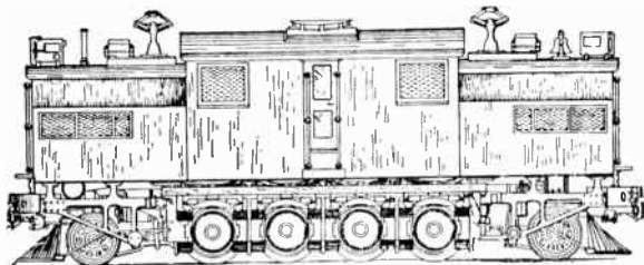
FIG. 3,647.—New York Central 1-4-1 locomotive.
