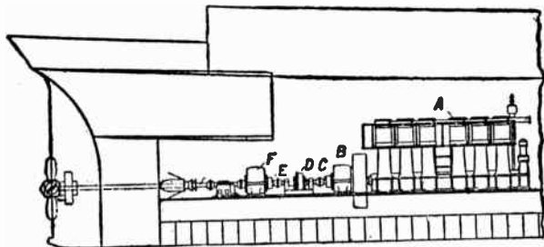
FIG. 3,758. —The Menlees system of propelling ships by gas engines. In the figure A is a six cylinder gas engine coupled to a dynamo B. The shaft C of the dynamo and engine is adapted to be connected by a clutch D with the shaft E of the electric motor F, which is connected with the propeller shaft. In operation , at all ahead ship speeds direct driving may be employed, but, for speeds less than half, the electrical transmission may be used, the motor F, receiving electrical energy from the dynamo B. The drive may also be employed for reversing the astern speed by not greater than half the full ahead speed, suitable switches and gear being provided.
