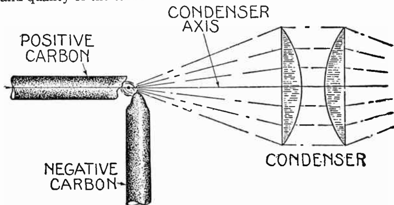
FIG. 3,860. —Stereopticon arc for direct current. This setting does not give as brilliant an arc as fig. 3,859, when a long arc is used, but for a short arc the carbons become so near that an arc of more brilliancy than fig. 3,859 is obtained.
