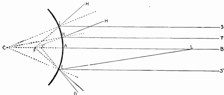
FIG. 3,791.—Foci of convex mirrors. This type of mirror has only virtual foci. Let SI, and TK be rays parallel to the principal axis of a convex mirror. These rays, after reflection, take the diverging directions IM, KH, which, when continued, meet at a point F, which is the principal virtual focus . In the triangle CKF, it may be shown, in the same manner as with concave mirrors, that the point F is approximately the center of the radius of curvature CA. If the incident luminous rays, instead of being parallel to the axis, proceed from a point L, situated on the axis at a finite distance, a virtual focus will be formed at a point L' , between the principal virtual focus and the mirror.
