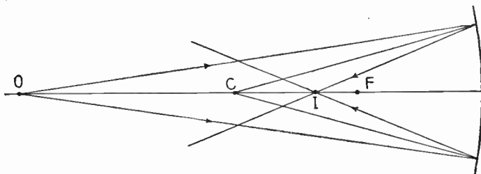
FIG. 3,787.—Conjugate foci. By definition, when two points are so related that object and image may exchange places, they are called conjugate foci. If a luminous object be placed at the point O, it projects divergent light rays upon the mirror. These rays will focus at a point I, a little further from the mirror than the principal focus F. If the source of light be now placed at I, the rays will pass back over the same paths and will come to a focus at O; the points I and O thus related to each other are called conjugate foci . Concave mirrors make divergent rays less divergent, parallel or convergent; parallel rays, convergent; convergent rays more convergent.
