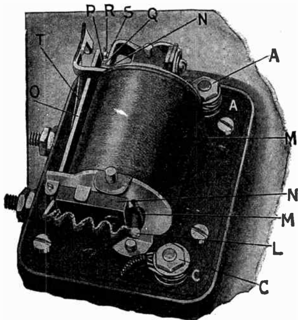
Fig. 4,046.—Wagner cut out of two unit starting and lighting system. It consists of two magnet coils L and M, wound on an iron core N, which attracts and repels an iron lever O. At the end of O are two main contact points P and Q at which the contact between the dynamo and battery is made and broken. There are also supplied two auxiliary contact points R and S which are for the purpose of minimizing sparking at the main contact points P and Q. The coil M called the shunt coil is connected directly across the two brushes H and I, and therefore the full dynamo voltage is impressed across the ends of this coil. The coil L, called the series coil , is connected in series with the battery and dynamo and therefore this coil carries the charging current when the battery is being charged. In operation , when the engine is started, the dynamo is driven by the engine and it, therefore, increases and decreases in speed with the engine. When the engine is speeded up, the dynamo follows with corresponding increase in speed and the voltage of the dynamo rises as the speed increases. As soon as the dynamo voltage gets to a point above the voltage of the battery, which is approximately six volts, the coil M pulls the iron lever O toward the magnet core, thereby closing the contact at the points P and Q-R and S. As soon as this contact is made, the dynamo is connected to the battery, and a charging current will flow from the dynamo to the battery through the series coil L, which is in series with the dynamo and battery. The dynamo continues to charge as long as these contact points P and Q-R and S remain together, but when the engine speed is decreased, so that the dynamo voltage falls below the battery voltage, the battery will discharge through the dynamo and therefore through the coil L. This discharge current, being in the opposite direction from the charging current, will neutralize the effect of coil M and allow the spring T to pull lever O away from the magnet core, thereby opening the contact at the points P and Q-R and S. As soon as these contacts open, the battery is off charge. The engine speed at which this relay closes corresponds to a car speed of 7 to 10 miles per hour.
