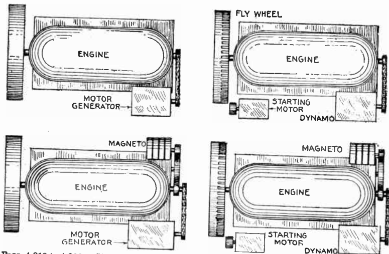
Figs. 4,019 to 4,022.—Classes of starter systems. Fig. 4,019, one unit system; fig. 4,020, two unit system; fig. 4,021 so called two unit system; fig. 4,022, so called three unit system.
