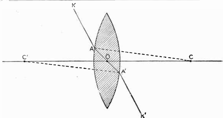
FIG. 3,796.— Optical center. Let two parallel radii or curvature CA and C'A' be drawn to the two surfaces of a double convex lens. Since the two plane elements of the lens A and A' are parallel, as being perpendicular to two parallel right lines, it is evident that the refracted ray AA' is propagated in a medium with parallel faces. Hence a ray KA , which reaches A at such an inclination that after refraction it takes the direction AA' , will emerge parallel to its first direction. The point O at which the right line cuts the axis is therefore the optical center. The position of this point may be determined from the case in which the curvature of the two faces is the same, which is the usual condition, by observing that the triangles COA and C'OA' are equal, and therefore that OC = OC' , which gives the point O . If the curvatures be unequal, the triangles COA and C'OA' are similar, and either CO or C'O may be found, and therefore also the point O . In double concave or concavo-convex lenses, the optical center may be determined by the same construction. In lenses with a plane face, this point is at the intersection of the axis by the curved face.
