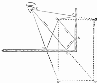
FIG. 3,768. —Multi-image formed by two mirrors. When an object is placed between two plane mirrors, which form an angle with each other, either right or acute, images of the object are formed, the number of which increases with the inclination of the mirrors. If they be at right angles to each other, three images are seen, arranged as represented in the figure. The rays OC and OD from the point O, after a single reflection, give the one, an image O', and the other an image O'', while the ray OA, which has undergone two reflections at A and B, gives the third image O'''. When the angle of the mirror is 60°, five images are produced, and seven if it be 45°. The number of image continues to increase in proportion as the angle diminishes, and when it is zero (mirrors parallel), the number of image is infinite. In general , if two mirrors be inclined to each other, the number of image they produce is equal to the number of times the angle between them is contained in 360.
