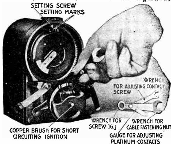
Figs. 3,978 and 3,979. —Eisemann type G4 magneto showing method of timing and special wrench. Timing the magneto: As the spark occurs when the primary circuit is broken by the opening of the platinum contacts in the make and break mechanism, it is necessary that the magneto will be so timed that at full retard position of the timing lever body, the platinum contacts will open when the respective piston of the engine has reached the top point on the firing stroke. Turn engine by hand until piston of No. 1 cylinder is on the upper dead center; remove distributor plate from magneto and turn the driving axle of the armature until the setting mark on the distributor disc is in line with the setting screw as shown. (For clockwise rotation use mark R, for counter clockwise, use mark L). With the armature in this position, the platinum contacts are just opening, and the metal insert of the distributor disc is in connection with carbon for No. 1 cylinder. The driving medium must now be fixed to the armature axle without disturbing the position of the latter, and the cables connected to the spark plugs.
