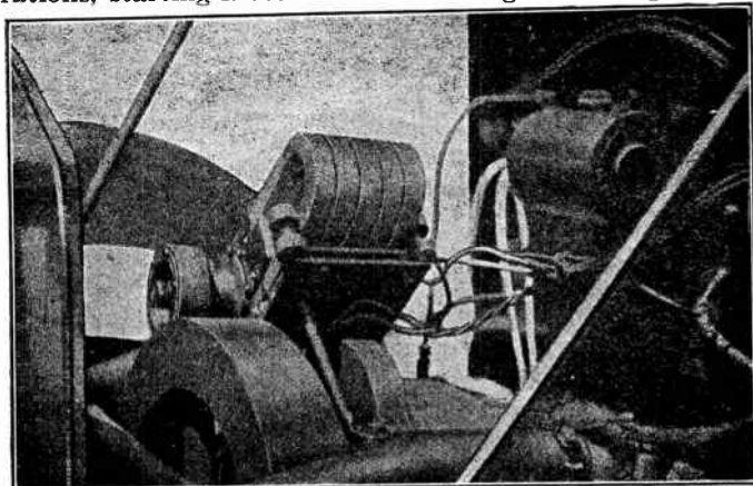
FIG. 4,030. —Method of driving a generator direct from engine fly wheel by friction pulley with spring or cushion base; the latter relieves the stress on the shaft from excessive vibration. The governor regulates the speed of the machine and prevents burning out of the lamps. The illustration shows a K-W magneto installed on an early Maxwell car.
