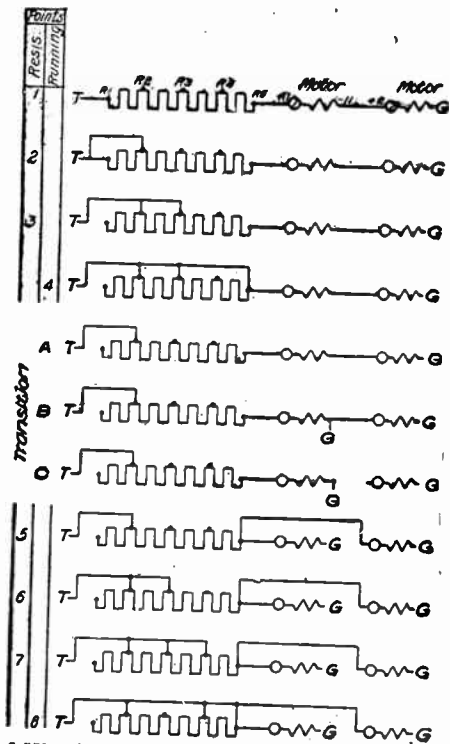
Figs. 3,559 to 3,569.—Diagrams showing control connections of General Electric type K series parallel two motor controller.
