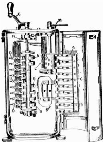
FIG. 3,548.—Ordinary rheostatic controller, designed to control one or more motors by means of resistance only. As shown, it consists of a switch cylinder A, carrying nine insulating supports upon which are mounted nine metallic conducting segments B, B, B. These segments differ in length and position, and when the cylinder is turned by means of the handle C, they come in contact at different times with the nine fixed contact springs D, D, D, which effect the changes in the connection by which more or less resistance is brought into or out of the motor circuit, thereby producing a change in the speed of the car. It is evident that after contact has been made between the motor and the trolley, an electric arc, very destructive to the breaking contact within the controller would be established unless some means were provided for breaking the arc at the instant of its formation. This is accomplished by means of a magnetic blow out device consisting of the magnet E and its pole piece, carrying the polar ridges G, G, G, which rest close to the contact springs D, D, D, when the pole pieces are placed in normal position. In operation, the current passing through the motor passes through the coils of the magnet E, and converts its core into an electromagnet which produces a powerful magnetic flux around the contact surfaces of the springs D, D, D. At the instant the circuit is broken either in changing connections or when the current is entirely shut off, the irresistible influence of this powerful magnetic flux prevents the severe sparking which would naturally occur otherwise by blowing out the arcs as soon as they are formed. The reversing cylinder H, carries four conducting segments K, and a corresponding number of contact spring L. By moving the handle M through an arc of about 60 degrees, the segments in contact with the springs L, can be changed and the direction of the current through the armature of the motor reversed, thereby causing it to rotate in the opposite direction and back the car. As the reversing operation cannot be safely accomplished while the motor is running, the handles C and M are made interlocking so that the latter cannot be moved unless the former be in the "off position." In other words the current must first be shut off before the direction of the car can be reversed. This prevents any arcing on the contacts of the reversing cylinder. The proper operation of a controller requires that all the successive contacts be made and none omitted. This is insured by the action of the star wheel located at N. Rheostatic controllers may be used for single motor railway equipments, single or double motor mining equipments, and for crane, etc. It is important to have a full knowledge of all the requirements of any particular service before selecting the controller. For service requiring frequent motor reversals, a controller with a single handle, with the motor circuits so arranged as to perform the function of the reverser, is found more convenient than a controller with a separate reversing handle. Controllers with single handles are usually employed to operate travelling cranes, turn tables, stationary and portable hoists, etc., while those having two handles are generally used with street railway and mining equipments.
