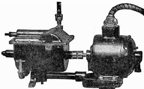
FIG. 3,885. —The arc controller or device designed to control the rate of feed of the carbons of an arc lamp, with the object of maintaining at all times a predetermined size of arc. It consists of the controller proper, direct coupled to a fractional horse power motor. There are two shafts, primary and secondary. The former, which is direct coupled to the motor, carries governor parts, and rotates constantly at the motor speed. The secondary, to which the telescope rod is geared, remains idle until the speed of the primary shaft exceeds the point of adjustment. The adjustment for any preferable size of arc is made with a brass adjusting nut upon a rod projecting from the cover of the controller. The inner end of the rod is connected through a heavy wire spring to a pawl, the function of which is to "step in" and transmit the power to the primary, through differential gearing to the secondary shaft, at the slightest tendency of the arc to become wider than the predetermined size adjusted for. The installation of the arc controller does not interfere with any of the lamp adjustments already provided. The operator may trim as he pleases, and feed by hand if he choose, by loosening a thumb screw at the feed handle gearing. Having loosened the thumb screw and trimmed the lamp, the operator strikes the arc by hand and makes the original and only feeding adjustment, by parting the carbons to the size of arc that he wishes to maintain; he then tightens thumb screw, and sets adjusting nut at the controller so that feeds do not occur below that size; the controller will then feed the carbons to that certain size of arc without further attention. To increase size of arc, tighten adjusting nut; to decrease size, loosen nut.
