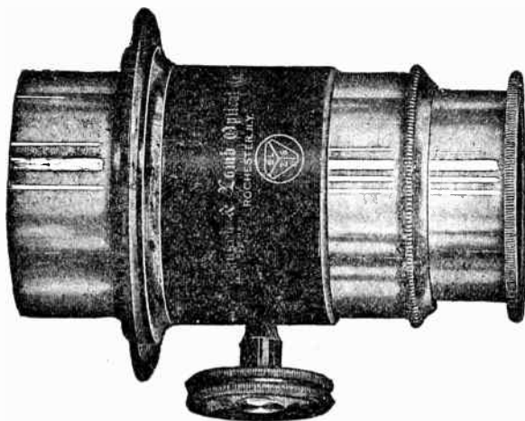
FIG. 3,814. —Bausch & Lomb standard projection lens. It consists of two combinations fitted into a cell and mounted in a brass tube which slides through a brass tube or sleeve. The focusing is by rack and prism, as shown. Connection is made for spherical and achromatic aberration. Equivalent focus 2\frac{1}{2} to 32 inches, and back focus 1\frac{1}{4} to 30 inches; corresponding diameter of lenses 1\frac{1}{8} to 2\frac{1}{16} .
