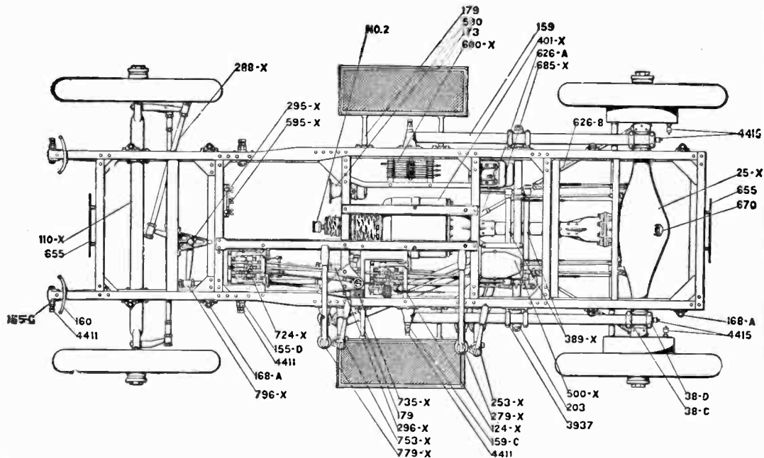
FIG. 4,060.—Plan view of Bakcr electric chassis. The parts are: 25-X, rear axle; 38-D, rear spring yoke rear; 110-X, front axle; 124-X, front levers, rear; 155-C, front spring bolt, front; 155-D, front spring bolt, rear; 159, rear spring; 159-C, rear spring bolt; 160, head lamp bracket; 168, A, fender bracket; 173, step pad; 179, step bracket; 203, rear spring seat, center; 253-X, rear control mast; 279-X, steering mast, rear; 288-X, lower steering rod, mast to mast; 296-X, lower steering rod, bell crank to spindle; 295-X, bell crank; 296-X, lower steering rod, mast to mast; 389-X, brake shaft; 401-X, motor; 500-X, controller; 590, horn; 595-X, fusc box; 600-X, resistance; 626-A, brace rod clevis; 626-B, brace rod; 655, license bracket; 670, oil inlet; 685-X, contactor; 724-X, foot levers, front; 735-X, interlock; 753-X, front control mast; 779-X, steering mast, front; 796-X, lower steering rod, mast to bell crank; 3,937, rear spring clip; 4,411, 4,415, No. 2 grease cups.
