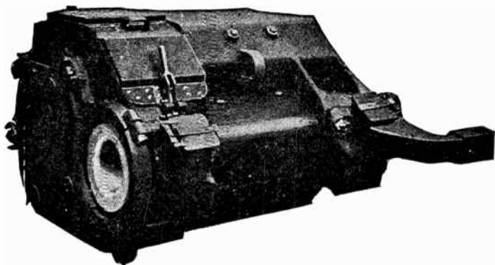
FIGS. 3,751 and 3,752.—Westinghouse interpole motor as used on Piedmont railway. Fig. 3,751 pinion end of motor; fig. 3,752 commutator end. The motor is rated at 110 horse power at 750 volts. Two motors are connected in series for 1,500 volt operation. These motors are geared to 36 inch wheels with a 20 tooth pinion and 57 tooth gear. The cars, weighing complete without load, approximately 41 tons, are operated at a schedule speed of 34 miles per hour. The weight of the motor complete is 4,150 pounds. The armature is especially designed to withstand the higher voltage, being insulated with mica, and having liberal creepage distances provided at the end of the commutator. The brush holders have extra heavy porcelain insulators. The length of the dust ring at the end of the commutator, and the clearances from the line parts of the motor to the ground are greater than in ordinary designs.
