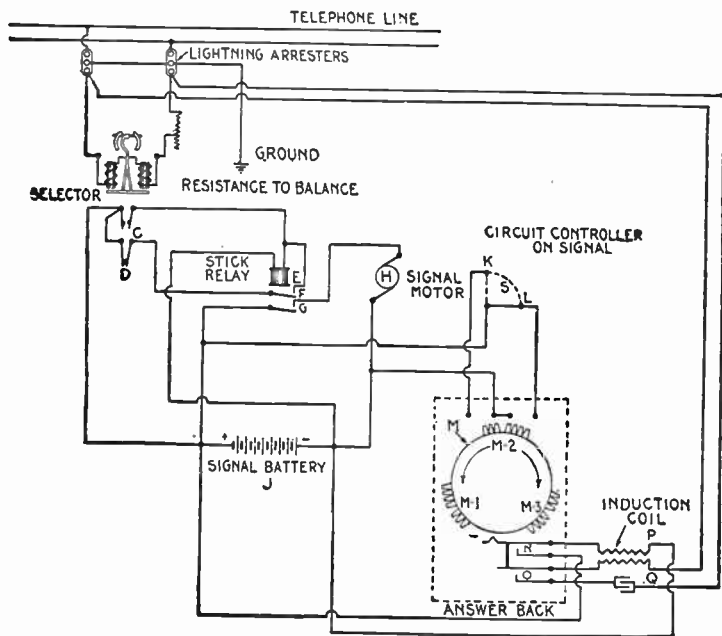
FIG. 3,741. —Train dispatcher's selector system. This is used to indicate to the train engineer whether he is to proceed on the main line or to take a side track. The indication may be in the form of a disc, a light, a semaphore, or any prescribed signal. When the indicator signal is turned from the normal to the reverse position a special "answer back" device is also operated, which makes an audible noise and informs the dispatcher that the signal has operated properly. This device is controlled by a commutator operating on the signal mechanism in connection with an induction coil. To display a "take siding" signal the dispatcher turns a switch or depresses a key which operates the selector by closing the normally open contacts marked C. The "stick relay" throws signal battery current into a motor which operates the signal. To restore the signal to normal position the dispatcher operates the selector in the reverse direction, which opens the contacts marked C. This causes the "stick relay" to restore to normal position and throws a reverse signal back to the dispatcher. This system is semi-automatic.
