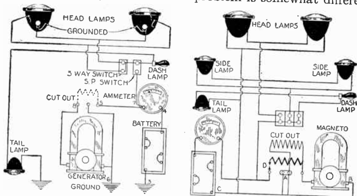
Figs. 4,028 and 4,029.—Holtzer-Cabot lighting magneto outfit installation, views showing location of switch, ammeter, cut out and their connections. Fig. 4,028, one wire system is applied to double bulb or turn down head lamps; fig. 4,229, two wire system, suitable also as a general guide for motor boat wiring.
