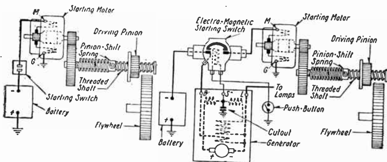
FIGS. 4,048 and 4,049.—Diagrams of Westinghouse electrical and mechanical connections of double reduction motor and switch for automatic screw pinion shaft. Fig. 4,048, with hand or foot operated starting switch; fig. 4,049, with electro magnetically operated starting switch controlled by push button. In the figures, when the starting switch is closed, the full battery voltage is impressed on the motor, and it starts immediately. The pinion, when the motor is at rest, is within the screw shift housing and entirely away from the flywheel gear. The threaded shaft is connected to the reduction gear shaft by a spring which thus forms a flexible coupling. As the load is not large enough to compress the spring when the motor starts, the threaded shaft is immediately revolved by the spring in released position. The pinion moves out on its shaft by virtue of the revolving threads, until it reaches the flywheel. If the teeth of the pinion and flywheel meet instead of meshing, the spring allows the pinion to revolve until it meshes with the flywheel. When the pinion is fully meshed into the flywheel teeth, the spring compresses and the pinion is then revolved by the motor as through a continuous shaft, turning the engine over. When the engine fires and the flywheel peripheral speed continuously exceeds that of the driving pinion, it forces the latter out of mesh, and it is returned to its original position in the screw shaft housing. During the periods immediately after the engine has passed over any one of the points of maximum compression, the spring offers an elastic cushion between the flywheel and the reduction gear so that the pinion will not be thrown out of mesh.
