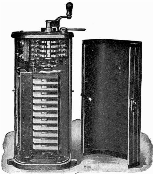
Figs. 3,549 and 3,550. —General Electric series parallel controller. In this type, of which there are several forms, the power circuits are not broken during transition from series to parallel connections. The series parallel controller, as is well known, is used to control two motors, or two pairs of motor, and serves to connect these motors in series or in parallel relation. By means of these connections a car may be run economically at a medium speed, as well as at full speed, and can be accelerated to full speed more efficiently than is possible with a simple rheostatic controller. Hence, the practically universal adoption of the series parallel controller in railway service. The older forms of K controller were designed for operation on a normal line pressure of approximately 500 volts. With the advent of the commutating pole railway motor, the use of higher operating pressures, 600 to 650 volts, became possible and is now common practice, especially on interurban lines. To successfully operate on these higher voltages, individual blow outs and other features were introduced.
