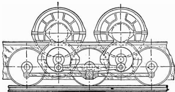
FIGS. 3,529 to 3,533.—Various motor suspensions. Fig. 3,529, New Haven geared motor; fig. 3,530, New Haven gearless motor; fig. 3,531, New Haven topgeared motor; fig. 3,532, Pennsylvania gearless motor with connecting rods; fig. 3,533, geared motors with yoke, or erroneously called Scotch yoke.
