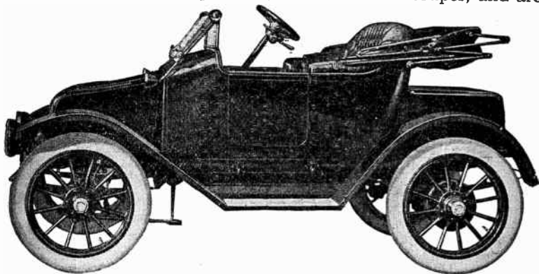
Fig. 4,058. —Baker electric roadster. The general specifications are as follows: frame, pressed steel; wheel base, 83 ins.; tread, 50 ins.; steering mechanism, two types, one with wheel steer, the other with lever steer; controller, continuous torque type, six speeds forward and three reverse; springs, semi-elliptic and full elliptic rear; battery, 3½ cells, 13 MV thin plate Exide, standard; tires, 32×4 special electric pneumatic front and rear or 34×4 cushion front and rear; brakes, two sets of internal expanding on rear wheels, operated independently by two foot pedals; body aluminum, with side doors, open top, nickel and black metal finishings throughout; painting, body black, blue, green, or maroon panels, striping to match; upholstery, blue, green, or maroon leathers, or imported broadcloths, standard; fenders, full skirted metal curved fenders; equipment, two head lamps, two side lamps, tail lamp, side and storm curtains; volt ammeter and shaft odometer, full kit of tools, special adjustable clear vision wind shield, electric horn.
