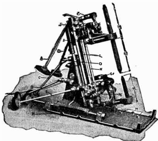
FIG. 3,877. —Simplex arc lamp. The carbon holders are furnished to accommodate carbons of \frac{1}{2} " to \frac{1}{4} " diameter and 12" upper and 6" lower in length, carrying capacity 75 amperes. There are eight adjustments, six being accessible from the back of the lamp house; and two, to alter the angle of the carbon, from the inside. The lamp can be withdrawn from the back of the lamp house, so that all parts are readily accessible.
