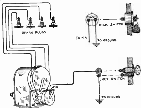
Figs. 4,017 and 4018. —Wiring diagram of Eisemann type G4 magneto. Troubles and remedies. If the engine misfire or refuse to start, it should be found out first whether the trouble lie in the magneto or in the spark plugs. The latter should be examined first, as they are the most frequent cause of trouble. If the missing be in one cylinder only, or in different cylinders, the corresponding spark plug should be examined to see that the gap be not too large. This gap between the electrodes should be approximately \frac{1}{8} of an inch. Also the spark plug may be short circuited through carbon, or the insulation may be cracked. Cleaning with gasoline or replacing is the remedy. The wiring should be very carefully examined and checked in accordance with the firing order of the engine. If cables be cracked or worn, they should be replaced. Clean same with gasoline until the contact surface appears quite white, or if pitted use a fine file—a manicure file will serve the purpose very well—but file very carefully, so that the surfaces will remain square to each other. The correct gap of the contact points is \frac{1}{16} " and in no case should it be more than \frac{1}{8} ". As these contacts wear away in time, they should be regulated by giving the adjustable screw "U" a forward turn, care being taken to securely tighten the lock nut "V". This can be accomplished without removing the timing lever or make and break mechanism, as shown in figs. 3,978 and 3,979. The cut also shows the combination wrench which is furnished with each magneto and which includes a gauge for the regulation of the gap between the platinum contacts ( \frac{1}{16} "). If the platinum contact riveted to the contact spring "17m", or that of the adjustable screw "U" should be worn down entirely, it would necessitate a change of either or both. When the adjustable screw "U" is replaced or adjusted, care must be taken that the lock nut is securely tightened in place. If after following these instructions, the engine still refuse to start, the magneto should then be tested by removing the distributor plate and resting a screw driver on the gear casing holding same about \frac{1}{8} " from the collector ring. Then, if upon rotating the armature, a spark jump across the \frac{1}{8} " gap, it shows that the trouble does not lie in the magneto, but in some other part of the engine, possibly the carburetter. If a spark do not jump across the \frac{1}{8} " gap previously mentioned, the magneto should be examined by an expert.
