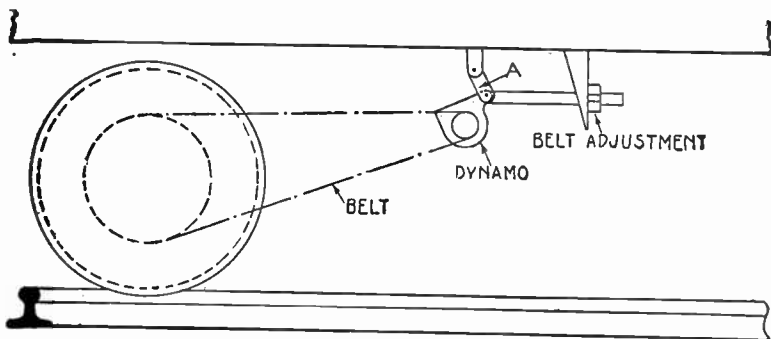
FIG. 3,673.—Method of dynamo suspension in Stone system. As shown, the dynamo is supported at one corner of its frame by the adjustable link A, in such a manner that it is free to swing toward or away from the driving axle. The suspending link is so placed that the belt draws the dynamo out of the diagonal position in which it would naturally hang, thus putting a definite tension on the belt, just sufficient to absorb the power required. It is obvious that when the pull on the belt exceeds that due to the offset suspension of the dynamo that the dynamo will be drawn toward the axle and the belt allowed to slip. Thus the dynamo will run at practically constant speed for all values of train speed above the critical value. A strong mechanical governor automatically closes the dynamo circuit when critical speed has been reached. A storage battery is suspended underneath the car to act as auxiliary in lighting the lights when the dynamo is inoperative. Another function of the storage battery is that it acts as a ballast or regulator to keep the lights constant, absorbing all the variations of dynamo output. The lubrication of the dynamo is effected by means of an electrically controlled oil supply so adjusted that when the dynamo is in operation oil will flow from the oil tank, but when the dynamo is inoperative, the supply is cut off and no waste takes place. The predetermined speed of dynamo was 915, at which it delivered 20 amperes.
