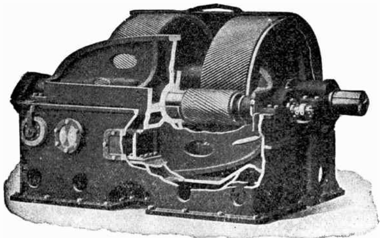
FIG. 3,780.—View of 6,000 horse power Melville-MacAlpine speed reduction gear with case broken away showing construction. It is a double helical spur gear, designed with involute teeth, and a transmission capacity of 6,000 horse power at a pinion speed of 1,500 r.p.m. The pinions have 35 teeth, the spur wheels 176 teeth. The 176th tooth constitutes a bunting cog and equalizes the wear. The pitch circle diameters are 14 ins. and 70 ins. respectively. The reduction ratio is thus practically 5 to 1, hence the power is delivered from the gear at a speed of only 300 r.p.m. The pitch line speed is 5,500 ft. per minute and the design is based on a limiting pressure of 450 lbs. per inch of tooth contact. Provision is made for the liberal use of lubricating and machine oil. Rear-Admiral Melville writing in Proc. Inst. Civil Engineer, Feb., 1910, states as follows: A full power test of 6,500 horse power was carried out for a period of 40 hours from 2.30 P.M. on Oct. 16, 1909, till 6.30 A.M. Oct. 18. At the close of this test the gear was found to be in excellent condition and without any sign of wear. This established without question the fact that gearing could be made to transmit such large powers continuously at high speed.
