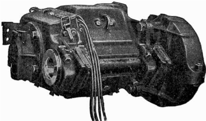
FIG. 3,517.—General Electric standard box frame motor. In this type the magnet frame is one piece of cast steel, and, as shown, is approximately octagonal in shape. The frame is provided with bored openings at each end, through which the armature, pole pieces, and field coils can be inserted or removed through the pinion end opening. Bails are cast on the frame at convenient points to facilitate handling. The opening through the frame over the commutator is large and inclined at an angle to allow easy access to the commutator and brush holders. Hand hole openings are located at points most convenient for the inspection of the interior of the motor. Drain holes are drilled in the lower side of the motor frame. The axle caps (which are inclined at an angle of approximately 60 degrees to the horizontal) are tongued and bolted to machined surfaces on the magnet frame.
