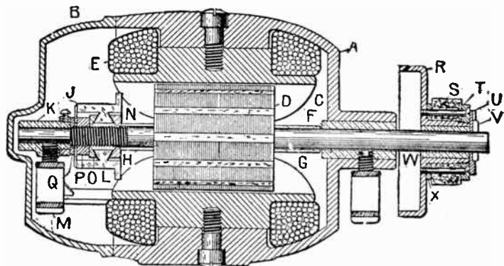
FIG. 3,951. —Sectional diagram of the Apple igniting dynamo. The parts shown are: A, cast iron body containing the moving parts; B, the hinged lid of the body; C, the one pole piece of one of the field magnets; F, brass bearing of the armature spindle; G and H, fibre tubes surrounding the spindle; K, brass spider supporting the spindle; L, commutator; M, wick feed oil cup; N, beveled nut supporting the commutator; O, P, Q, supports of the commutator; R, the driving disc; S, lever friction pinion. This machine can generate a direct current at 8 volts at a speed of between 1,000 and 1,200 revolutions per minute. It is provided with a simple centrifugal governor that automatically interrupts the driving connections when a certain speed has been exceeded.
