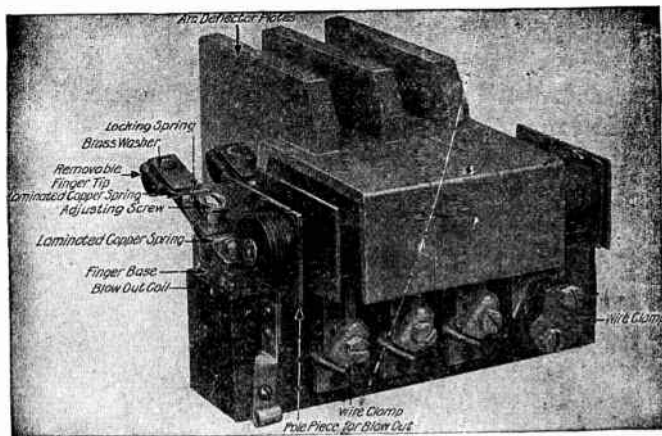
FIG. 3,551.—Detail of General Electric type K magnetic blow out showing main finger and wire clamps. The figure shows the construction of blow outs used in forms K-34, K-35, K-36 and K-44 controller. Each finger is supplied with a separate magnetic blow out, consisting of a complete magnetic circuit, blow out coils and arc deflecting chutes. In this illustration one of the iron plates forming part of the magnetic circuit is removed to show the finger and blow out coil. The current entering at the clamp terminal passes through the blow out coil, through the finger to the segment, generating a strong magnetic field across the space between the arc deflector plates, so that when the circuit is broken the arc is blown in an outward direction, away from the cylinder. In order to extend the pole pieces to a point where arcing occurs, between the finger and segment, iron plates are imbedded in the insulation of the arc chutes. The arc chutes are made of a special moulded insulation compound, which does not carbonize under the influence of an arc. Ample space is provided in these chutes for the expansion of the arc when breaking a circuit. As the arc is projected away from the cylinder, the danger from short circuiting, which occurred with the older form of blow out, has been eliminated. In the older controllers, the magnetic blow out is composed of one magnetic field, extending the full length of the cylinder, and produced by a single coil. The effect of this field is to extinguish the arcs by blowing them either up or down against the deflector plates, and not directly away from the cylinder.
