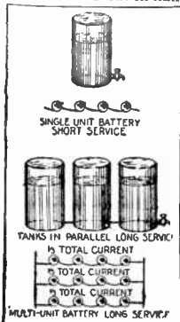
Figs. 3,938 to 3,941.— Hydraulic analogy of recuperation.
