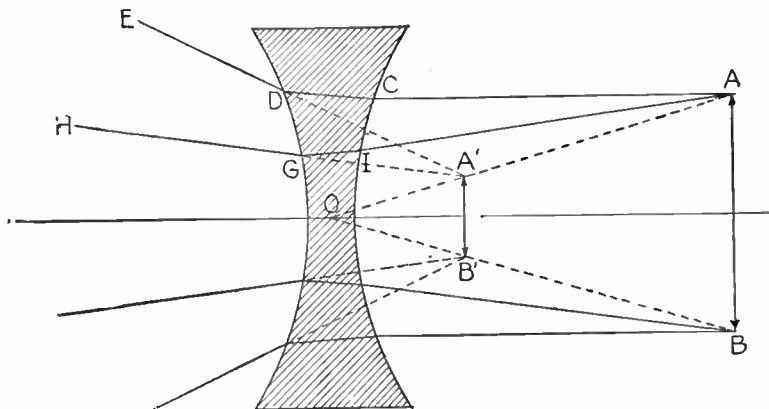
FIG. 3,805. —Formation of virtual image in double concave lens; no real image is formed with this type of lens. Let AB be an object placed in front of the lens. If the secondary axis AO be drawn from the point A , all rays AC, AD, AE, \dots , from this point are twice refracted in the same direction, diverging from the axis AO , so that the eye receiving the emergent rays DE and GH , supposes them to proceed from the point where their prolongations cut the secondary axis AO in the point A' . Similarly, drawing a secondary axis from the point B , the rays from this point form a pencil of divergent rays, the directions of which, prolonged, intersect in B' . Accordingly the eye sees at A'B' , a virtual image of AB , which is always erect, and smaller than the object .
