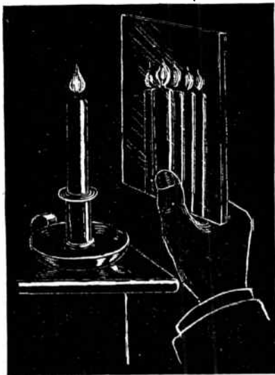
FIG. 3,774. —Experiment illustrating multi-image in ordinary mirror. Let the flame of a candle be observed very obliquely in an ordinary mirror. From four to ten images of the flame may be seen arranged in a row, as here shown. The second image of the series will be by far the most brilliant.
