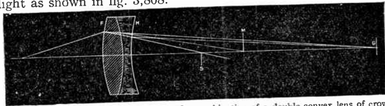
FIG. 3,809. —Achromatic lens, consisting of a combination of a double convex lens of crown glass, and a double concave lens of flint glass. Whenever it is desired to project especially good pictures upon a screen, lenses are often combined as shown in the figure. Here M indicates the line through the principal axis, at which the red rays reflected by the double convex lens would strike, and S, the line where the violet rays would be projected. The addition of the double concave lens brings the red and violet together again at G. A combination of two such lenses F H, placed the proper distance apart and the surfaces properly proportioned, may be made to combine any two of the colors of the spectrum. Accordingly even with these connected lenses there is always some coloring on the screen, although hardly noticeable.
