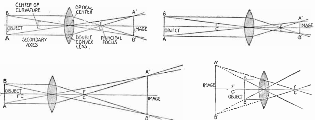
Figs. 3,801 to 3,804.—Images formed by double convex lens with object at various distances from the lens. Fig. 3,801, object at twice the focal distance; fig. 3,802, object more than twice focal distance; fig. 3,803, object at a distance less than twice the focal distance; fig. 3,804, object at a distance less than the focal distance. In the construction of these figures, two rays from any point are all that are needed to locate the image. The two most convenient are, one parallel to the principal axis and the other through the optical center. The former will, after refraction, pass through the principal focus, which in cases here considered is at the center of curvature, and the latter will pass through the lens without change of direction.
