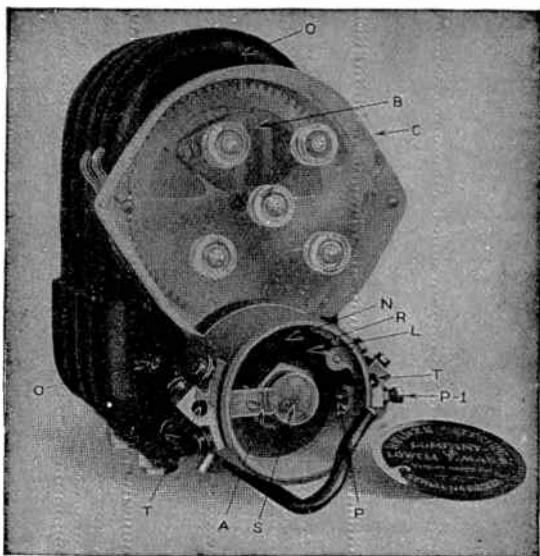
FIG. 3,956. —Heinze low tension magneto. The reason round magnets are used is because it is claimed better contact is thus obtained with the pole pieces or by carefully grinding the ends of the magnets and reaming the holes in pole pieces. Magneto instructions: 1, Keep interior of breaker box clean; 2, keep phosphor bronze studs on end of armature clean; 3, keep steel plate in breaker box clean; 4, keep platinum points clean and surfaces flat; 5, use nothing but emery paper or fine file on platinum points; 6, be sure all leads are soldered in terminals or rigidly connected; 7, platinum points should be adjusted to .02 of an inch; 8, lubricate bearing in interrupter lever with one drop of very light oil every two or three thousand miles; 9, spark plug gap should be adjusted to a minimum of .02 inch and maximum of .025 inch; 10, connect dry cells so as to produce not more than 3 or 4 volts; 11, never leave switch on battery point for any length of time either when engine is idle or running, as this causes excessive battery current and will injure the platinum points; 12, magnetos are considered running clockwise looking at the driving end. How to efficiently operate a Heinze magneto. In the figure the distributor cover C, and brush arm A, are shown semi-transparent so as to distinguish parts behind them. Be sure magneto is securely fastened to base and driving shaft is in perfect alignment. Be sure all connections are soldered or otherwise positively connected. Keep interior of breaker box clean. Keep phosphor bronze studs S clean and lubricate occasionally with a few drops of very thin oil. Keep inside surface of brush arm A, clean, as studs S make contact on this. Keep platinum points P, clean and surfaces of same flat. Use only emery cloth or fine file for this purpose. Platinum points should be adjusted to .02 of an inch separation when open. Gauge furnished on small wrench with magneto is proper thickness for this purpose. Adjust by turning platinum point screw P1 in or out as necessary. Lubricate bearing in make and break lever L, with one drop of very thin oil every two weeks when magneto is in continuous use. If make and break lever roll R, should become flat from wear, loosen nut N, and turn roll slightly to present a new surface to cam, and then tighten again. Be sure leads are rigidly connected in terminals TT. Leads must be long enough to allow free movement of breaker box. Remove distributor cover C occasionally and wipe out interior of same, also clean off any carbon dust or dirt from distributor brush B. Magneto bearings should be lubricated by oiling at 000 every week when magneto is in continuous use. Two or three drops are enough at a time. There is one oiler at rear end which does not show in cut.
