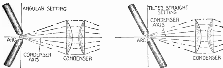
FIG. 3,866. —Arc setting for alternating current arc with cored carbons. When cored carbons are used, the crater will form in the end of the core, keeping in the center of the carbon pencil, and the vapor of the soft core will hold the arc between alternations. Without cored carbons, an alternating current arc has a tendency to run to the nearer edges of the carbons with loss of brilliancy upon the condensers.
