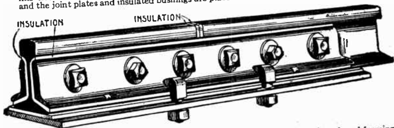
FIG. 3,720.—Simple method of connecting a relay between insulated joints of track and forming a block signal, the circuit being closed by the train as it passes over that section of track.
