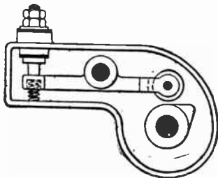
FIG. 3,986. —Contact breaker. This device keeps the circuit closed at all times except during the brief interval necessary for the passage of the spark at the plug points. It is used to advantage on engines running at very high speeds, as it allows time for the magnetic flux in the core of the coil to attain a density sufficient to produce a good spark.
