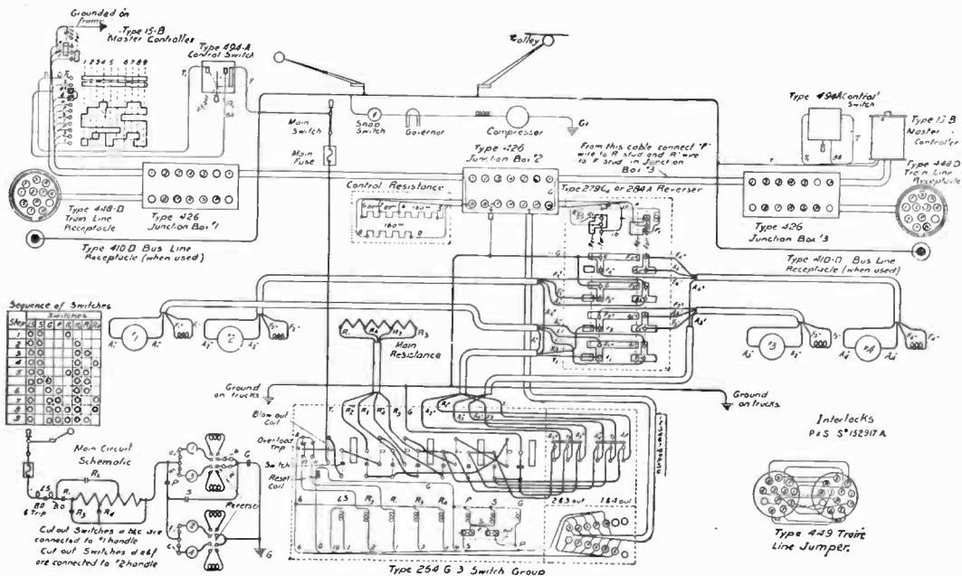
FIG. 3,754.—Complete wiring diagram of Westinghouse type HL control for four 50 horse power 500 volt motors.
