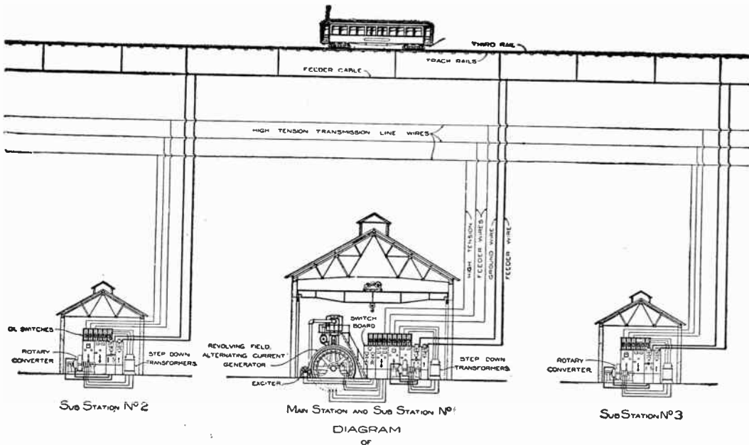
FIGS. 3,489 to 3,491.— Alternating current transmission, direct current distribution. The diagram shows the main station and two sub-stations with apparatus and connections to the line. In the system here shown three phase current is generated at the main station, where it passes to step up transformers to increase the pressure a suitable amount for economical transmission. At various points along the railway line are sub-stations , where the three phase current is reduced in pressure to 500 or 600 volts by step down transformers, and converted into direct current by rotary converters. The relatively low pressure direct current is then conveyed by feeders to the rails, resulting in a considerable saving in copper in moderate and long distance lines.
