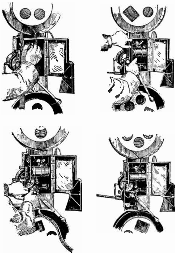
Figs. 3,842 to 3,845. —“Threading” a typical motion picture machine. Fig. 3,842 illustrates the method of threading the film through the film trap by forming the upper loop with the second finger of the left hand and gripping the film below the intermittent sprocket with the first finger. Fig. 3,843 illustrates how the film is threaded through the film trap by forming the upper loop with the second finger of the left hand and gripping the film below the intermittent sprocket with the first and third fingers of the right hand and closing the film trap gate by tripping the film trip lever with second finger. Fig. 3,844 illustrates the method of forming the lower loop, threading the film over the lower feed sprocket and closing the lower feed sprocket roll arm by a downward pressure with the first finger of the right hand. The film is then inserted through the fire valve by means of the slot in the base of the mechanism and is then fastened on to the lower reel so as to rewind to the right. Fig. 3,845 shows the machine completely threaded from the top reel to the feed sprocket through the film trap and on to the lower feed sprocket and the take up reel.
