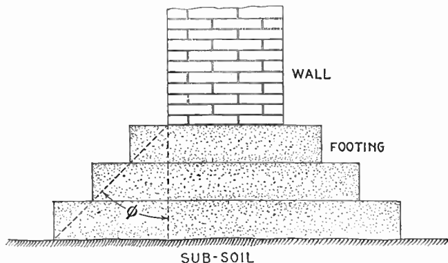
FIG. 2,733. —Angle for foundation footing. In ordinary practice the footing courses upon which the walls of the building proper rest, consist of blocks or slabs of stone as large as are available and convenient to handle. Footings of brick or concrete are also used in very soft soils; footings consisting of timber grillage are often employed. A grillage of iron or steel beams has also been used successfully. The inclination of the angle \phi , of footing should be about as follows: for metal footings 75^\circ ; for stone, 60^\circ ; for concrete, 45^\circ ; for brick, 30^\circ . Damp proof courses of slate, or layer of asphalt are laid in or on the foundations or lower walls to prevent moisture arising or penetrating by capillary attraction.
