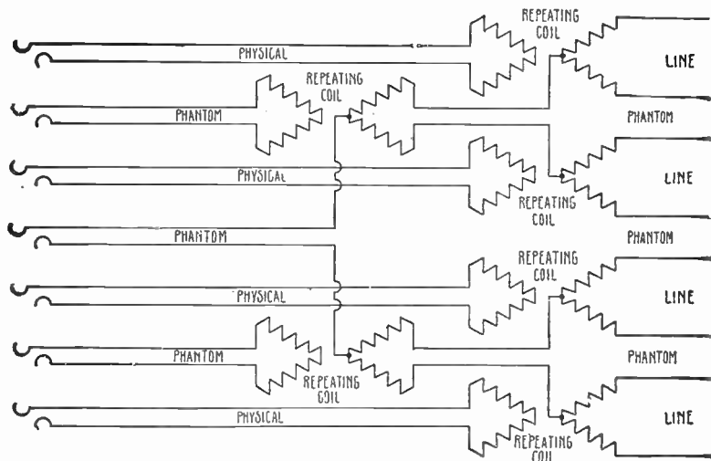
FIG. 2,984.—Complex phantom circuits. Circuits may be combined with repeating coils to form additional phantom circuits so that, as shown, an extra phantom circuit may be built up on two other phantom circuits, each of which is built up on two physical metallic circuits. The fundamental object of the phantom circuit is one of economy, since it results in the practicability of securing three good metallic circuits from four wires, such as are used at present for trans-continental work and the possibility of securing seven circuits from eight wires as shown in the diagram. The transposition necessary to secure freedom from inductive disturbances will probably result in such a disarrangement of the wires as to make it inadvisable to use any higher form of phantom than the single phantom. With this there is actual betterment of transmission so that some long distance operators give preference to the phantom circuits because of the better transmission secured over them. The use of phantom circuits is confined almost wholly to open wire construction. It is possible, however, to build up phantom circuits in ordinary cable by using pairs in reversely wound layers, and it is also possible to construct a cable, using four wire units, as to permit the use of phantoms.
