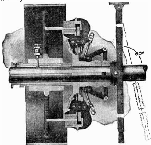
FIG. 2,316. —The Hill friction clutch pulley for power control. The clutch mechanism will start a load equivalent to the double belt capacity of the pulley to which the clutch is attached.
