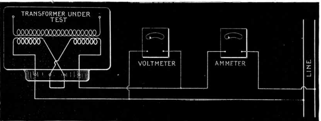
FIG. 2,904. —Transformer internal insulation test, sometimes called double normal voltage test, from the fact that most transformers are tested with double normal voltage across their terminals. If either the primary or secondary of the transformer be connected to some source of current with voltage double that of the voltage of the transformer under test, the insulation between adjacent turns, and also the insulation between adjacent layers will be subjected to twice the normal operating voltage. It is good practice to employ high frequency for this test in order to prevent an abnormal current from passing through the transformer. Sixty cycle transformers are usually tested on 133 cycle, and 25 cycle transformers on 60 cycle circuits for this double normal voltage test. It is necessary to insert the resistance in the circuit of the transformer and bring the voltage up gradually, the same as applying other high insulation tests in order to prevent abnormal rises in pressure at the instant of closing the circuit.
