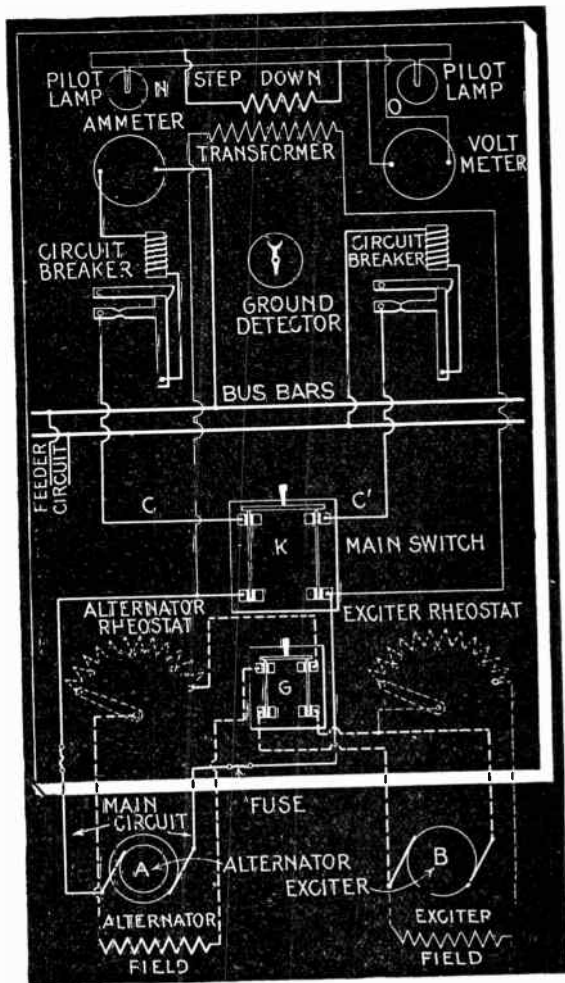
FIG. 2,820.—Switchboard wiring for a single phase separately excited alternator. The direct current circuits are represented by dotted lines, and the alternating current circuit, by solid lines.
