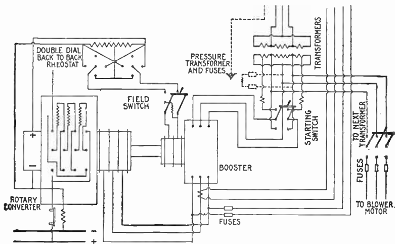
FIG. 2,869. —Wiring diagram for General Electric synchronous converter with series booster as illustrated in fig. 2,868.
