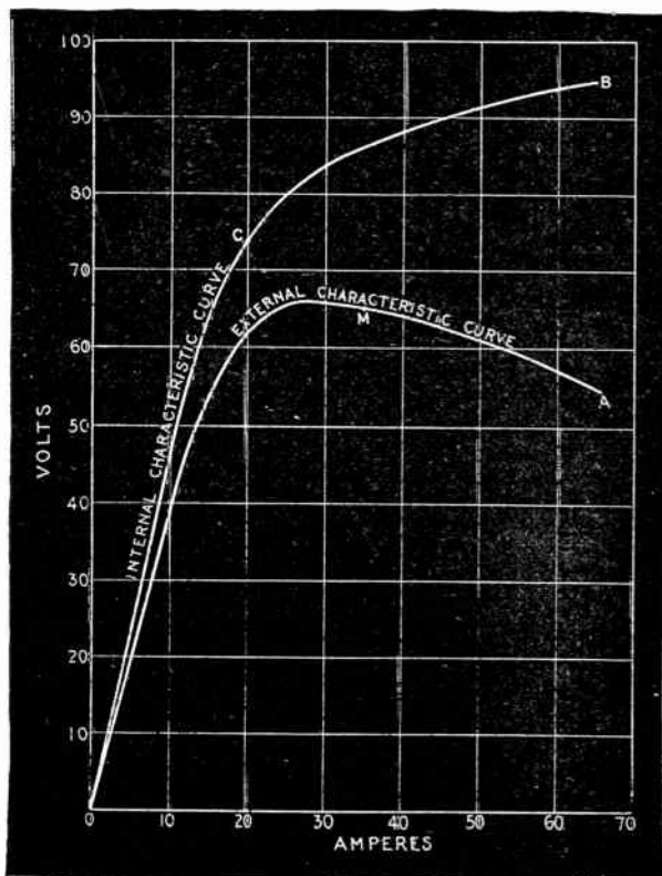
FIG. 2,908. —General form of characteristic curves for a series dynamo. The general curve that may be expected is OA. It is obtained practically in the same manner as for the shunt characteristic curve, except that no field rheostat is employed. Commencing with no load or amperes, there will probably be a small deflection noticeable on the voltmeter, due to the residual magnetism. The other readings are taken with successive reductions of main current resistance. The curve OA thus obtained for a certain series generator is practically a straight line at the beginning, representing thereby a proportional increase of voltage with increase of current, but after a certain current is reached (about 20 amperes in this case) the curve flattens and takes a downward direction. The turning point occurs in the characteristic curves of all series generators, and it denotes the stage at which the iron magnet cores become so saturated with lines of magnetic force that they will not readily allow more to pass through them; this turning point is technically known as the point of saturation, and the current corresponding (20 amperes in this case) is called the critical current of the dynamo. The point of saturation in any given series machine is governed by the amount of iron in the magnetic circuit; its position in the curve therefore varies according to the design of the generator as does also the critical current. The value of the latter is important inasmuch as the valuable features of a series generator assert them-
