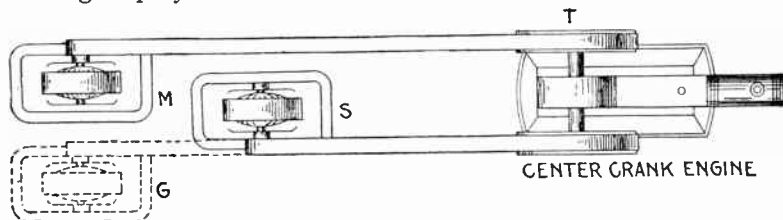
FIG. 2,811. —Double pulley drive for economizing floor space with belt transmission. Where a center crank engine is used both pulleys may be employed by belting a machine to each as shown. Although considerable floor space would be saved by the use of this scheme if the generators thus belted were placed at M and G yet still more floor space would be saved by having them occupy the positions indicated at M and S.
