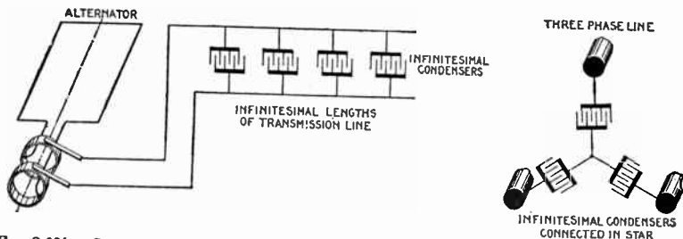
FIG. 2,681.—Capacity effect in single phase transmission line. The effect is the same as would be produced by shunting across the line at each point an infinitesimal condenser having a capacity equal to that of an infinitesimal length of circuit. For the purpose of calculating the charging current, a very simple and sufficiently accurate method is to determine the current taken by a condenser having a capacity equal to that of the entire line when charged to the pressure on the line at the generating end. The effect of capacity of the line is to reduce the pressure drop, that is, improve the regulation, and to decrease or increase the power loss depending on the load and power factor of the receiver.
