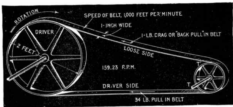
FIG. 2,813. —One horse power transmitted by belt to illustrate the rule given above. A pulley is driven by a belt by means of the friction between the surfaces in contact. Let T be the tension on the driving side of the belt, and T' the tension on the loose side; then the driving force = T - T' . In the figure T is taken at 34 lbs. and T' at 1 lb.; hence driving force = 34 - 1 = 33 lbs. Since the belt is travelling at a velocity of 1,000 feet per minute the power transmitted = 33 lbs. \times 1,000 ft. = 33,000 ft. lbs. per minute = 1 horse power.
