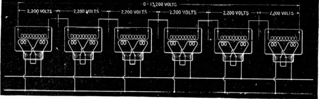
FIG. 2,903. —Transformer insulation test as made when a special high tension transformer be not available. In this method a number of standard transformers, connected as shown may be employed, but great care should be taken to have such transformer cases thoroughly insulated from the ground and from one another, in order to minimize the insulation strains in the testing transformers. Care should be taken to insert in the circuit of each testing transformer a fuse, not in excess of the transformer capacity, which will blow, in case of a break down in the apparatus under test. In testing insulation between secondary and core, disconnect the primary entirely, apply one terminal of the testing transformer to the secondary terminals of the transformer under test, and the other terminal of the testing transformer to the core of the transformer under test. This test should also not be in excess of one minute.
