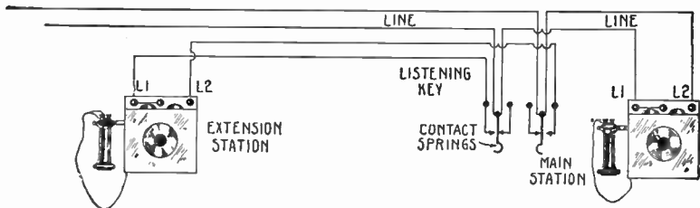
FIG. 2,951. —Wiring diagram showing two telephones with a listening key at the main instrument to cut off the extension station. This key can be placed at either inner or outer contacts, and the extension wired to either inner or outer contacts. As shown the key is at the main station and the extension is on the outer contacts. This is called plan 10.
