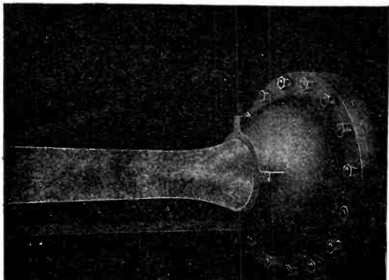
FIG. 2,762.—Water discharging from a needle nozzle due to a pressure of 169 lbs. per sq. in.
