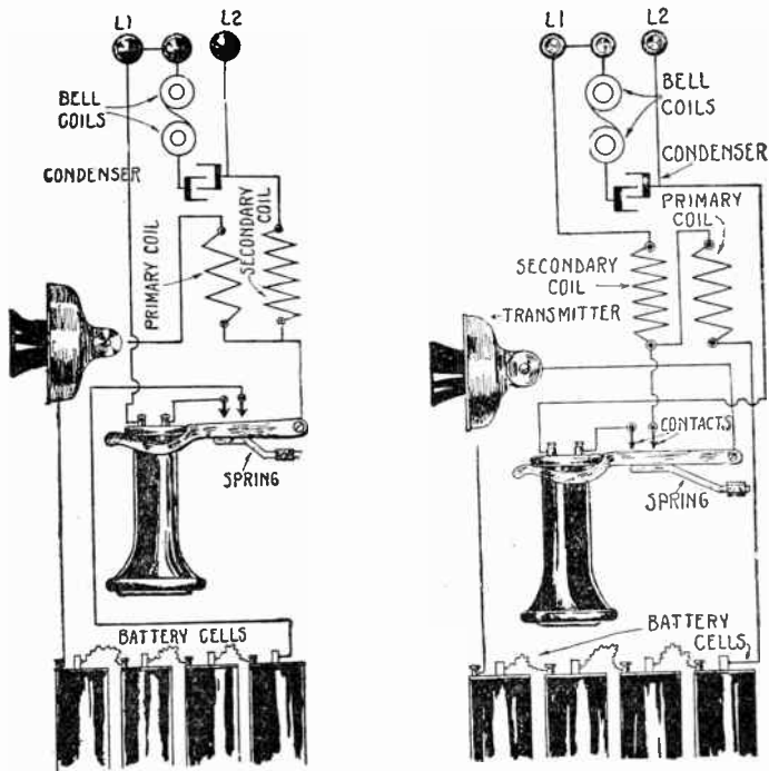
FIG. 2,953. —Wiring diagram of booster set with battery connected in the circuit to strengthen transmitting and receiving power of common battery instrument. The primary and secondary windings of special induction coil are connected at one end and the battery cells are connected in series, as shown, with the switch hook contact and transmitter; otherwise the circuit is the same as all common battery telephone instruments.
