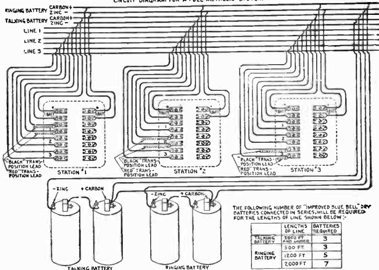
CIRCUIT DIAGRAM FOR A COMMON RETURN SYSTEM
