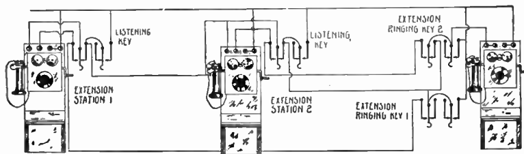
FIG. 2,929.—Wiring diagram showing three magnetos wired so that only one bell at a time can be rung by central (according to which listening key is thrown) but one can talk from any one of the three instruments when the keys are normal. If either listening key be thrown so that the swinging contact springs touch the outer contacts, the main instrument will be cut out of circuit. If listening key 1 be thrown, both the main and other extension station will be cut out; if key 2 be thrown, station 1 can talk and hear but the bell will not ring. With the keys normal, the main bell is rung by central. If a listening key be thrown the bell at that station will be rung by central. Each extension has its own ringing key for ringing from the main which makes the system intercommunicating. Each station is fed by its own battery and each has its own magneto. This is called plan 5 magneto by the New York Telephone Co.
