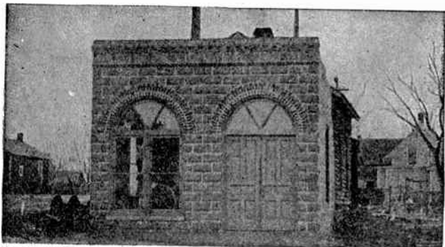
FIG. 2,707. —Exterior of central station at Lewis, Ia.; example of very small station located in the principal business section of a town. It also illustrates the use of a direct connected gasoline electric set. The central station is located on Main Street, which is the principal thoroughfare, and is installed in a low one story building for which a mere nominal rental charge is paid, the company having the option to buy the property later at the value of the land plus the cost of the improvements and simple interest on the same. To the front of an old frame building about 16 feet by 28 feet has been built a neat, well lighted concrete block room, about 16 feet by 16 feet, carrying the building to the lot line and affording ample space for the generating set and switchboards, and such desk room as is needed for the ordinary office business of the company. In this room, which is finished in natural pine with plastered walls, has been installed a standard General Electric 25 kw. gasoline electric generating set consisting of a four cylinder, four cycle, vertical water cooled, 43-54 H.P. gasoline engine, direct connected to a three phase, 2,300 volt, 600 R.P.M. alternator with a 125 volt exciter mounted on the same shaft and in the same frame. With the generating set is a slate switchboard panel equipped with three ammeters, one voltmeter, an instrument plug switch for voltage indication, one single pole carbon break switch, one automatic oil circuit breaker line switch and rheostats. Instrument transformers are mounted above and back of the board. For street lighting service a 4 kw. constant current transformer has been installed, and with it a gray marble switchboard panel mounted on iron frames and carrying an ammeter and a four point plug switch. On a board near the generator set are mounted in convenient reach suitable wrenches, spanners, and repair parts and tools. To cool the engine cylinders five 6 X 8 steel tanks have been installed in the old building, a pump on engine giving forced circulation.
