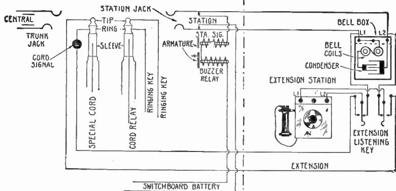
FIG. 2,952. —Wiring diagram showing private line extension station circuit from P.B.X. switchboard, whereby absolute secrecy with outside exchanges is obtained. When extension listening key is normal, extension signals operator in same way as do all other extensions. After asking for private connection special cord, without listening key being plugged in central (trunk) jack by operator, subscriber throws extension listening key and conversation ensues. If P.B.X. operator's attention be again desired, listening key is thrown normal. Operator calls extension in usual way on any cord except special and rings extension special bell no matter how listening key be thrown. Since there is no listening key on special cord, operator must use any other cord for connection between P.B.X. and extension station.
