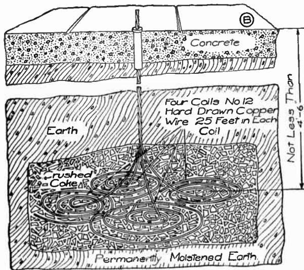
Figs. 3,015 and 3,016.—Correct method of making an exchange ground. A is the method of connecting to a water pipe. B, shows best method of making a ground connection. In this method, four coils of copper wire, each containing 25 feet are buried in gas coke or charcoal below the permanent moisture level, as shown. The area of the plate should not be less than 10 sq. ft. The protectors should be grounded before any lines are connected to the switchboard. Serious fires have occurred during the night in new central offices before they were placed in service, due to being left without lightning protection. There are various types of protector used at telephone stations and central offices, but they generally consist of carbon or copper blocks and fuses or heat coils. Where the line wires enter the central office the ordinary station lightning arrester consists of copper blocks and fuses or heat coils. Where the line wires enter the central office the ordinary station lightning arrester consists of copper blocks and fuses or heat coils. These are made with a fusible alloy which fuses readily at a given temperature. After this metal has been fused once the fusing point is considerably increased. The heat coils are placed in the protectors so that the metallic tips occupy the forward end of the slot in the spring nearest the protector bar while the fibre tips rest in the rear of the slot of a corresponding spring.
