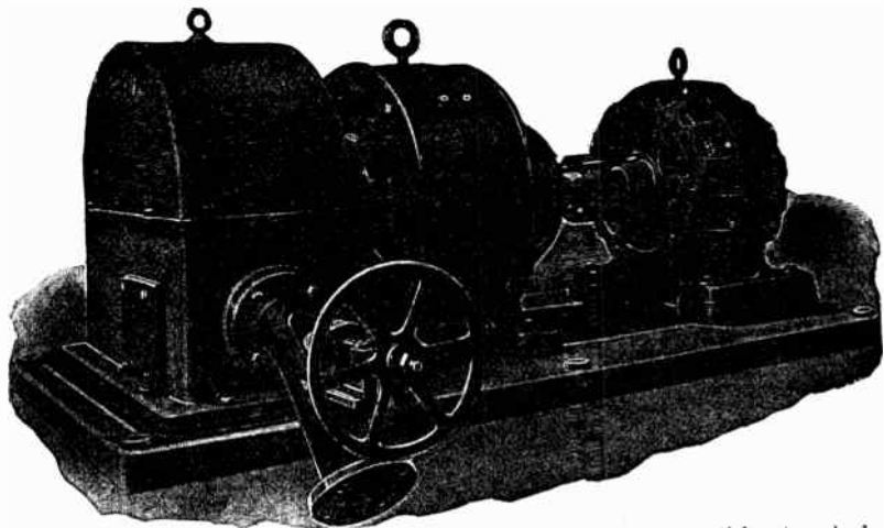
FIG. 2860.—Motor generator exciter set driven by a Pelton-Doble tangential water wheel. The water wheel runner is mounted on the shaft overhung and the jet is regulated by either a hand actuated or governor controlled needle nozzle. The speed of the water wheel is equivalent to the synchronous speed of the induction motor, hence, the latter floats on the line, and under certain conditions may perform the functions of an alternator by feeding into the circuit, should the water wheel tend to operate above synchronous speed. Should any interruption to the operation of the wheel occur, causing a diminution of speed, the induction motor would drop back to full load speed and take up the exciter load, resulting in no appreciable drop of exciter voltage. The only variation of speed possible is dependent upon the "slip" of the motor. Where two or more exciter sets are employed in the station, an advantageous arrangement embraces the installation of a water wheel driven motor generator set and an exciter set, consisting of merely the direct current generator and water wheel. The induction motor being electrically tied into the circuit, the possibility of a runaway of the water wheel is eliminated, since its speed can only slightly exceed the synchronous speed of the system.
