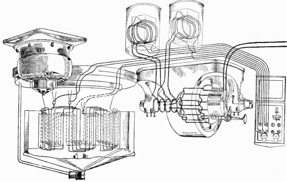
FIG. 2,867.—Skeleton diagram showing wiring of alternator, exciter, transformer and converter. The cut also shows switchboard and connects.
