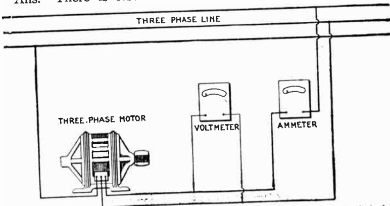
FIG. 2,881. —Three phase motor test ; voltmeter and ammeter method. If it be desired to determine the approximate load on a three phase motor, this may be done by means of the connections as shown in the figure, and the current through one of the three lines and the voltage across the phase measured. If the voltage be approximately the rated voltage of the motor and the amperes the rated current of the motor (as noted on the name plate) it may be assumed that the motor is carrying approximately full load. If, on the other hand, the amperes show much in excess of full load rating, the motor is carrying an overload. The heat generated in the copper varies as the square of the current. That generated in the iron varies anywhere from the 1.6 power, to the square. This method is very convenient if a wattmeter be not available, although, it is, of course, of no value for the determination of the efficiency or power factor of the apparatus. This method gives fairly accurate results, providing the load on the three phases of the motor be fairly well balanced. If there be much difference, however, in the voltage of the three phases, the ammeter should be switched from one circuit to another, and the current measured in each phase. If the motor be very lightly loaded and the voltage of the different phases vary by 2 or 3 per cent., the current in the three legs of the circuit will vary 20 to 30 per cent.
