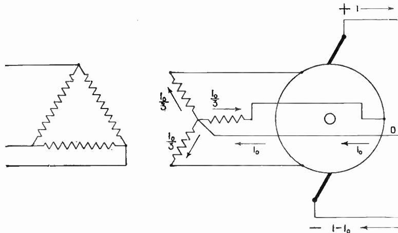
FIG. 2,870. —Wiring diagram for three wire synchronous converter with delta-Y connected step down transformer with the neutral brought out. It is evident that in this case each transformer secondary receives \frac{1}{3} of the neutral current, and if this current be not so small, as compared with the exciting current of the transformer, it will cause an increase in the magnetic density.
