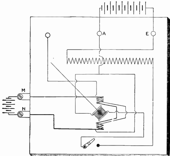
Fig. 2,898. —Diagram of connections for calibrating a wattmeter. The calibration of a portable wattmeter is accomplished with direct current of constant value which is passed through the series winding by connecting the source thereof with the current terminals. A direct current voltage which may be varied throughout the range of the wattmeter is also applied to the instrument between the middle and right hand pressure terminals A and E the wiring in the meter between these terminals being such that its differential winding is then cut out of circuit. The method of procedure consists in comparing the deflections on the wattmeter at five or six approximately equidistant points over its scale with the corresponding products of volts and amperes used to obtain them. The changes in the wattmeter deflections are effected by merely varying the voltage, the value of the current being maintained constant at a value which represents the full current capacity of the meter.
