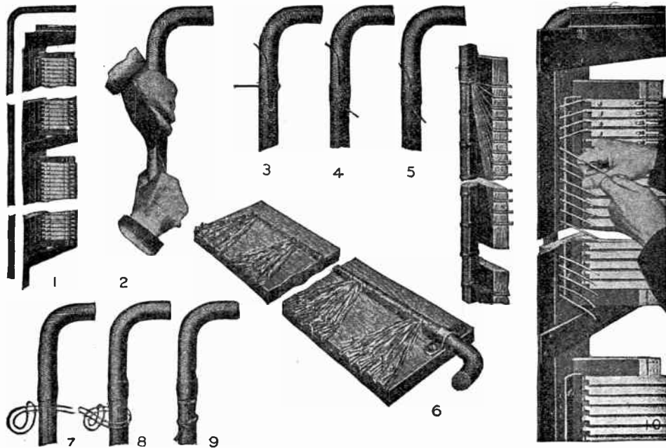
Figs. 3,004 to 3,014.—Forming and installing the line cable. —Uncoil the line cable which is coiled up either within the section or on top of it and lay it in the position which it will occupy permanently, thus measuring the length to the protective apparatus. Mark the cable \frac{3}{8} inch from the point where the first pair of wire will be let out to the apparatus (first operation). Determine by placing the cable parallel with the arrester strips, the length of cable which will allow sufficient length of wire to reach any terminal to which a conductor must be connected and cut away all excess cable. Remove the line cables from the supports, remove the braiding and serving and butt the cable as shown. Form up the cable. Place cables in rack in position they will occupy and fasten permanently in place by sewing them to the support with lacing twine. The wires should now be drawn through the holes in the fanning strips, the insulation removed, and the bare wires wrapped once around their respective terminals and soldered with resin core solder.
