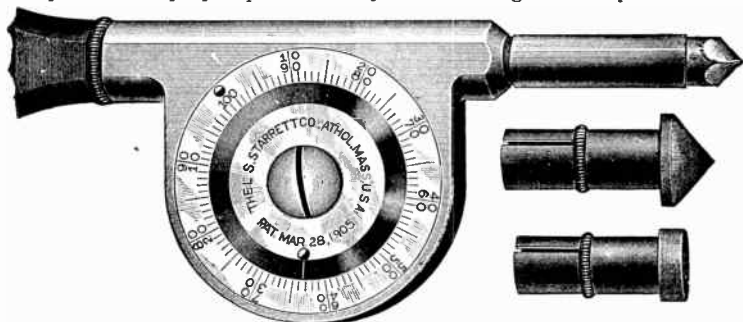
Figs. 2,800 to 2,802. —Starrett's improved speed indicator. In construction, the working parts are enclosed like a watch. The graduations show every revolution, and with two rows of figures read both right and left as the shaft may run. While looking at the watch, each hundred revolutions may be counted by allowing the oval headed pin on the revolving disc to pass under the thumb as the instrument is pressed to its work. A late improvement in this indicator consists in the rotating disc, which, being carried by friction, may be moved to the starting point where the raised knobs coincide. When the spindle is placed in connection with the revolving shaft, pressing the raised knob with the thumb will prevent the disc rotating, while the hand of the watch gets to the right position to take the time. By releasing the pressure the disc is liberated for counting the revolutions of the shaft when every 100 may be noted by feeling the knob pass under the thumb lightly pressed against it, thus relieving the eye, which has only to look on the watch to note the time.
