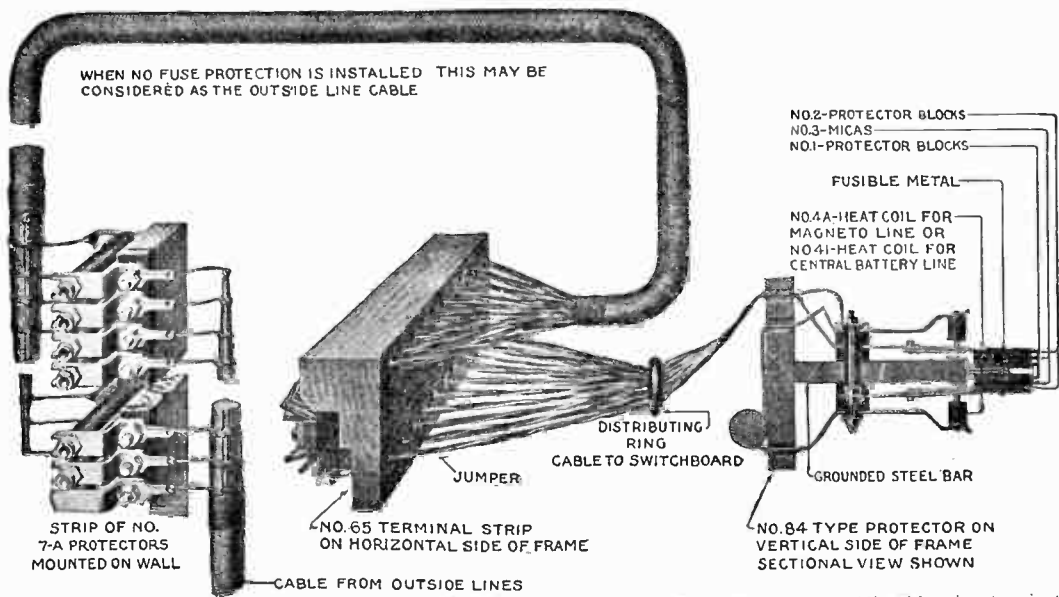
FIG. 3,011.—Various parts and cross connection of Western Electric No. 1,425 distributing frame. All cable wires terminate at a common distributing frame which is sometimes called a distributing board. The distributing board proper is fastened to the opposite side of the lightning arrester frame and each set of terminal on the board are connected to a pair of lightning arrester terminal by means of short twisted wires called jumper wires , which are passed through distributing rings. The terminals of each pair on the lightning arrester are connected to the bottom terminals of each pair on the terminal strip board. All the short jack springs are connected to the tip or ground side of the line, the metal frame of the lightning arrester and the ground strip in the cable box both being connected to ground. It is only necessary at a central office to have one good ground. From the upper terminals of each pair on the terminal strip, distributing cable wires run to and connect with protection fuses mounted on the distributing frame. The outside wires connect with the fuses and the switchboard wires with the arresters.
