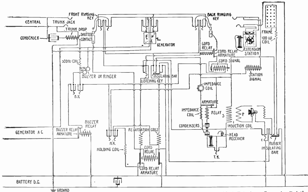
FIG. 2,936.—Circuit diagram of the new standard P.B.X. switchboard adopted by the New York Telephone Co. and called the positive supervision type . One pair of cord and plug are shown with one cord relay, also one station signal is shown and one station jack connected to the one extension station. One central jack is shown with its drop, shutter, and condenser. Two ringing keys connect to the two cords (front and back cords constitute a pair) and one listening key. With this type of switchboard, each pair of cord is supervised by the positive supervision relay which controls the bull's eye cord signal. There are as many station jacks and station signals as there are extension stations and as many central jacks and drops as there are central (trunk) lines coming into switchboard. There is only one buzzer key B.K., one night key N.K., one generator key G.K., one emergency key E.K. and one telephone receiver key T.K. mounted on each switchboard.
