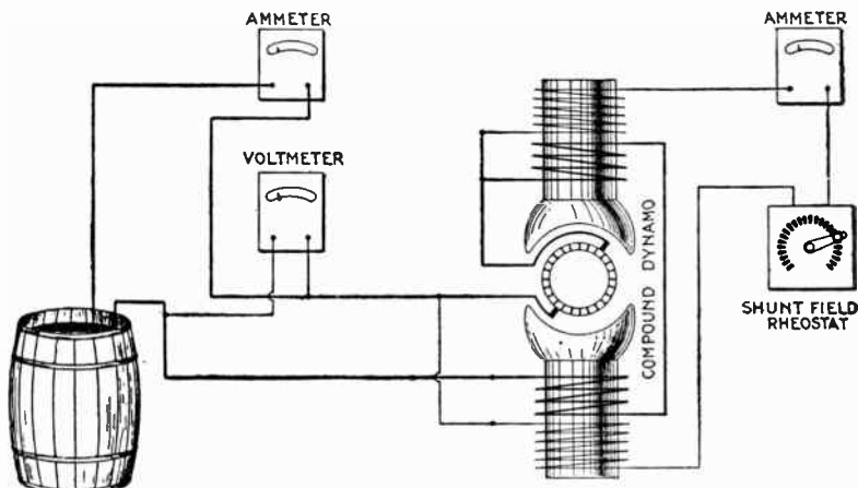
FIG. 2,895.—Compound dynamo external characteristics test; adjustable load.
