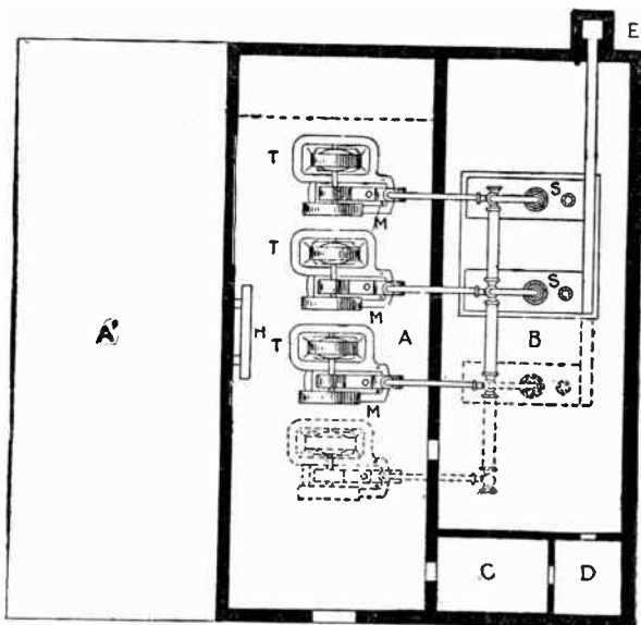
FIG. 2,732. —Plan of electrical station containing direct connected units. As shown, space is provided for an extra boiler and engine and generator set, as indicated by the dotted lines. Space also exists for a storage battery room if necessary, and the partition dividing this room from the engine and dynamo room is shown by a dotted line as in previous cases.
