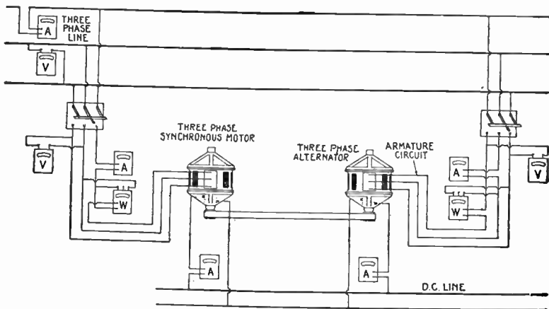
FIG. 2,889. —Three phase alternator or synchronous motor temperature test. In this test two alternators or synchronous motors of same size and type are used, and are belted together, one to be driven as a synchronous motor and the other as an alternator. The method employed is to synchronize the synchronous motor with the alternator or alternators on the three phase circuit, and then connect to the line by means of a three pole single throw switch. The alternator is then similarly synchronized with the alternator of the three phase circuit and thrown onto the line. By varying the field of the alternator it can be made to carry approximately full load, and the motor will then be also approximately fully loaded. The usual method is to have the motor carry slightly in excess of full load, and the alternator slightly less than full load. Under these conditions the motor will run a little warmer than it should with normal load, while the alternator will run slightly cooler. Temperature measurements are made in the same way as discussed under three phase motors. The necessary ammeters, voltmeters and wattmeters for adjusting the loads on the motors and generator are shown in above figure. If pulleys be of sufficient size to transmit the full load, with, say one per cent. slip, the pulley on the motor should be one per cent. larger in diameter than the pulley on the alternator, so as to enable the alternator to remain in synchronism and at the same time deliver power to the circuit. With very large machines under test, it is inadvisable to use the above method as it is sometimes difficult to so adjust the pulleys and belt tension that the belt slip will be just right to make up for the difference in diameter of the pulleys, and very violent flapping of the belt results. To meet such cases, various other methods have been devised. One which gives consistent results is shown in fig. 2,890.
