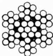
FIG. 2.704.—Rope type of stranded copper cable which is used when a high degree of flexibility is required. The construction of this cable is the stranding together of seven groups, each containing seven wires and producing a total of 49 wires. In cases when a greater carrying capacity is desired than can be obtained through the use of the 7 \times 7 or 49 wire cable, the number of groups is increased to nineteen thereby making a total of 133 wires ( 19 \times 7 ).
