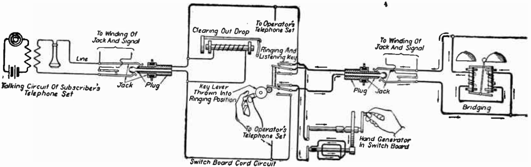
FIG. 2,989.—How the magneto system works: 4. Ringing the desired subscriber. After learning the number of the desired subscriber, the operator takes the other plug of the pair used in answering (known as the calling plug) and inserts it into the desired subscriber's jack. She next throws the cam, previously used for listening, in the opposite direction, which act dis-bell. The arrows indicate the path of the ringing current.
