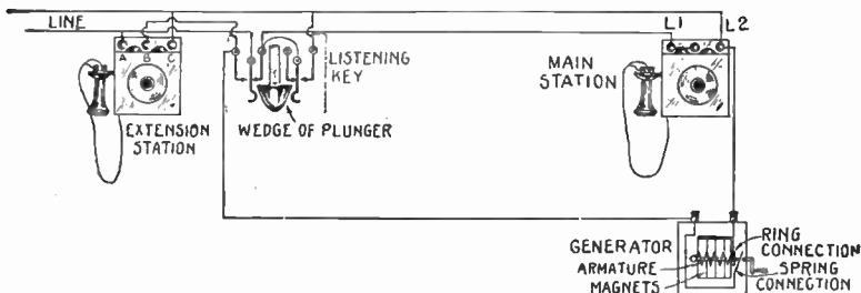
Fig. 2,948.—Wiring diagram showing two common battery instruments wired so that only one bell at a time can be rung by central. With the listening key normal (as shown) central can ring only the main station bell but the extension can talk, and by throwing the listening key, the main is completely cut out and allows only the extension to ring and talk. The ringing key must be thrown to ring the extension station from the main, which makes the system intercommunicating. This is called plan 3 by the New York Telephone Co. The generator posts are connected between posts B and C of the extension but it does not short circuit the line because the spring connection is open, as shown, until the handle is turned which renders it operative.
