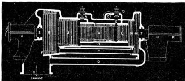
FIG. 2,748. —Longitudinal section of elementary Parsons type steam turbine. The turbine consists essentially of a fixed casing, or cylinder, and a revolving spindle or drum. The ends of the spindle are extended in the form of a shaft, carried in two bearings A and B, and, excepting the small parts of the governing mechanism and the oil pump, these bearings are the only rubbing parts in the entire turbine. Steam enters from the steam pipe at C and passes through the main throttle or regulating valve D, which, as actually constructed, is a balanced valve. This valve is operated by the governor through suitable controlling mechanism. The steam enters the cylinder through the passage E and, turning to the left passes through alternate stationary and revolving rows of blades, finally emerging from them at F and flowing through the connection G to the condenser or to the atmosphere, depending upon whether the turbine is condensing or non-condensing. Each row of blades, both stationary and revolving, extends completely around the turbine and the steam flows through the full annulus between the spindle and the cylinder. In an ideal turbine the lengths of the blades and the diameter of the spindle which carries them would continuously and gradually increase from the steam inlet to the exhaust. Practically, however, the desired effect is produced by making the spindle in steps, there being generally three such steps or stages, H, J and K. The blades in each step are arranged in groups of increasing length. At the beginning of each of the larger steps, the blades are usually shorter than at the end of the preceding smaller step, the change being made in such a way that the correct relation of blade length to spindle diameter is secured. The steam, acting as previously described, produces a thrust tending to force the spindle toward the left, as seen in the cut. This thrust, however, is counteracted by the "balance pistons," L, M and N, which are of the necessary diameter to neutralize the thrust on the spindle steps, H, J and K, respectively. These elements are called "pistons" for convenience, although they do not come in contact with the cylinder, but both the pistons and the cylinder are provided with alternate rings which form a labyrinth packing to retard the leakage of steam. In order that each balance piston may have the proper pressure on both sides, equalizing passages O, P and Q are provided connecting the balance pistons with the corresponding stages of the blading: The end thrust being thus practically neutralized by means of the balance pistons, the spindle "floats" so that it can be easily moved in one direction or the other. In order to definitely fix the position of the spindle, a small adjustable collar bearing is provided at R, inside the housing of the main bearing B. This collar bearing is adjustable so as to locate and hold the spindle in such position so that there will be such a clearance between the rings of the balance piston and those of the cylinder, that the leakage of steam will be reduced to a minimum and, at the same time, prevent actual contact under varying conditions of temperature. Where the shaft passes out of the cylinder, at S and T, it is necessary to provide against in-leakage of air or out-leakage of steam by means of glands. These glands are made tight by water packing without metallic contact. The shaft of the turbine is extended at U and coupled to the shaft of the alternator by means of a flexible coupling. The high pressure turbines are so proportioned that, when using steam as previously described, they have enough capacity to take care of the ordinary fluctuations of load when controlled by the governor through the valve D, thus insuring maximum economy of steam consumption at approximately the rated load. To provide for overloads, the valve V is supplied to admit steam to an intermediate stage of the turbine. This valve shown diagrammatically in the illustration, is arranged to be operated by the governor and is, according to circumstances, located either as shown by the illustration, or at another stage of the turbine.
