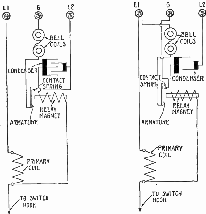
FIG. 2,960.—Wiring diagram of four party line M bell station showing the primary of the induction coil, the selective ringing relay and the condenser connected in series across the line. One end of the bell coil connects with L2 post and the other end connects with the relay armature. When this armature is held up against its contact spring, the bell circuit is complete to G post, and rings through ground.
