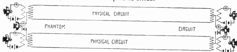
FIG. 2,982. —Wiring diagram showing phantom circuit . As shown, two telephone stations are connected by metallic circuits through toll switchboards to two other distant stations. A repeating coil is inserted at each end of each metallic circuit. At each telephone station, the two line wires from a third telephone station are connected to the middle of each repeating coil. Telephone conversation can therefore be carried on over the phantom circuit without disturbance from the two physical circuits because the two halves of the repeating coils oppose one another. Receivers R and transmitters are connected in series.
