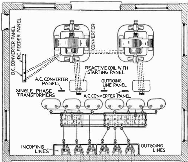
FIG. 2,776.—Plan of small sub-station with single phase oil insulated self-cooling transformers and hand operated oil switches 11,000 or 13,200 volts, overhead high tension lines.
