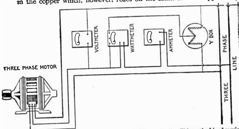
FIG. 2,884. —Three phase motor, one wattmeter and Y box method. This method is of service only, provided the voltages of the three phases are the same. A slight variation of the voltage of the different phases may cause a very large error in the readings of the wattmeter, and inasmuch as the voltage of all commercial three phase circuits is more or less unbalanced, this method is not to be recommended for motor testing. With balanced voltage in all three phases, the power is that indicated by the wattmeter, multiplied by three. Power factor may be calculated as before.
