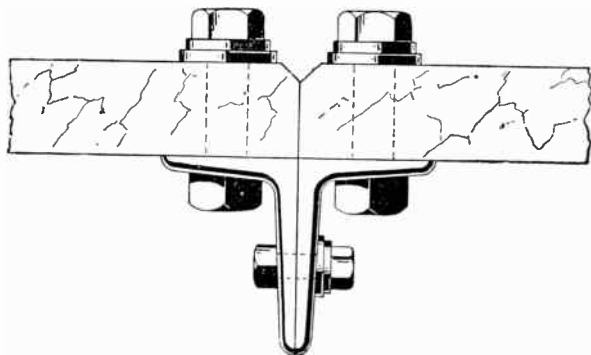
FIG. 2.819.—Method of joining adjacent switchboard panels.
