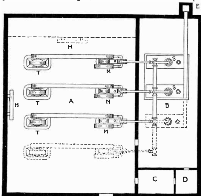
FIG. 2,731. —Plan of electrical station with belt drive without counter shaft. The installation here represented consists of two boilers, S, etc., and three sets of engines and generators, T, M, etc. Sufficient allowance has been made in the plans, however, for future increase of business, as additional space has been provided for an extra engine and generator set, as indicated by the dotted lines.
