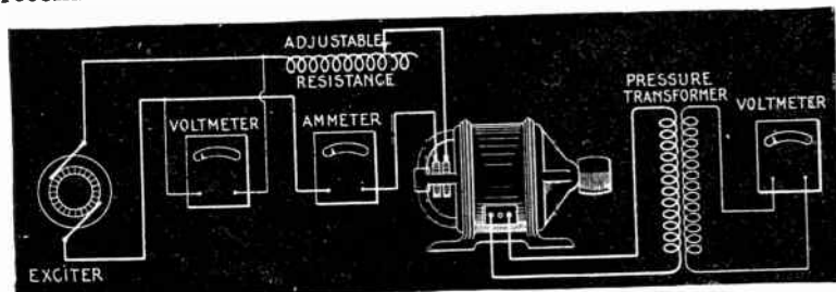
FIG. 2,784.—Diagram of connections for testing to obtain the saturation curve of an alternator. The saturation curve shows the relation between the volts generated in the armature and the amperes of field current (or ampere turns of the field) for a constant armature current. The armature current may be zero, in which case the curve is called no load saturation curve , or sometimes the open circuit characteristic curve . A saturation curve may be taken with full load current in the armature; but this is rarely done, except in alternators of comparatively small output. If a full load saturation curve be desired, it can be approximately calculated from the no load saturation curve. The figure shows the connections. If the voltage generated is greater than the capacity of the voltmeter, a multiplying coil or a step down pressure transformer may be used, as shown. A series of observations of the voltage between the terminals of one of the phases, is made for different values of the field current. Eight or nine points along the curve are usually sufficient, the series extending from zero to about fifty per cent. above normal rated voltage. The points should be taken more closely together in the vicinity of normal voltage than at other portions of the curve. Care must be taken that the alternator is run at its rated speed, and this speed must be kept constant. Deviations from constant speed may be most easily detected by the use of a tachometer. If the machine be two phase or three phase, the voltmeter may be connected to any one phase throughout a complete series of observations. The voltage of all the phases should be observed for normal full load excitation by connecting the voltmeter to each phase successively, keeping the field current constant at normal voltage. This is done in order to see how closely the voltage of the different phases agree.
