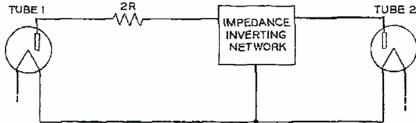
Fig. 3—Fundamental form of a high-efficiency circuit.
