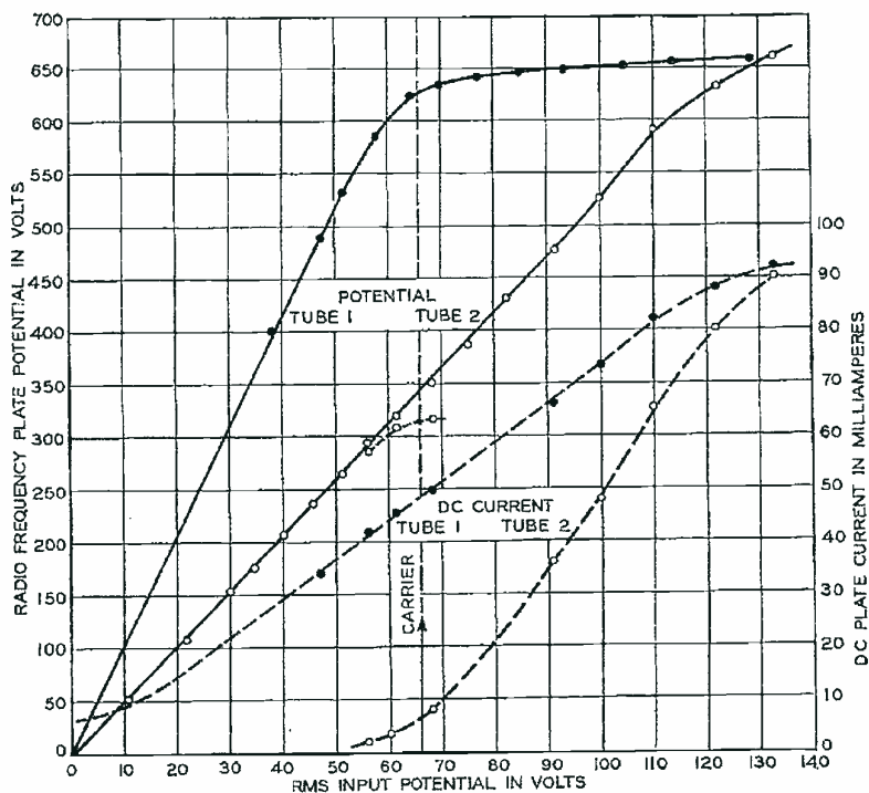
Fig. 11—Typical experimental results.
