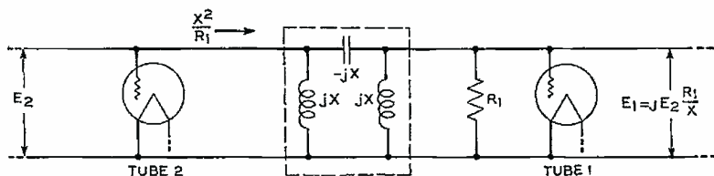
Fig. 10—Grid exciting circuit.
