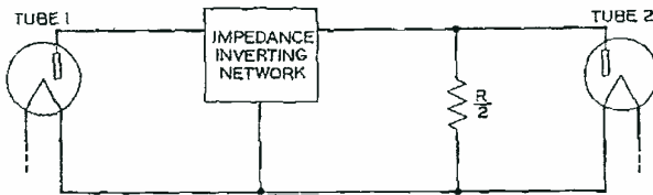
Fig. 4—Second fundamental form of high-efficiency circuit.
