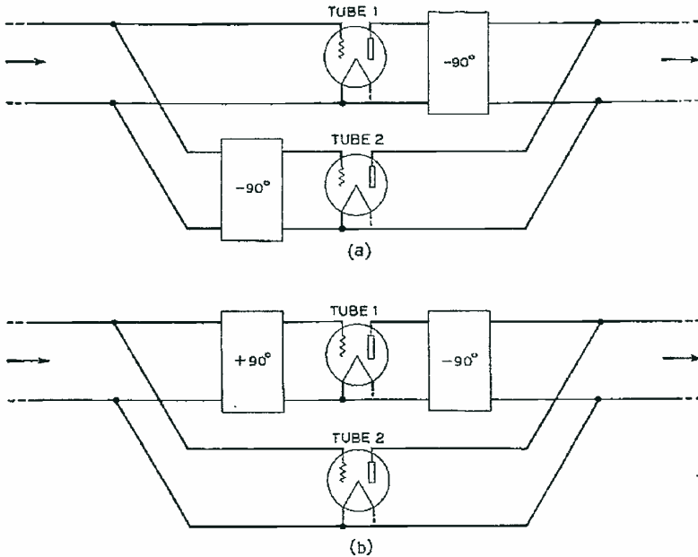
Fig. 9—Alternative arrangements of the grid phase-shifting network.
