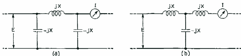
Fig. 7—Typical impedance-inverting networks.
