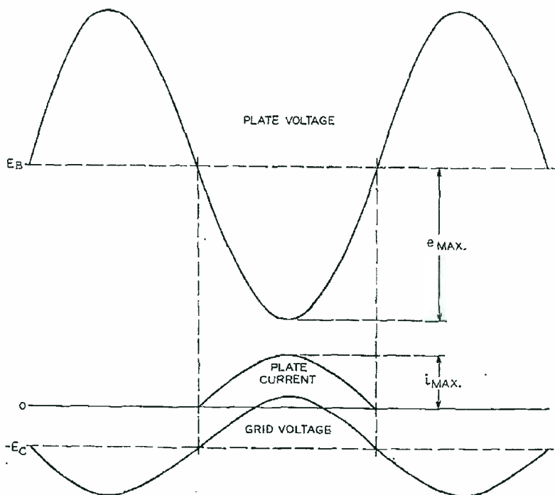
Fig. 1—Operating conditions in a linear power amplifier.
