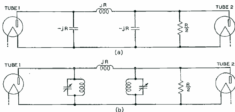
Fig. 8—Evolution of the output circuit.
