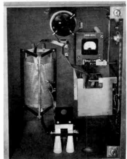
Fig. 7-5. A typical antenna tuning unit. The lighting choke is at the top of the cabinet.
