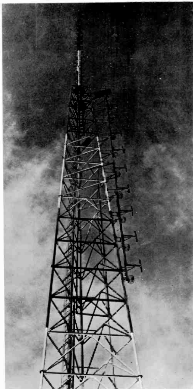
Fig. 8-5. Dual polarized antenna radiators side-mounted on an existing TV tower as an interlaced system.
