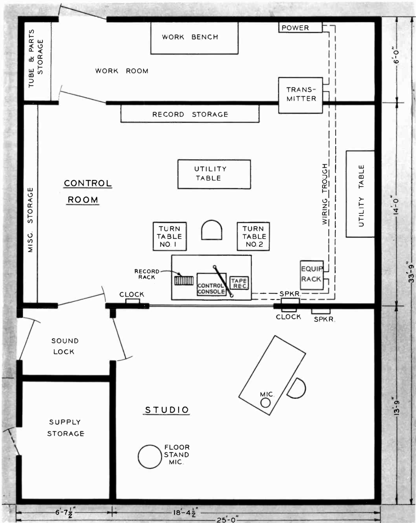
Fig. 4-2. Another desirable layout for "Plan 1."
