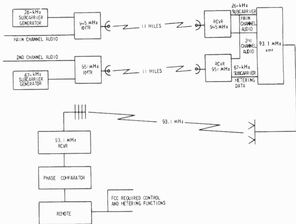
Fig. 9-5. Block diagram of a typical FM remote control system using an STL.
