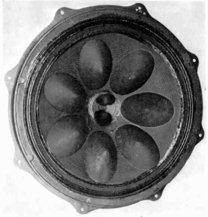
Fig. 10-11. Duo-cone speaker ideal for control room or studio monitoring.
