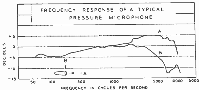
Fig. 12-6. Typical pressure microphone response curve.
