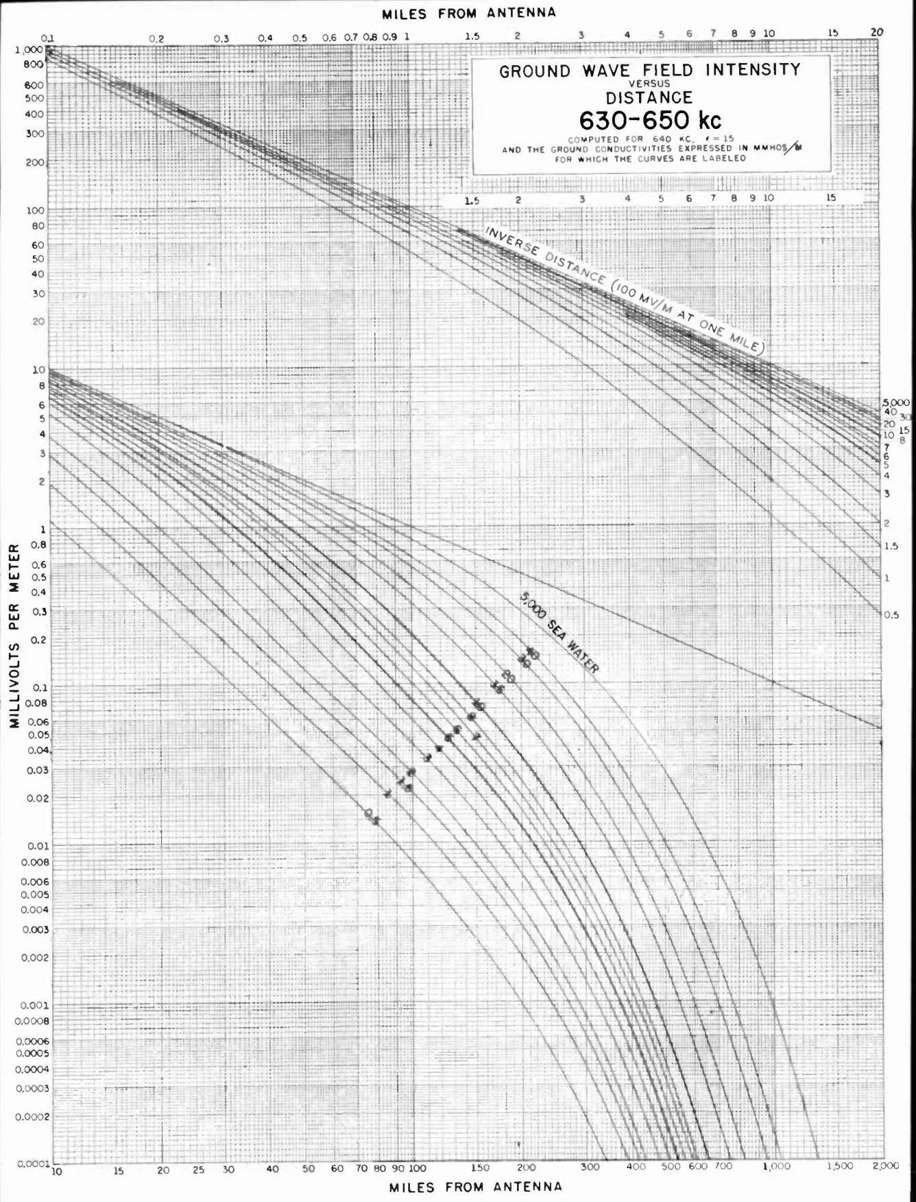
Fig. 2-3. Groundwave field intensity chart.
