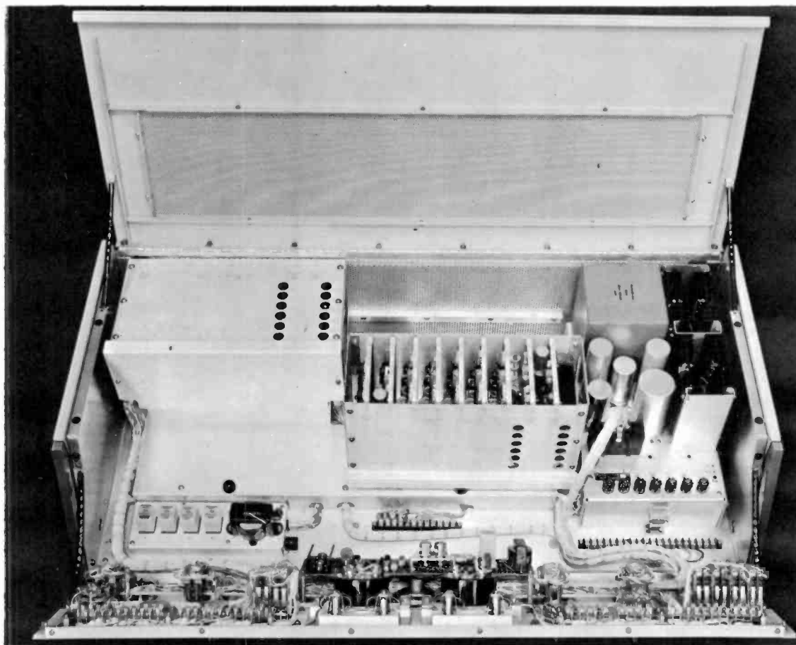
Fig. 10-4. Card box used to mount the plug-in cards.
