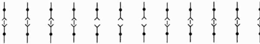
Fig. 6-5. Typical jack panel terminations for "Plan 1 or 2" broadcast stations.
