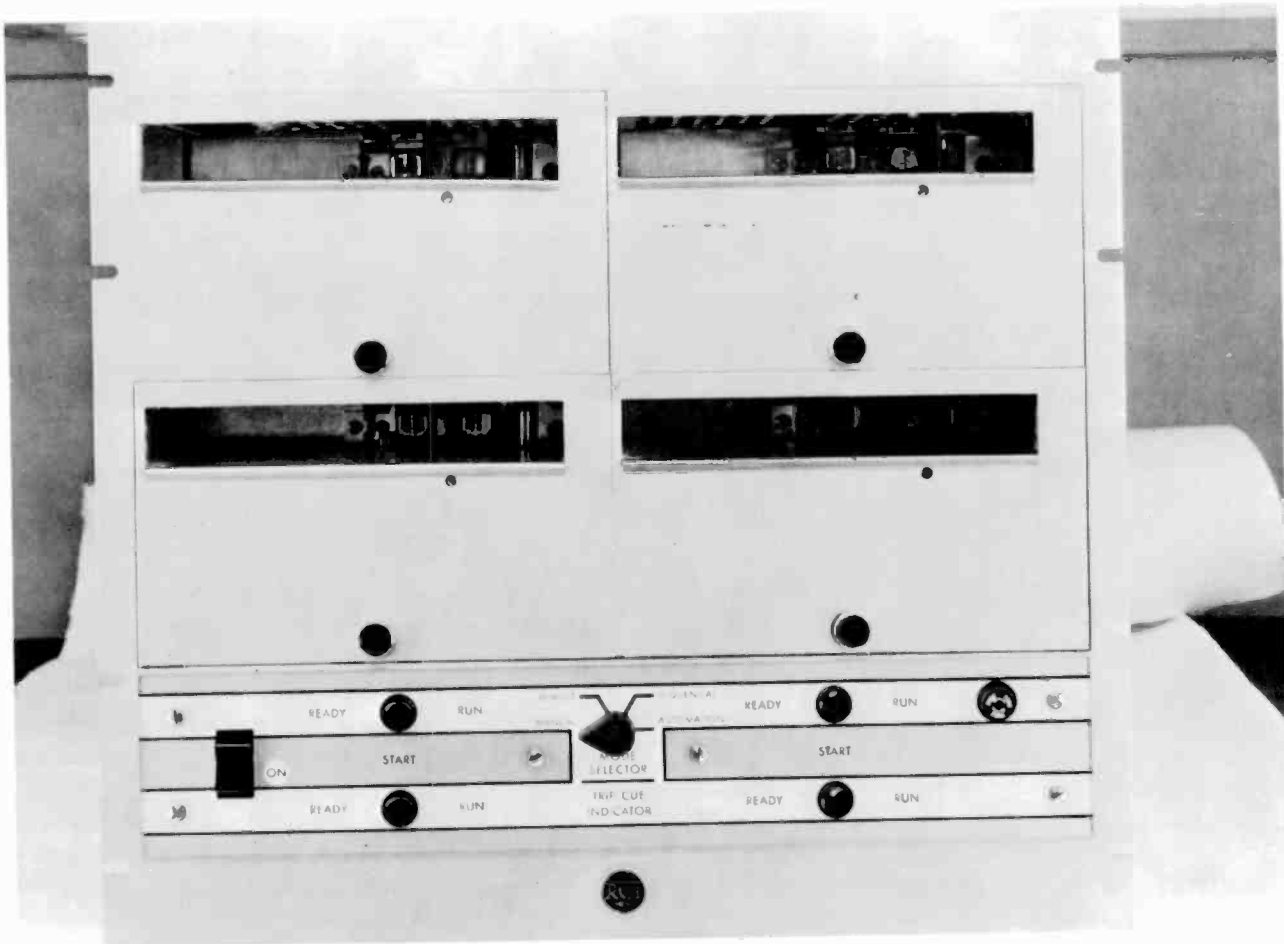
Fig. 11-3. A compact multicartridge tape system used in many semi-automated control rooms.
