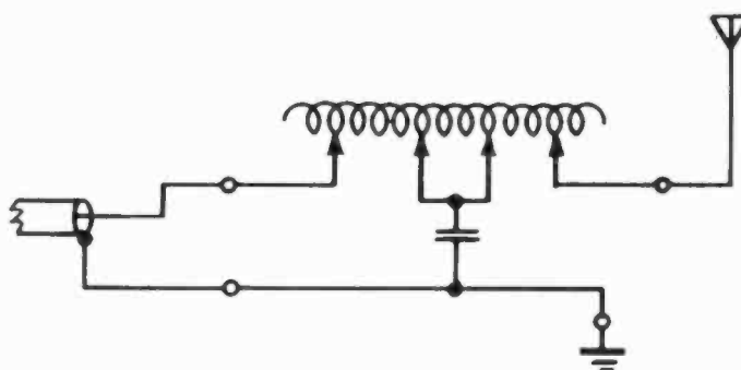
Fig. 7-13. Simplified schematic diagram of a single-tower tuning unit.
