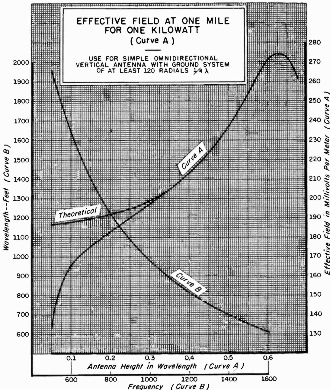
Fig. 3-4. Curve illustrating the requirements for the effective field at one mile.
