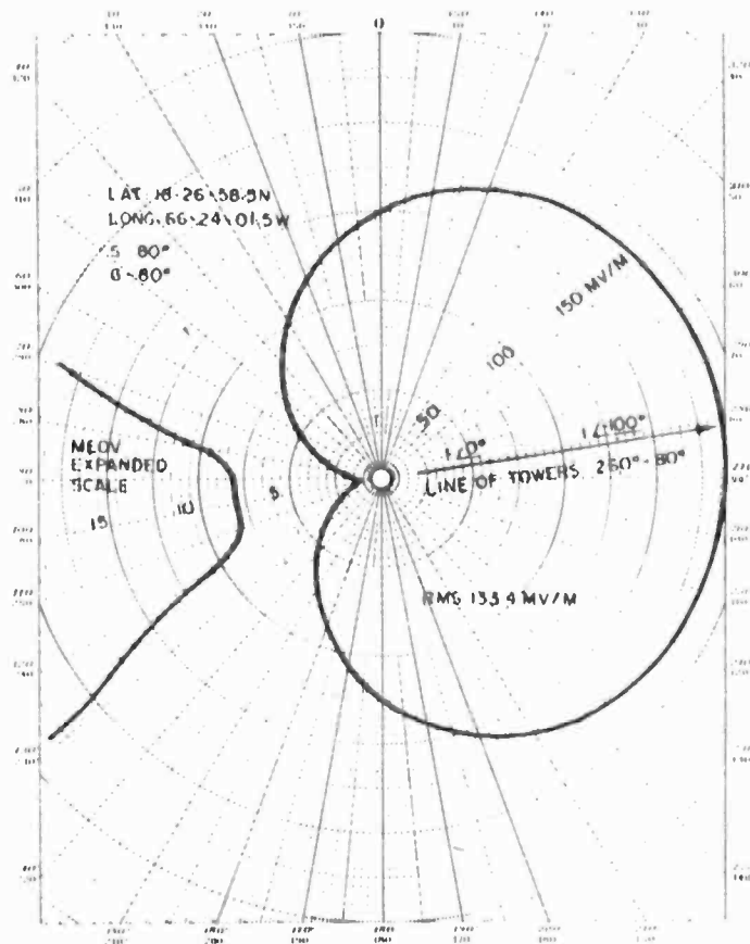
Fig. 7-15. Directional antenna pattern sketch showing protection for stations in Cities B and C.
