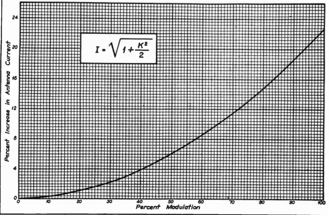
Relation Between Antenna Current and Modulation
