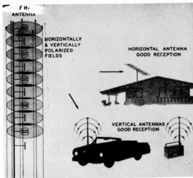
Fig. 8-2. Dual polarized transmission provides excellent reception for all types of receivers.
