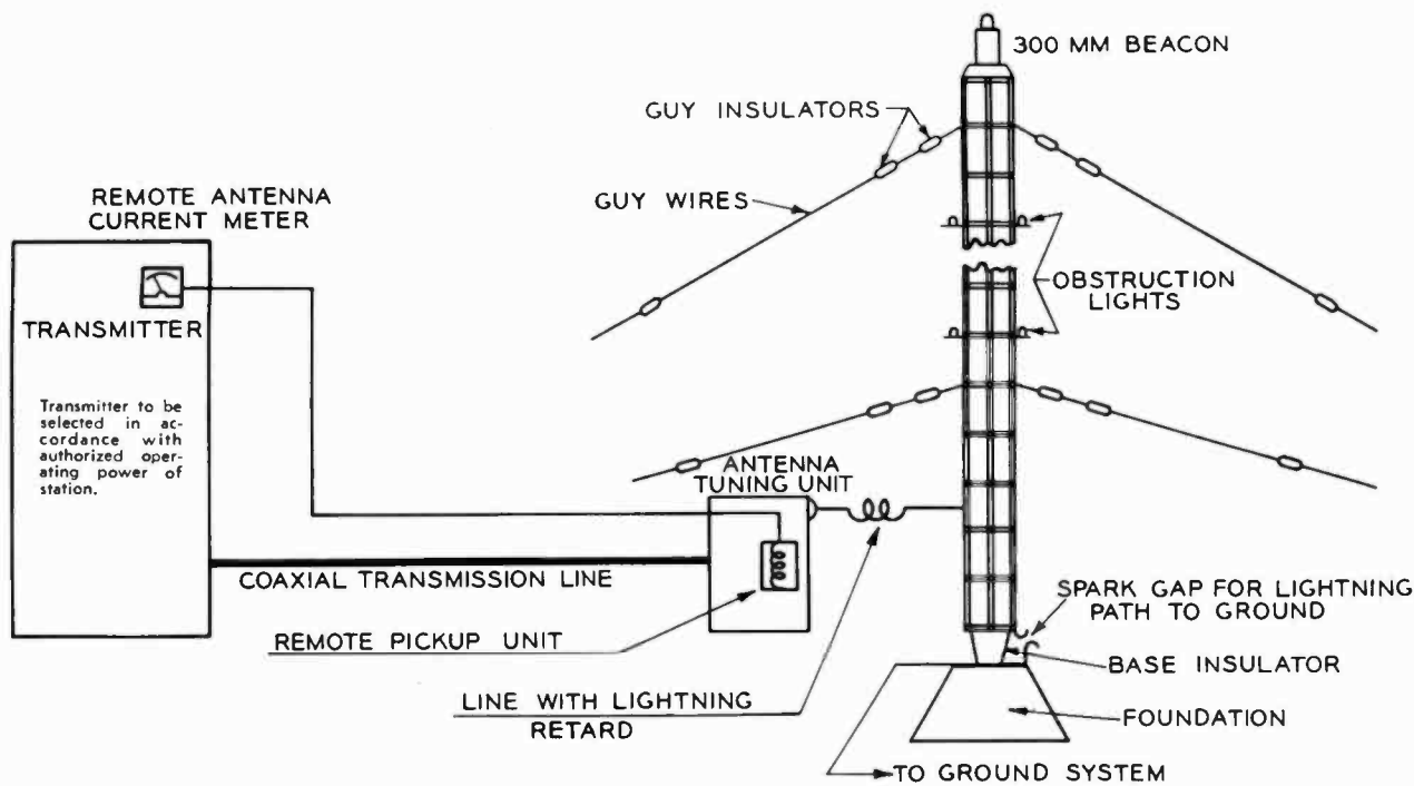
Fig. 7-8. A typical single-tower AM system. The remote antenna current is measured at the transmitter. Observe the position of the tower lights.
