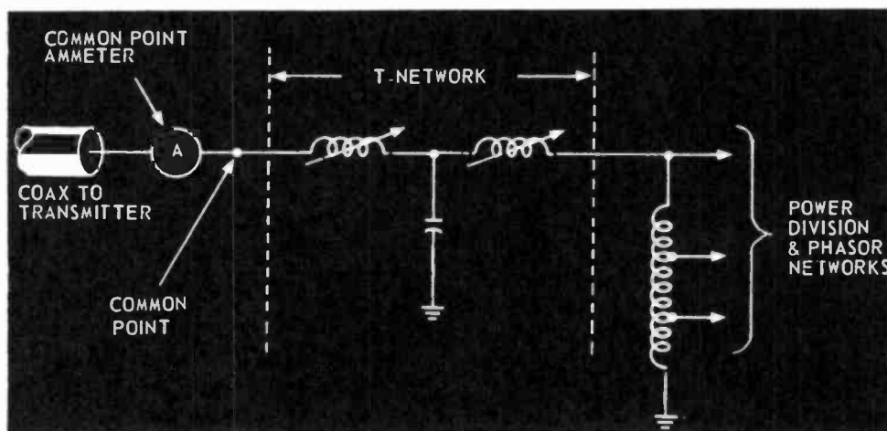
Fig. 7-14. Common-point circuit schematic showing location of the ammeter.
