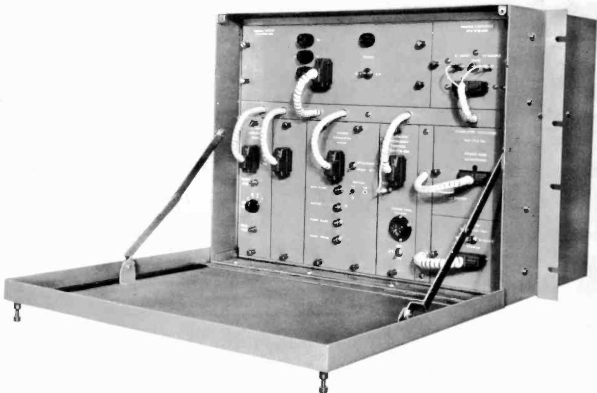
Fig. 13-8. A typical solid-state FM exciter.
