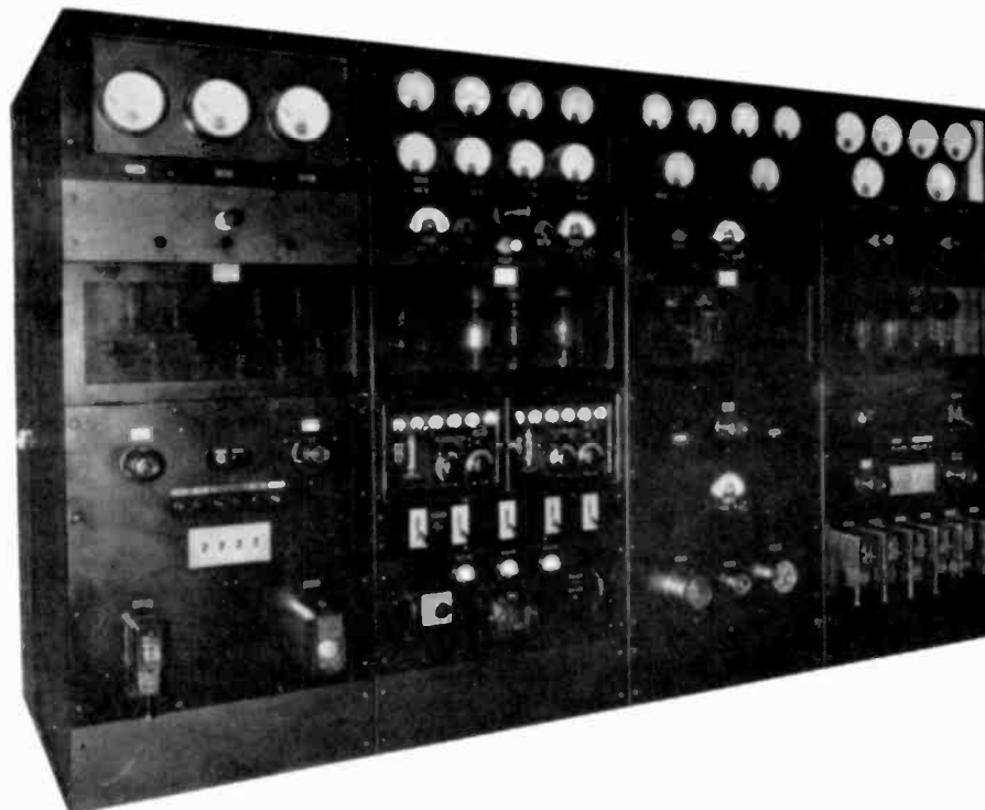
Fig. 1-2. This 5-kilowatt broadcast transmitter was "the equipment" at the time broadcasting was in its infancy.
