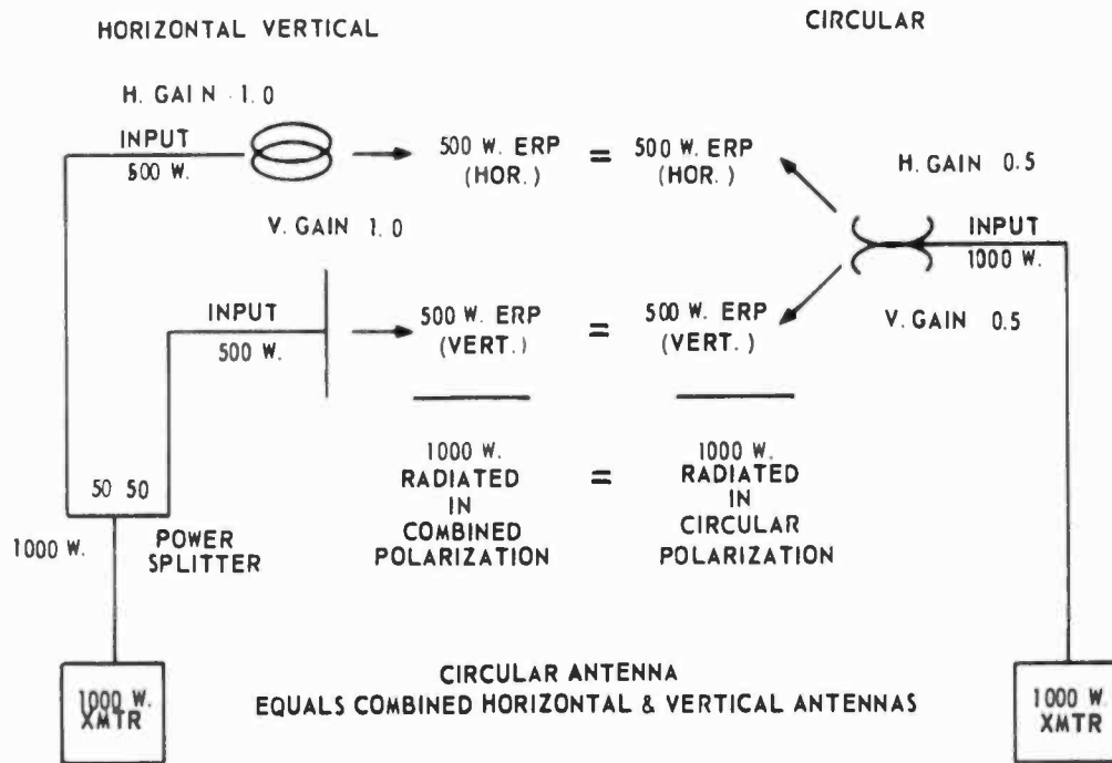
Fig. 8-9. Comparison of feed systems and the effective radiated power of a circularly-polarized antenna with combined horizontally and vertically polarized antennas. No power splitter is required for the circularly polarized antenna.
