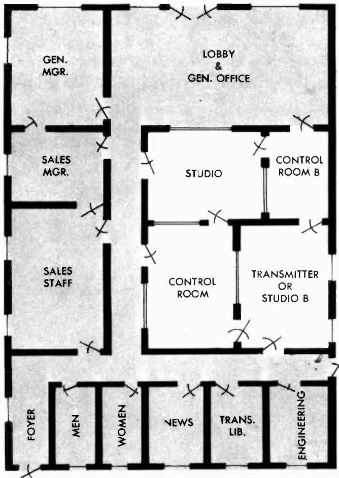
Fig. 4-12. A more desirable version of a "Plan 2" station layout.
