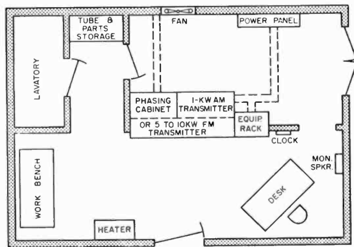
Fig. 5-3. Typical transmitter building layout for a one-kilowatt AM directional. Floor plan can also accommodate up to a 10-KW FM transmitter.
