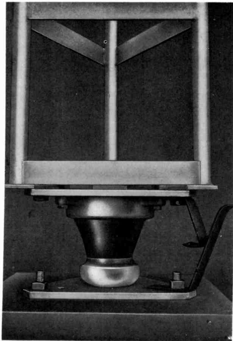
Fig. 5-11. A typical insulated tower base with horn gap across the insulator.
