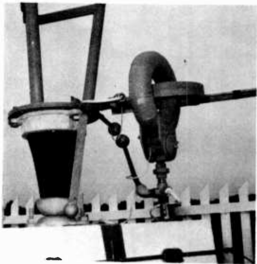
Fig. 7-6. Typical installation of a lighting transformer to isolate the AC circuit from RF.
