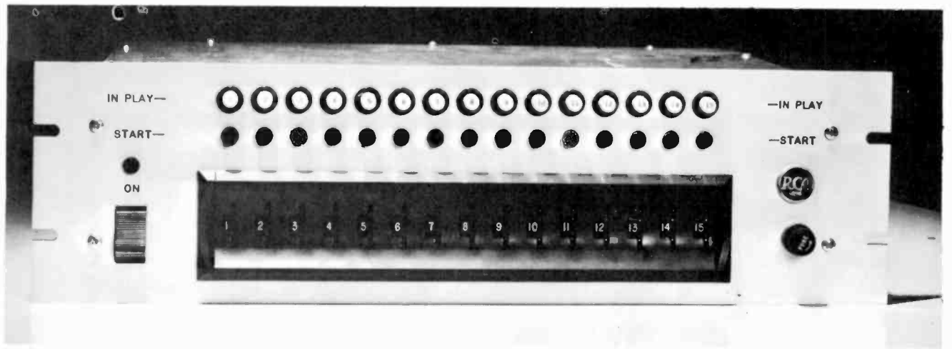
Fig. 11-10. Another automatic programmer.
