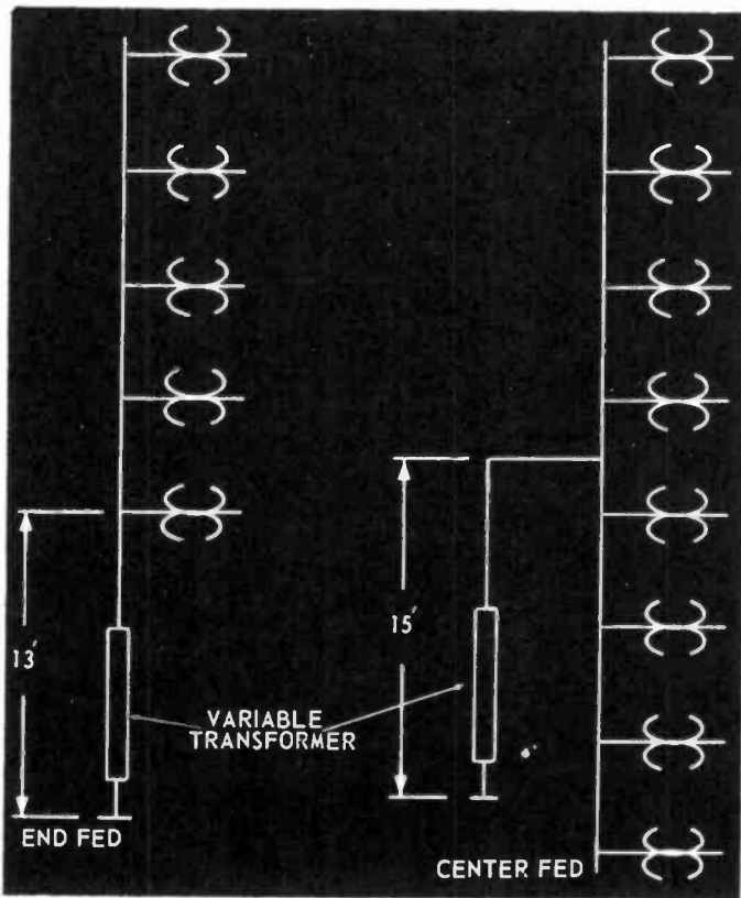
Fig. 8-10. Simplified diagram showing feed line input locations for end-fed and center-fed antennas.
