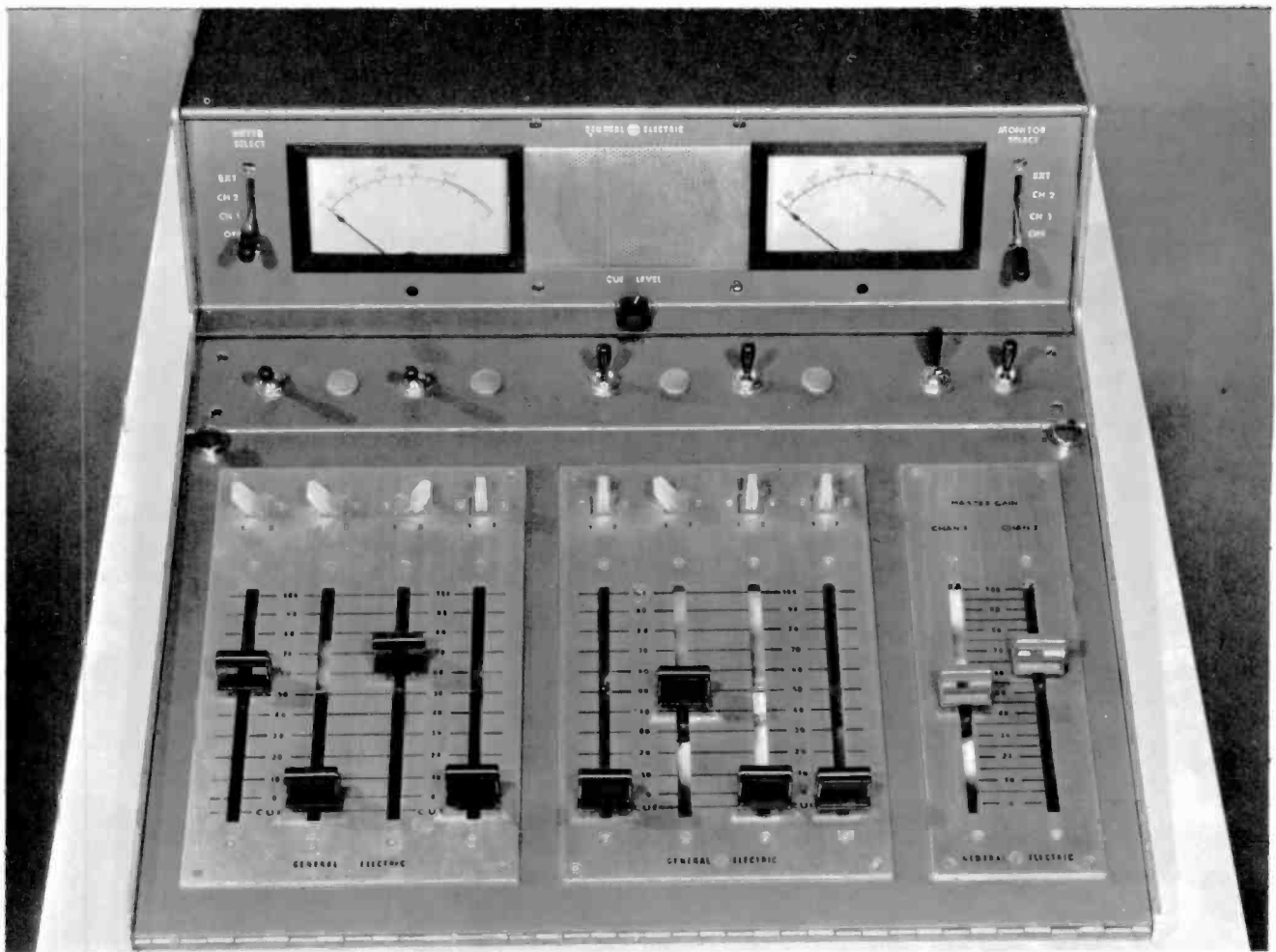
Fig. 10-6. A solid-state monaural audio control console.
