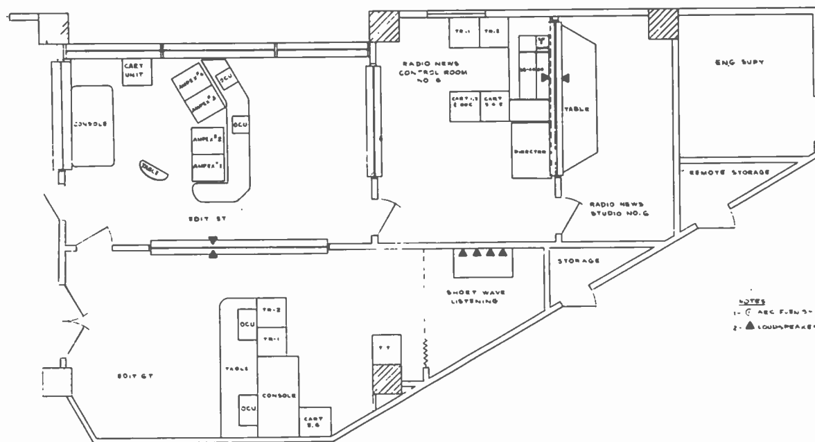
Fig. 16-2. ABC Network Studios, 5, 6, 5T, and 6T.
