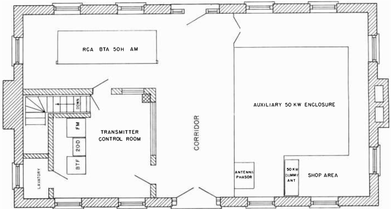
Fig. 16-20. WRVA radio transmitter building floor plan.
