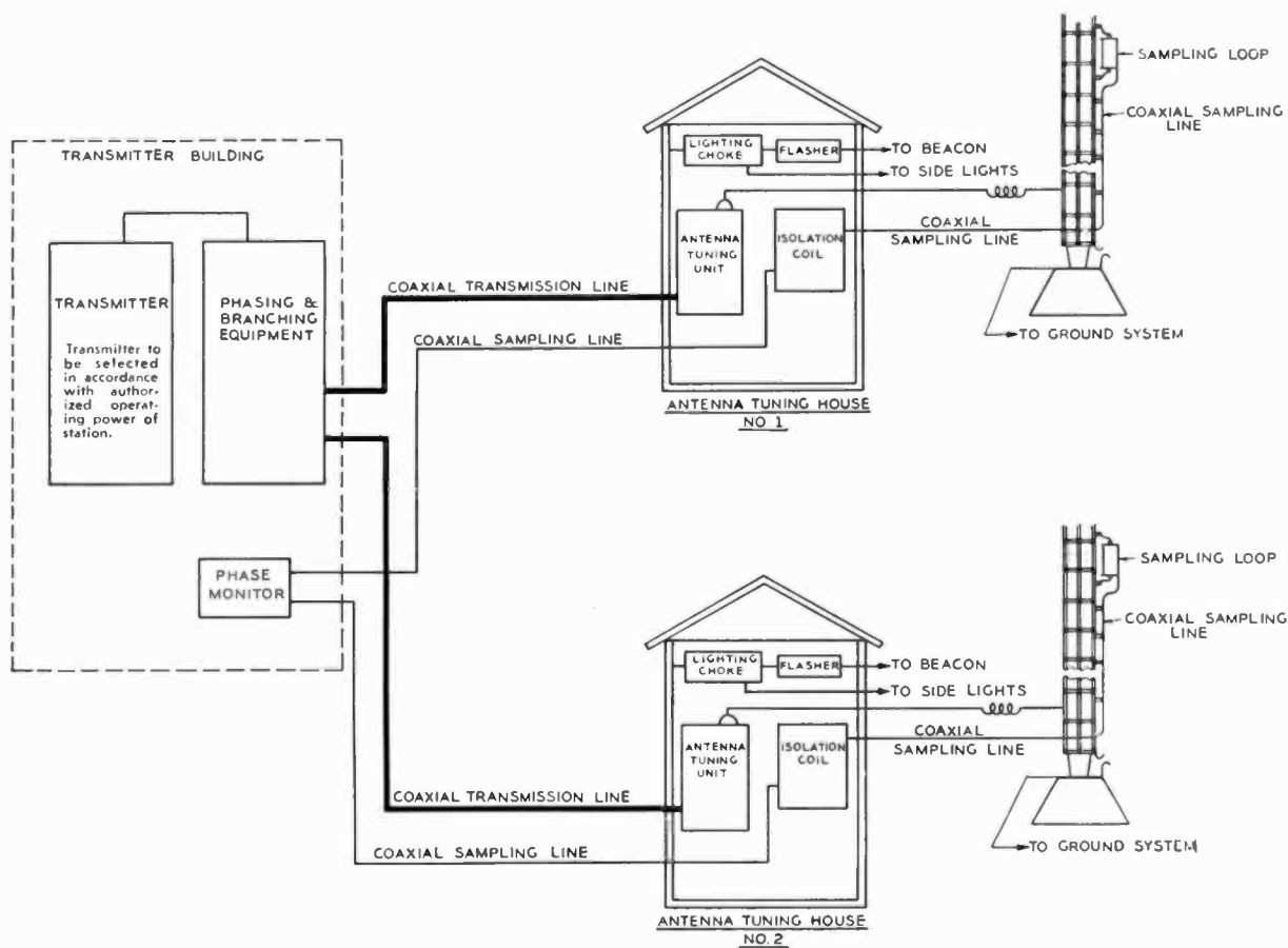
Fig. 7-9. Layout of a typical two-tower directional AM system showing the position of the phasing and branching equipments.
