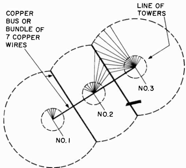
Fig. 7-20. Ground system diagram for a three-tower directional array showing, in part, ground radials which should be bonded in the main copper busses.
