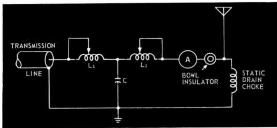
Fig. 7-12. Schematic of a single-tower basic antenna tuning unit.
