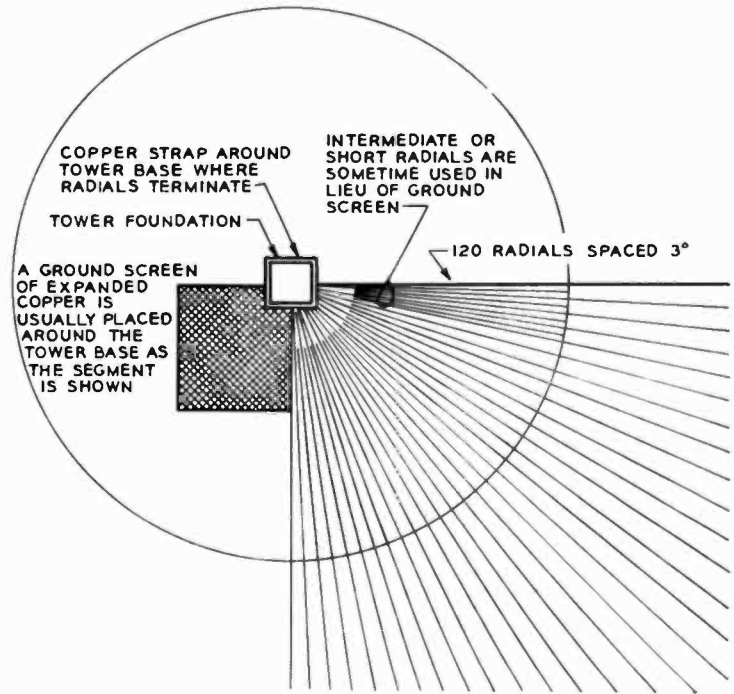
Fig. 7-19. Sketch of a typical single-tower ground system.
