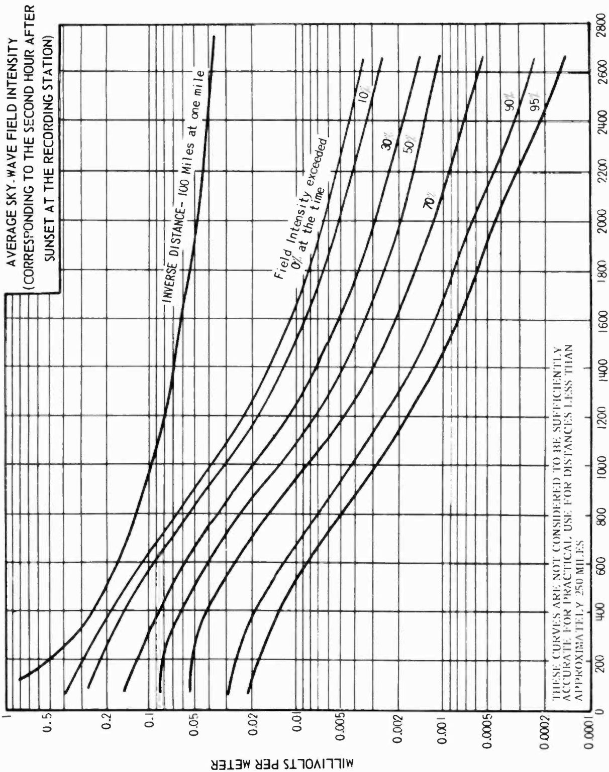
Fig. 2-4. Average skywave field intensity chart.
