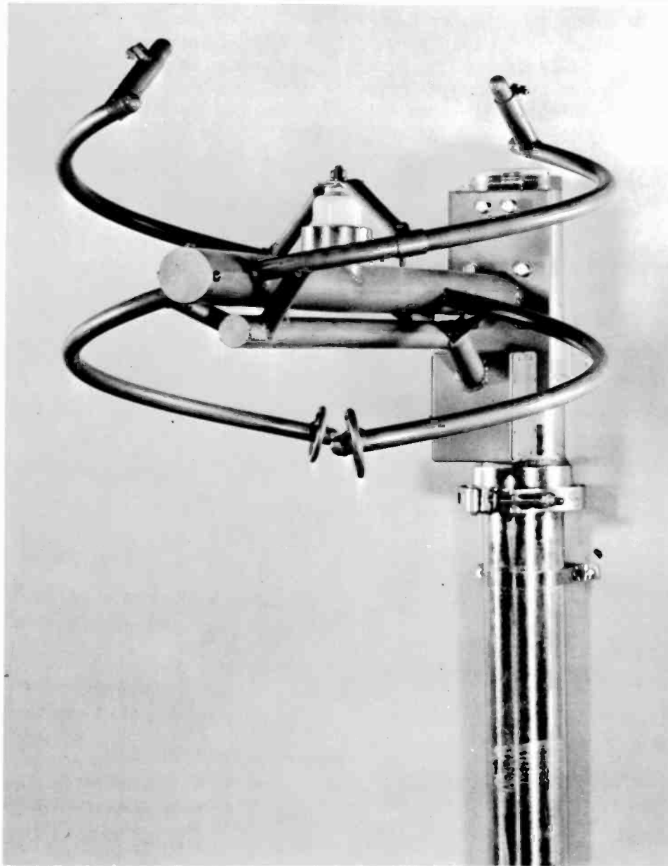
Fig. 8-6. A circularly-polarized antenna replaces horizontal and vertical elements. One antenna does the work of two.
