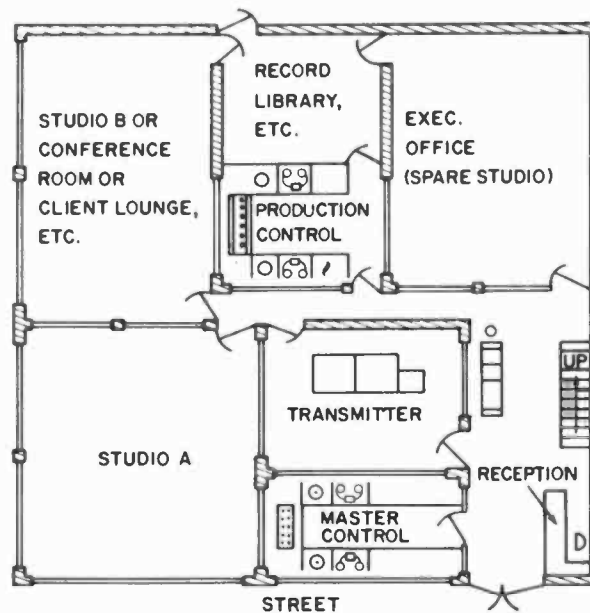
Fig. 4-21. Floor plan designed for operational flexibility (A) and a plan allowing for future expansion (B).
