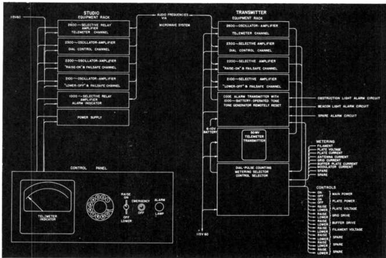
Fig. 9-7. A block diagram of an STL remote control and telemetering system.
