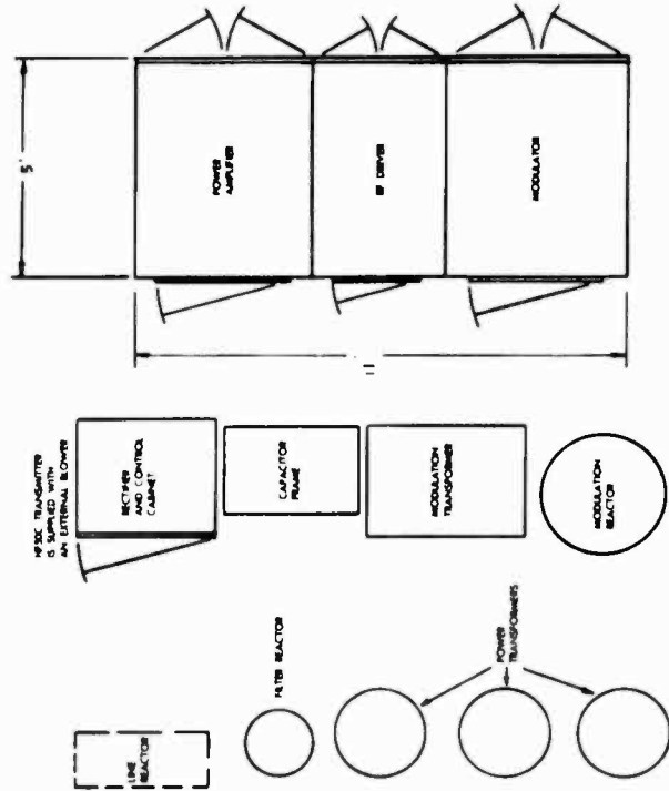
Fig. 5-6. Transmitter building floor plan for a 50-KW AM station.
