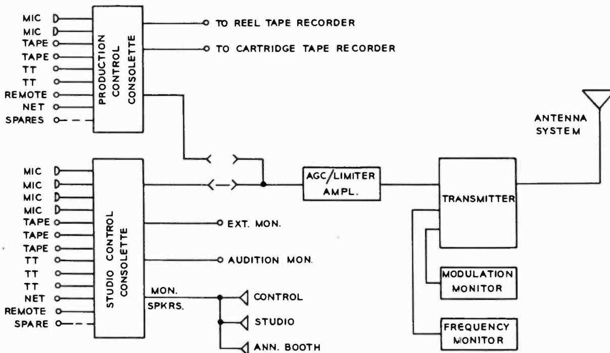
Fig. 4-11. "Plan 2" system block diagram showing how production control can also be patched into output line.
