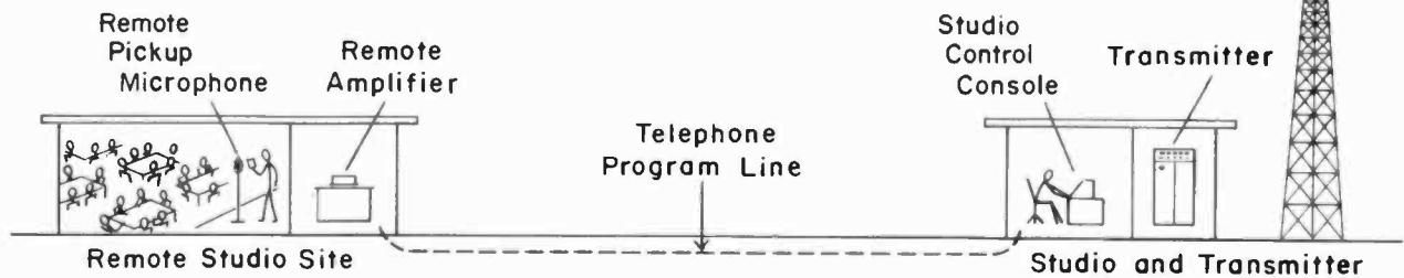
Fig. 1-5. Another variation in separate studio and transmitter facilities: Pickup and control equipment installed in public meeting places provides additional program sources.
