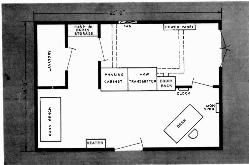
Fig. 5-2. Transmitter plant floor plan for a directional 1-KW attended operation.
