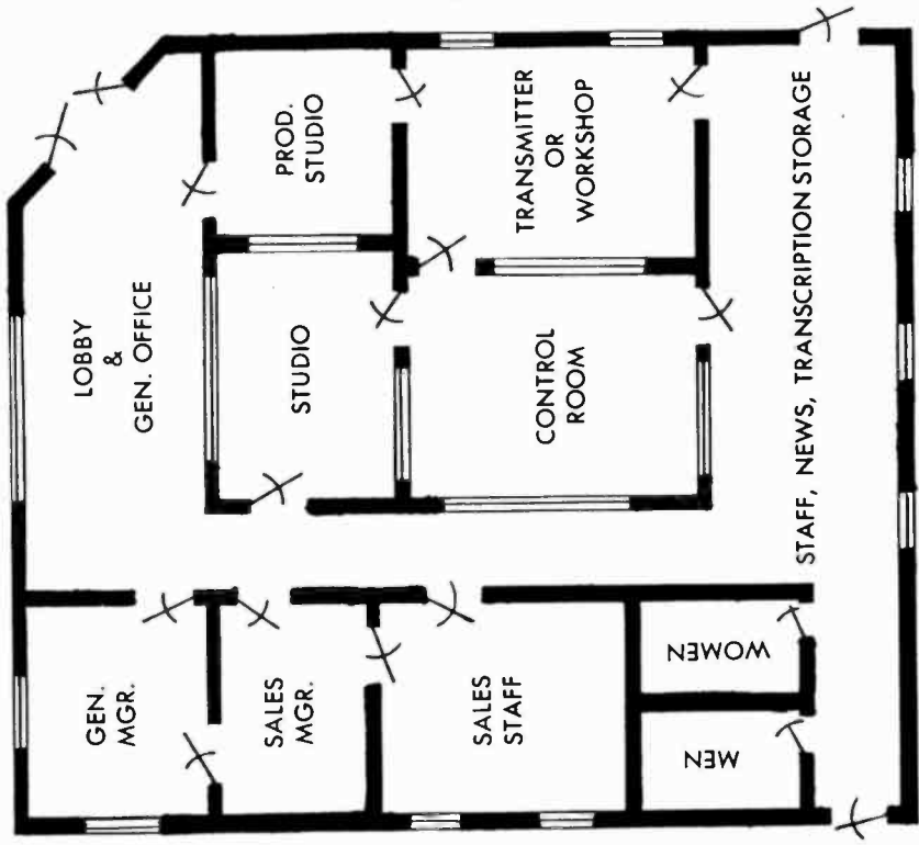
Fig. 4-3. "Plan 1" small-market, minimum-staff layout.
