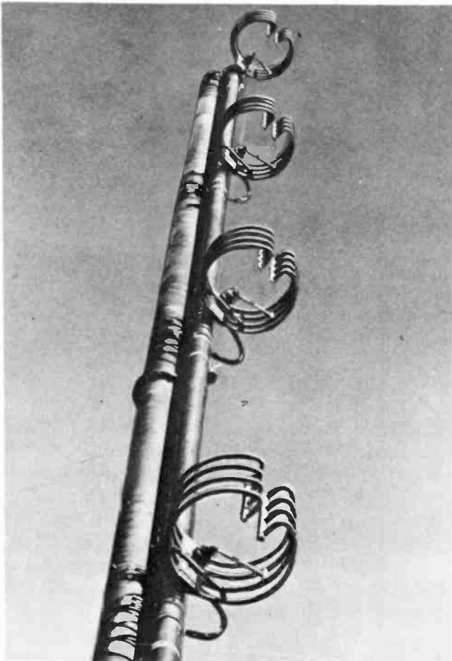
Fig. 8-11. A four-bay horizontally-polarized FM antenna array.
