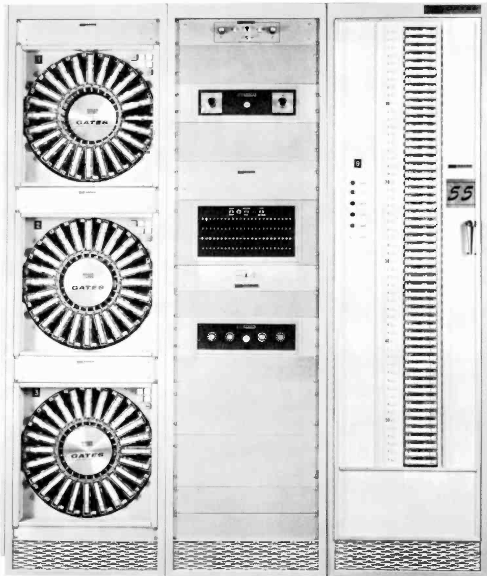
Fig. 11-11. The WVMI automation system, using tape cartridges exclusively.
