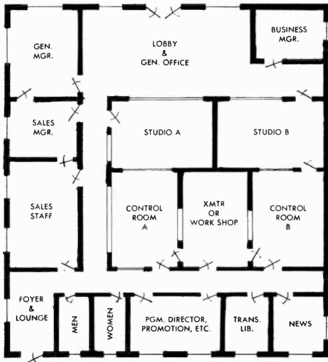
Fig. 4-18. A "Plan 3" layout arranged to suit AM/FM programming.
