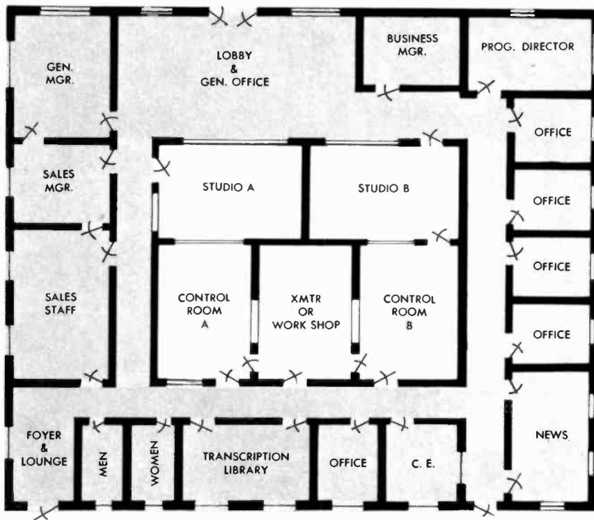
Fig. 4-19. A "Plan 3" metropolitan market layout.
