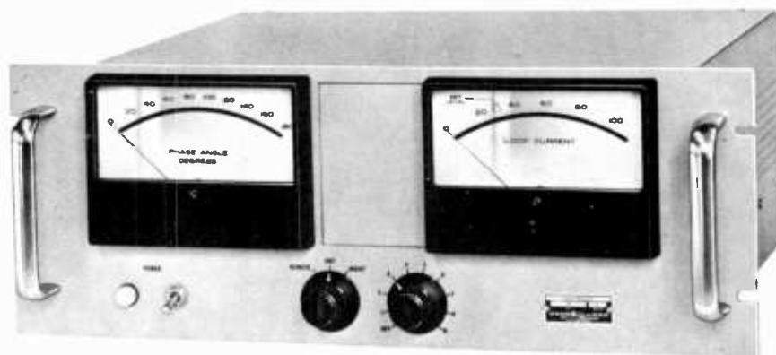
Fig. 7-17. This new solid state phase monitor is designed for multi-tower directional AM system.
