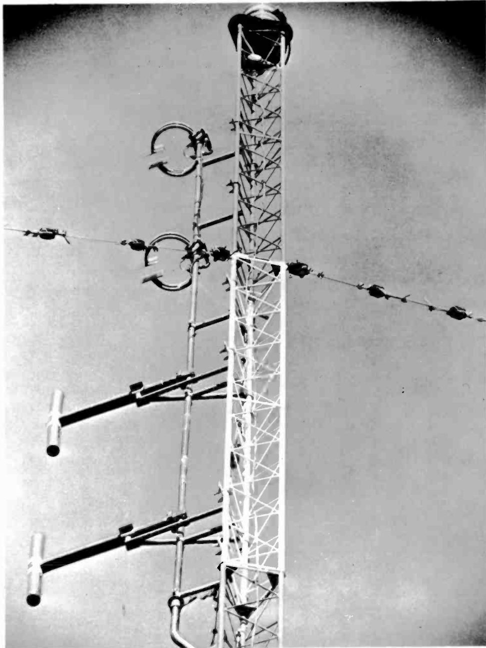
Fig. 8-13. A typical dual-polarized FM antenna array.
