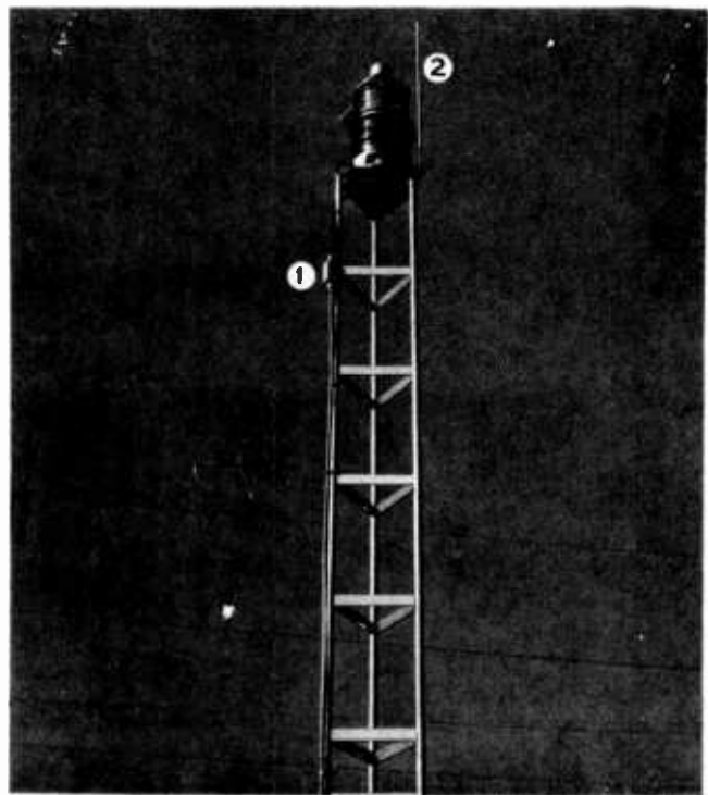
Fig. 7-7. A typical beacon installation. Notice the location of the junction box (1) and the lightning rod protector (2).
