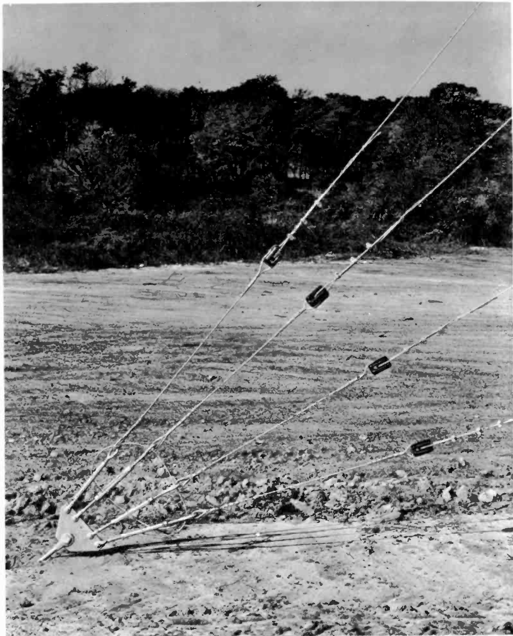
Fig. 5-10. Ground anchor point showing cable looped through turnbuckles to prevent turning.
