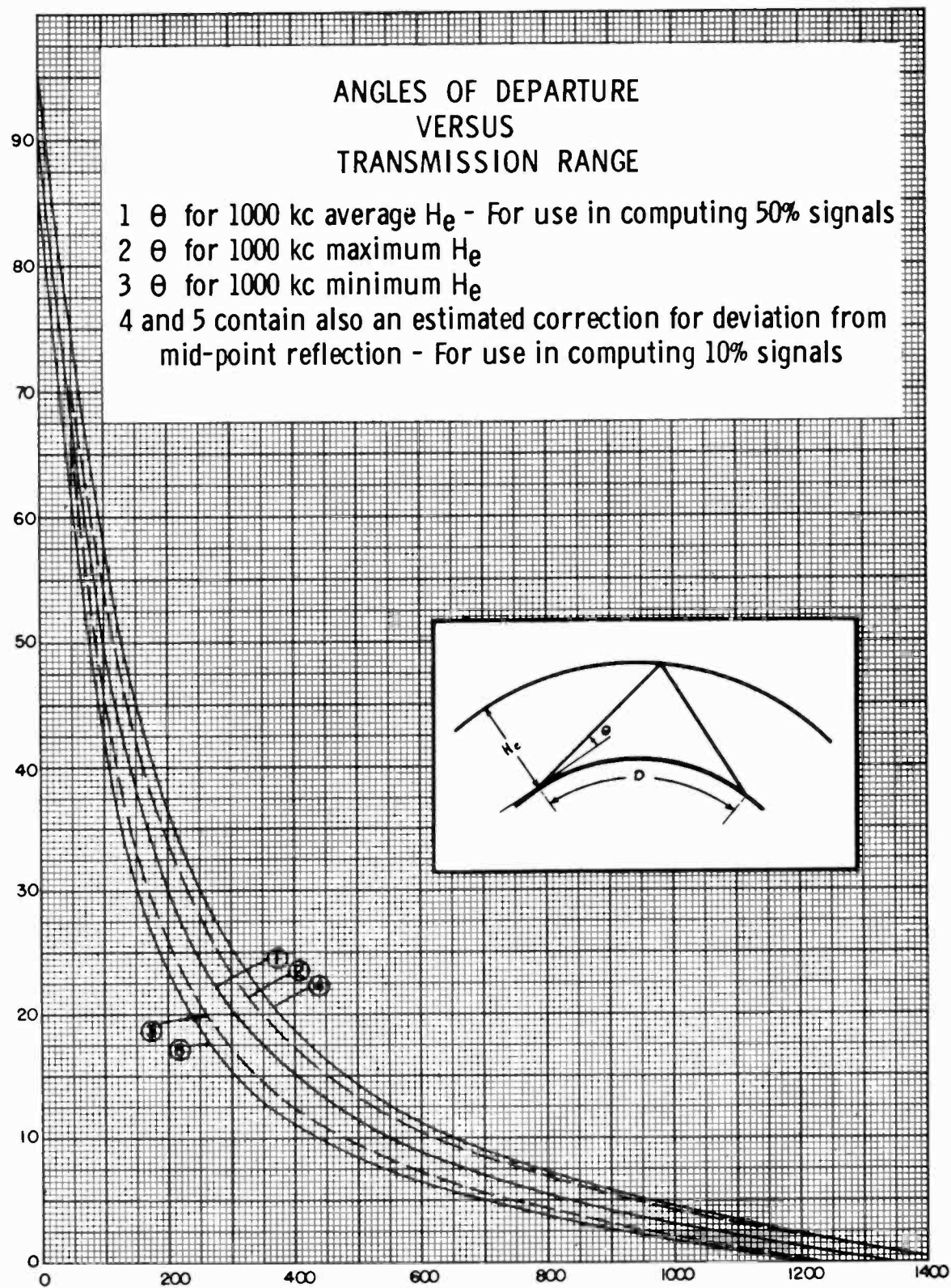
Fig. 2-7. Curves showing angles of departure versus transmission range.
