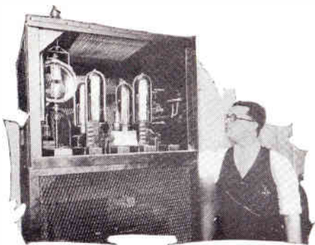
The heart of WRNY's transmitting equipment is shown above. Four large 250 watt vacuum tubes provide the power for putting over the big "kick" at this station. Note the size of tubes as compared with the small receiving tube placed between them.
