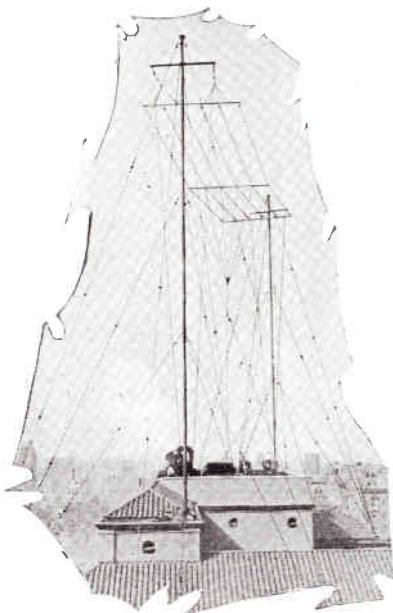
The antenna atop The Roosevelt Hotel, New York, a twenty-story structure, showing the two 125-foot steel masts supported by their many insulated guy wires. The aerial itself is composed of six wires 74 feet long strung between large spreaders.
