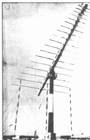
Weight of the LP-antenna 16.4 tn Height of the LP-antenna 23.4 meters Length of the rectangular antenna boom 39.6 meters Maximum width of span of the longest dipole 26.1 meters Maximum diameter of the mast 1.6 meters
