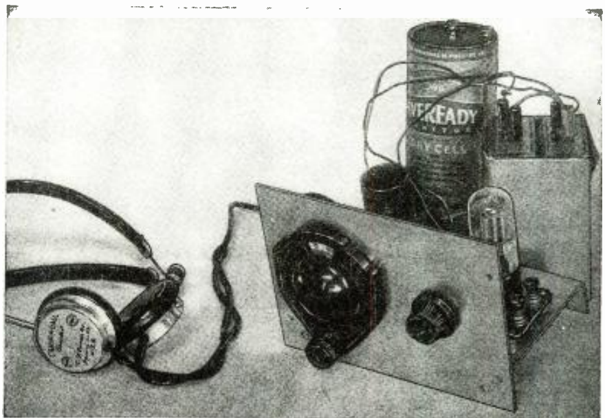
In the modernized Twinplex receiver here shown, one tube does the work of two. Plug-in coils permit all-wave coverage.
