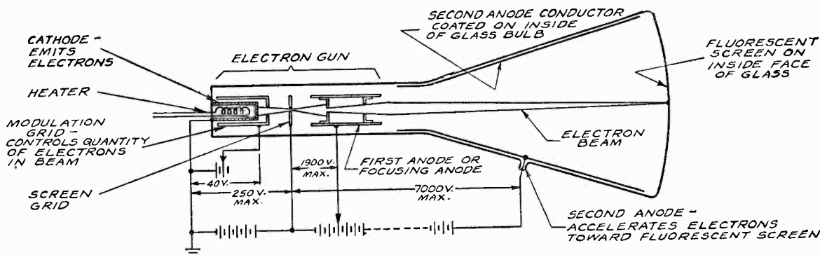
FIG. 6a.—The different elements of a picture tube are designated in the above sketch with typical voltages shown. Fig. 6b on the right shows a common schematic representation; where K is the cathode; G, the modulation grid; S, the screen grid; F, the focusing anode, and A, the second anode.
