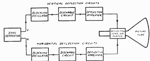
FIG. 52.—Block diagram of the essential parts of a widely-used type of deflection circuit.
