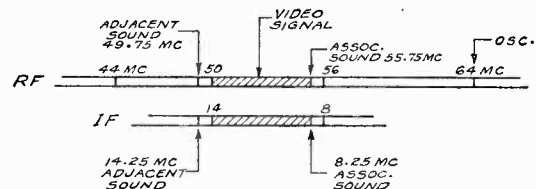
FIG. 32.—The sound signal of the associated channel at 8.25 mc and the sound signal of the adjacent channel at 14.25 mc are both close to the edges of the video band. Traps are provided to prevent interference from these signals.
