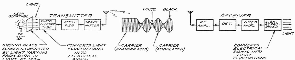
FIG. 1B—TELEVISION TRANSMISSION SYSTEM
