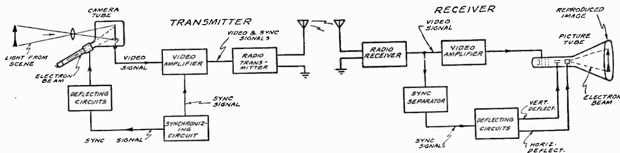
FIG. 16.—The principal elements of a complete television system. Note the provision made for synchronizing the scanning at the picture tube with that at the camera tube.
