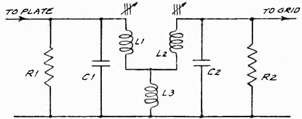
FIG. 35.—A simplified diagram of the video i-f transformers used in RCA television receivers. Direct coupling by the inductance L3 which is common to both primary and secondary circuits.
