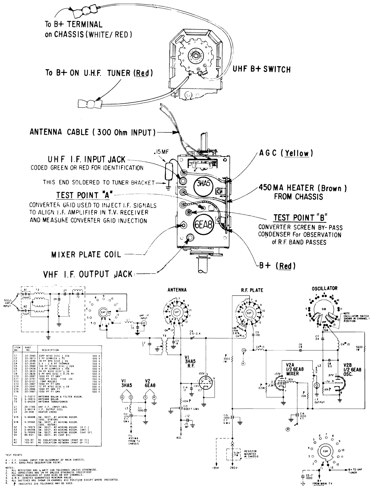
Schematic Diagram and Top View of De Luxe Video VHF Tuner (700 Series) Nos. 175-717 and 175-718.
