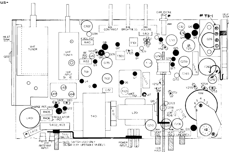
TOP VIEW MAJOR COMPONENT AND ADJUSTMENT LOCATION
