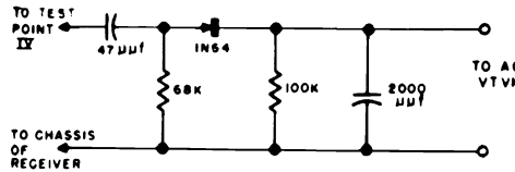
DETECTOR NETWORK
