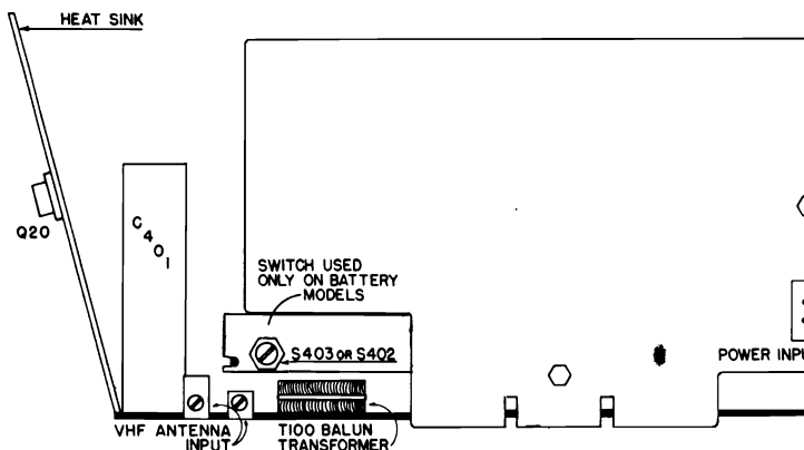
REAR VIEW ADJUSTMENT LOCATION
