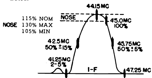
I-F RESPONSE CURVE
