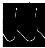
● 48 volts p/p, 15,750 cps
