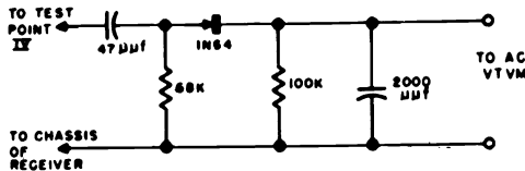
DETECTOR NETWORK
