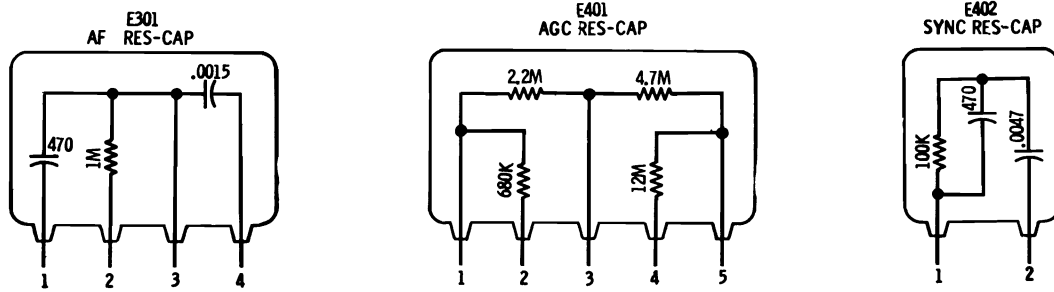
RES-CAP DETAILS
