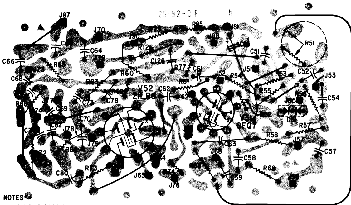
WIRING DIAGRAM I.F. AND SOUND BOARD
