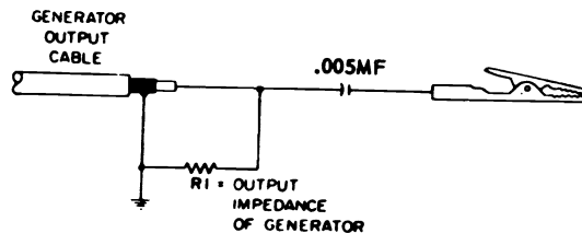
Figure 3. - Generator Cable Termination
