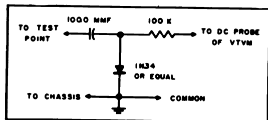
Figure 4 - Diode Detector Detail
