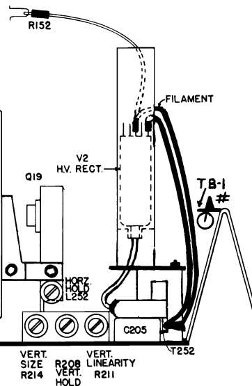
REAR VIEW ADJUSTMENT LOCATION
