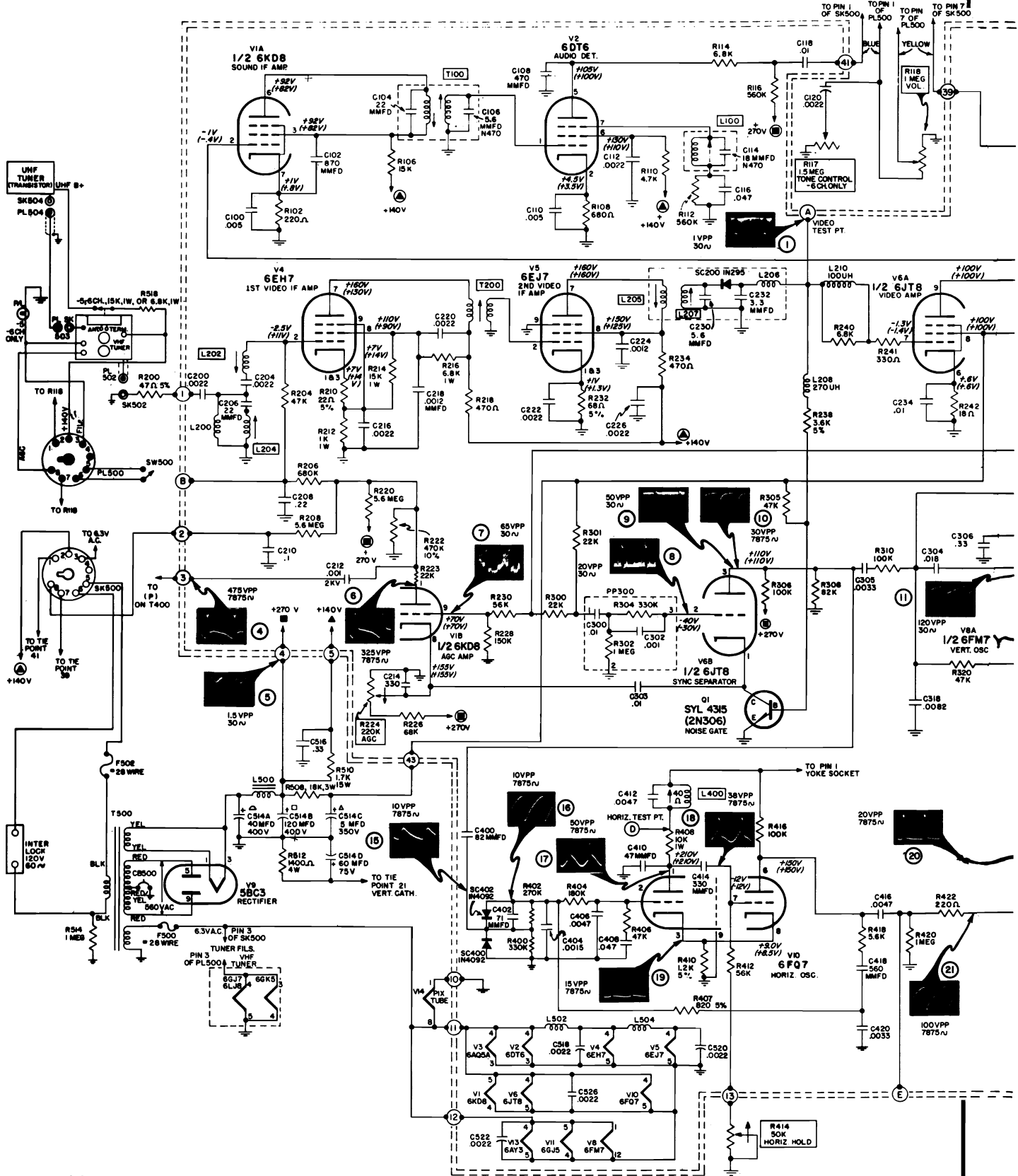
SCHEMATIC DIAGRAM (B04-5,-6)
