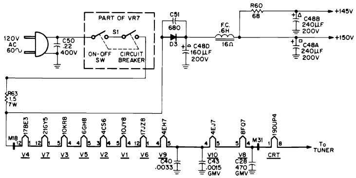
17J27 VOLTAGE AND RESISTANCE CHART
