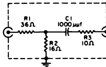
I-F INJECTION NETWORK
