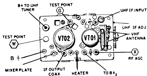
Fig. E TOP DRAWING OF VHF TUNER
