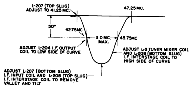
Figure 5 - Video I.F. Phased Pattern
