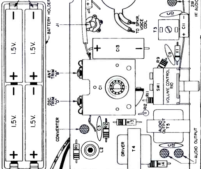
TOP VIEW OF PRINTED CIRCUIT CHASSIS
