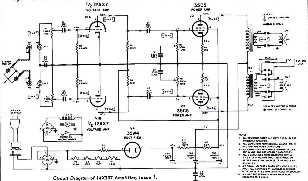
Circuit Diagram of 14X307 Amplifier, Issue 1.
