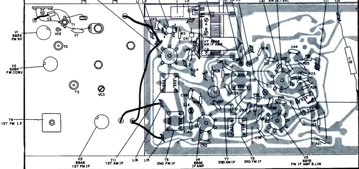
Top View - Showing Alignment Points, Tube Locations and Tie Lugs
