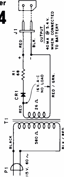
Schematic Diagram of Battery Charger Unit
