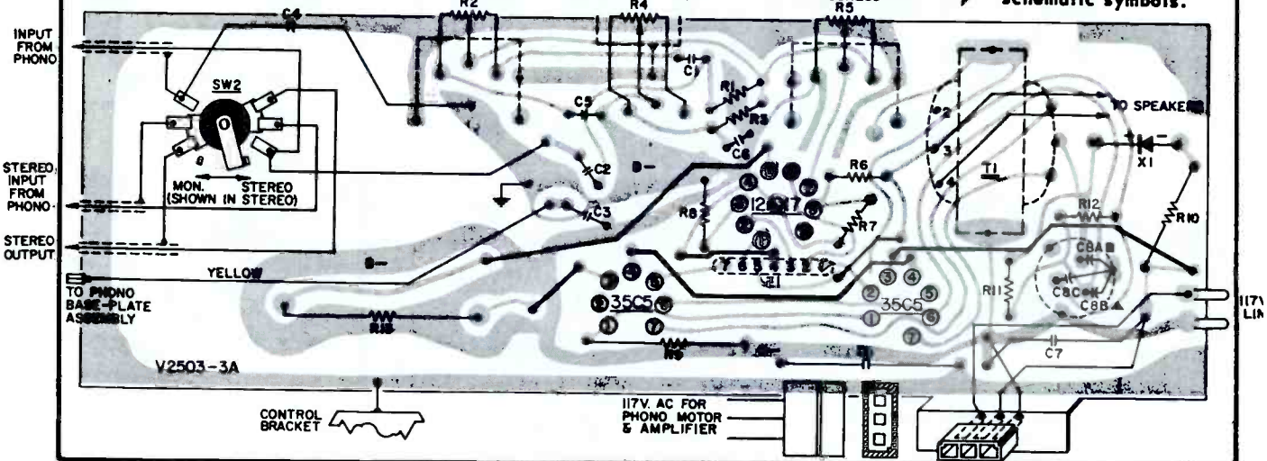
Bottom view of PC board showing top components as schematic symbols.
