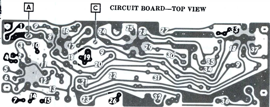
WHITE NUMBERS ON PRINTED CIRCUIT BOARD DRAWING CORRESPOND TO NUMBERS ENCIRCLED ON SCHEMATIC.
