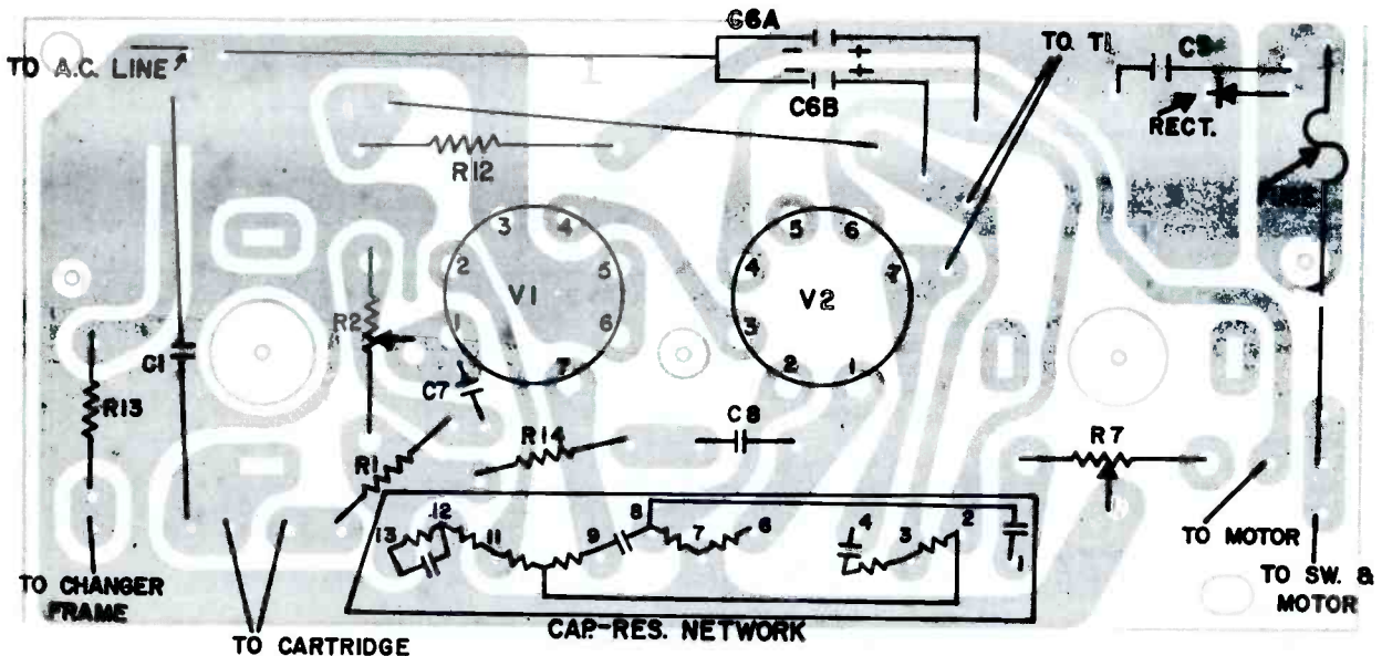
COMPONENT LOCATIONS - BOTTOM VIEW
