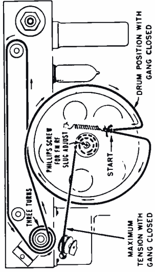
Dial Stringing (Chassis 7N1A).
