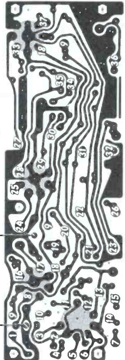
PARTS LAYOUT—CHASSIS VIEW
