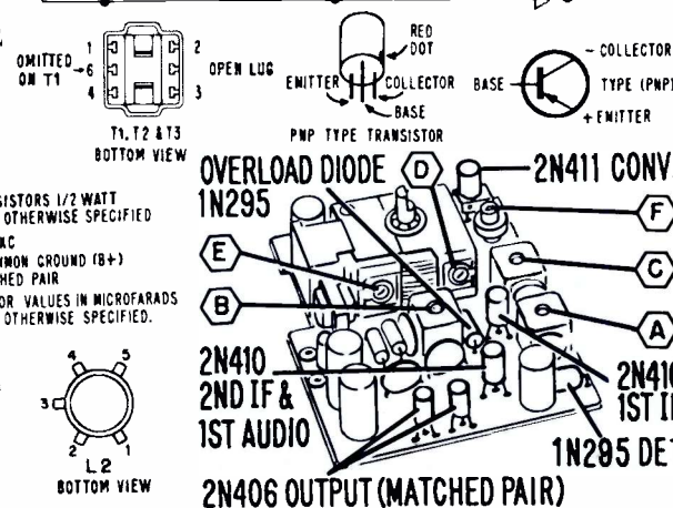
Transistor and Alignment Locations
