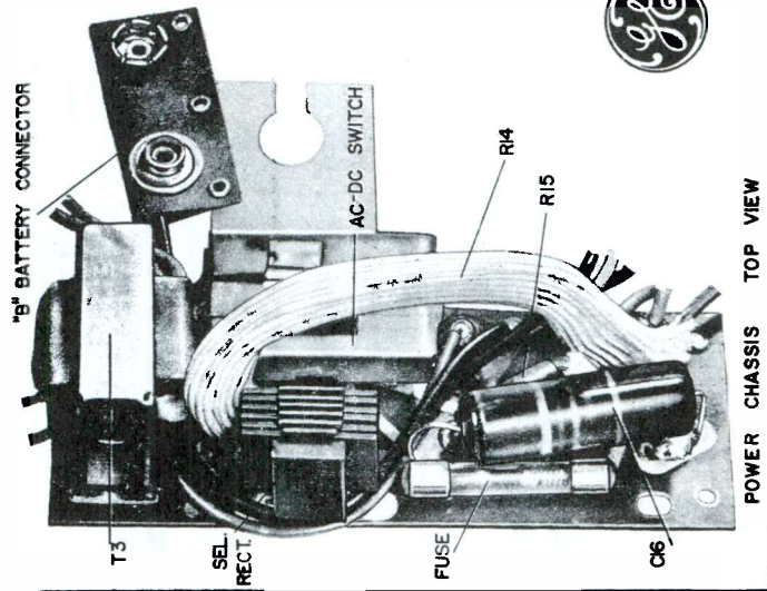
POWER CHASSIS TOP VIEW
