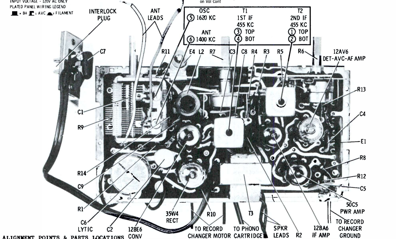
ALIGNMENT POINTS & PARTS LOCATIONS
